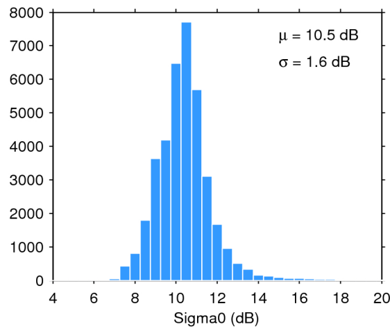
Figure 28. Histogram of science-valid sigma0 over oceans and lakes for 04/10/2017. The mean ( \mu ) and standard deviation ( \sigma ) are also shown. Note that values outside [4 20] dB are excluded from the histogram for the sake of readability but not from the computation of \mu and \sigma .
