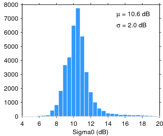
Figure 25. Histogram of flag-valid sigma0 over oceans and lakes for 04/10/2017. The mean ( \mu ) and standard deviation ( \sigma ) are also shown. Note that values outside [4 20] dB are excluded from the histogram for the sake of readability but not from the computation of \mu and \sigma .
