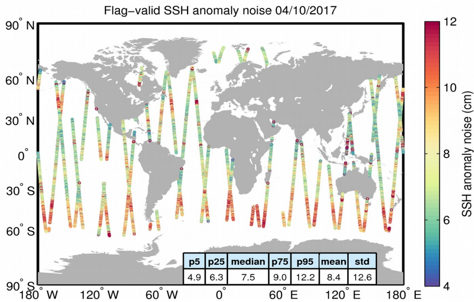
Figure 8. Geographical distribution of flag-valid 20-Hz SSH anomaly measurement noise over oceans and lakes for 04/10/2017. The statistical values shown in the table refer to the SSH anomaly noise and are calculated over all measurements shown in the figure.
