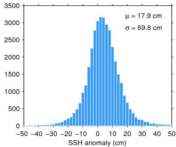
Figure 7. Histogram of flag-valid SSH anomaly over oceans and lakes for 04/10/2017. The mean ( \mu ) and standard deviation ( \sigma ) are also shown. Note that values outside [-50 50] cm are excluded from the histogram for the sake of readability but not from the computation of \mu and \sigma .
