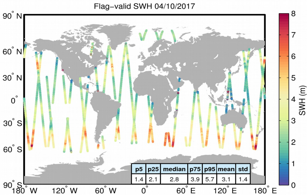
Figure 15. Geographical distribution of flag-valid SWH data over oceans and lakes for 04/10/2017. The statistical values shown in the table refer to the SWH in m and are calculated over all measurements shown in the figure.
