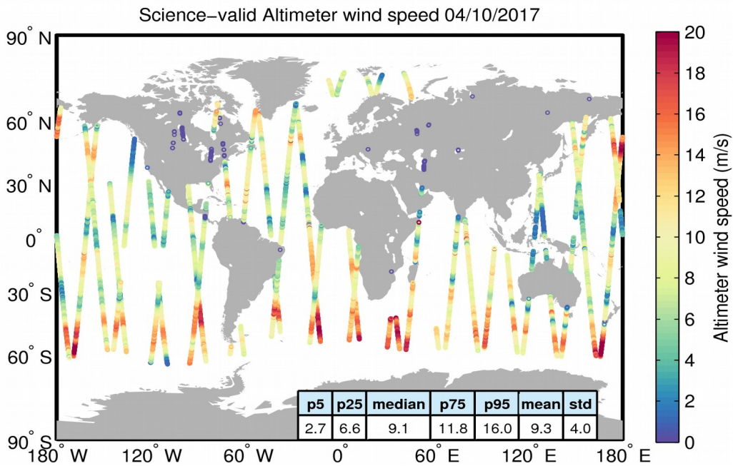
Figure 34. Geographical distribution of science-valid wind data over oceans and lakes for 04/10/2017. The statistical values shown in the table refer to the wind in m/s and are calculated over all measurements shown in the figure. Gray circles denote records that have been rejected based on the editing criteria described in Table 5.
