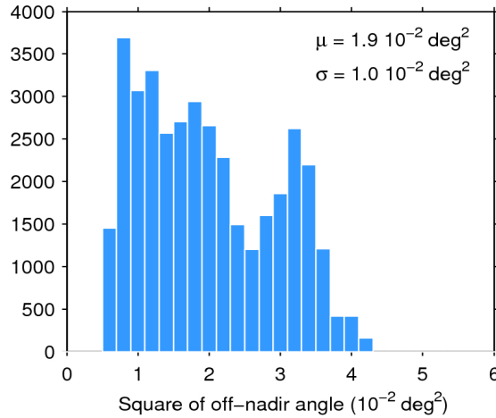
Figure 39. Histogram of flag-valid mispointing over oceans and lakes for 04/10/2017. The mean ( \mu ) and standard deviation ( \sigma ) are also shown. Note that values larger than 6 \cdot 10^{-2} \text{ deg}^2 are excluded from the histogram for the sake of readability but not from the computation of \mu and \sigma .
