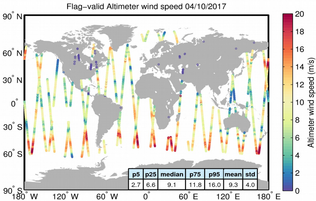
Figure 31. Geographical distribution of flag-valid wind data over oceans and lakes for 04/10/2017. The statistical values shown in the table refer to the wind in m/s and are calculated over all measurements shown in the figure.
