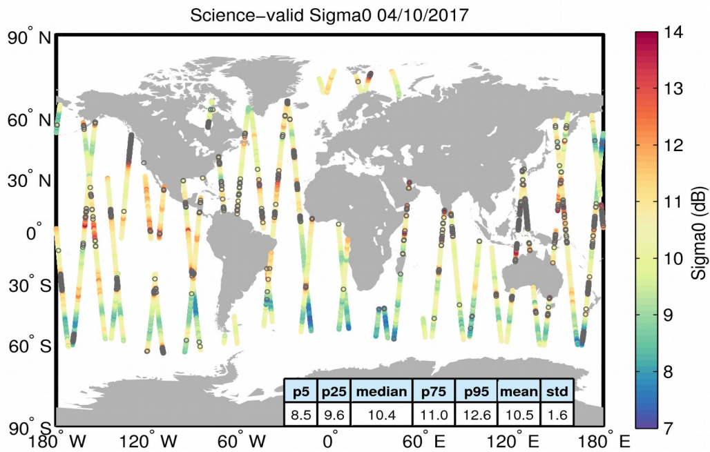
Figure 27. Geographical distribution of science-valid sigma0 data over oceans and lakes for 04/10/2017. The statistical values shown in the table refer to the sigma0 in dB and are calculated over all measurements shown in the figure. Gray circles denote records that have been rejected based on the editing criteria described in Table 4.
