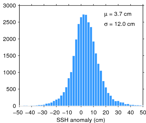
Figure 11. Histogram of science-valid SSH anomaly over oceans and lakes for 04/10/2017. The mean ( \mu ) and standard deviation ( \sigma ) are also shown. Note that values outside [-50 50] cm are excluded from the histogram for the sake of readability but not from the computation of \mu and \sigma .
