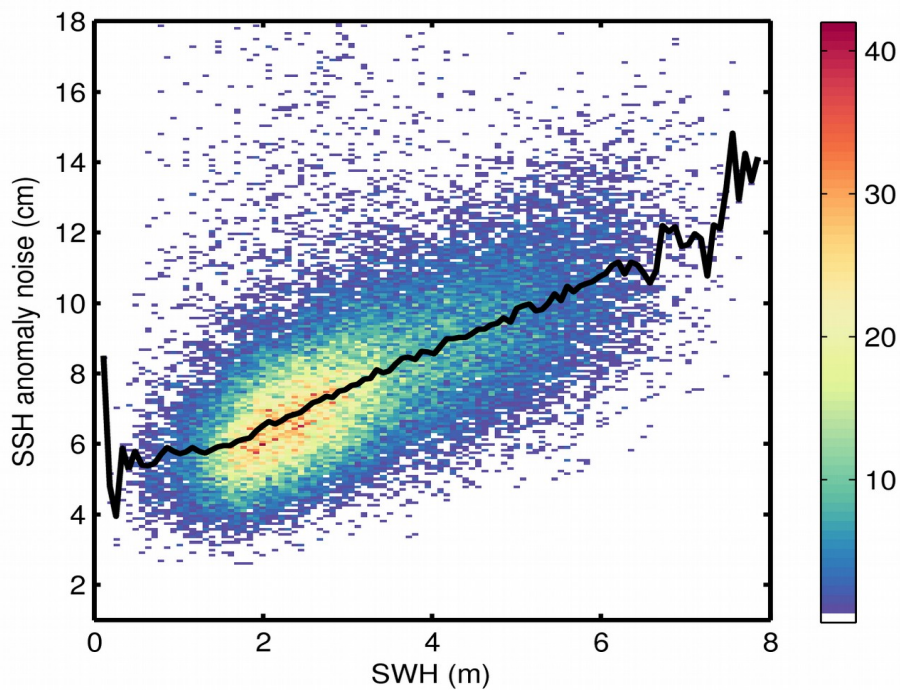
Figure 9. 2D histogram showing flag-valid SSH anomaly noise as a function of SWH for 04/10/2017. The black line denotes the median SSH anomaly noise as a function of SWH.
