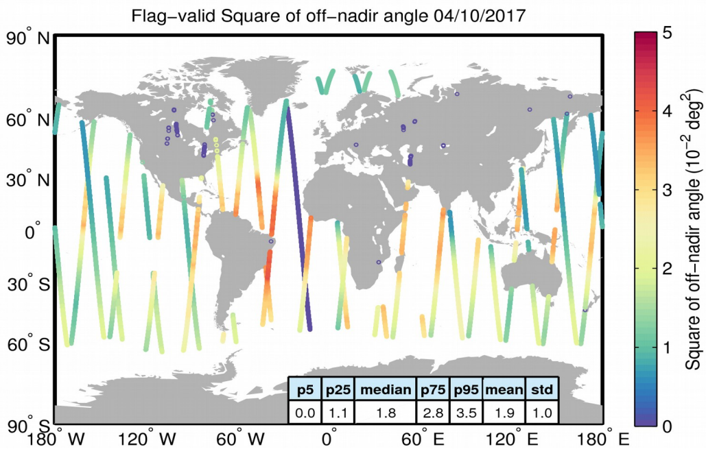
Figure 37. Geographical distribution of flag-valid mispointing data over oceans and lakes for 04/10/2017. The statistical values shown in the table refer to the mispointing in 10^{-2} \text{ deg}^2 and are calculated over all measurements shown in the figure.
