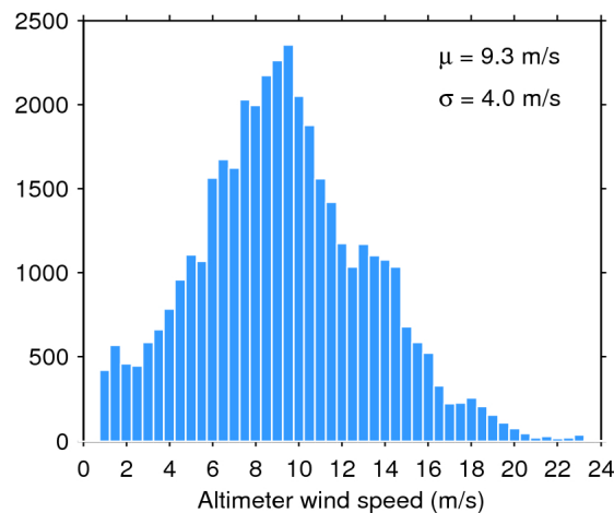
Figure 35. Histogram of science-valid wind over oceans and lakes for 04/10/2017. The mean ( \mu ) and standard deviation ( \sigma ) are also shown. Note that values larger than 24 m/s are excluded from the histogram for the sake of readability but not from the computation of \mu and \sigma .
