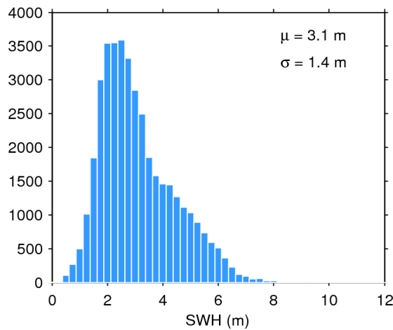
Figure 17. Histogram of flag-valid SWH over oceans and lakes for 04/10/2017. The mean ( \mu ) and standard deviation ( \sigma ) are also shown. Note that values larger than 12 m are excluded from the histogram for the sake of readability but not from the computation of \mu and \sigma .
