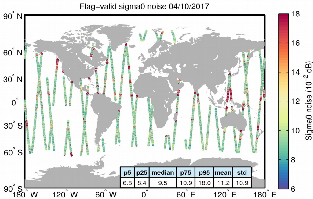
Figure 26. Geographical distribution of flag-valid 20-Hz sigma0 measurement noise over oceans and lakes for 04/10/2017. The statistical values shown in the table refer to the sigma0 noise and are calculated over all measurements shown in the figure.
