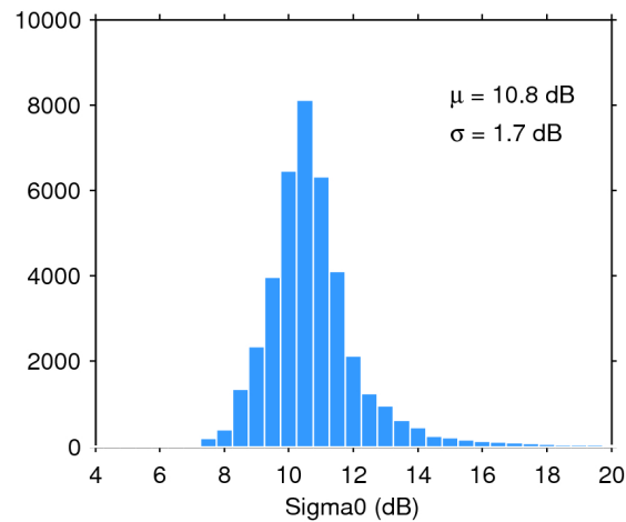
Figure 25. Histogram of flag-valid sigma0 over oceans and lakes for 03/10/2017. The mean ( \mu ) and standard deviation ( \sigma ) are also shown. Note that values outside [4 20] dB are excluded from the histogram for the sake of readability but not from the computation of \mu and \sigma .
