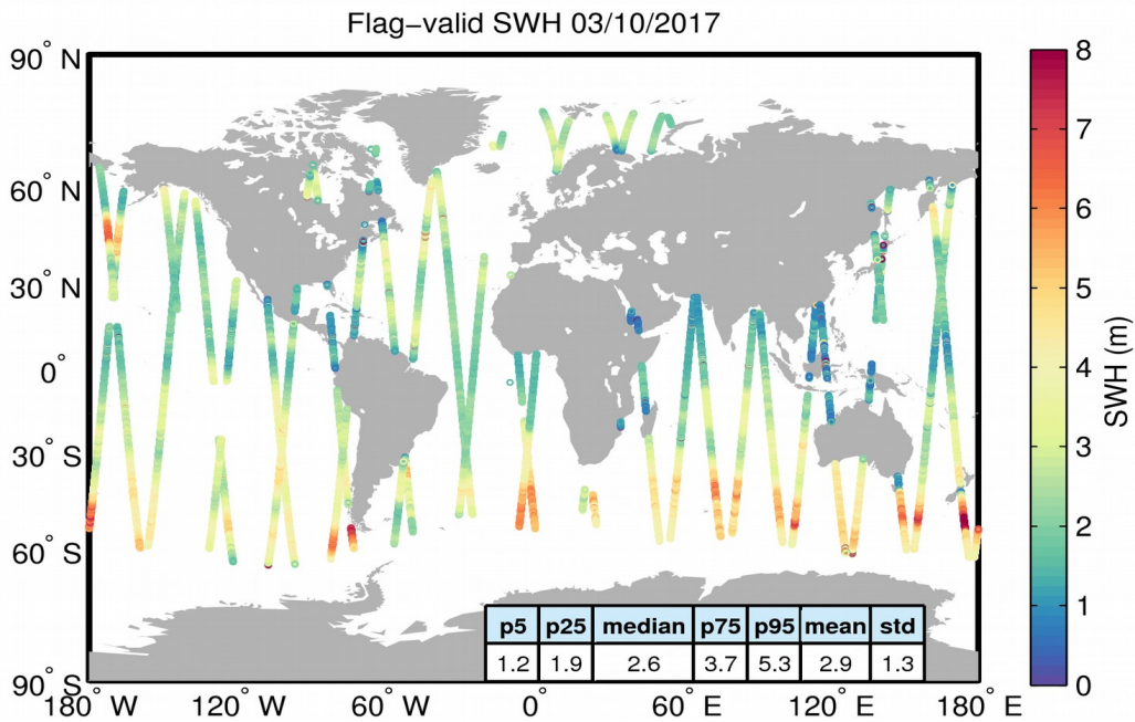
Figure 15. Geographical distribution of flag-valid SWH data over oceans and lakes for 03/10/2017. The statistical values shown in the table refer to the SWH in m and are calculated over all measurements shown in the figure.
