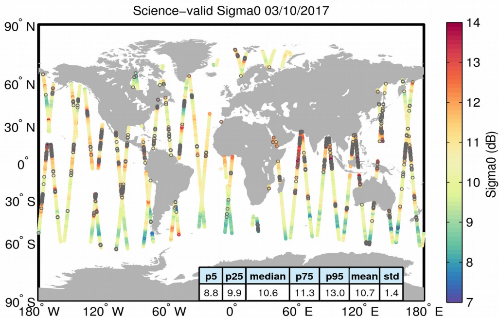
Figure 27. Geographical distribution of science-valid sigma0 data over oceans and lakes for 03/10/2017. The statistical values shown in the table refer to the sigma0 in dB and are calculated over all measurements shown in the figure. Gray circles denote records that have been rejected based on the editing criteria described in Table 4.
