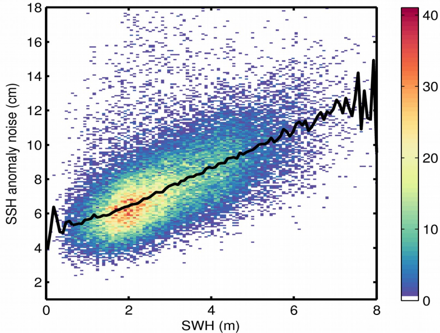
Figure 9. 2D histogram showing flag-valid SSH anomaly noise as a function of SWH for 03/10/2017. The black line denotes the median SSH anomaly noise as a function of SWH.
