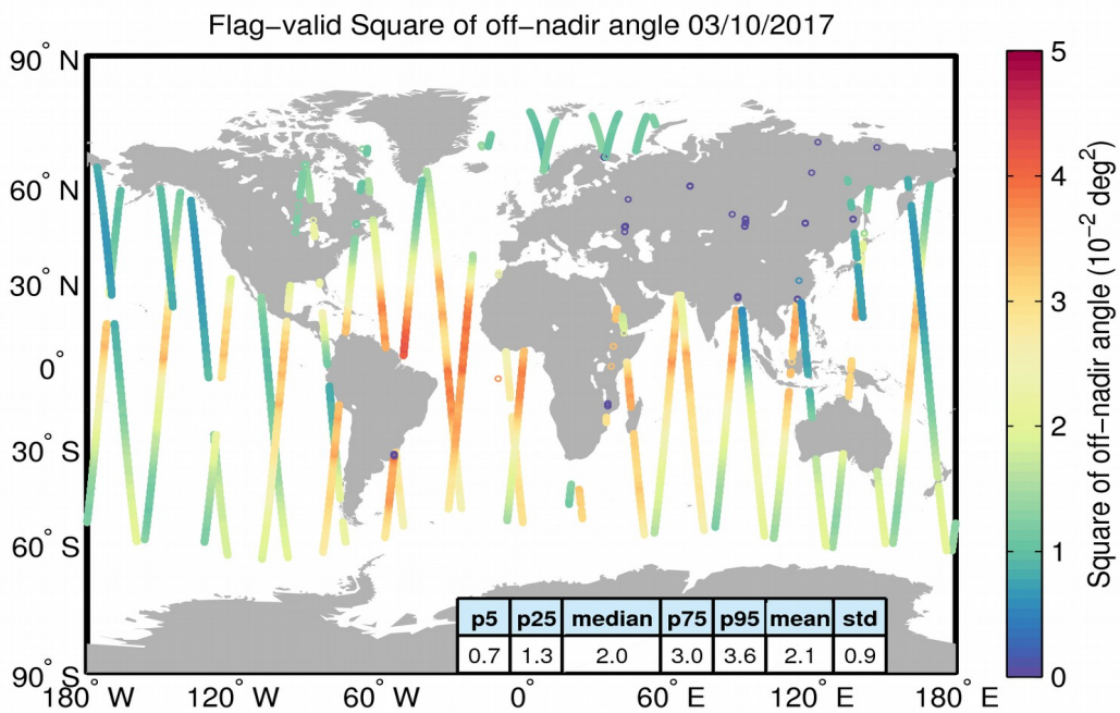
Figure 37. Geographical distribution of flag-valid mispointing data over oceans and lakes for 03/10/2017. The statistical values shown in the table refer to the mispointing in 10^{-2} deg 2 and are calculated over all measurements shown in the figure.
