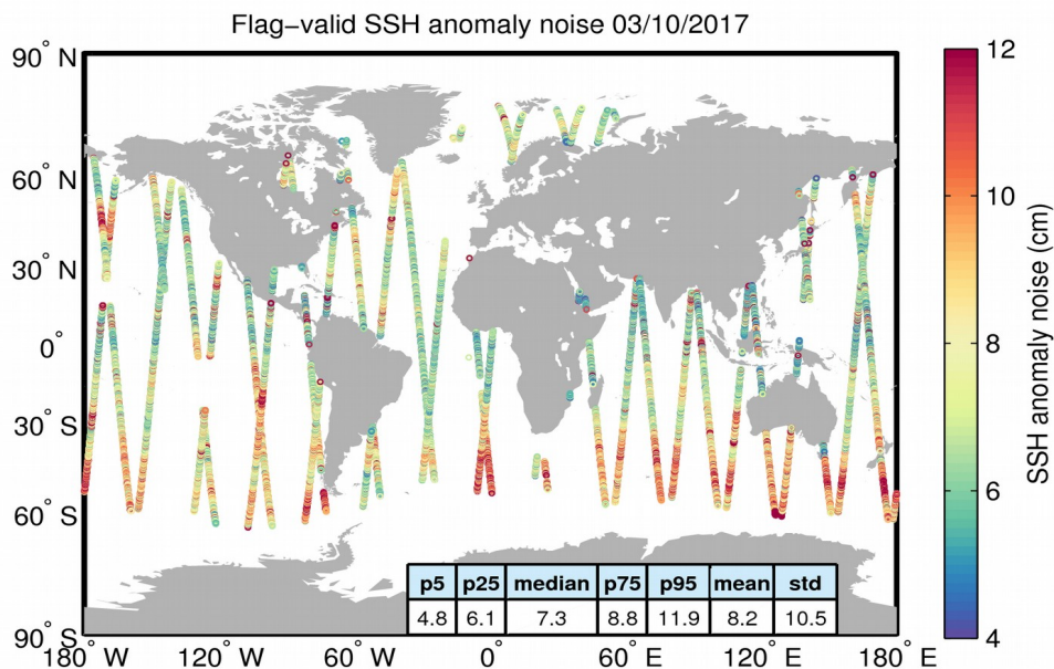
Figure 8. Geographical distribution of flag-valid 20-Hz SSH anomaly measurement noise over oceans and lakes for 03/10/2017. The statistical values shown in the table refer to the SSH anomaly noise and are calculated over all measurements shown in the figure.
