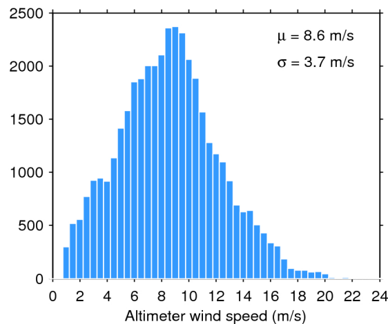
Figure 35. Histogram of science-valid wind over oceans and lakes for 03/10/2017. The mean ( \mu ) and standard deviation ( \sigma ) are also shown. Note that values larger than 24 m/s are excluded from the histogram for the sake of readability but not from the computation of \mu and \sigma .
