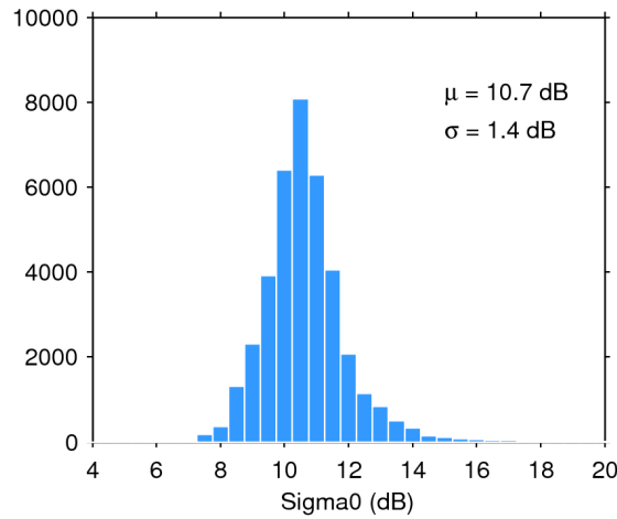
Figure 28. Histogram of science-valid sigma0 over oceans and lakes for 03/10/2017. The mean ( \mu ) and standard deviation ( \sigma ) are also shown. Note that values outside [4 20] dB are excluded from the histogram for the sake of readability but not from the computation of \mu and \sigma .
