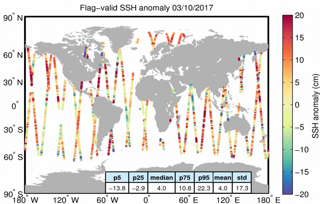
Figure 5. Geographical distribution of flag-valid 1-Hz SSH anomaly data over oceans and lakes for 03/10/2017. The statistical values shown in the table refer to the SSH anomaly in cm and are calculated over all measurements shown in the figure.
