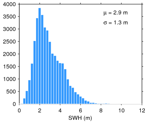
Figure 17. Histogram of flag-valid SWH over oceans and lakes for 03/10/2017. The mean ( \mu ) and standard deviation ( \sigma ) are also shown. Note that values larger than 12 m are excluded from the histogram for the sake of readability but not from the computation of \mu and \sigma .
