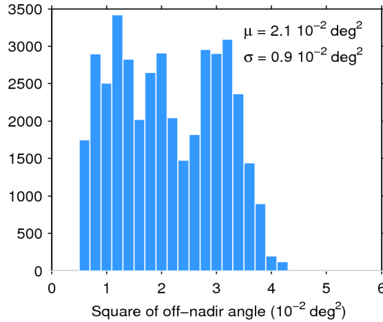
Figure 39. Histogram of flag-valid mispointing over oceans and lakes for 03/10/2017. The mean ( \mu ) and standard deviation ( \sigma ) are also shown. Note that values larger than 6 \cdot 10^{-2} \text{ deg}^2 are excluded from the histogram for the sake of readability but not from the computation of \mu and \sigma .
