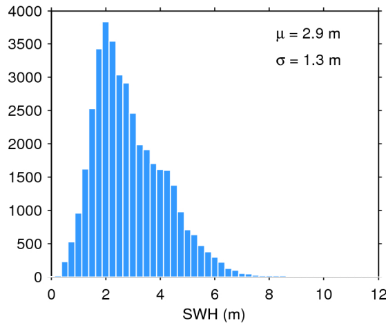
Figure 20. Histogram of science-valid SWH over oceans and lakes for 03/10/2017. The mean ( \mu ) and standard deviation ( \sigma ) are also shown. Note that values larger than 12 m are excluded from the histogram for the sake of readability but not from the computation of \mu and \sigma .
