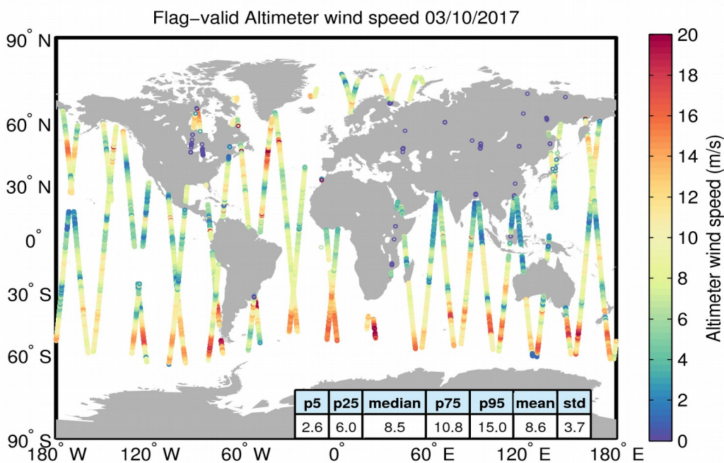
Figure 31. Geographical distribution of flag-valid wind data over oceans and lakes for 03/10/2017. The statistical values shown in the table refer to the wind in m/s and are calculated over all measurements shown in the figure.
