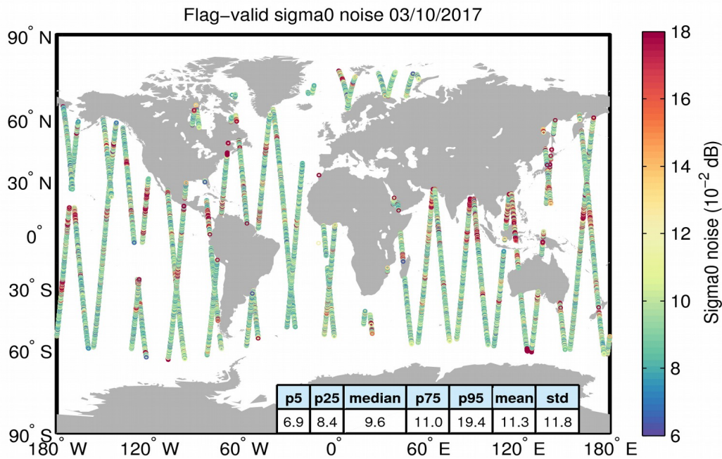
Figure 26. Geographical distribution of flag-valid 20-Hz sigma0 measurement noise over oceans and lakes for 03/10/2017. The statistical values shown in the table refer to the sigma0 noise and are calculated over all measurements shown in the figure.
