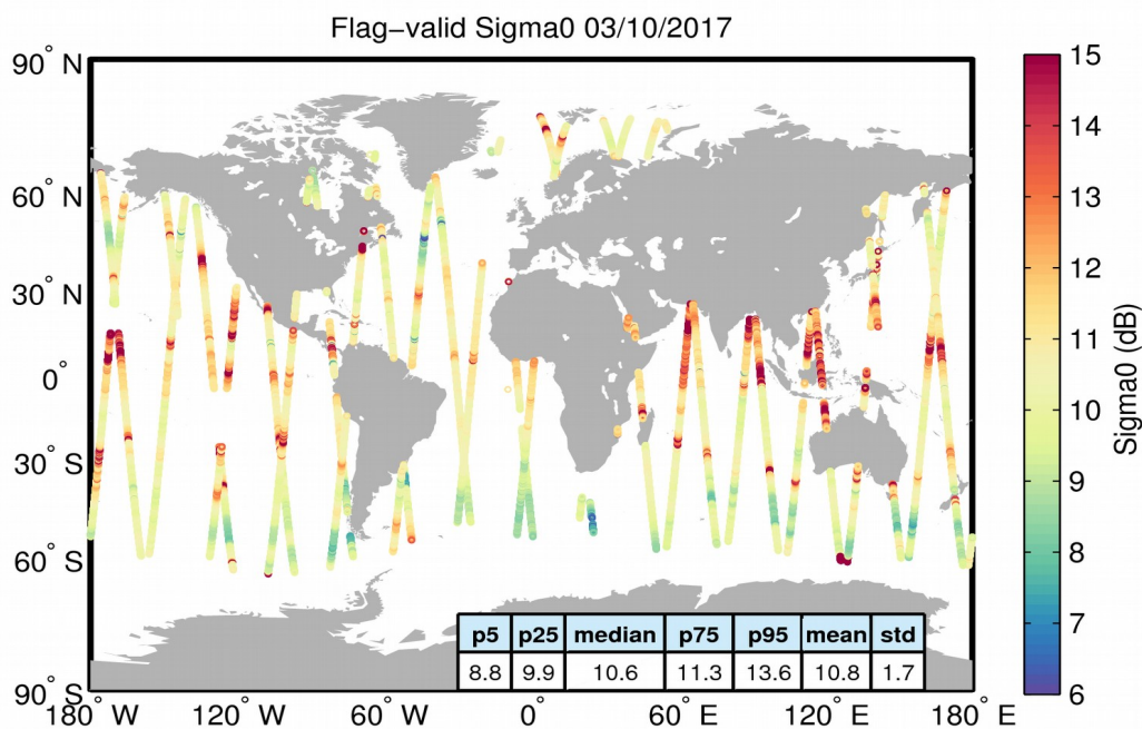
Figure 23. Geographical distribution of flag-valid sigma0 data over oceans and lakes for 03/10/2017. The statistical values shown in the table refer to the sigma0 in dB and are calculated over all measurements shown in the figure.
