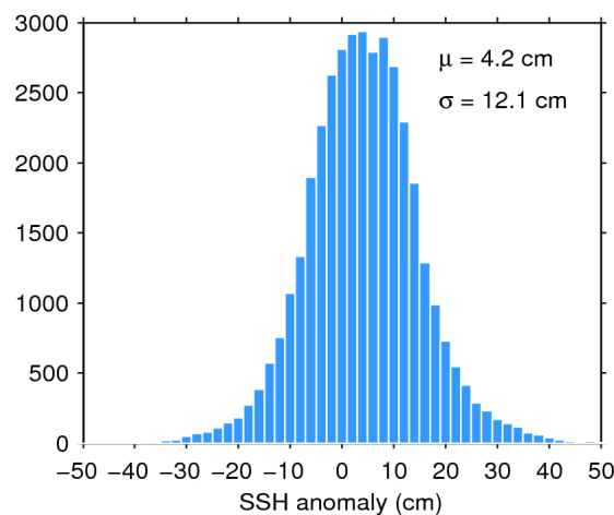
Figure 11. Histogram of science-valid SSH anomaly over oceans and lakes for 03/10/2017. The mean ( \mu ) and standard deviation ( \sigma ) are also shown. Note that values outside [-50 50] cm are excluded from the histogram for the sake of readability but not from the computation of \mu and \sigma .
