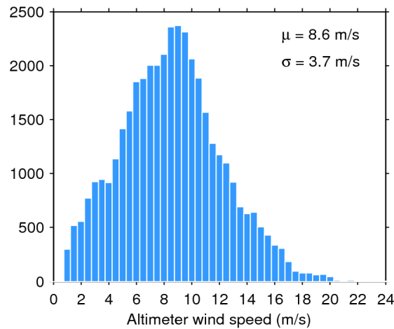
Figure 33. Histogram of flag-valid wind over oceans and lakes for 03/10/2017. The mean ( \mu ) and standard deviation ( \sigma ) are also shown. Note that values larger than 24 m/s are excluded from the histogram for the sake of readability but not from the computation of \mu and \sigma .
