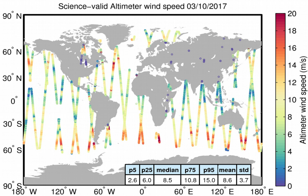
Figure 34. Geographical distribution of science-valid wind data over oceans and lakes for 03/10/2017. The statistical values shown in the table refer to the wind in m/s and are calculated over all measurements shown in the figure. Gray circles denote records that have been rejected based on the editing criteria described in Table 5.
