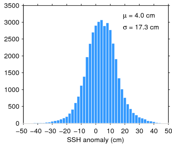
Figure 7. Histogram of flag-valid SSH anomaly over oceans and lakes for 03/10/2017. The mean ( \mu ) and standard deviation ( \sigma ) are also shown. Note that values outside [-50 50] cm are excluded from the histogram for the sake of readability but not from the computation of \mu and \sigma .
