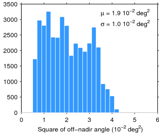
Figure 39. Histogram of flag-valid mispointing over oceans and lakes for 02/10/2017. The mean ( \mu ) and standard deviation ( \sigma ) are also shown. Note that values larger than 6 \cdot 10^{-2} \text{ deg}^2 are excluded from the histogram for the sake of readability but not from the computation of \mu and \sigma .
