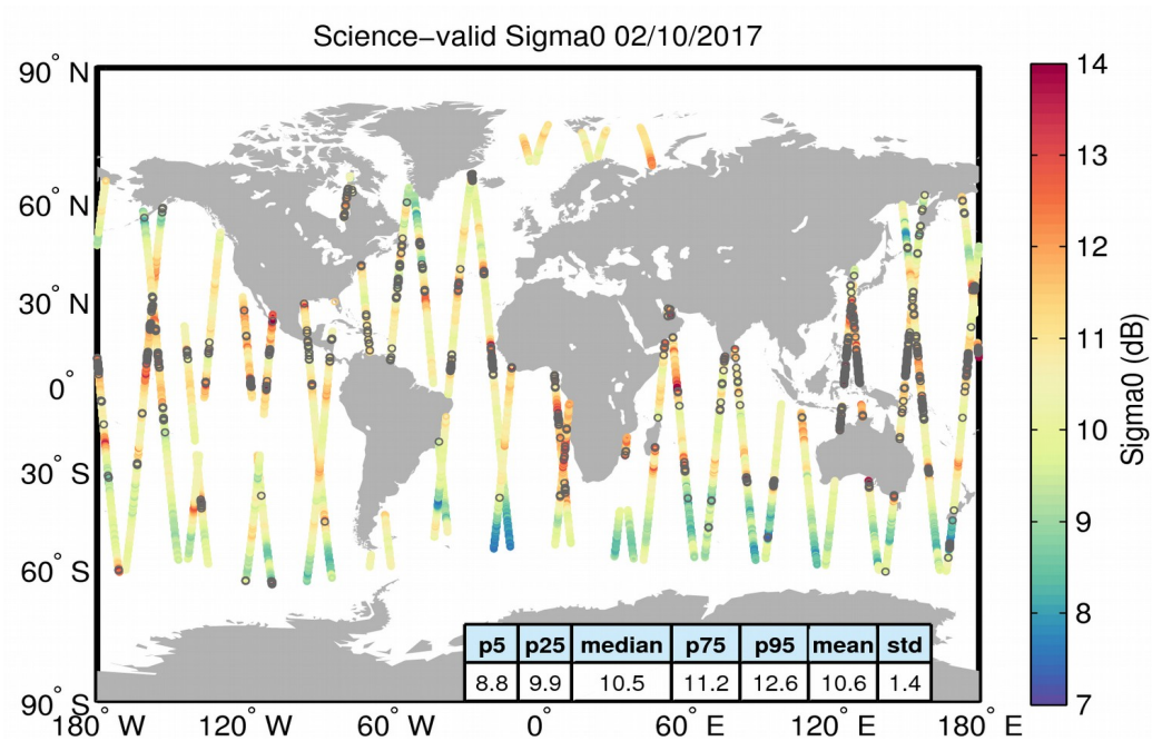
Figure 27. Geographical distribution of science-valid sigma0 data over oceans and lakes for 02/10/2017. The statistical values shown in the table refer to the sigma0 in dB and are calculated over all measurements shown in the figure. Gray circles denote records that have been rejected based on the editing criteria described in Table 4.
