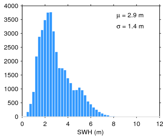
Figure 17. Histogram of flag-valid SWH over oceans and lakes for 02/10/2017. The mean ( \mu ) and standard deviation ( \sigma ) are also shown. Note that values larger than 12 m are excluded from the histogram for the sake of readability but not from the computation of \mu and \sigma .
