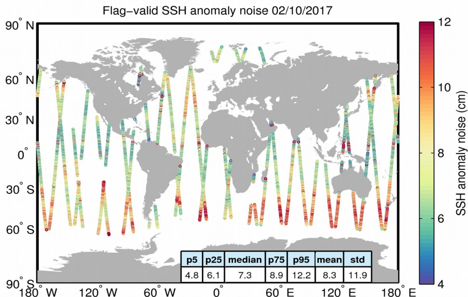
Figure 8. Geographical distribution of flag-valid 20-Hz SSH anomaly measurement noise over oceans and lakes for 02/10/2017. The statistical values shown in the table refer to the SSH anomaly noise and are calculated over all measurements shown in the figure.
