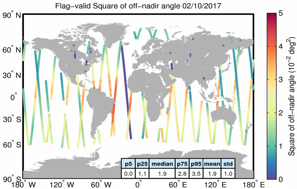
Figure 37. Geographical distribution of flag-valid mispointing data over oceans and lakes for 02/10/2017. The statistical values shown in the table refer to the mispointing in 10^{-2} deg 2 and are calculated over all measurements shown in the figure.
