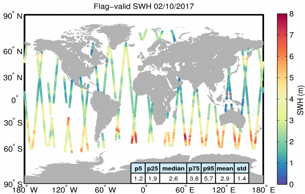
Figure 15. Geographical distribution of flag-valid SWH data over oceans and lakes for 02/10/2017. The statistical values shown in the table refer to the SWH in m and are calculated over all measurements shown in the figure.
