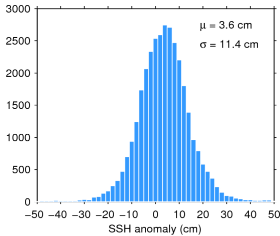
Figure 11. Histogram of science-valid SSH anomaly over oceans and lakes for 02/10/2017. The mean ( \mu ) and standard deviation ( \sigma ) are also shown. Note that values outside [-50 50] cm are excluded from the histogram for the sake of readability but not from the computation of \mu and \sigma .
