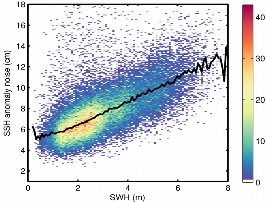
Figure 9. 2D histogram showing flag-valid SSH anomaly noise as a function of SWH for 02/10/2017. The black line denotes the median SSH anomaly noise as a function of SWH.
