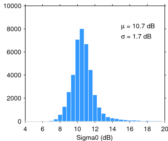
Figure 25. Histogram of flag-valid sigma0 over oceans and lakes for 02/10/2017. The mean ( \mu ) and standard deviation ( \sigma ) are also shown. Note that values outside [4 20] dB are excluded from the histogram for the sake of readability but not from the computation of \mu and \sigma .
