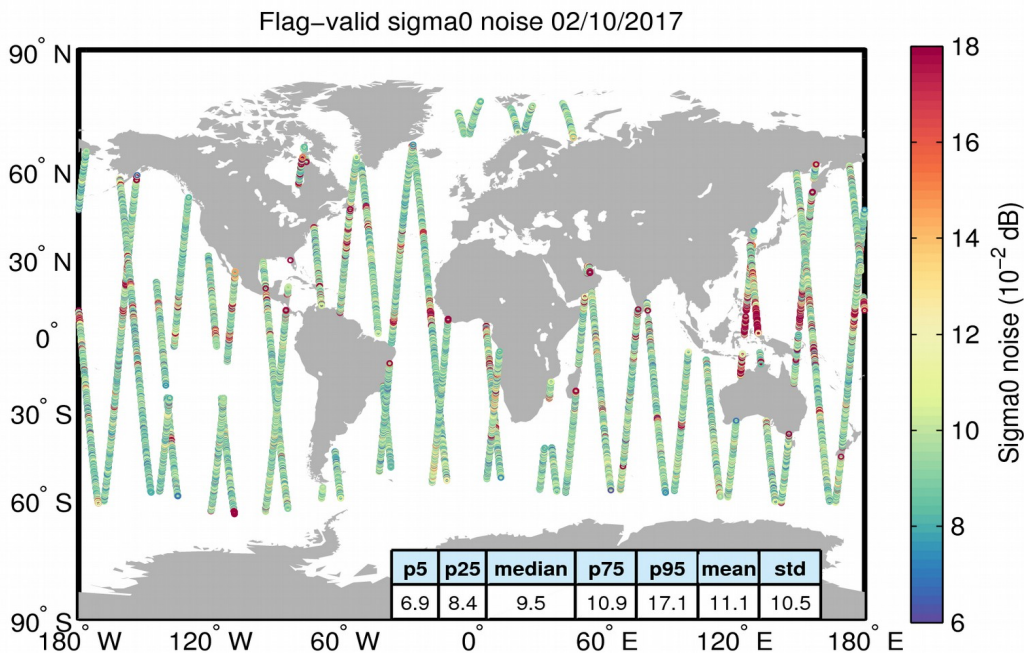
Figure 26. Geographical distribution of flag-valid 20-Hz sigma0 measurement noise over oceans and lakes for 02/10/2017. The statistical values shown in the table refer to the sigma0 noise and are calculated over all measurements shown in the figure.
