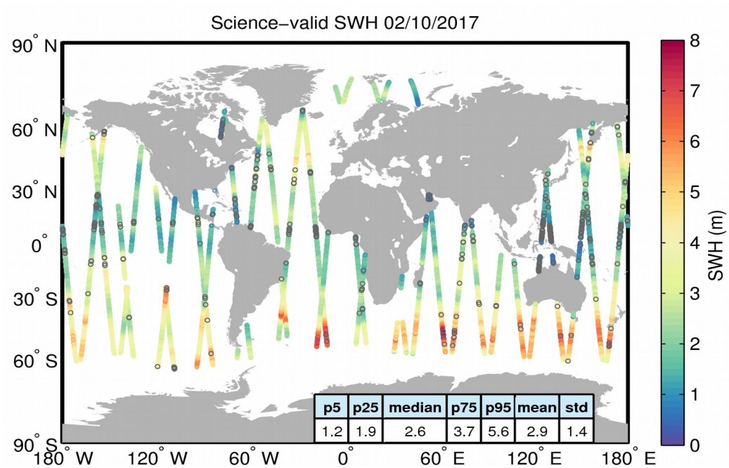
Figure 19. Geographical distribution of science-valid SWH data over oceans and lakes for 02/10/2017. The statistical values shown in the table refer to the SWH in m and are calculated over all measurements shown in the figure. Gray circles denote records that have been rejected based on the editing criteria described in Table 3.
