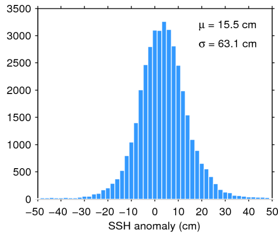
Figure 7. Histogram of flag-valid SSH anomaly over oceans and lakes for 02/10/2017. The mean ( \mu ) and standard deviation ( \sigma ) are also shown. Note that values outside [-50 50] cm are excluded from the histogram for the sake of readability but not from the computation of \mu and \sigma .
