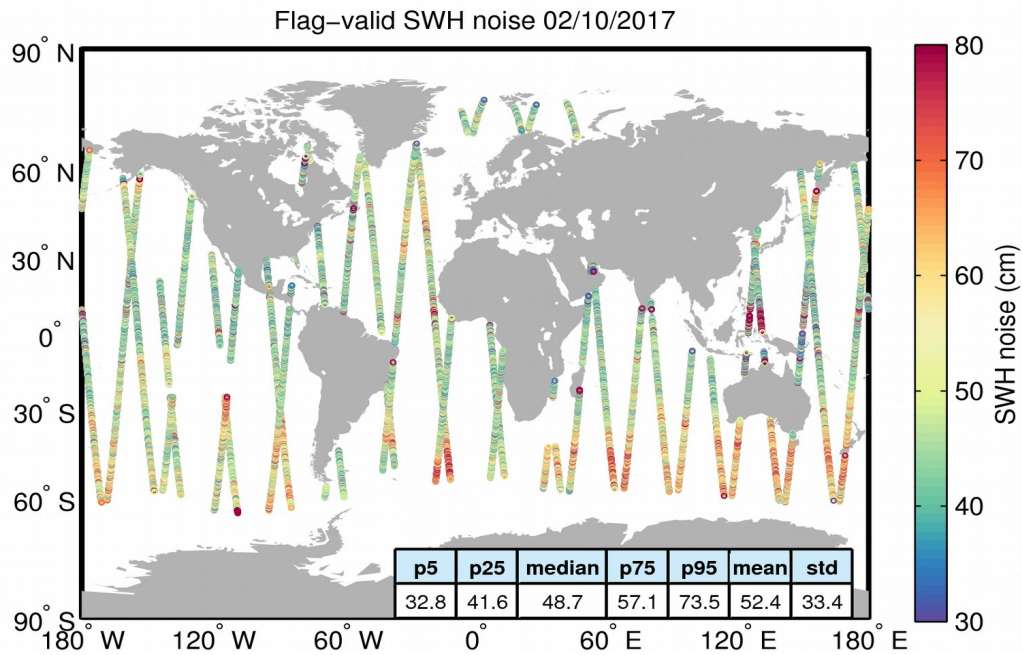
Figure 18. Geographical distribution of flag-valid 20-Hz SWH measurement noise over oceans and lakes for 02/10/2017. The statistical values shown in the table refer to the SWH noise and are calculated over all measurements shown in the figure.
