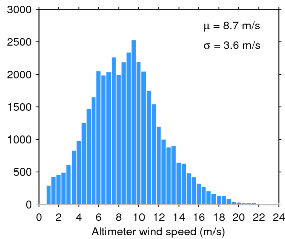
Figure 33. Histogram of flag-valid wind over oceans and lakes for 02/10/2017. The mean ( \mu ) and standard deviation ( \sigma ) are also shown. Note that values larger than 24 m/s are excluded from the histogram for the sake of readability but not from the computation of \mu and \sigma .
