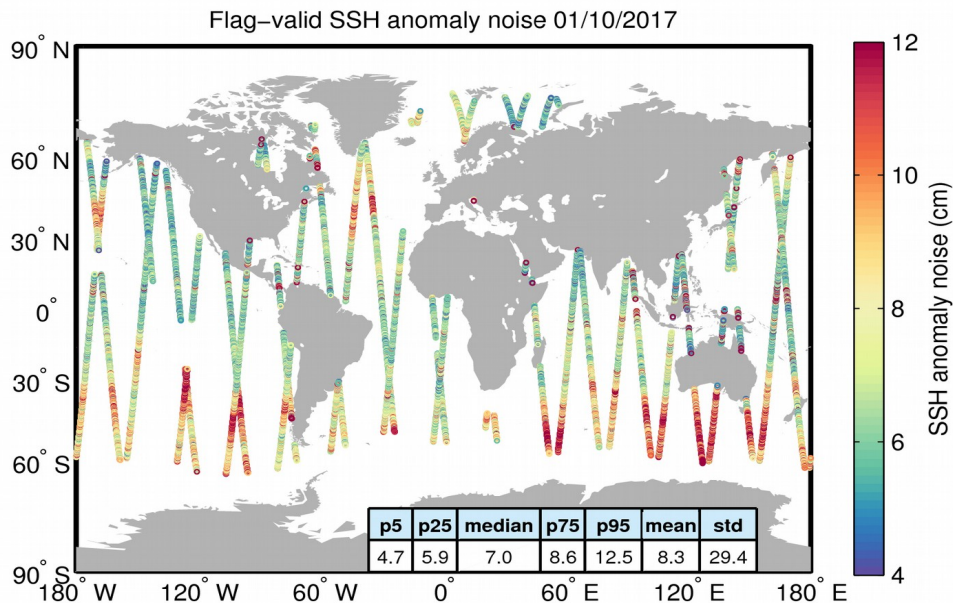
Figure 8. Geographical distribution of flag-valid 20-Hz SSH anomaly measurement noise over oceans and lakes for 01/10/2017. The statistical values shown in the table refer to the SSH anomaly noise and are calculated over all measurements shown in the figure.
