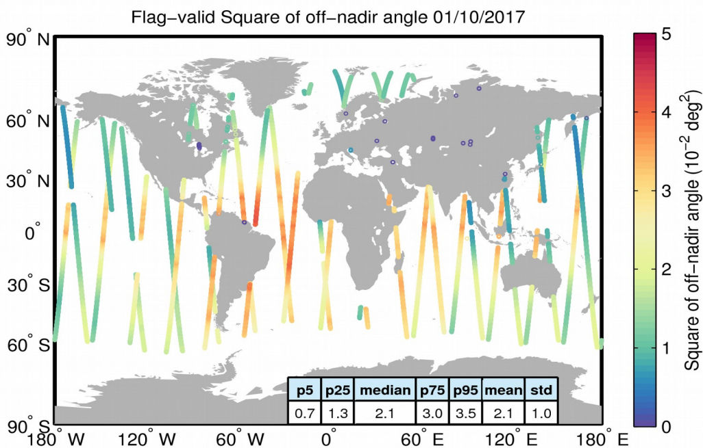
Figure 37. Geographical distribution of flag-valid mispointing data over oceans and lakes for 01/10/2017. The statistical values shown in the table refer to the mispointing in 10^{-2} deg 2 and are calculated over all measurements shown in the figure.
