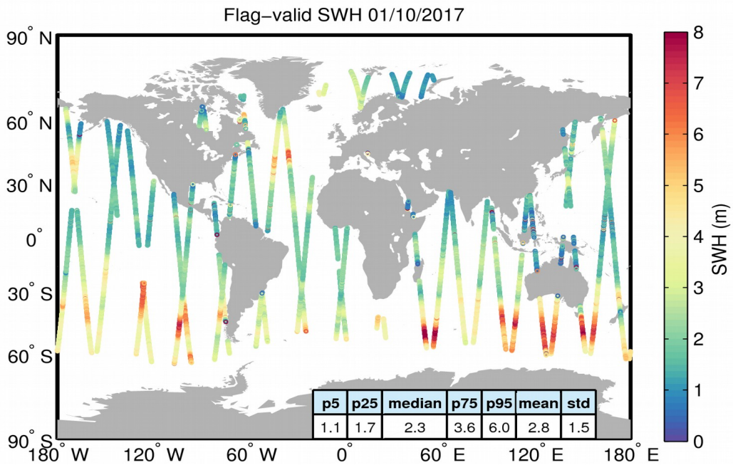
Figure 15. Geographical distribution of flag-valid SWH data over oceans and lakes for 01/10/2017. The statistical values shown in the table refer to the SWH in m and are calculated over all measurements shown in the figure.
