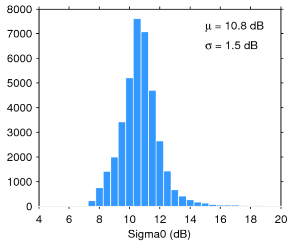
Figure 28. Histogram of science-valid sigma0 over oceans and lakes for 01/10/2017. The mean ( \mu ) and standard deviation ( \sigma ) are also shown. Note that values outside [4 20] dB are excluded from the histogram for the sake of readability but not from the computation of \mu and \sigma .
