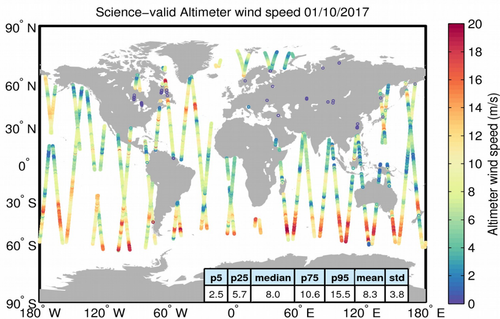
Figure 34. Geographical distribution of science-valid wind data over oceans and lakes for 01/10/2017. The statistical values shown in the table refer to the wind in m/s and are calculated over all measurements shown in the figure. Gray circles denote records that have been rejected based on the editing criteria described in Table 5.
