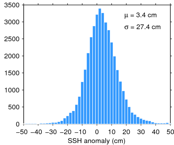
Figure 7. Histogram of flag-valid SSH anomaly over oceans and lakes for 01/10/2017. The mean ( \mu ) and standard deviation ( \sigma ) are also shown. Note that values outside [-50 50] cm are excluded from the histogram for the sake of readability but not from the computation of \mu and \sigma .
