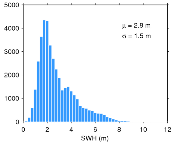
Figure 17. Histogram of flag-valid SWH over oceans and lakes for 01/10/2017. The mean ( \mu ) and standard deviation ( \sigma ) are also shown. Note that values larger than 12 m are excluded from the histogram for the sake of readability but not from the computation of \mu and \sigma .
