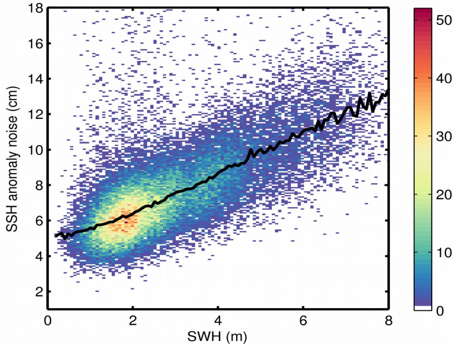
Figure 9. 2D histogram showing flag-valid SSH anomaly noise as a function of SWH for 01/10/2017. The black line denotes the median SSH anomaly noise as a function of SWH.
