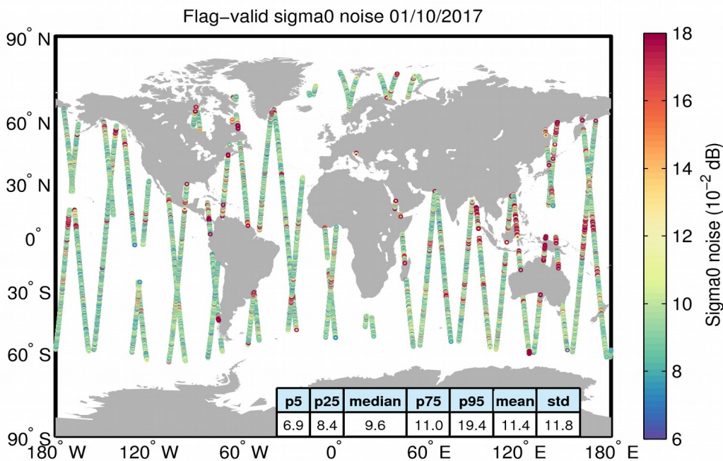
Figure 26. Geographical distribution of flag-valid 20-Hz sigma0 measurement noise over oceans and lakes for 01/10/2017. The statistical values shown in the table refer to the sigma0 noise and are calculated over all measurements shown in the figure.
