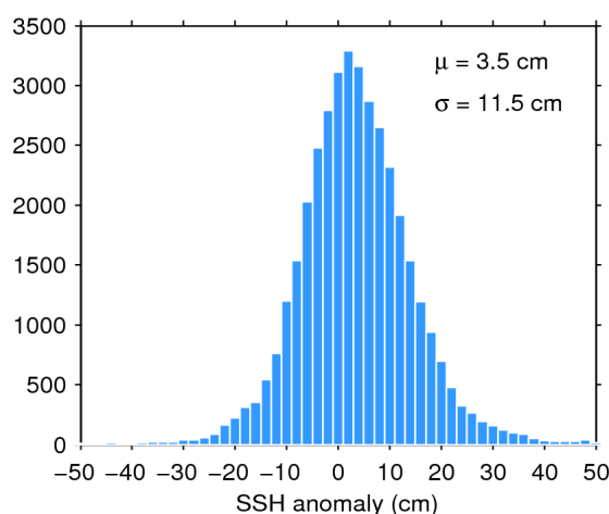
Figure 11. Histogram of science-valid SSH anomaly over oceans and lakes for 01/10/2017. The mean ( \mu ) and standard deviation ( \sigma ) are also shown. Note that values outside [-50 50] cm are excluded from the histogram for the sake of readability but not from the computation of \mu and \sigma .
