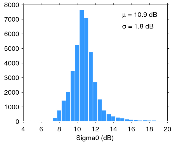
Figure 25. Histogram of flag-valid sigma0 over oceans and lakes for 01/10/2017. The mean ( \mu ) and standard deviation ( \sigma ) are also shown. Note that values outside [4 20] dB are excluded from the histogram for the sake of readability but not from the computation of \mu and \sigma .
