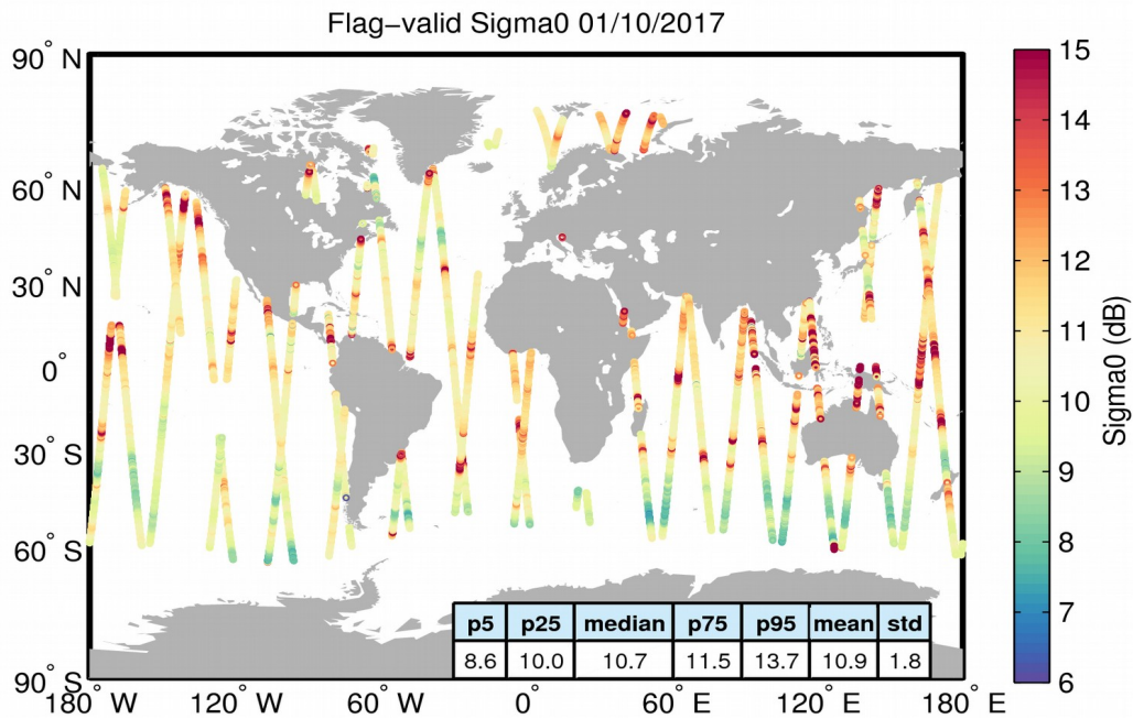
Figure 23. Geographical distribution of flag-valid sigma0 data over oceans and lakes for 01/10/2017. The statistical values shown in the table refer to the sigma0 in dB and are calculated over all measurements shown in the figure.
