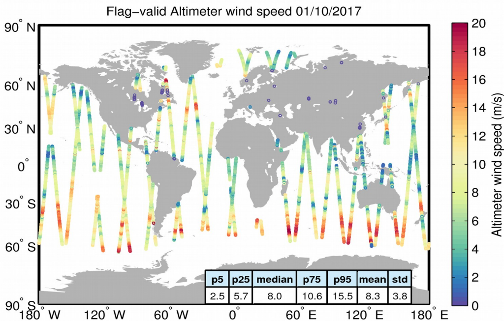
Figure 31. Geographical distribution of flag-valid wind data over oceans and lakes for 01/10/2017. The statistical values shown in the table refer to the wind in m/s and are calculated over all measurements shown in the figure.
