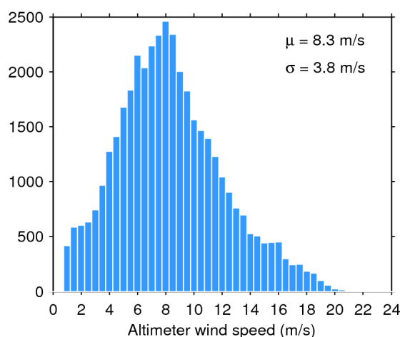
Figure 35. Histogram of science-valid wind over oceans and lakes for 01/10/2017. The mean ( \mu ) and standard deviation ( \sigma ) are also shown. Note that values larger than 24 m/s are excluded from the histogram for the sake of readability but not from the computation of \mu and \sigma .
