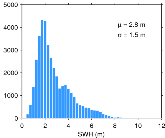
Figure 20. Histogram of science-valid SWH over oceans and lakes for 01/10/2017. The mean ( \mu ) and standard deviation ( \sigma ) are also shown. Note that values larger than 12 m are excluded from the histogram for the sake of readability but not from the computation of \mu and \sigma .
