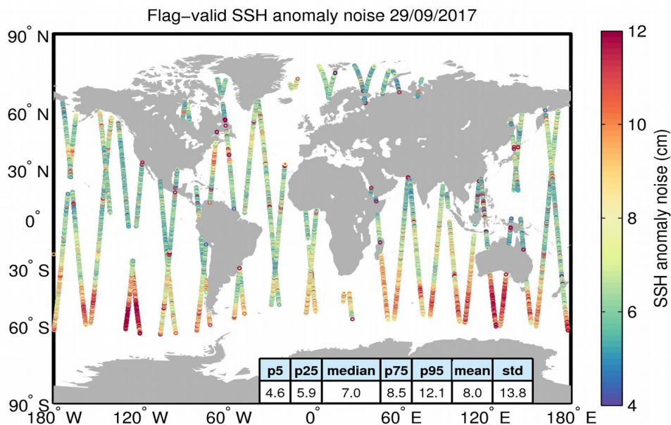
Figure 8. Geographical distribution of flag-valid 20-Hz SSH anomaly measurement noise over oceans and lakes for 29/09/2017. The statistical values shown in the table refer to the SSH anomaly noise and are calculated over all measurements shown in the figure.
