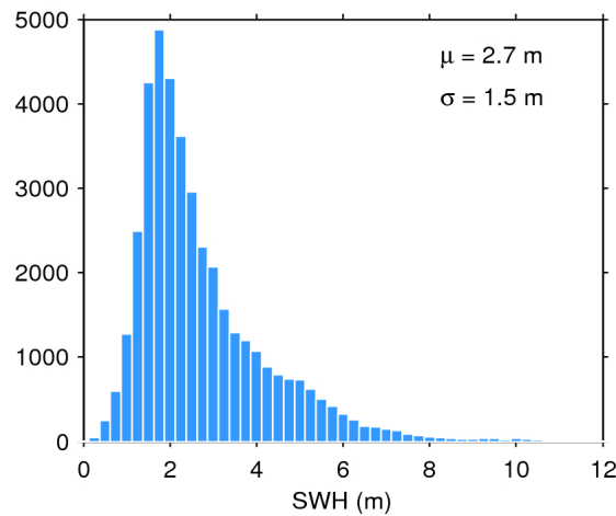
Figure 17. Histogram of flag-valid SWH over oceans and lakes for 29/09/2017. The mean ( \mu ) and standard deviation ( \sigma ) are also shown. Note that values larger than 12 m are excluded from the histogram for the sake of readability but not from the computation of \mu and \sigma .
