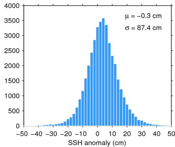
Figure 7. Histogram of flag-valid SSH anomaly over oceans and lakes for 29/09/2017. The mean ( \mu ) and standard deviation ( \sigma ) are also shown. Note that values outside [-50 50] cm are excluded from the histogram for the sake of readability but not from the computation of \mu and \sigma .
