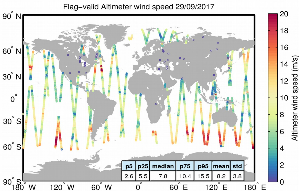
Figure 31. Geographical distribution of flag-valid wind data over oceans and lakes for 29/09/2017. The statistical values shown in the table refer to the wind in m/s and are calculated over all measurements shown in the figure.
