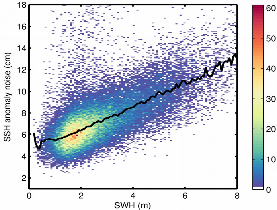
Figure 9. 2D histogram showing flag-valid SSH anomaly noise as a function of SWH for 29/09/2017. The black line denotes the median SSH anomaly noise as a function of SWH.
