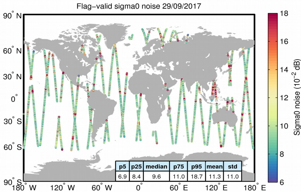
Figure 26. Geographical distribution of flag-valid 20-Hz sigma0 measurement noise over oceans and lakes for 29/09/2017. The statistical values shown in the table refer to the sigma0 noise and are calculated over all measurements shown in the figure.
