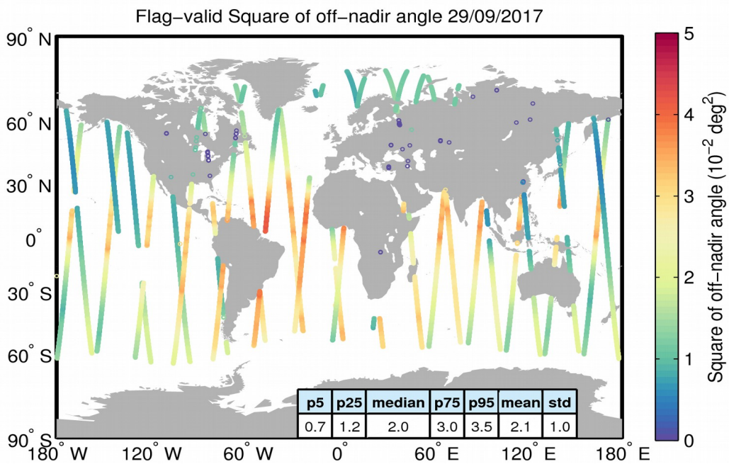
Figure 37. Geographical distribution of flag-valid mispointing data over oceans and lakes for 29/09/2017. The statistical values shown in the table refer to the mispointing in 10^{-2} deg 2 and are calculated over all measurements shown in the figure.
