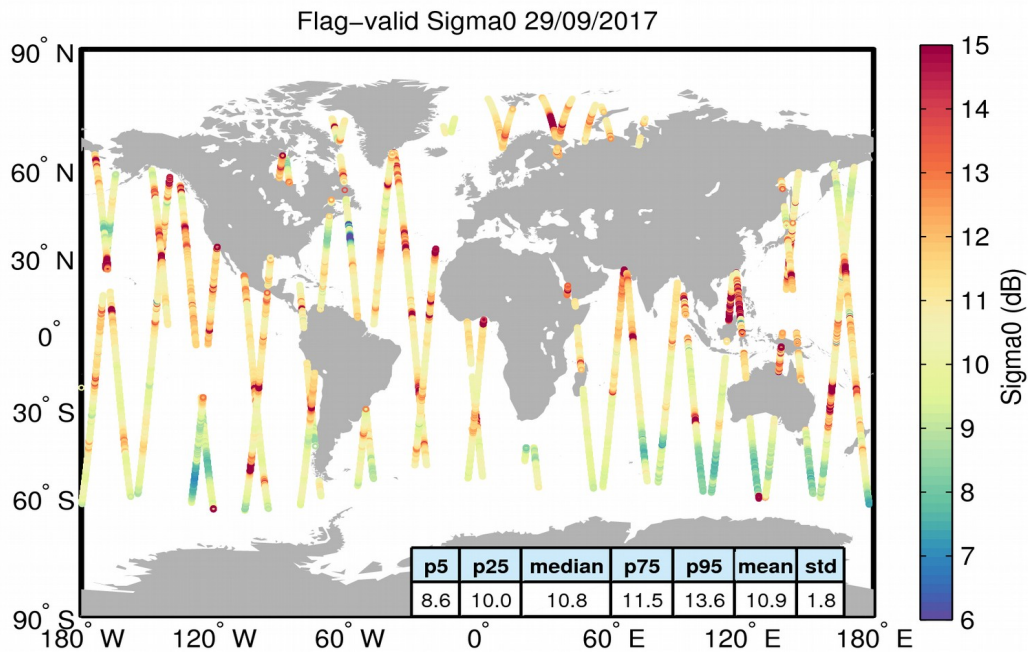
Figure 23. Geographical distribution of flag-valid sigma0 data over oceans and lakes for 29/09/2017. The statistical values shown in the table refer to the sigma0 in dB and are calculated over all measurements shown in the figure.
