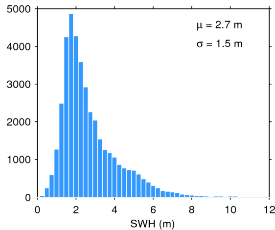
Figure 20. Histogram of science-valid SWH over oceans and lakes for 29/09/2017. The mean ( \mu ) and standard deviation ( \sigma ) are also shown. Note that values larger than 12 m are excluded from the histogram for the sake of readability but not from the computation of \mu and \sigma .
