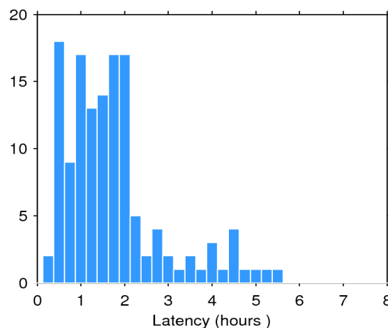
Figure 2. Histogram of the data latency for 29/09/2017. The y-axis denotes the number of files that are made available with a delay of x-hours with respect to the mean time of the records stored in the file.
