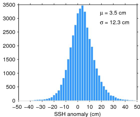
Figure 11. Histogram of science-valid SSH anomaly over oceans and lakes for 29/09/2017. The mean ( \mu ) and standard deviation ( \sigma ) are also shown. Note that values outside [-50 50] cm are excluded from the histogram for the sake of readability but not from the computation of \mu and \sigma .
