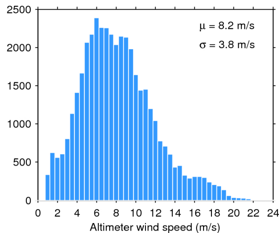
Figure 35. Histogram of science-valid wind over oceans and lakes for 29/09/2017. The mean ( \mu ) and standard deviation ( \sigma ) are also shown. Note that values larger than 24 m/s are excluded from the histogram for the sake of readability but not from the computation of \mu and \sigma .
