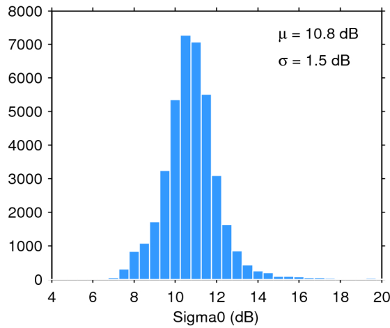
Figure 28. Histogram of science-valid sigma0 over oceans and lakes for 29/09/2017. The mean ( \mu ) and standard deviation ( \sigma ) are also shown. Note that values outside [4 20] dB are excluded from the histogram for the sake of readability but not from the computation of \mu and \sigma .
