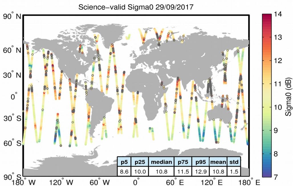
Figure 27. Geographical distribution of science-valid sigma0 data over oceans and lakes for 29/09/2017. The statistical values shown in the table refer to the sigma0 in dB and are calculated over all measurements shown in the figure. Gray circles denote records that have been rejected based on the editing criteria described in Table 4.
