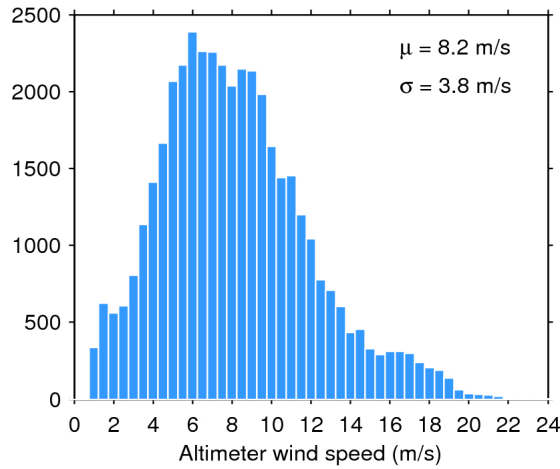
Figure 33. Histogram of flag-valid wind over oceans and lakes for 29/09/2017. The mean ( \mu ) and standard deviation ( \sigma ) are also shown. Note that values larger than 24 m/s are excluded from the histogram for the sake of readability but not from the computation of \mu and \sigma .
