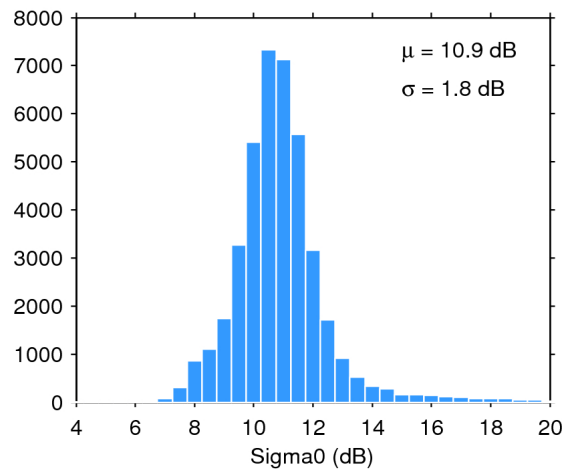
Figure 25. Histogram of flag-valid sigma0 over oceans and lakes for 29/09/2017. The mean ( \mu ) and standard deviation ( \sigma ) are also shown. Note that values outside [4 20] dB are excluded from the histogram for the sake of readability but not from the computation of \mu and \sigma .
