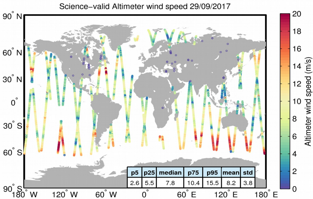
Figure 34. Geographical distribution of science-valid wind data over oceans and lakes for 29/09/2017. The statistical values shown in the table refer to the wind in m/s and are calculated over all measurements shown in the figure. Gray circles denote records that have been rejected based on the editing criteria described in Table 5.
