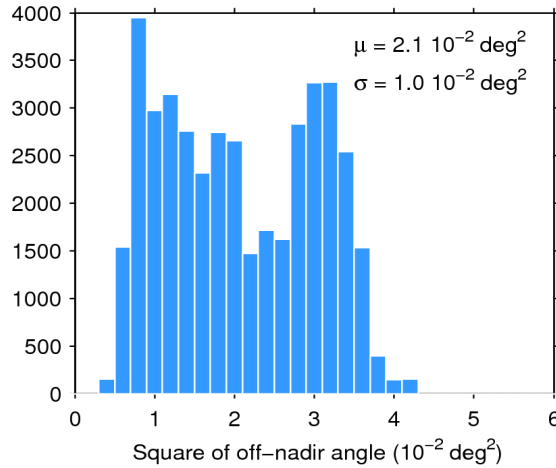
Figure 39. Histogram of flag-valid mispointing over oceans and lakes for 29/09/2017. The mean ( \mu ) and standard deviation ( \sigma ) are also shown. Note that values larger than 6 \cdot 10^{-2} \text{ deg}^2 are excluded from the histogram for the sake of readability but not from the computation of \mu and \sigma .
