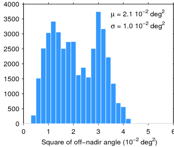
Figure 39. Histogram of flag-valid mispointing over oceans and lakes for 28/09/2017. The mean ( \mu ) and standard deviation ( \sigma ) are also shown. Note that values larger than 6 \cdot 10^{-2} \text{ deg}^2 are excluded from the histogram for the sake of readability but not from the computation of \mu and \sigma .
