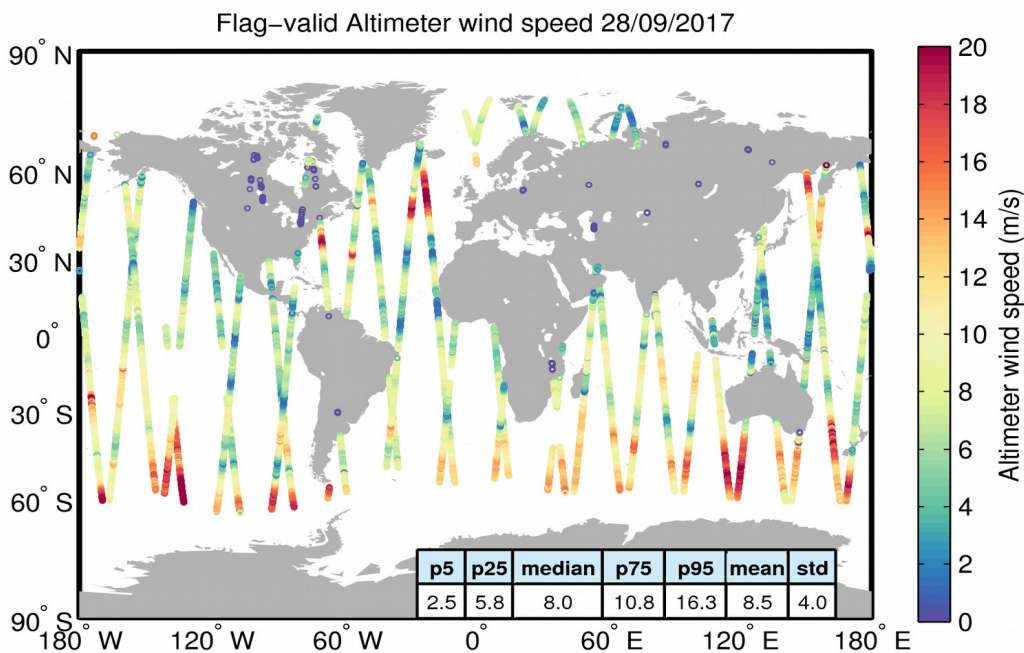
Figure 31. Geographical distribution of flag-valid wind data over oceans and lakes for 28/09/2017. The statistical values shown in the table refer to the wind in m/s and are calculated over all measurements shown in the figure.
