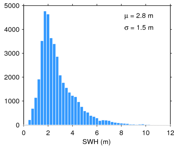
Figure 17. Histogram of flag-valid SWH over oceans and lakes for 28/09/2017. The mean ( \mu ) and standard deviation ( \sigma ) are also shown. Note that values larger than 12 m are excluded from the histogram for the sake of readability but not from the computation of \mu and \sigma .
