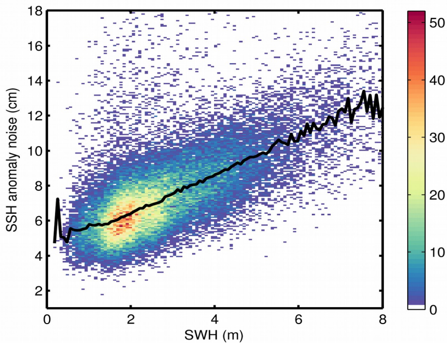
Figure 9. 2D histogram showing flag-valid SSH anomaly noise as a function of SWH for 28/09/2017. The black line denotes the median SSH anomaly noise as a function of SWH.
