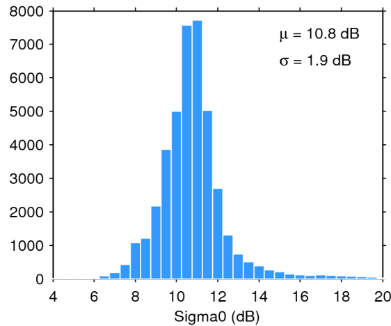
Figure 25. Histogram of flag-valid sigma0 over oceans and lakes for 28/09/2017. The mean ( \mu ) and standard deviation ( \sigma ) are also shown. Note that values outside [4 20] dB are excluded from the histogram for the sake of readability but not from the computation of \mu and \sigma .
