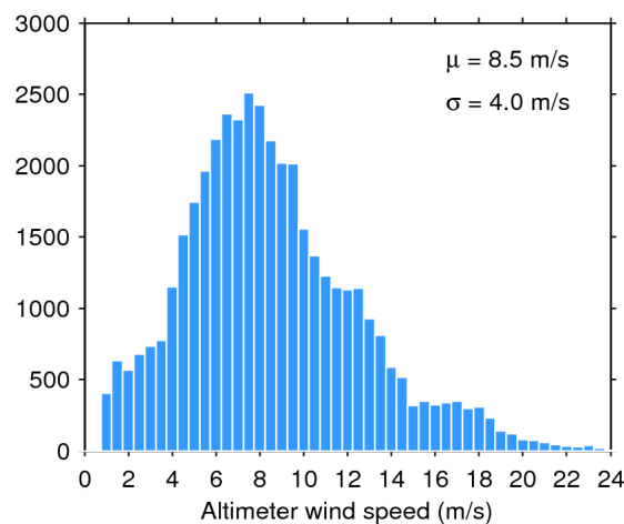
Figure 35. Histogram of science-valid wind over oceans and lakes for 28/09/2017. The mean ( \mu ) and standard deviation ( \sigma ) are also shown. Note that values larger than 24 m/s are excluded from the histogram for the sake of readability but not from the computation of \mu and \sigma .
