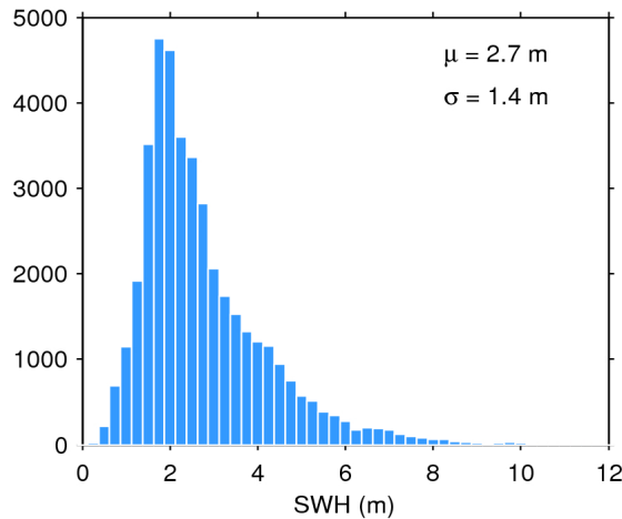
Figure 20. Histogram of science-valid SWH over oceans and lakes for 28/09/2017. The mean ( \mu ) and standard deviation ( \sigma ) are also shown. Note that values larger than 12 m are excluded from the histogram for the sake of readability but not from the computation of \mu and \sigma .
