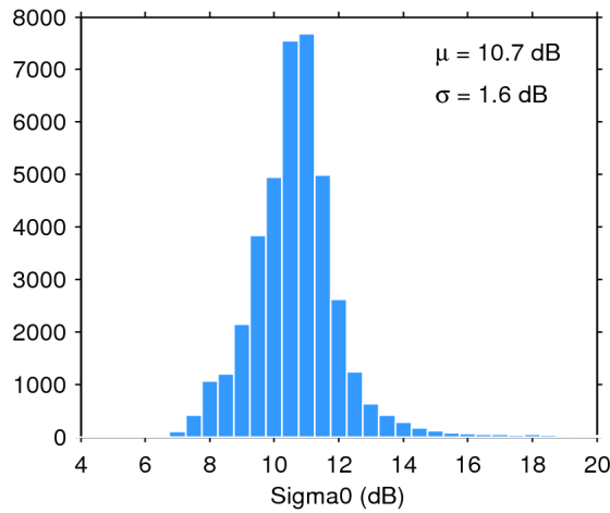
Figure 28. Histogram of science-valid sigma0 over oceans and lakes for 28/09/2017. The mean ( \mu ) and standard deviation ( \sigma ) are also shown. Note that values outside [4 20] dB are excluded from the histogram for the sake of readability but not from the computation of \mu and \sigma .
