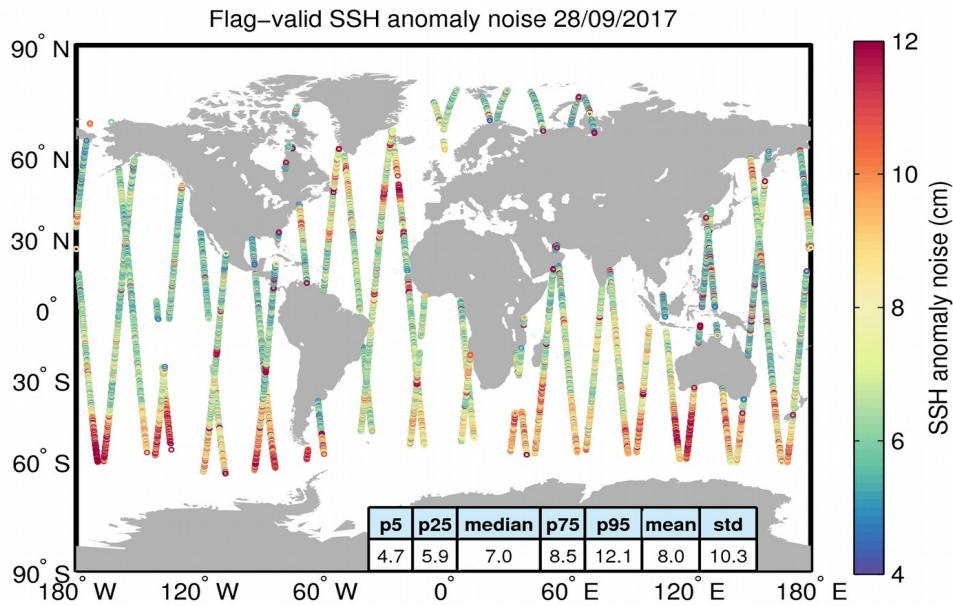
Figure 8. Geographical distribution of flag-valid 20-Hz SSH anomaly measurement noise over oceans and lakes for 28/09/2017. The statistical values shown in the table refer to the SSH anomaly noise and are calculated over all measurements shown in the figure.
