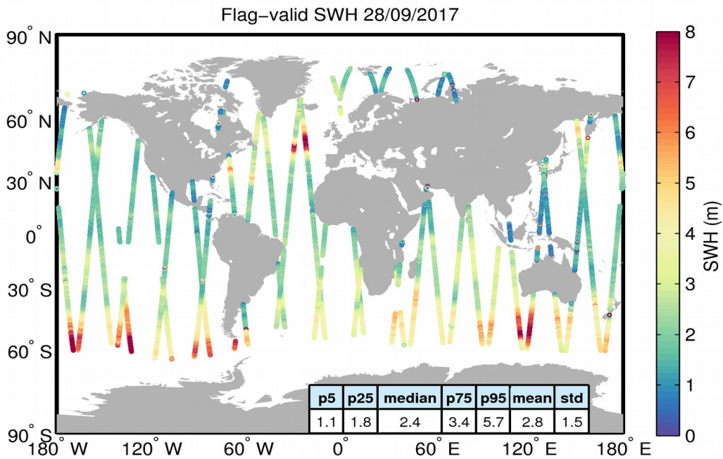
Figure 15. Geographical distribution of flag-valid SWH data over oceans and lakes for 28/09/2017. The statistical values shown in the table refer to the SWH in m and are calculated over all measurements shown in the figure.
