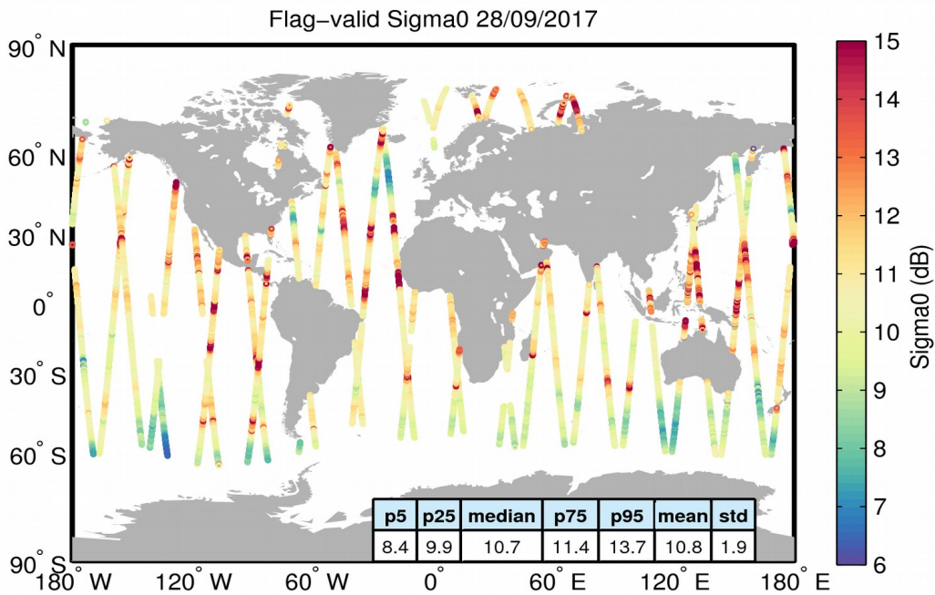
Figure 23. Geographical distribution of flag-valid sigma0 data over oceans and lakes for 28/09/2017. The statistical values shown in the table refer to the sigma0 in dB and are calculated over all measurements shown in the figure.
