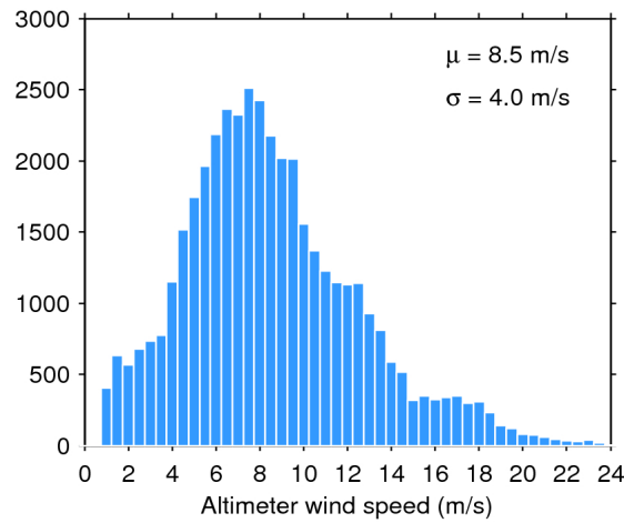
Figure 33. Histogram of flag-valid wind over oceans and lakes for 28/09/2017. The mean ( \mu ) and standard deviation ( \sigma ) are also shown. Note that values larger than 24 m/s are excluded from the histogram for the sake of readability but not from the computation of \mu and \sigma .
