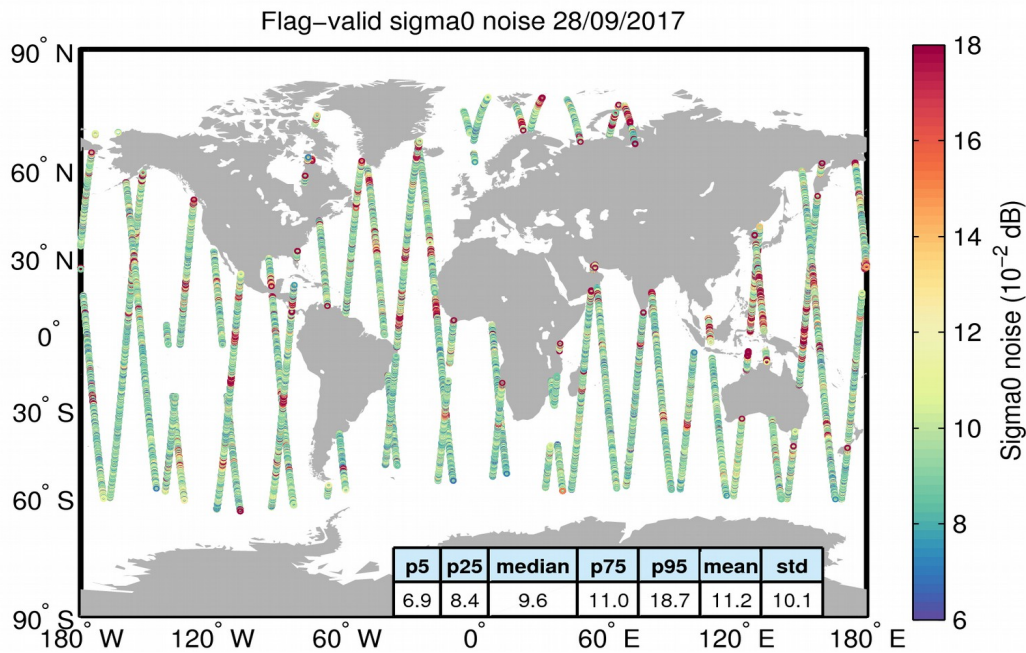
Figure 26. Geographical distribution of flag-valid 20-Hz sigma0 measurement noise over oceans and lakes for 28/09/2017. The statistical values shown in the table refer to the sigma0 noise and are calculated over all measurements shown in the figure.
