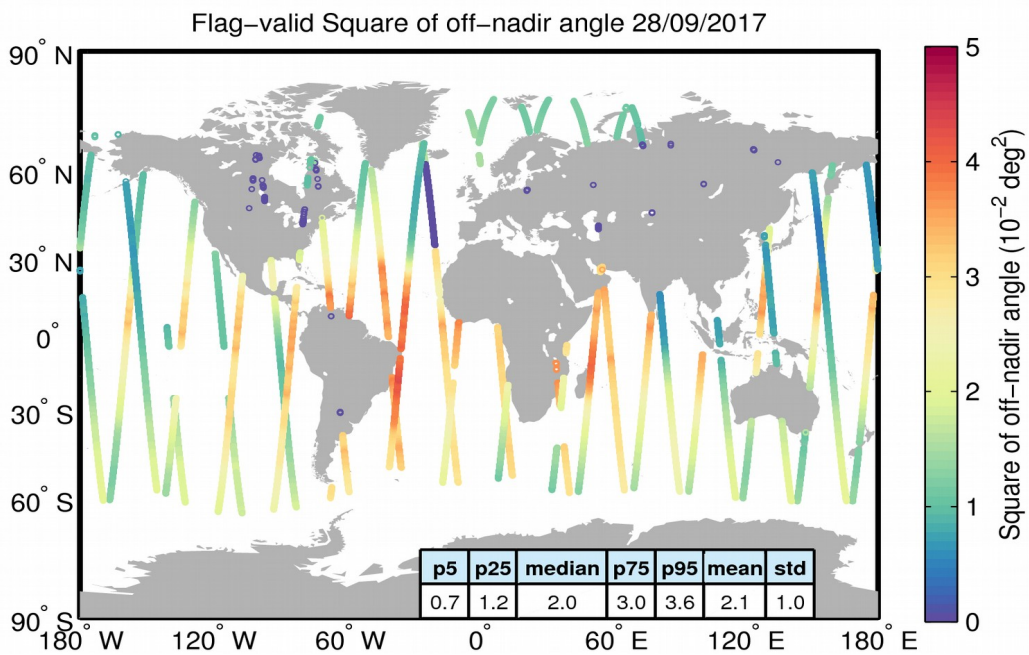
Figure 37. Geographical distribution of flag-valid mispointing data over oceans and lakes for 28/09/2017. The statistical values shown in the table refer to the mispointing in 10^{-2} deg 2 and are calculated over all measurements shown in the figure.
