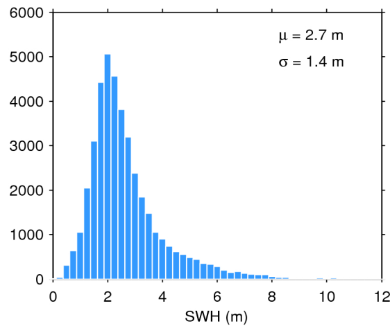
Figure 17. Histogram of flag-valid SWH over oceans and lakes for 27/09/2017. The mean ( \mu ) and standard deviation ( \sigma ) are also shown. Note that values larger than 12 m are excluded from the histogram for the sake of readability but not from the computation of \mu and \sigma .
