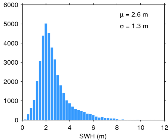
Figure 20. Histogram of science-valid SWH over oceans and lakes for 27/09/2017. The mean ( \mu ) and standard deviation ( \sigma ) are also shown. Note that values larger than 12 m are excluded from the histogram for the sake of readability but not from the computation of \mu and \sigma .
