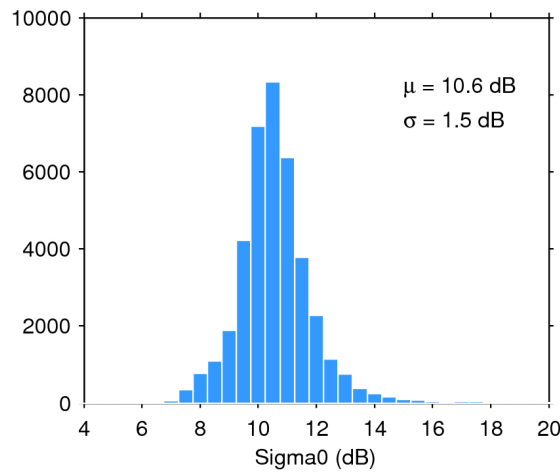
Figure 28. Histogram of science-valid sigma0 over oceans and lakes for 27/09/2017. The mean ( \mu ) and standard deviation ( \sigma ) are also shown. Note that values outside [4 20] dB are excluded from the histogram for the sake of readability but not from the computation of \mu and \sigma .
