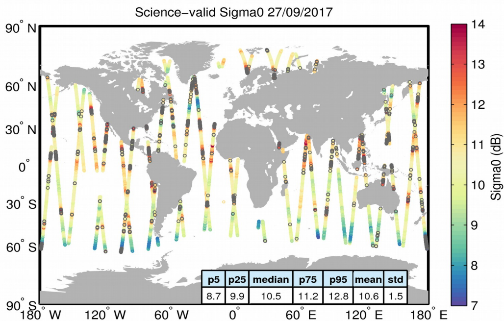
Figure 27. Geographical distribution of science-valid sigma0 data over oceans and lakes for 27/09/2017. The statistical values shown in the table refer to the sigma0 in dB and are calculated over all measurements shown in the figure. Gray circles denote records that have been rejected based on the editing criteria described in Table 4.
