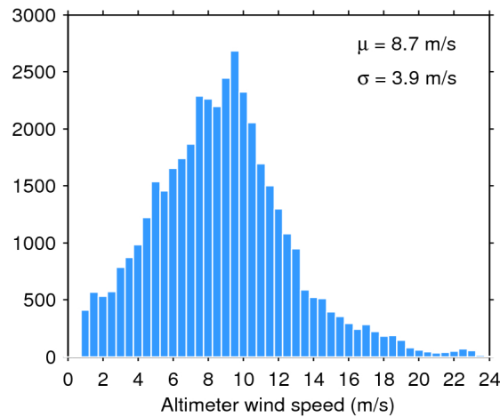
Figure 33. Histogram of flag-valid wind over oceans and lakes for 27/09/2017. The mean ( \mu ) and standard deviation ( \sigma ) are also shown. Note that values larger than 24 m/s are excluded from the histogram for the sake of readability but not from the computation of \mu and \sigma .
