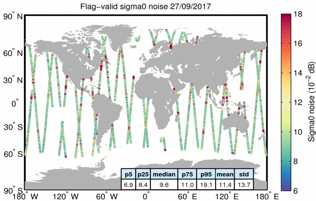
Figure 26. Geographical distribution of flag-valid 20-Hz sigma0 measurement noise over oceans and lakes for 27/09/2017. The statistical values shown in the table refer to the sigma0 noise and are calculated over all measurements shown in the figure.
