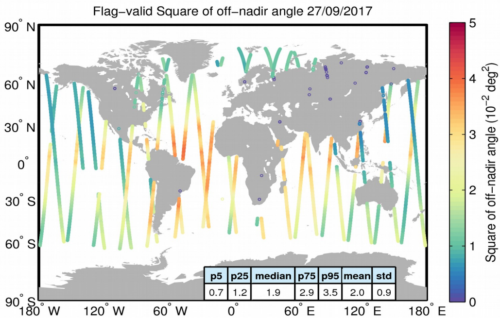
Figure 37. Geographical distribution of flag-valid mispointing data over oceans and lakes for 27/09/2017. The statistical values shown in the table refer to the mispointing in 10^{-2} deg 2 and are calculated over all measurements shown in the figure.
