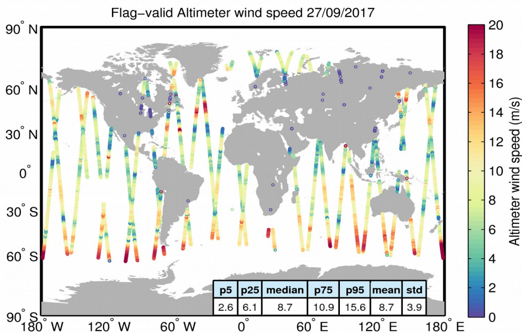
Figure 31. Geographical distribution of flag-valid wind data over oceans and lakes for 27/09/2017. The statistical values shown in the table refer to the wind in m/s and are calculated over all measurements shown in the figure.
