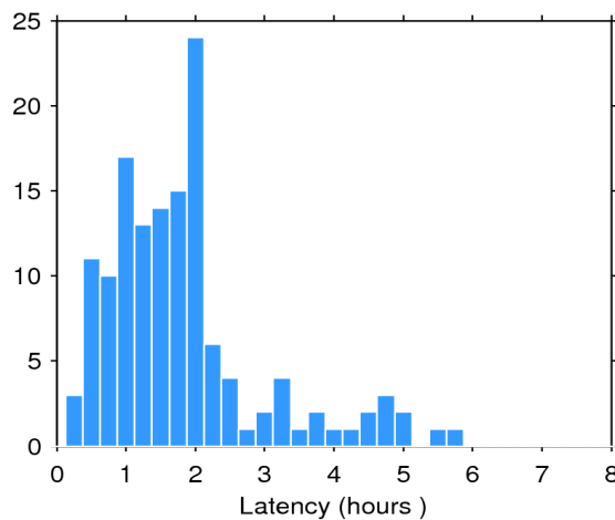
Figure 2. Histogram of the data latency for 27/09/2017. The y-axis denotes the number of files that are made available with a delay of x-hours with respect to the mean time of the records stored in the file.
