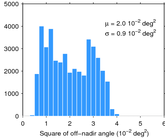
Figure 39. Histogram of flag-valid mispointing over oceans and lakes for 27/09/2017. The mean ( \mu ) and standard deviation ( \sigma ) are also shown. Note that values larger than 6 \cdot 10^{-2} \text{ deg}^2 are excluded from the histogram for the sake of readability but not from the computation of \mu and \sigma .
