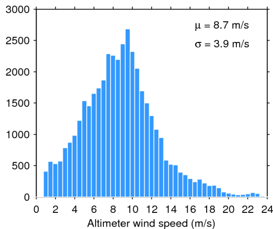
Figure 35. Histogram of science-valid wind over oceans and lakes for 27/09/2017. The mean ( \mu ) and standard deviation ( \sigma ) are also shown. Note that values larger than 24 m/s are excluded from the histogram for the sake of readability but not from the computation of \mu and \sigma .
