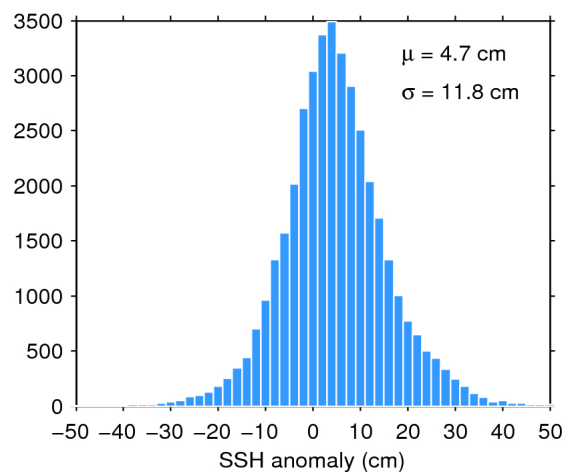
Figure 11. Histogram of science-valid SSH anomaly over oceans and lakes for 27/09/2017. The mean ( \mu ) and standard deviation ( \sigma ) are also shown. Note that values outside [-50 50] cm are excluded from the histogram for the sake of readability but not from the computation of \mu and \sigma .
