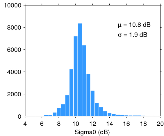
Figure 25. Histogram of flag-valid sigma0 over oceans and lakes for 27/09/2017. The mean ( \mu ) and standard deviation ( \sigma ) are also shown. Note that values outside [4 20] dB are excluded from the histogram for the sake of readability but not from the computation of \mu and \sigma .
