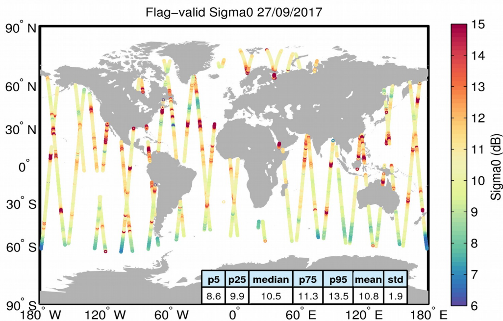
Figure 23. Geographical distribution of flag-valid sigma0 data over oceans and lakes for 27/09/2017. The statistical values shown in the table refer to the sigma0 in dB and are calculated over all measurements shown in the figure.
