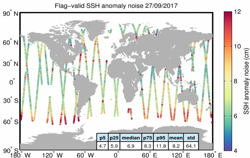
Figure 8. Geographical distribution of flag-valid 20-Hz SSH anomaly measurement noise over oceans and lakes for 27/09/2017. The statistical values shown in the table refer to the SSH anomaly noise and are calculated over all measurements shown in the figure.
