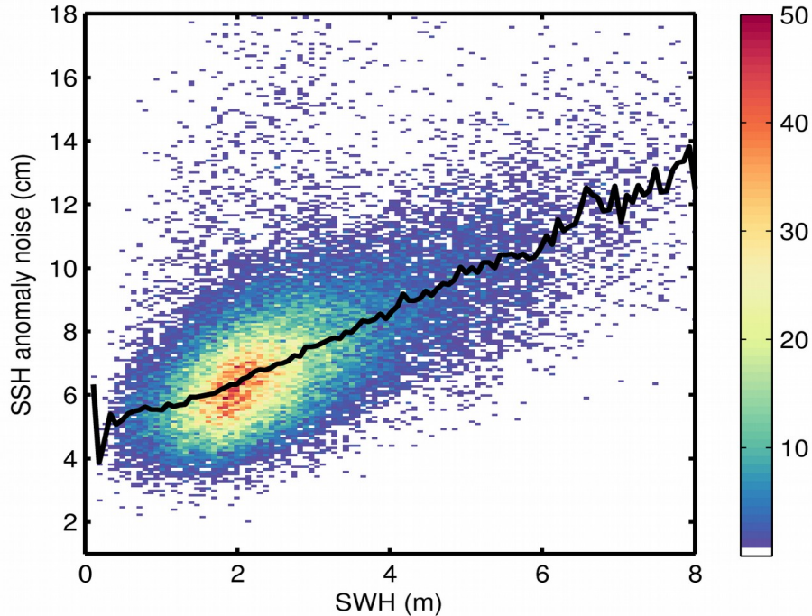
Figure 9. 2D histogram showing flag-valid SSH anomaly noise as a function of SWH for 27/09/2017. The black line denotes the median SSH anomaly noise as a function of SWH.
