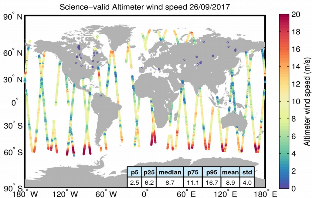
Figure 34. Geographical distribution of science-valid wind data over oceans and lakes for 26/09/2017. The statistical values shown in the table refer to the wind in m/s and are calculated over all measurements shown in the figure. Gray circles denote records that have been rejected based on the editing criteria described in Table 5.
