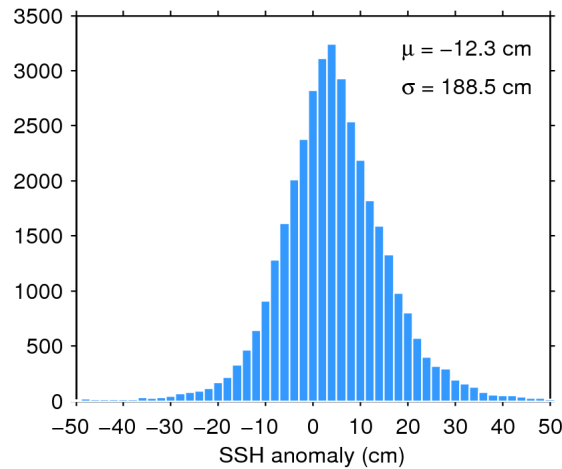
Figure 7. Histogram of flag-valid SSH anomaly over oceans and lakes for 26/09/2017. The mean ( \mu ) and standard deviation ( \sigma ) are also shown. Note that values outside [-50 50] cm are excluded from the histogram for the sake of readability but not from the computation of \mu and \sigma .
