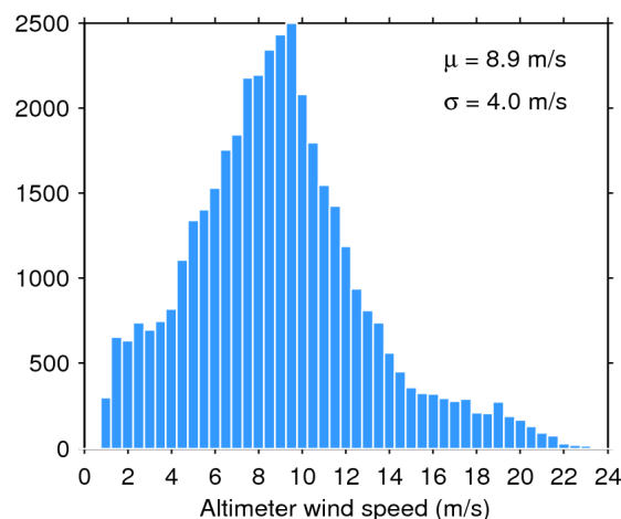
Figure 35. Histogram of science-valid wind over oceans and lakes for 26/09/2017. The mean ( \mu ) and standard deviation ( \sigma ) are also shown. Note that values larger than 24 m/s are excluded from the histogram for the sake of readability but not from the computation of \mu and \sigma .
