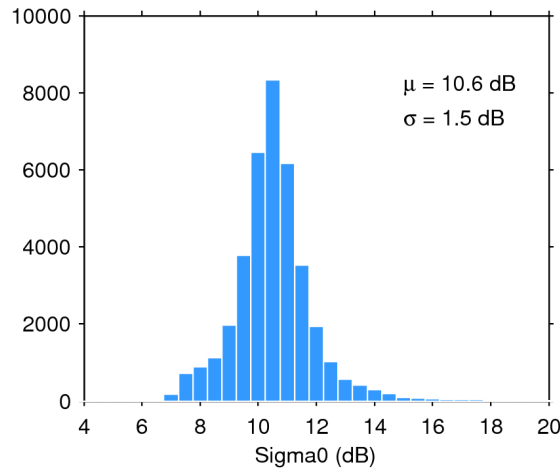
Figure 28. Histogram of science-valid sigma0 over oceans and lakes for 26/09/2017. The mean ( \mu ) and standard deviation ( \sigma ) are also shown. Note that values outside [4 20] dB are excluded from the histogram for the sake of readability but not from the computation of \mu and \sigma .
