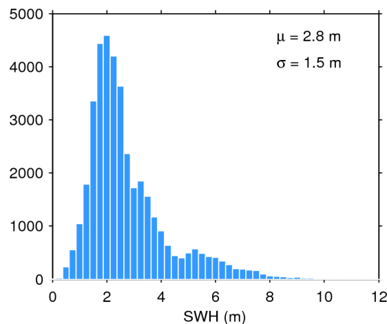
Figure 20. Histogram of science-valid SWH over oceans and lakes for 26/09/2017. The mean ( \mu ) and standard deviation ( \sigma ) are also shown. Note that values larger than 12 m are excluded from the histogram for the sake of readability but not from the computation of \mu and \sigma .
