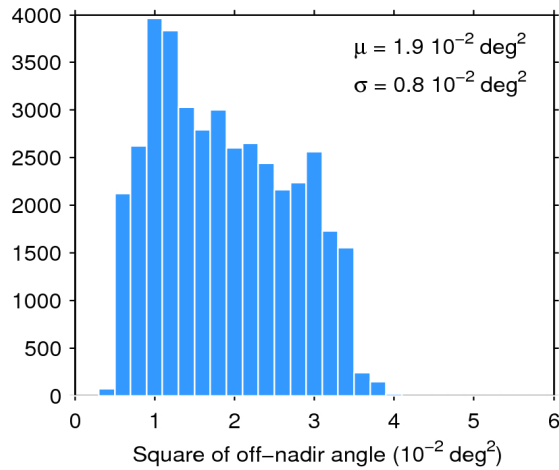
Figure 39. Histogram of flag-valid mispointing over oceans and lakes for 26/09/2017. The mean ( \mu ) and standard deviation ( \sigma ) are also shown. Note that values larger than 6 \cdot 10^{-2} \text{ deg}^2 are excluded from the histogram for the sake of readability but not from the computation of \mu and \sigma .
