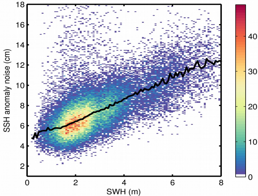
Figure 9. 2D histogram showing flag-valid SSH anomaly noise as a function of SWH for 26/09/2017. The black line denotes the median SSH anomaly noise as a function of SWH.
