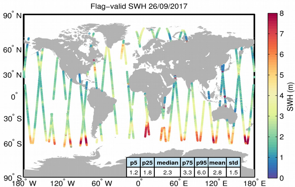
Figure 15. Geographical distribution of flag-valid SWH data over oceans and lakes for 26/09/2017. The statistical values shown in the table refer to the SWH in m and are calculated over all measurements shown in the figure.
