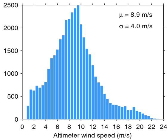
Figure 33. Histogram of flag-valid wind over oceans and lakes for 26/09/2017. The mean ( \mu ) and standard deviation ( \sigma ) are also shown. Note that values larger than 24 m/s are excluded from the histogram for the sake of readability but not from the computation of \mu and \sigma .
