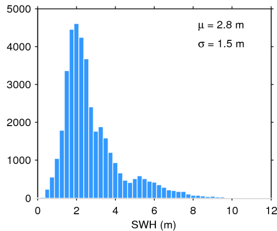
Figure 17. Histogram of flag-valid SWH over oceans and lakes for 26/09/2017. The mean ( \mu ) and standard deviation ( \sigma ) are also shown. Note that values larger than 12 m are excluded from the histogram for the sake of readability but not from the computation of \mu and \sigma .
