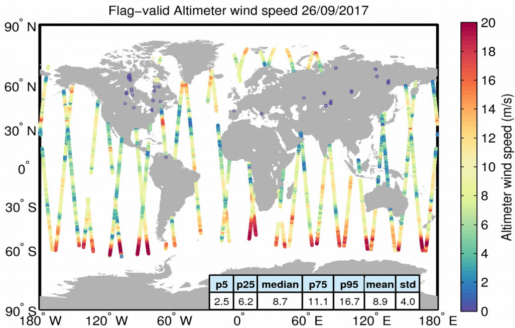
Figure 31. Geographical distribution of flag-valid wind data over oceans and lakes for 26/09/2017. The statistical values shown in the table refer to the wind in m/s and are calculated over all measurements shown in the figure.
