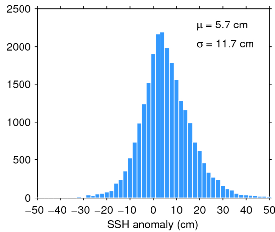
Figure 11. Histogram of science-valid SSH anomaly over oceans and lakes for 26/09/2017. The mean ( \mu ) and standard deviation ( \sigma ) are also shown. Note that values outside [-50 50] cm are excluded from the histogram for the sake of readability but not from the computation of \mu and \sigma .
