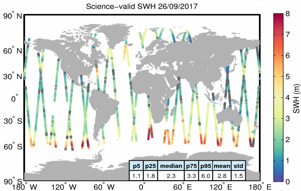
Figure 19. Geographical distribution of science-valid SWH data over oceans and lakes for 26/09/2017. The statistical values shown in the table refer to the SWH in m and are calculated over all measurements shown in the figure. Gray circles denote records that have been rejected based on the editing criteria described in Table 3.
