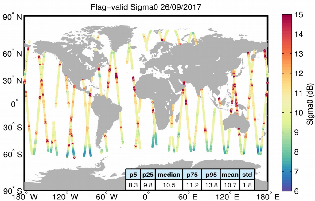
Figure 23. Geographical distribution of flag-valid sigma0 data over oceans and lakes for 26/09/2017. The statistical values shown in the table refer to the sigma0 in dB and are calculated over all measurements shown in the figure.
