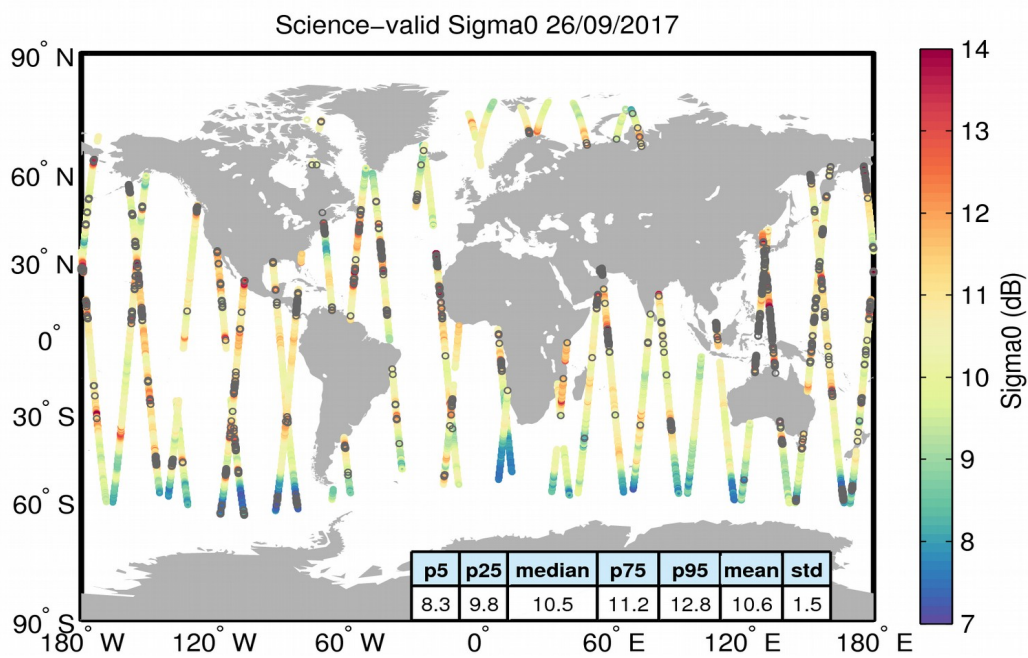
Figure 27. Geographical distribution of science-valid sigma0 data over oceans and lakes for 26/09/2017. The statistical values shown in the table refer to the sigma0 in dB and are calculated over all measurements shown in the figure. Gray circles denote records that have been rejected based on the editing criteria described in Table 4.
