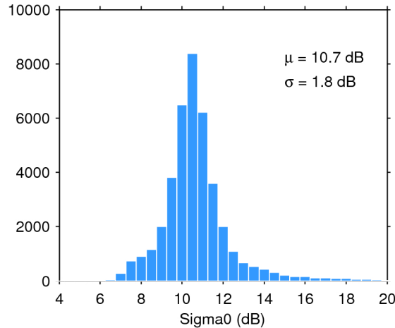
Figure 25. Histogram of flag-valid sigma0 over oceans and lakes for 26/09/2017. The mean ( \mu ) and standard deviation ( \sigma ) are also shown. Note that values outside [4 20] dB are excluded from the histogram for the sake of readability but not from the computation of \mu and \sigma .
