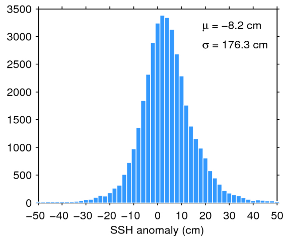
Figure 7. Histogram of flag-valid SSH anomaly over oceans and lakes for 24/09/2017. The mean ( \mu ) and standard deviation ( \sigma ) are also shown. Note that values outside [-50\ 50] cm are excluded from the histogram for the sake of readability but not from the computation of \mu and \sigma .
