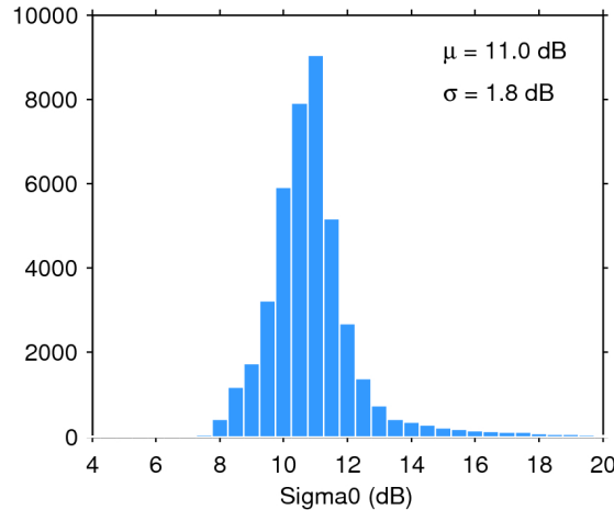
Figure 25. Histogram of flag-valid sigma0 over oceans and lakes for 24/09/2017. The mean ( \mu ) and standard deviation ( \sigma ) are also shown. Note that values outside [4 20] dB are excluded from the histogram for the sake of readability but not from the computation of \mu and \sigma .
