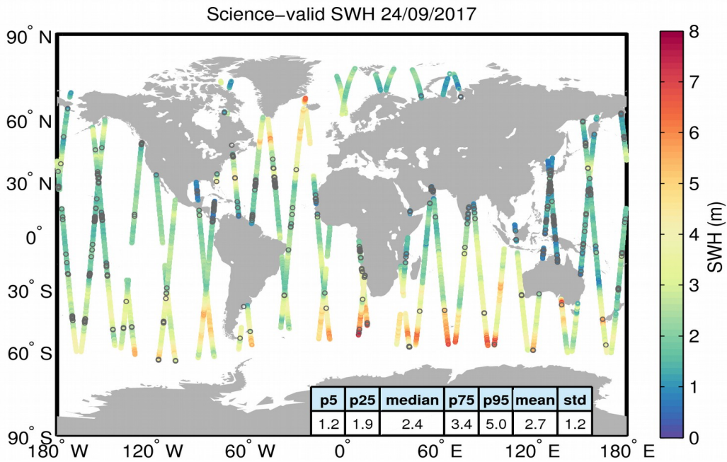
Figure 19. Geographical distribution of science-valid SWH data over oceans and lakes for 24/09/2017. The statistical values shown in the table refer to the SWH in m and are calculated over all measurements shown in the figure. Gray circles denote records that have been rejected based on the editing criteria described in Table 3.
