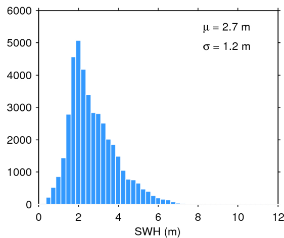
Figure 17. Histogram of flag-valid SWH over oceans and lakes for 24/09/2017. The mean ( \mu ) and standard deviation ( \sigma ) are also shown. Note that values larger than 12 m are excluded from the histogram for the sake of readability but not from the computation of \mu and \sigma .
