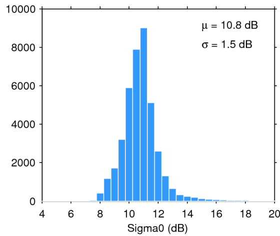
Figure 28. Histogram of science-valid sigma0 over oceans and lakes for 24/09/2017. The mean ( \mu ) and standard deviation ( \sigma ) are also shown. Note that values outside [4 20] dB are excluded from the histogram for the sake of readability but not from the computation of \mu and \sigma .
