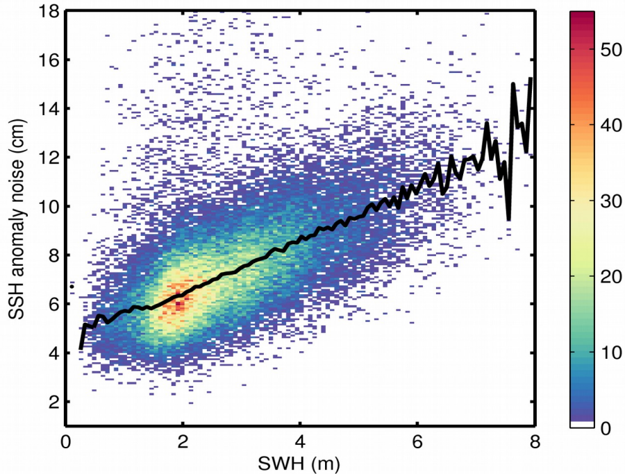
Figure 9. 2D histogram showing flag-valid SSH anomaly noise as a function of SWH for 24/09/2017. The black line denotes the median SSH anomaly noise as a function of SWH.
