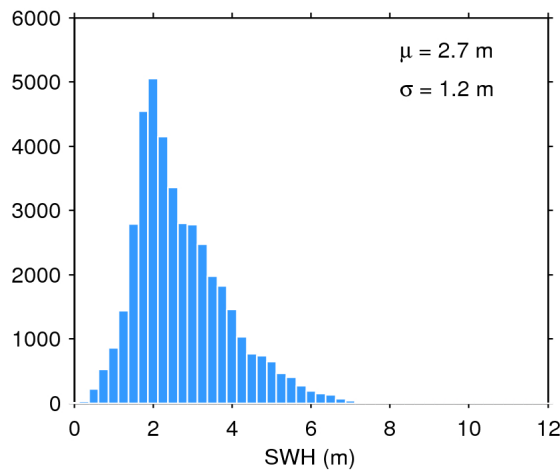
Figure 20. Histogram of science-valid SWH over oceans and lakes for 24/09/2017. The mean ( \mu ) and standard deviation ( \sigma ) are also shown. Note that values larger than 12 m are excluded from the histogram for the sake of readability but not from the computation of \mu and \sigma .
