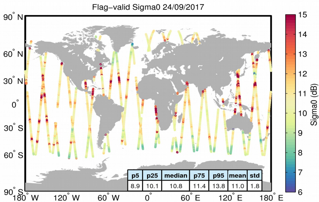
Figure 23. Geographical distribution of flag-valid sigma0 data over oceans and lakes for 24/09/2017. The statistical values shown in the table refer to the sigma0 in dB and are calculated over all measurements shown in the figure.
