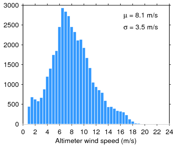
Figure 33. Histogram of flag-valid wind over oceans and lakes for 24/09/2017. The mean ( \mu ) and standard deviation ( \sigma ) are also shown. Note that values larger than 24 m/s are excluded from the histogram for the sake of readability but not from the computation of \mu and \sigma .
