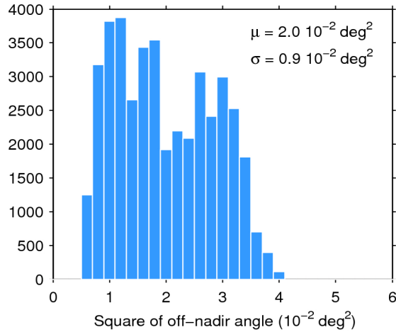
Figure 39. Histogram of flag-valid mispointing over oceans and lakes for 24/09/2017. The mean ( \mu ) and standard deviation ( \sigma ) are also shown. Note that values larger than 6 \cdot 10^{-2} \text{ deg}^2 are excluded from the histogram for the sake of readability but not from the computation of \mu and \sigma .
