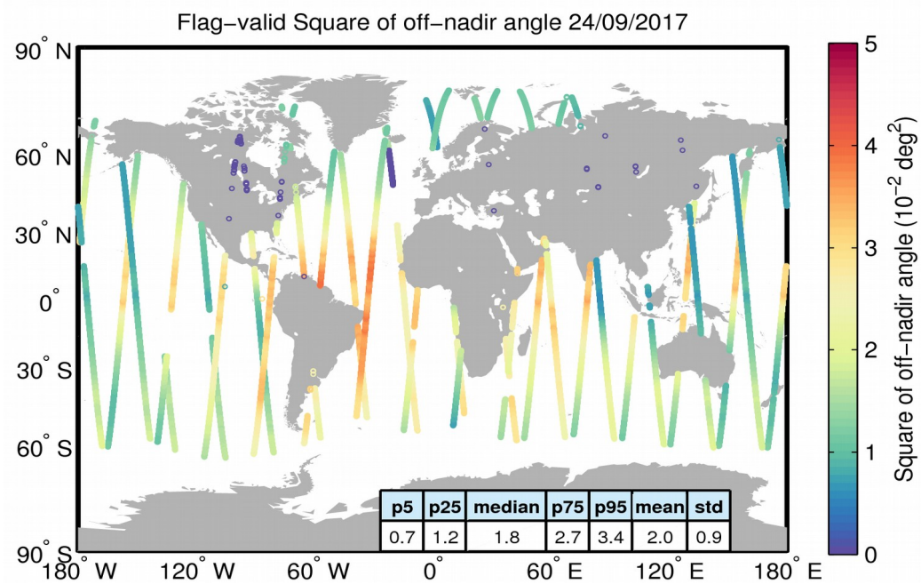
Figure 37. Geographical distribution of flag-valid mispointing data over oceans and lakes for 24/09/2017. The statistical values shown in the table refer to the mispointing in 10^{-2} \text{ deg}^2 and are calculated over all measurements shown in the figure.
