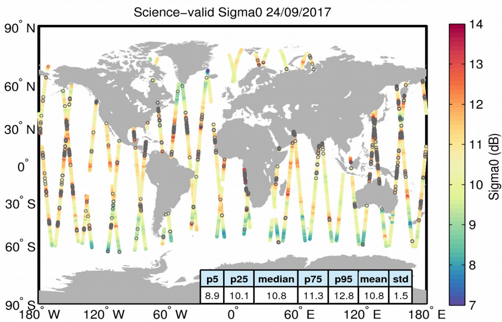
Figure 27. Geographical distribution of science-valid sigma0 data over oceans and lakes for 24/09/2017. The statistical values shown in the table refer to the sigma0 in dB and are calculated over all measurements shown in the figure. Gray circles denote records that have been rejected based on the editing criteria described in Table 4.
