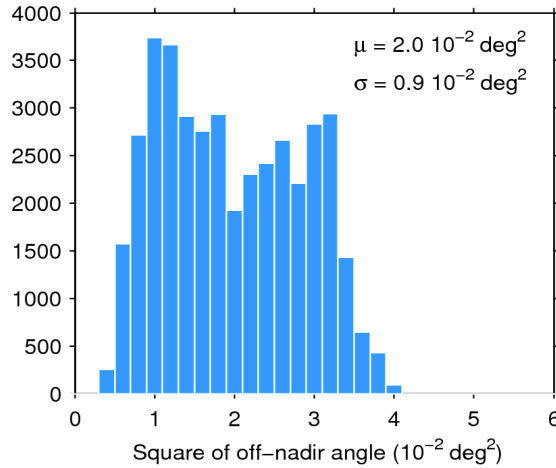
Figure 39. Histogram of flag-valid mispointing over oceans and lakes for 23/09/2017. The mean ( \mu ) and standard deviation ( \sigma ) are also shown. Note that values larger than 6 \cdot 10^{-2} \text{ deg}^2 are excluded from the histogram for the sake of readability but not from the computation of \mu and \sigma .
