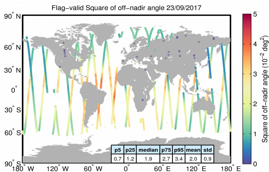
Figure 37. Geographical distribution of flag-valid mispointing data over oceans and lakes for 23/09/2017. The statistical values shown in the table refer to the mispointing in 10^{-2} deg 2 and are calculated over all measurements shown in the figure.
