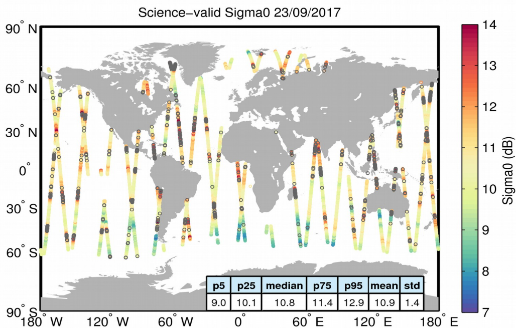
Figure 27. Geographical distribution of science-valid sigma0 data over oceans and lakes for 23/09/2017. The statistical values shown in the table refer to the sigma0 in dB and are calculated over all measurements shown in the figure. Gray circles denote records that have been rejected based on the editing criteria described in Table 4.
