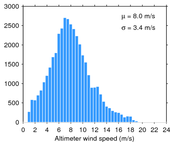
Figure 35. Histogram of science-valid wind over oceans and lakes for 23/09/2017. The mean ( \mu ) and standard deviation ( \sigma ) are also shown. Note that values larger than 24 m/s are excluded from the histogram for the sake of readability but not from the computation of \mu and \sigma .
