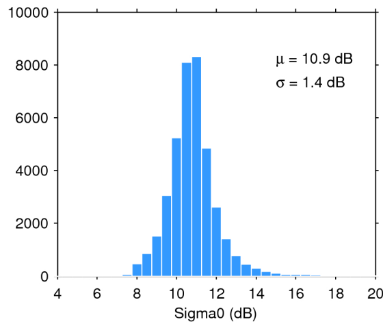
Figure 28. Histogram of science-valid sigma0 over oceans and lakes for 23/09/2017. The mean ( \mu ) and standard deviation ( \sigma ) are also shown. Note that values outside [4 20] dB are excluded from the histogram for the sake of readability but not from the computation of \mu and \sigma .
