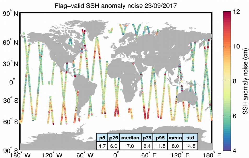
Figure 8. Geographical distribution of flag-valid 20-Hz SSH anomaly measurement noise over oceans and lakes for 23/09/2017. The statistical values shown in the table refer to the SSH anomaly noise and are calculated over all measurements shown in the figure.
