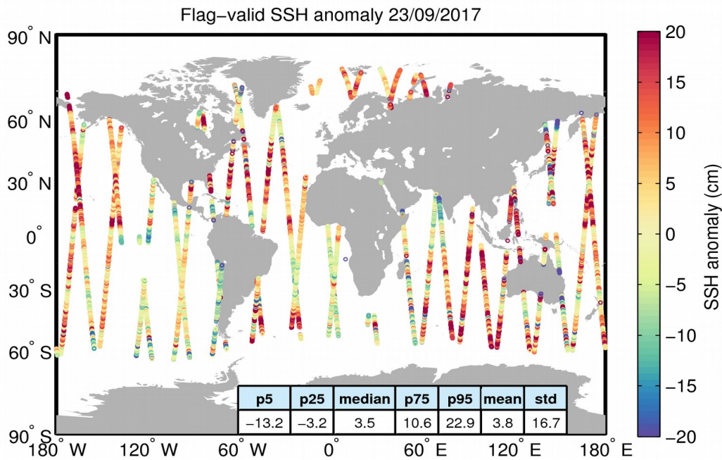
Figure 5. Geographical distribution of flag-valid 1-Hz SSH anomaly data over oceans and lakes for 23/09/2017. The statistical values shown in the table refer to the SSH anomaly in cm and are calculated over all measurements shown in the figure.
