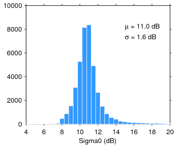
Figure 25. Histogram of flag-valid sigma0 over oceans and lakes for 23/09/2017. The mean ( \mu ) and standard deviation ( \sigma ) are also shown. Note that values outside [4 20] dB are excluded from the histogram for the sake of readability but not from the computation of \mu and \sigma .
