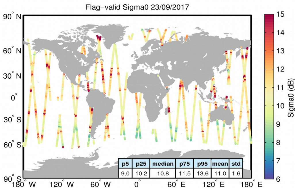
Figure 23. Geographical distribution of flag-valid sigma0 data over oceans and lakes for 23/09/2017. The statistical values shown in the table refer to the sigma0 in dB and are calculated over all measurements shown in the figure.
