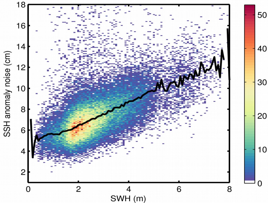
Figure 9. 2D histogram showing flag-valid SSH anomaly noise as a function of SWH for 23/09/2017. The black line denotes the median SSH anomaly noise as a function of SWH.
