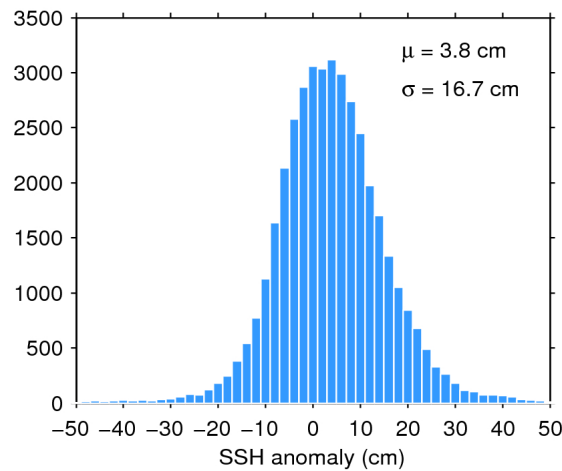
Figure 7. Histogram of flag-valid SSH anomaly over oceans and lakes for 23/09/2017. The mean ( \mu ) and standard deviation ( \sigma ) are also shown. Note that values outside [-50 50] cm are excluded from the histogram for the sake of readability but not from the computation of \mu and \sigma .
