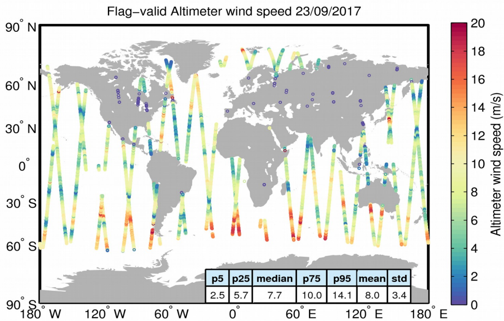
Figure 31. Geographical distribution of flag-valid wind data over oceans and lakes for 23/09/2017. The statistical values shown in the table refer to the wind in m/s and are calculated over all measurements shown in the figure.
