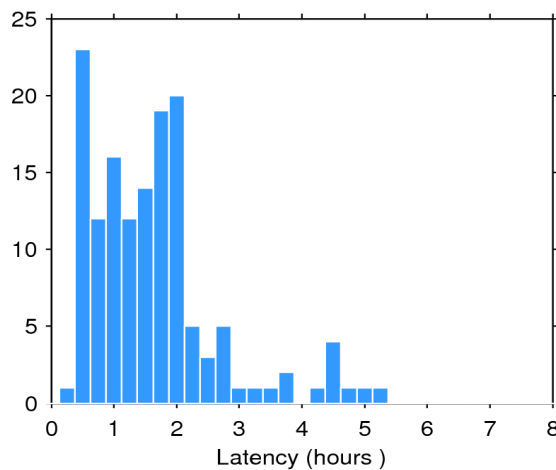
Figure 2. Histogram of the data latency for 23/09/2017. The y-axis denotes the number of files that are made available with a delay of x-hours with respect to the mean time of the records stored in the file.
