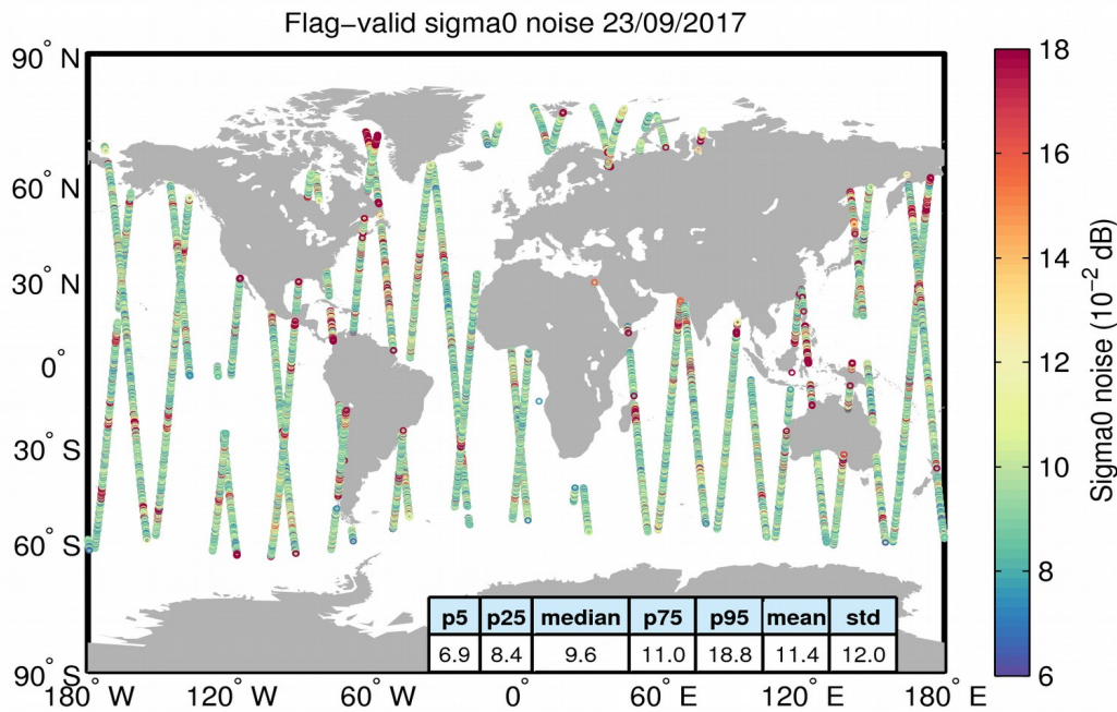
Figure 26. Geographical distribution of flag-valid 20-Hz sigma0 measurement noise over oceans and lakes for 23/09/2017. The statistical values shown in the table refer to the sigma0 noise and are calculated over all measurements shown in the figure.
