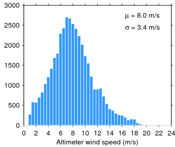
Figure 33. Histogram of flag-valid wind over oceans and lakes for 23/09/2017. The mean ( \mu ) and standard deviation ( \sigma ) are also shown. Note that values larger than 24 m/s are excluded from the histogram for the sake of readability but not from the computation of \mu and \sigma .
