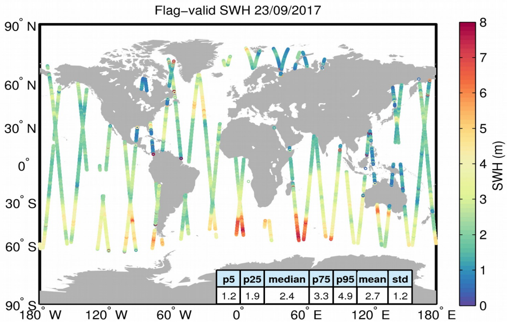
Figure 15. Geographical distribution of flag-valid SWH data over oceans and lakes for 23/09/2017. The statistical values shown in the table refer to the SWH in m and are calculated over all measurements shown in the figure.
