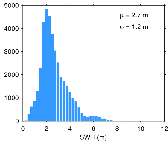
Figure 20. Histogram of science-valid SWH over oceans and lakes for 23/09/2017. The mean ( \mu ) and standard deviation ( \sigma ) are also shown. Note that values larger than 12 m are excluded from the histogram for the sake of readability but not from the computation of \mu and \sigma .
