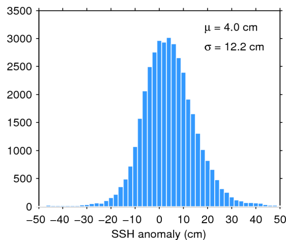
Figure 11. Histogram of science-valid SSH anomaly over oceans and lakes for 23/09/2017. The mean ( \mu ) and standard deviation ( \sigma ) are also shown. Note that values outside [-50 50] cm are excluded from the histogram for the sake of readability but not from the computation of \mu and \sigma .
