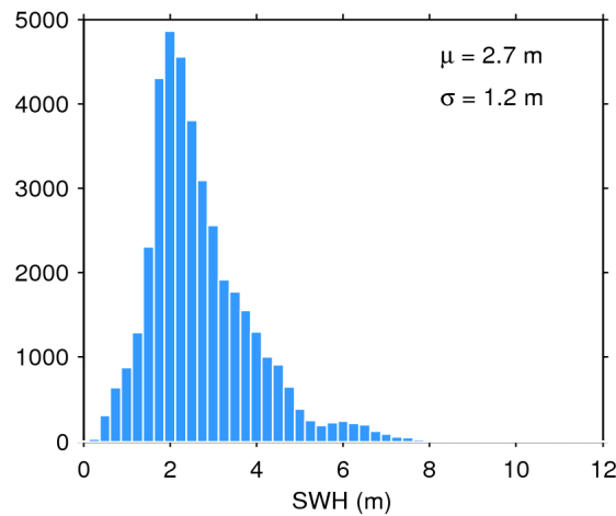
Figure 17. Histogram of flag-valid SWH over oceans and lakes for 23/09/2017. The mean ( \mu ) and standard deviation ( \sigma ) are also shown. Note that values larger than 12 m are excluded from the histogram for the sake of readability but not from the computation of \mu and \sigma .
