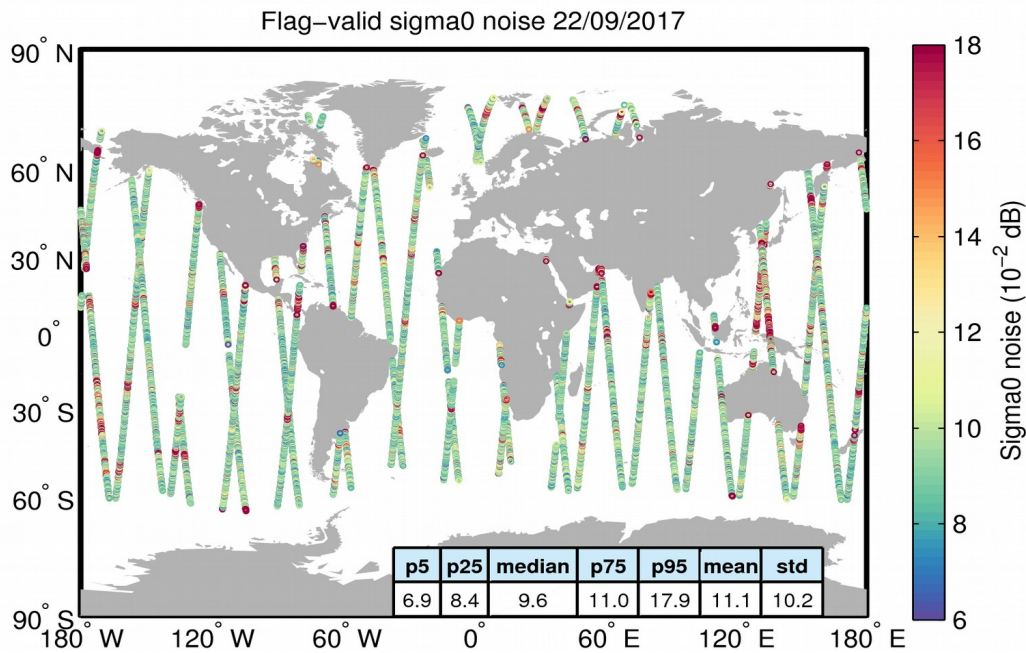
Figure 26. Geographical distribution of flag-valid 20-Hz sigma0 measurement noise over oceans and lakes for 22/09/2017. The statistical values shown in the table refer to the sigma0 noise and are calculated over all measurements shown in the figure.
