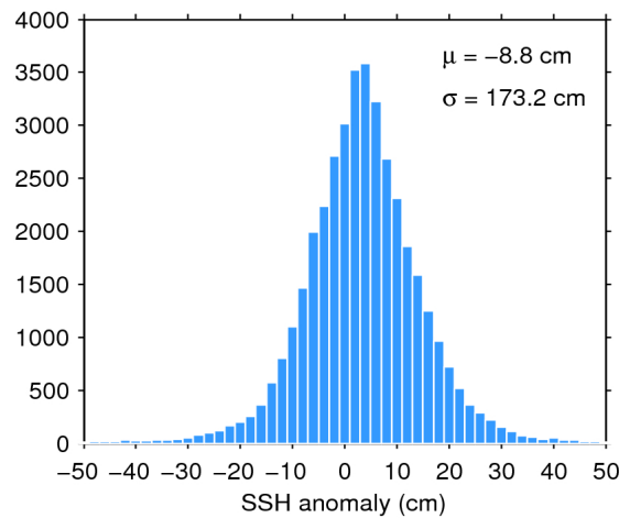
Figure 7. Histogram of flag-valid SSH anomaly over oceans and lakes for 22/09/2017. The mean ( \mu ) and standard deviation ( \sigma ) are also shown. Note that values outside [-50 50] cm are excluded from the histogram for the sake of readability but not from the computation of \mu and \sigma .
