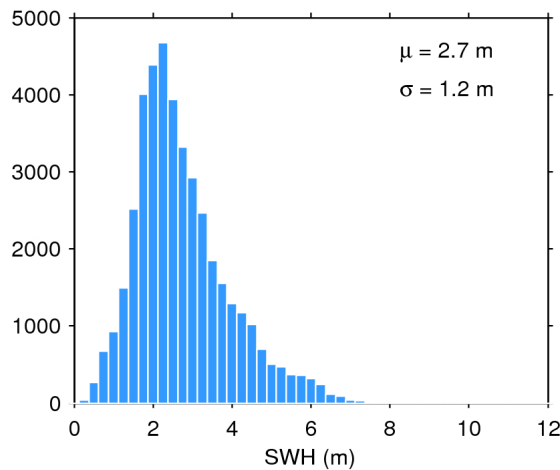
Figure 20. Histogram of science-valid SWH over oceans and lakes for 22/09/2017. The mean ( \mu ) and standard deviation ( \sigma ) are also shown. Note that values larger than 12 m are excluded from the histogram for the sake of readability but not from the computation of \mu and \sigma .
