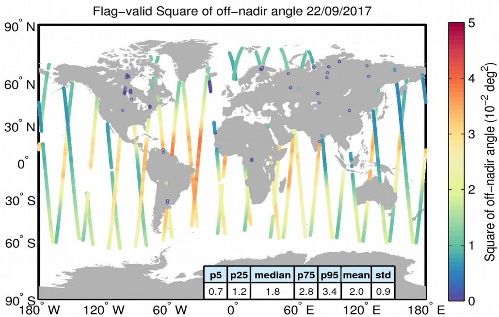
Figure 37. Geographical distribution of flag-valid mispointing data over oceans and lakes for 22/09/2017. The statistical values shown in the table refer to the mispointing in 10^{-2} deg 2 and are calculated over all measurements shown in the figure.
