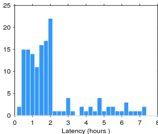
Figure 2. Histogram of the data latency for 22/09/2017. The y-axis denotes the number of files that are made available with a delay of x-hours with respect to the mean time of the records stored in the file.
