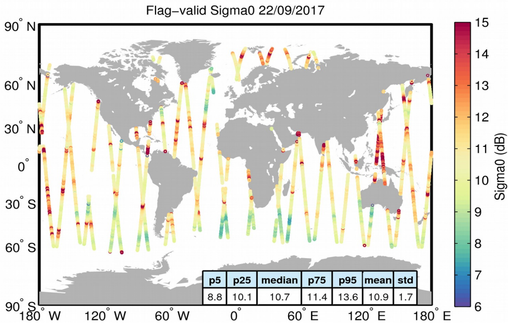
Figure 23. Geographical distribution of flag-valid sigma0 data over oceans and lakes for 22/09/2017. The statistical values shown in the table refer to the sigma0 in dB and are calculated over all measurements shown in the figure.
