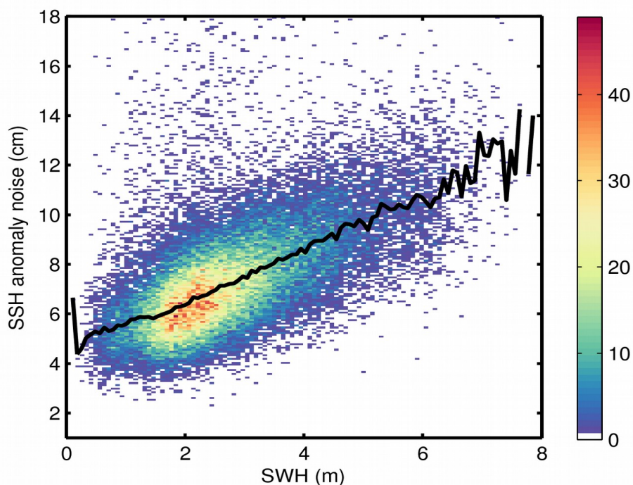
Figure 9. 2D histogram showing flag-valid SSH anomaly noise as a function of SWH for 22/09/2017. The black line denotes the median SSH anomaly noise as a function of SWH.
