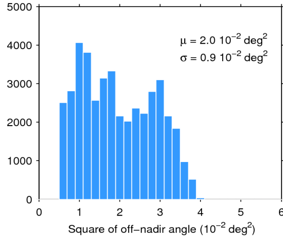
Figure 39. Histogram of flag-valid mispointing over oceans and lakes for 22/09/2017. The mean ( \mu ) and standard deviation ( \sigma ) are also shown. Note that values larger than 6 \cdot 10^{-2} \text{ deg}^2 are excluded from the histogram for the sake of readability but not from the computation of \mu and \sigma .
