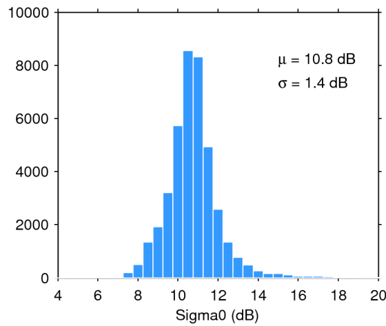
Figure 28. Histogram of science-valid sigma0 over oceans and lakes for 22/09/2017. The mean ( \mu ) and standard deviation ( \sigma ) are also shown. Note that values outside [4 20] dB are excluded from the histogram for the sake of readability but not from the computation of \mu and \sigma .
