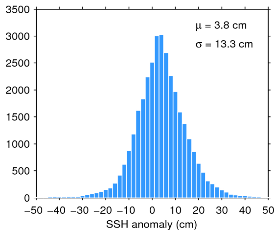
Figure 11. Histogram of science-valid SSH anomaly over oceans and lakes for 22/09/2017. The mean ( \mu ) and standard deviation ( \sigma ) are also shown. Note that values outside [-50 50] cm are excluded from the histogram for the sake of readability but not from the computation of \mu and \sigma .
