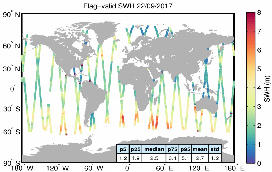
Figure 15. Geographical distribution of flag-valid SWH data over oceans and lakes for 22/09/2017. The statistical values shown in the table refer to the SWH in m and are calculated over all measurements shown in the figure.
