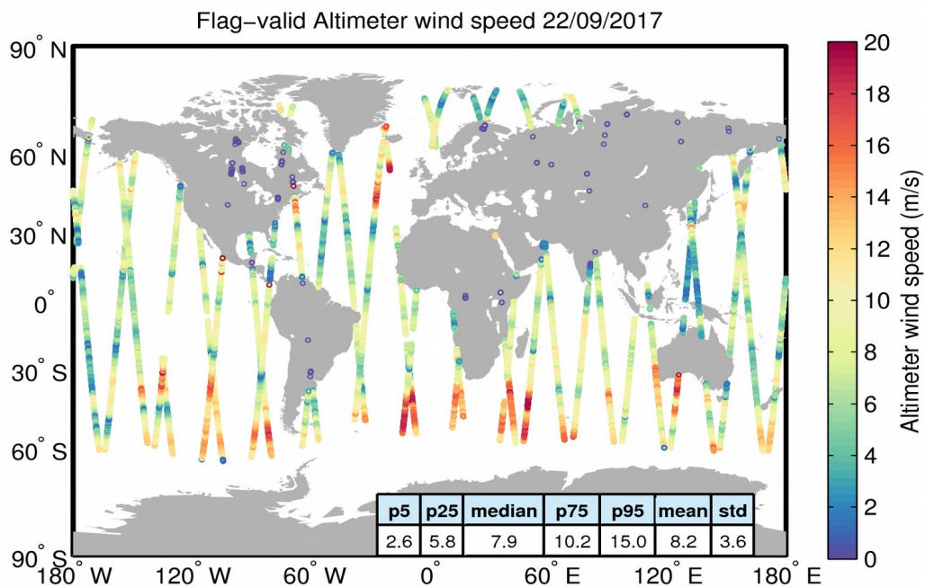
Figure 31. Geographical distribution of flag-valid wind data over oceans and lakes for 22/09/2017. The statistical values shown in the table refer to the wind in m/s and are calculated over all measurements shown in the figure.
