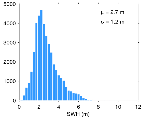
Figure 17. Histogram of flag-valid SWH over oceans and lakes for 22/09/2017. The mean ( \mu ) and standard deviation ( \sigma ) are also shown. Note that values larger than 12 m are excluded from the histogram for the sake of readability but not from the computation of \mu and \sigma .
