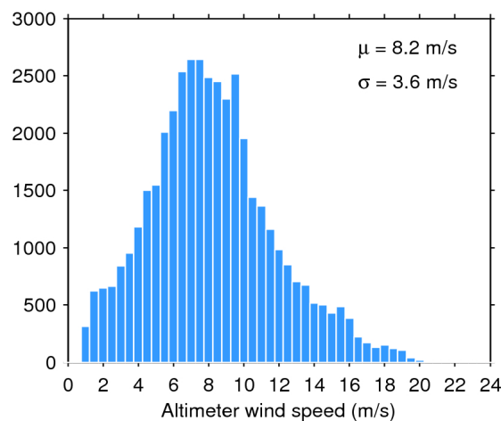
Figure 35. Histogram of science-valid wind over oceans and lakes for 22/09/2017. The mean ( \mu ) and standard deviation ( \sigma ) are also shown. Note that values larger than 24 m/s are excluded from the histogram for the sake of readability but not from the computation of \mu and \sigma .
