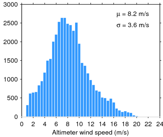
Figure 33. Histogram of flag-valid wind over oceans and lakes for 22/09/2017. The mean ( \mu ) and standard deviation ( \sigma ) are also shown. Note that values larger than 24 m/s are excluded from the histogram for the sake of readability but not from the computation of \mu and \sigma .
