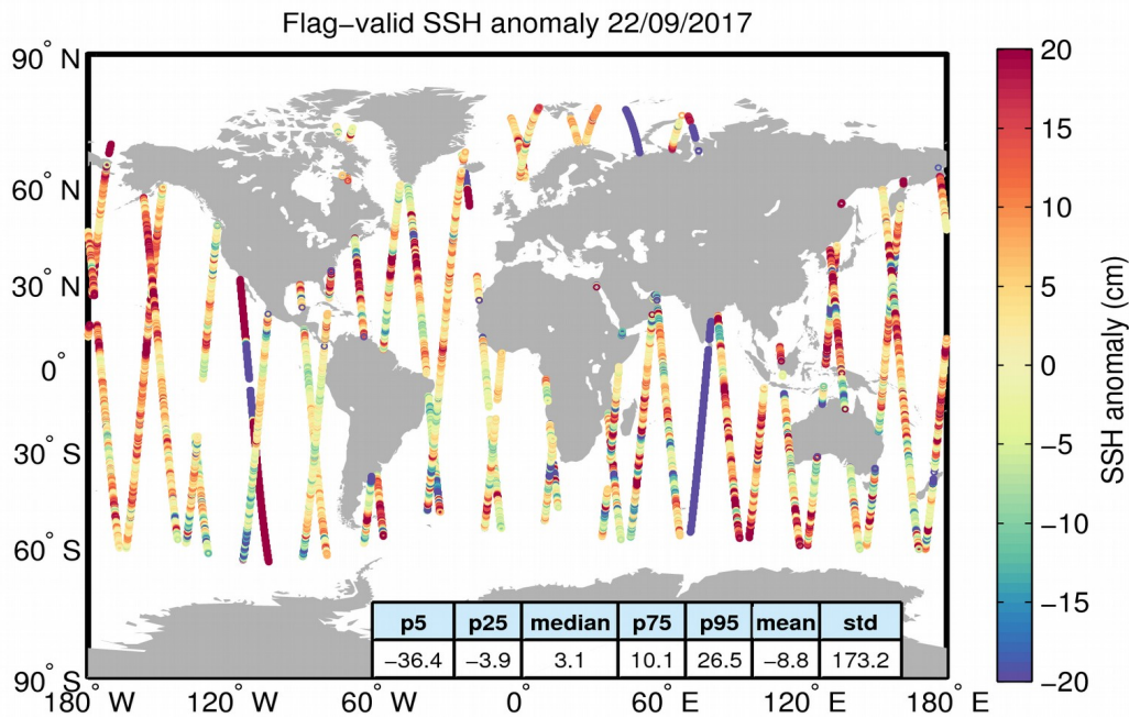
Figure 5. Geographical distribution of flag-valid 1-Hz SSH anomaly data over oceans and lakes for 22/09/2017. The statistical values shown in the table refer to the SSH anomaly in cm and are calculated over all measurements shown in the figure.
