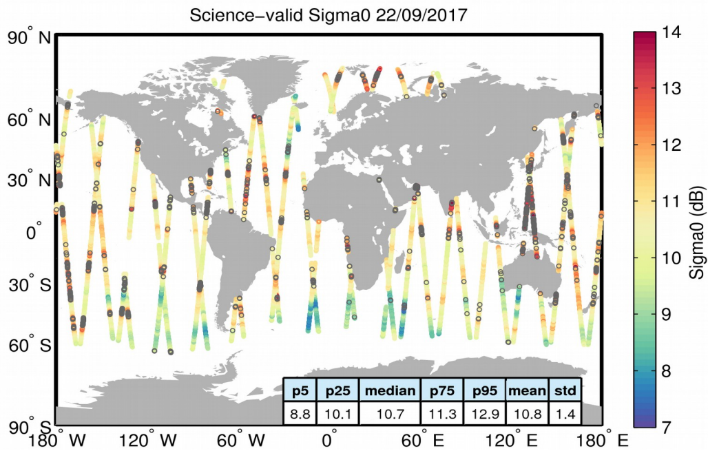
Figure 27. Geographical distribution of science-valid sigma0 data over oceans and lakes for 22/09/2017. The statistical values shown in the table refer to the sigma0 in dB and are calculated over all measurements shown in the figure. Gray circles denote records that have been rejected based on the editing criteria described in Table 4.
