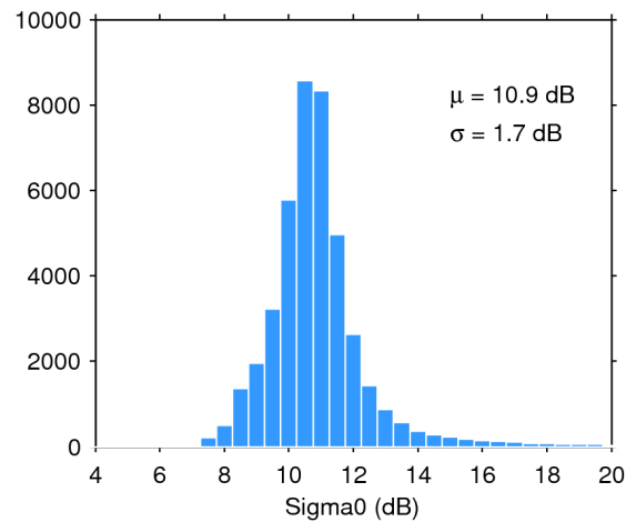
Figure 25. Histogram of flag-valid sigma0 over oceans and lakes for 22/09/2017. The mean ( \mu ) and standard deviation ( \sigma ) are also shown. Note that values outside [4 20] dB are excluded from the histogram for the sake of readability but not from the computation of \mu and \sigma .
