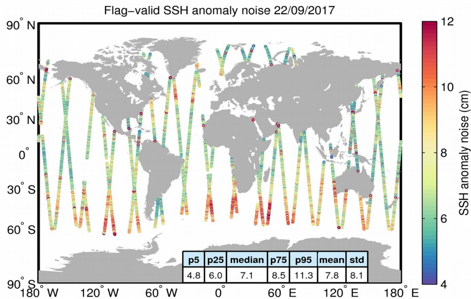
Figure 8. Geographical distribution of flag-valid 20-Hz SSH anomaly measurement noise over oceans and lakes for 22/09/2017. The statistical values shown in the table refer to the SSH anomaly noise and are calculated over all measurements shown in the figure.
