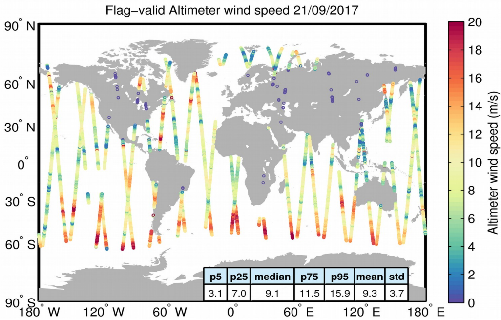
Figure 31. Geographical distribution of flag-valid wind data over oceans and lakes for 21/09/2017. The statistical values shown in the table refer to the wind in m/s and are calculated over all measurements shown in the figure.
