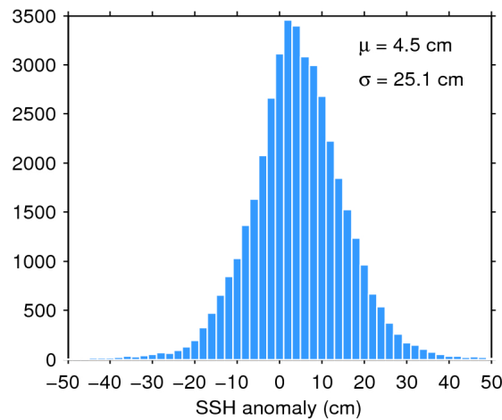
Figure 7. Histogram of flag-valid SSH anomaly over oceans and lakes for 21/09/2017. The mean ( \mu ) and standard deviation ( \sigma ) are also shown. Note that values outside [-50\ 50] cm are excluded from the histogram for the sake of readability but not from the computation of \mu and \sigma .
