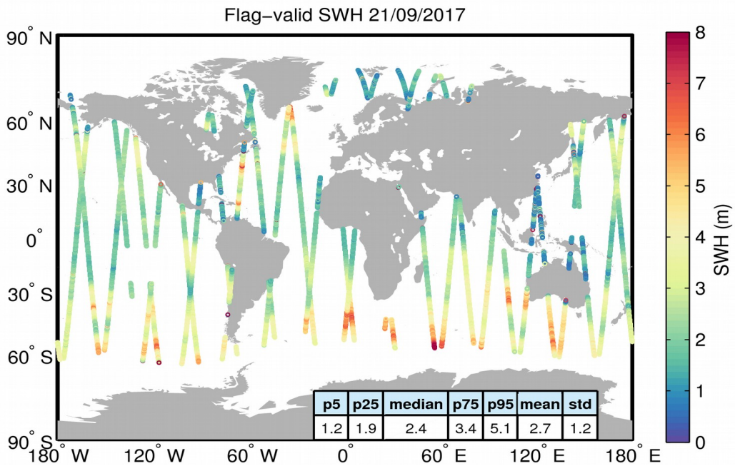
Figure 15. Geographical distribution of flag-valid SWH data over oceans and lakes for 21/09/2017. The statistical values shown in the table refer to the SWH in m and are calculated over all measurements shown in the figure.
