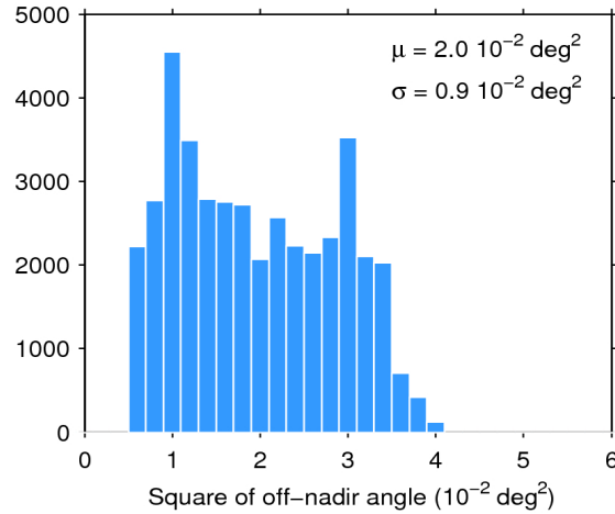
Figure 39. Histogram of flag-valid mispointing over oceans and lakes for 21/09/2017. The mean ( \mu ) and standard deviation ( \sigma ) are also shown. Note that values larger than 6 \cdot 10^{-2} \text{ deg}^2 are excluded from the histogram for the sake of readability but not from the computation of \mu and \sigma .
