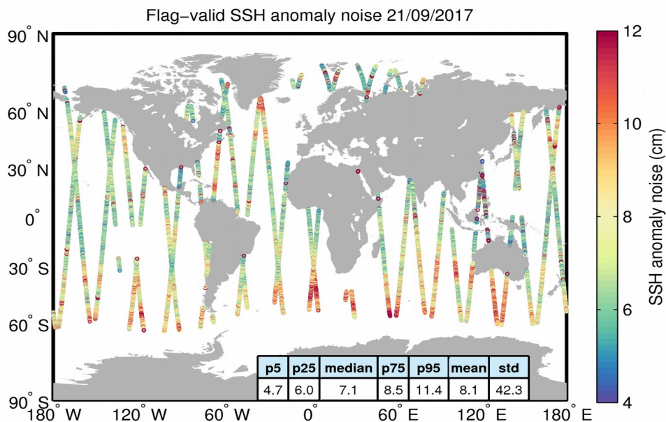
Figure 8. Geographical distribution of flag-valid 20-Hz SSH anomaly measurement noise over oceans and lakes for 21/09/2017. The statistical values shown in the table refer to the SSH anomaly noise and are calculated over all measurements shown in the figure.
