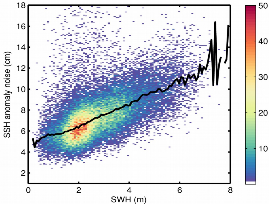
Figure 9. 2D histogram showing flag-valid SSH anomaly noise as a function of SWH for 21/09/2017. The black line denotes the median SSH anomaly noise as a function of SWH.
