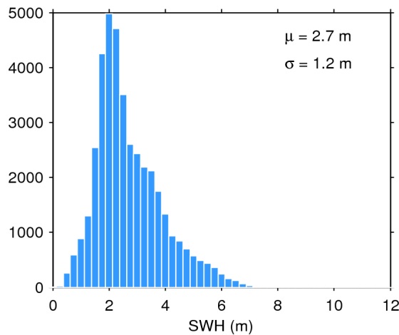
Figure 20. Histogram of science-valid SWH over oceans and lakes for 21/09/2017. The mean ( \mu ) and standard deviation ( \sigma ) are also shown. Note that values larger than 12 m are excluded from the histogram for the sake of readability but not from the computation of \mu and \sigma .
