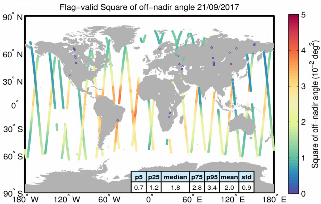
Figure 37. Geographical distribution of flag-valid mispointing data over oceans and lakes for 21/09/2017. The statistical values shown in the table refer to the mispointing in 10^{-2} deg 2 and are calculated over all measurements shown in the figure.
