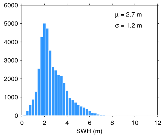
Figure 17. Histogram of flag-valid SWH over oceans and lakes for 21/09/2017. The mean ( \mu ) and standard deviation ( \sigma ) are also shown. Note that values larger than 12 m are excluded from the histogram for the sake of readability but not from the computation of \mu and \sigma .
