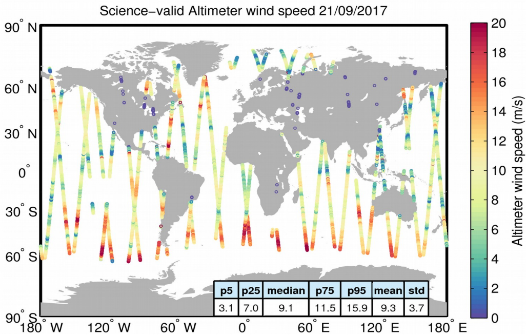
Figure 34. Geographical distribution of science-valid wind data over oceans and lakes for 21/09/2017. The statistical values shown in the table refer to the wind in m/s and are calculated over all measurements shown in the figure. Gray circles denote records that have been rejected based on the editing criteria described in Table 5.
