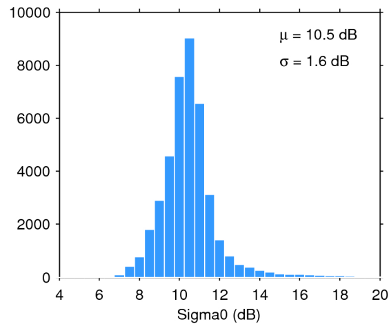
Figure 25. Histogram of flag-valid sigma0 over oceans and lakes for 21/09/2017. The mean ( \mu ) and standard deviation ( \sigma ) are also shown. Note that values outside [4 20] dB are excluded from the histogram for the sake of readability but not from the computation of \mu and \sigma .
