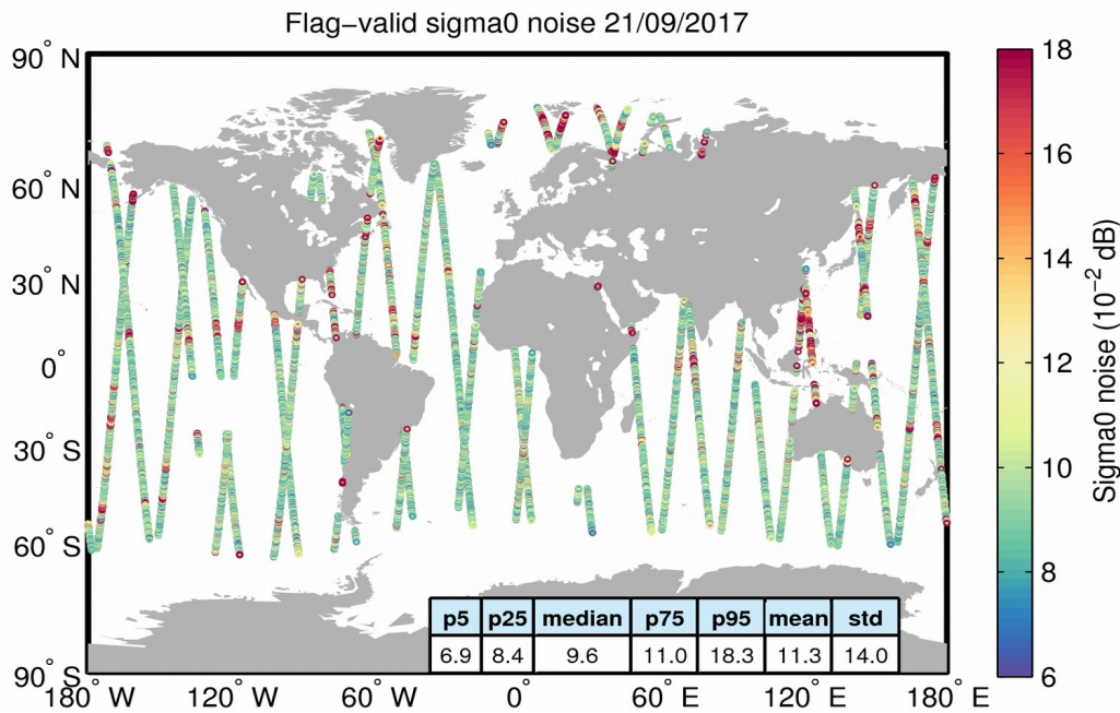
Figure 26. Geographical distribution of flag-valid 20-Hz sigma0 measurement noise over oceans and lakes for 21/09/2017. The statistical values shown in the table refer to the sigma0 noise and are calculated over all measurements shown in the figure.
