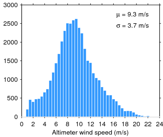
Figure 33. Histogram of flag-valid wind over oceans and lakes for 21/09/2017. The mean ( \mu ) and standard deviation ( \sigma ) are also shown. Note that values larger than 24 m/s are excluded from the histogram for the sake of readability but not from the computation of \mu and \sigma .
