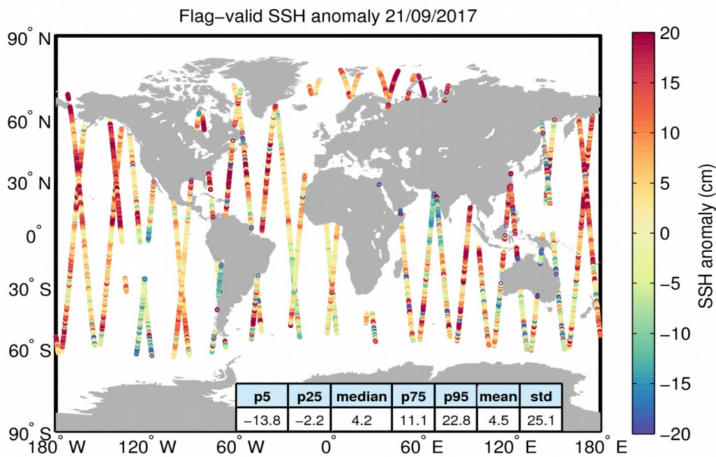
Figure 5. Geographical distribution of flag-valid 1-Hz SSH anomaly data over oceans and lakes for 21/09/2017. The statistical values shown in the table refer to the SSH anomaly in cm and are calculated over all measurements shown in the figure.
