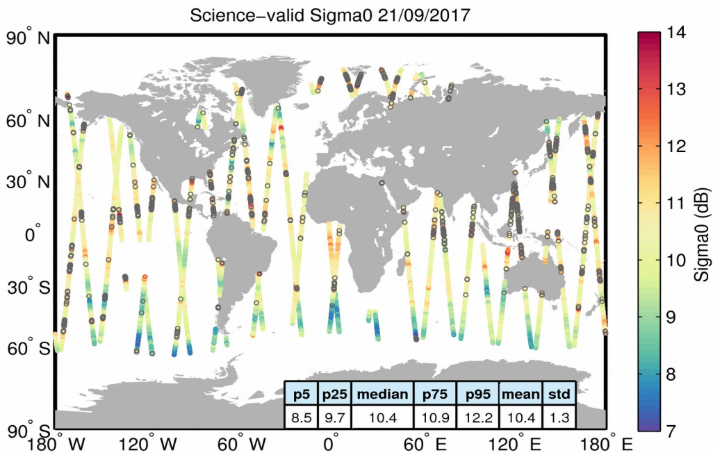
Figure 27. Geographical distribution of science-valid sigma0 data over oceans and lakes for 21/09/2017. The statistical values shown in the table refer to the sigma0 in dB and are calculated over all measurements shown in the figure. Gray circles denote records that have been rejected based on the editing criteria described in Table 4.
