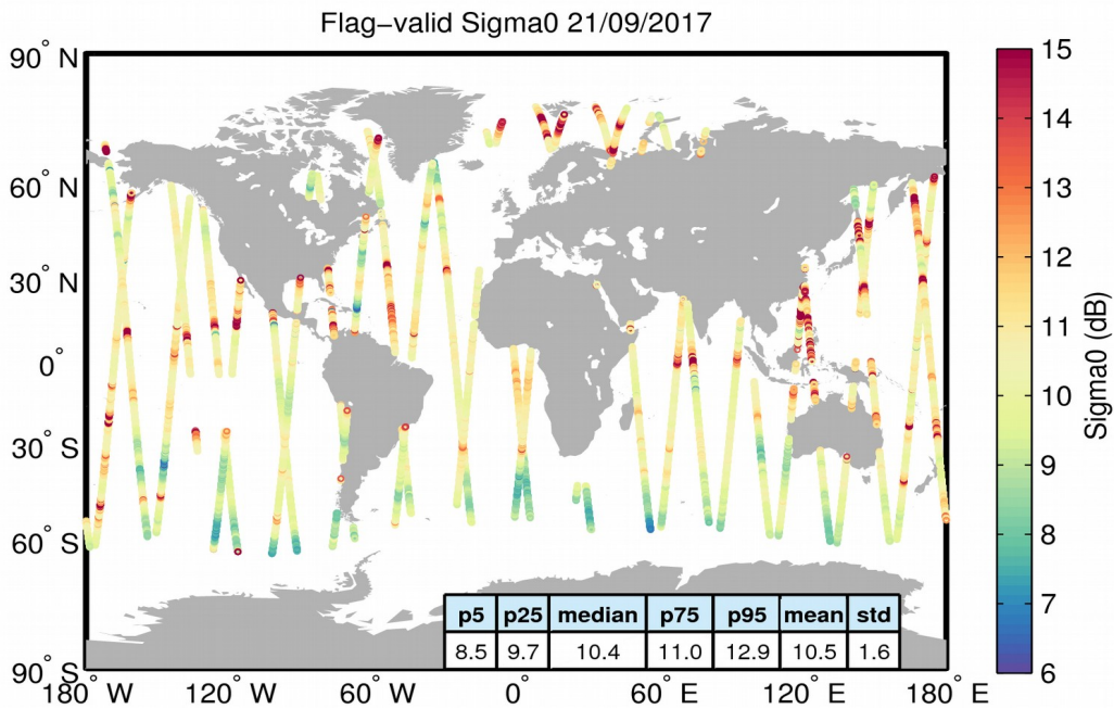
Figure 23. Geographical distribution of flag-valid sigma0 data over oceans and lakes for 21/09/2017. The statistical values shown in the table refer to the sigma0 in dB and are calculated over all measurements shown in the figure.
