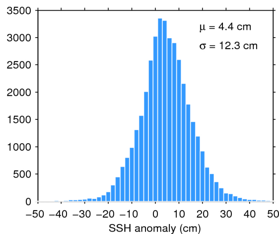
Figure 11. Histogram of science-valid SSH anomaly over oceans and lakes for 21/09/2017. The mean ( \mu ) and standard deviation ( \sigma ) are also shown. Note that values outside [-50 50] cm are excluded from the histogram for the sake of readability but not from the computation of \mu and \sigma .
