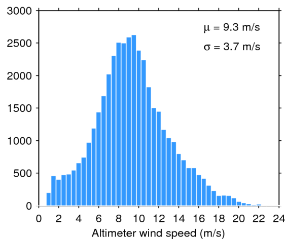
Figure 35. Histogram of science-valid wind over oceans and lakes for 21/09/2017. The mean ( \mu ) and standard deviation ( \sigma ) are also shown. Note that values larger than 24 m/s are excluded from the histogram for the sake of readability but not from the computation of \mu and \sigma .
