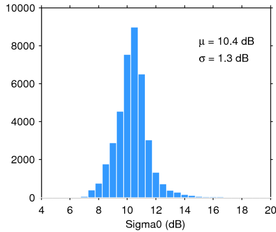
Figure 28. Histogram of science-valid sigma0 over oceans and lakes for 21/09/2017. The mean ( \mu ) and standard deviation ( \sigma ) are also shown. Note that values outside [4 20] dB are excluded from the histogram for the sake of readability but not from the computation of \mu and \sigma .
