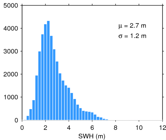
Figure 20. Histogram of science-valid SWH over oceans and lakes for 20/09/2017. The mean ( \mu ) and standard deviation ( \sigma ) are also shown. Note that values larger than 12 m are excluded from the histogram for the sake of readability but not from the computation of \mu and \sigma .
