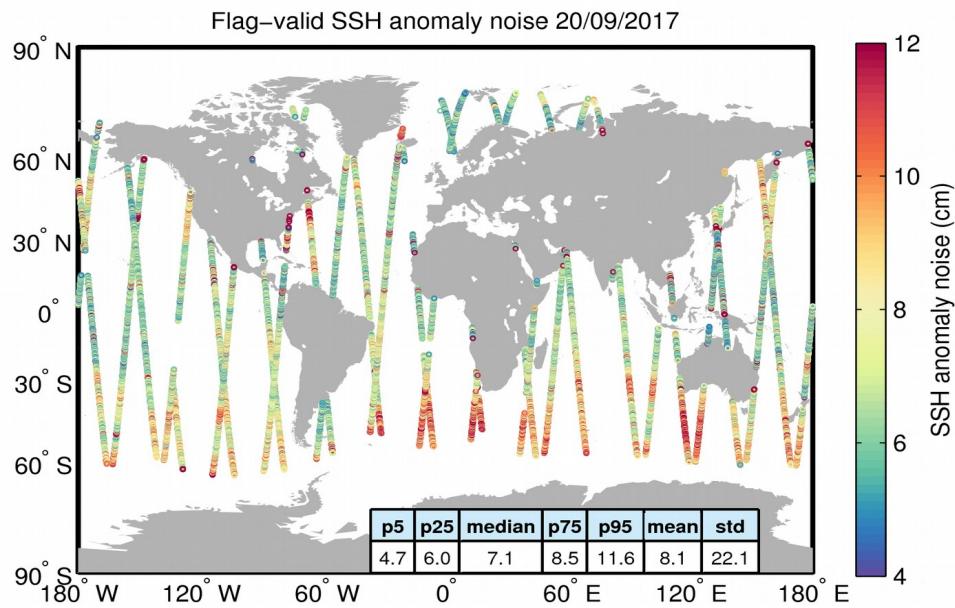
Figure 8. Geographical distribution of flag-valid 20-Hz SSH anomaly measurement noise over oceans and lakes for 20/09/2017. The statistical values shown in the table refer to the SSH anomaly noise and are calculated over all measurements shown in the figure.
