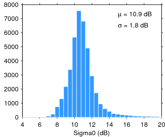
Figure 25. Histogram of flag-valid sigma0 over oceans and lakes for 20/09/2017. The mean ( \mu ) and standard deviation ( \sigma ) are also shown. Note that values outside [4 20] dB are excluded from the histogram for the sake of readability but not from the computation of \mu and \sigma .
