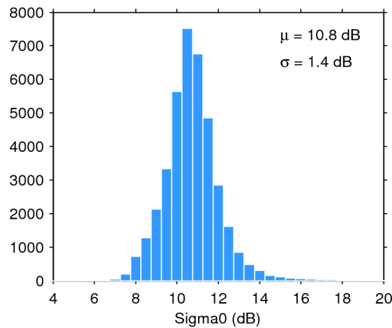
Figure 28. Histogram of science-valid sigma0 over oceans and lakes for 20/09/2017. The mean ( \mu ) and standard deviation ( \sigma ) are also shown. Note that values outside [4 20] dB are excluded from the histogram for the sake of readability but not from the computation of \mu and \sigma .
