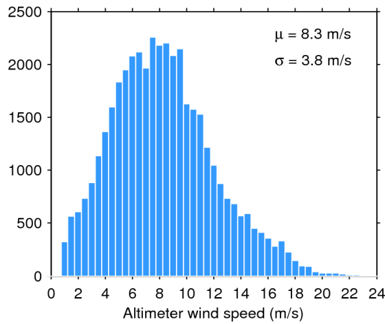
Figure 33. Histogram of flag-valid wind over oceans and lakes for 20/09/2017. The mean ( \mu ) and standard deviation ( \sigma ) are also shown. Note that values larger than 24 m/s are excluded from the histogram for the sake of readability but not from the computation of \mu and \sigma .
