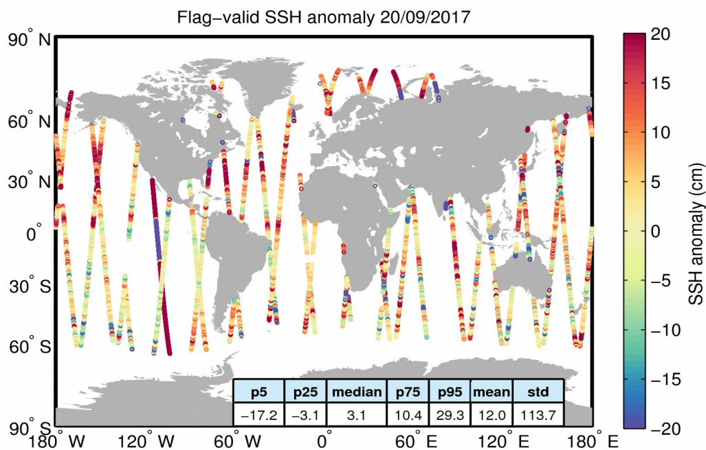
Figure 5. Geographical distribution of flag-valid 1-Hz SSH anomaly data over oceans and lakes for 20/09/2017. The statistical values shown in the table refer to the SSH anomaly in cm and are calculated over all measurements shown in the figure.
