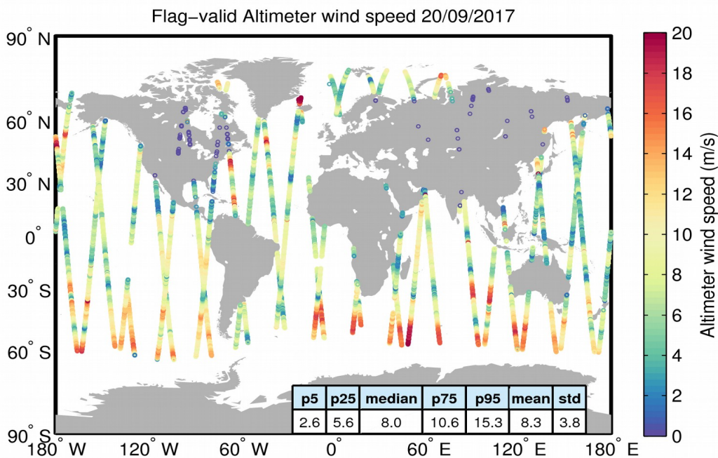
Figure 31. Geographical distribution of flag-valid wind data over oceans and lakes for 20/09/2017. The statistical values shown in the table refer to the wind in m/s and are calculated over all measurements shown in the figure.
