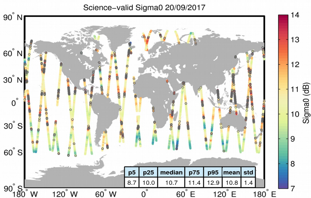
Figure 27. Geographical distribution of science-valid sigma0 data over oceans and lakes for 20/09/2017. The statistical values shown in the table refer to the sigma0 in dB and are calculated over all measurements shown in the figure. Gray circles denote records that have been rejected based on the editing criteria described in Table 4.
