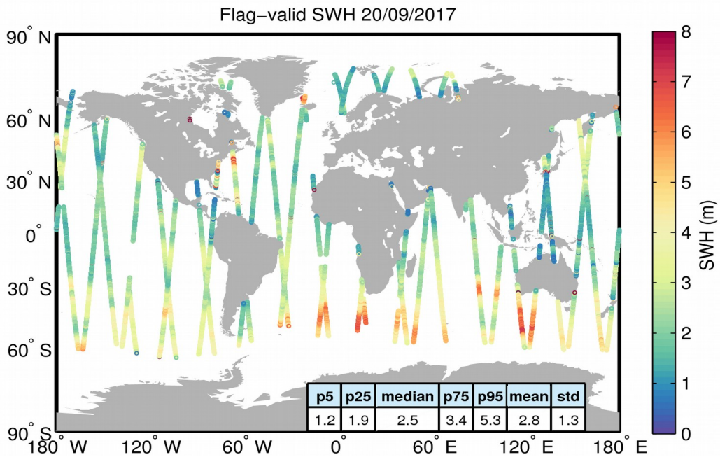
Figure 15. Geographical distribution of flag-valid SWH data over oceans and lakes for 20/09/2017. The statistical values shown in the table refer to the SWH in m and are calculated over all measurements shown in the figure.
