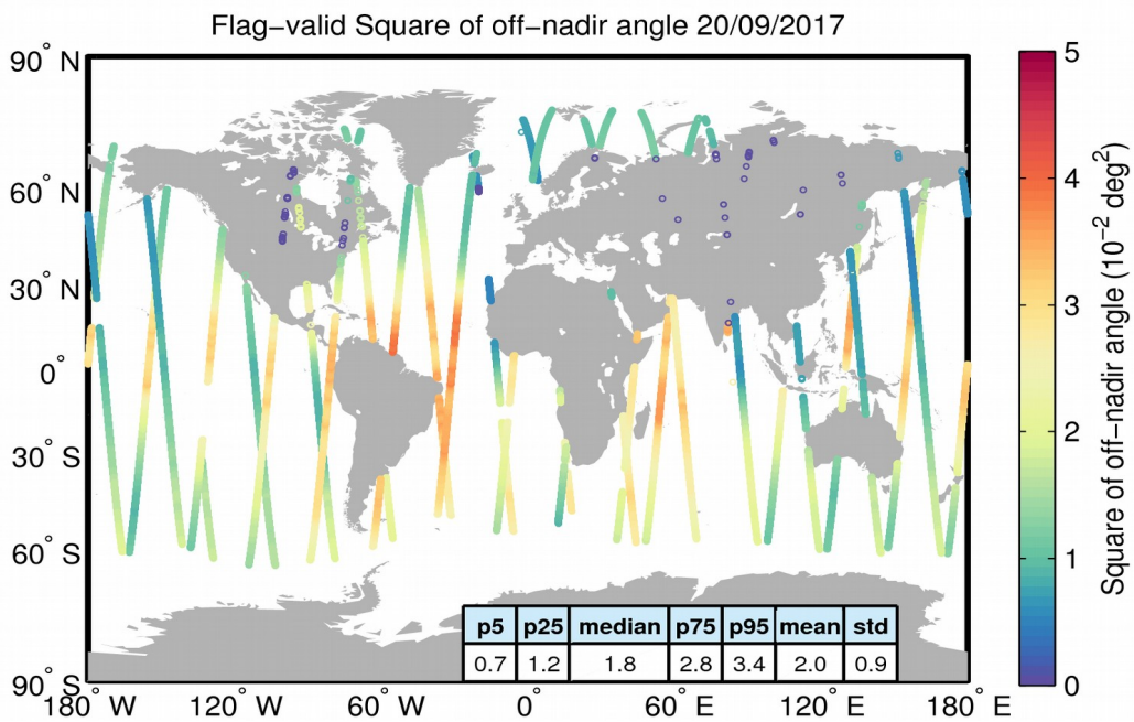
Figure 37. Geographical distribution of flag-valid mispointing data over oceans and lakes for 20/09/2017. The statistical values shown in the table refer to the mispointing in 10^{-2} deg 2 and are calculated over all measurements shown in the figure.
