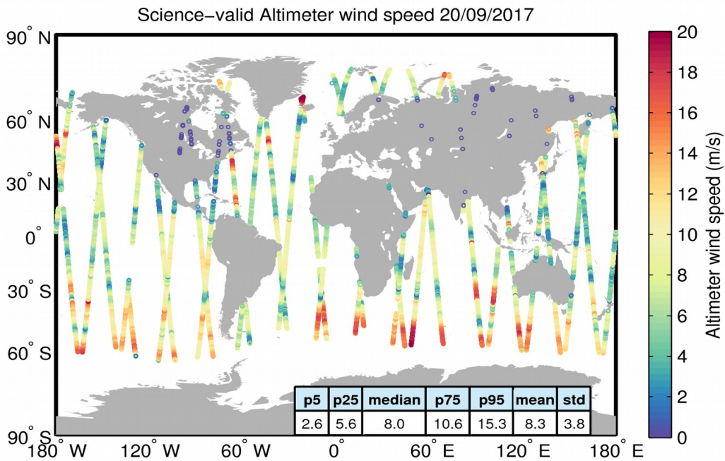
Figure 34. Geographical distribution of science-valid wind data over oceans and lakes for 20/09/2017. The statistical values shown in the table refer to the wind in m/s and are calculated over all measurements shown in the figure. Gray circles denote records that have been rejected based on the editing criteria described in Table 5.
