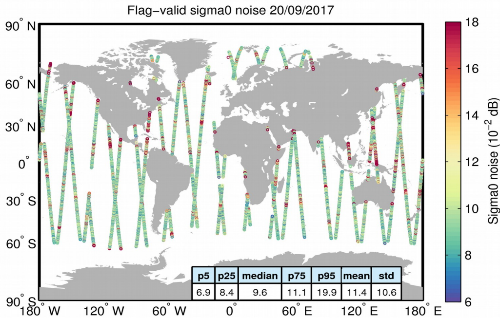
Figure 26. Geographical distribution of flag-valid 20-Hz sigma0 measurement noise over oceans and lakes for 20/09/2017. The statistical values shown in the table refer to the sigma0 noise and are calculated over all measurements shown in the figure.
