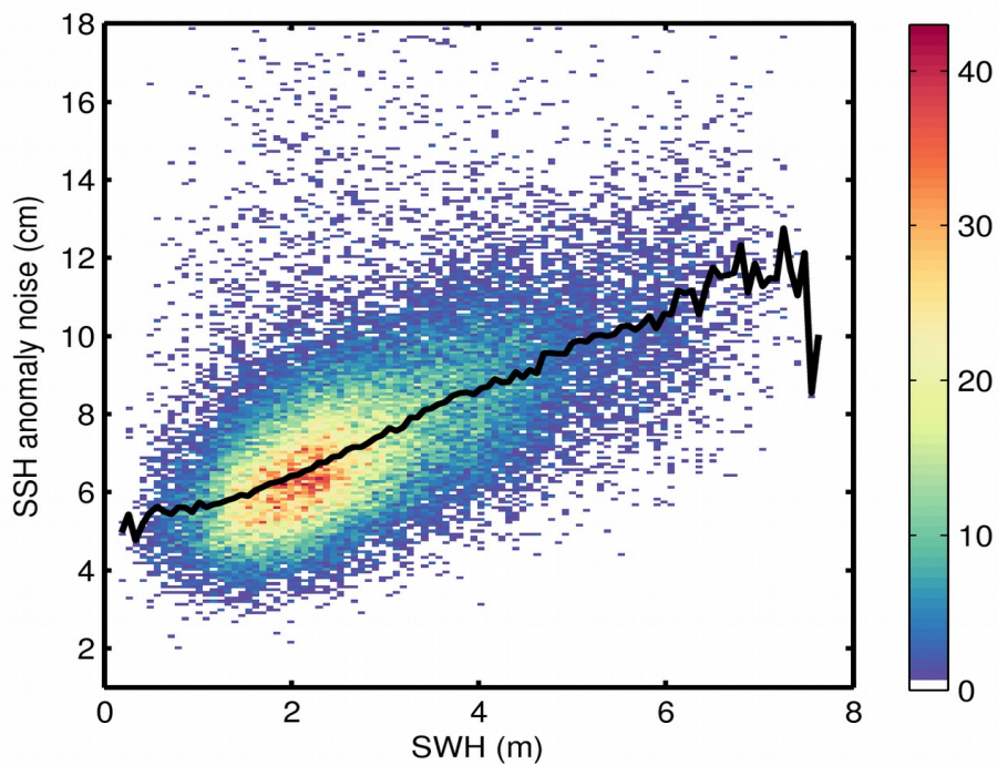
Figure 9. 2D histogram showing flag-valid SSH anomaly noise as a function of SWH for 20/09/2017. The black line denotes the median SSH anomaly noise as a function of SWH.
