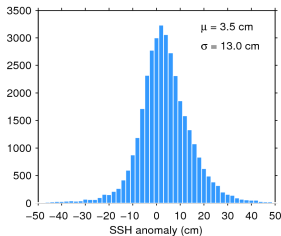
Figure 11. Histogram of science-valid SSH anomaly over oceans and lakes for 20/09/2017. The mean ( \mu ) and standard deviation ( \sigma ) are also shown. Note that values outside [-50 50] cm are excluded from the histogram for the sake of readability but not from the computation of \mu and \sigma .
