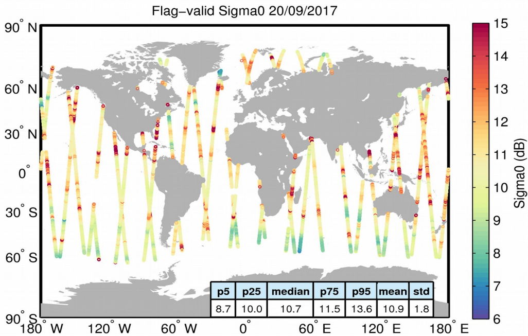
Figure 23. Geographical distribution of flag-valid sigma0 data over oceans and lakes for 20/09/2017. The statistical values shown in the table refer to the sigma0 in dB and are calculated over all measurements shown in the figure.
