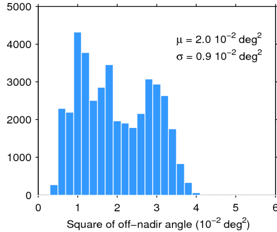
Figure 39. Histogram of flag-valid mispointing over oceans and lakes for 20/09/2017. The mean ( \mu ) and standard deviation ( \sigma ) are also shown. Note that values larger than 6 \cdot 10^{-2} \text{ deg}^2 are excluded from the histogram for the sake of readability but not from the computation of \mu and \sigma .
