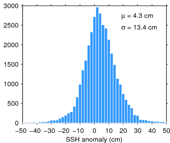
Figure 11. Histogram of science-valid SSH anomaly over oceans and lakes for 18/09/2017. The mean ( \mu ) and standard deviation ( \sigma ) are also shown. Note that values outside [-50 50] cm are excluded from the histogram for the sake of readability but not from the computation of \mu and \sigma .
