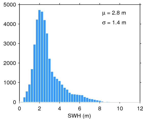
Figure 20. Histogram of science-valid SWH over oceans and lakes for 18/09/2017. The mean ( \mu ) and standard deviation ( \sigma ) are also shown. Note that values larger than 12 m are excluded from the histogram for the sake of readability but not from the computation of \mu and \sigma .
