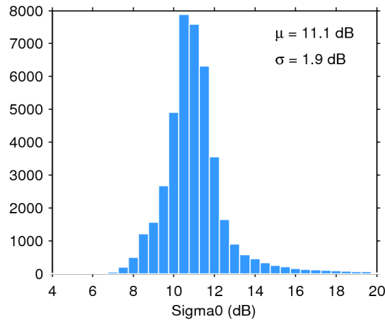
Figure 25. Histogram of flag-valid sigma0 over oceans and lakes for 18/09/2017. The mean ( \mu ) and standard deviation ( \sigma ) are also shown. Note that values outside [4 20] dB are excluded from the histogram for the sake of readability but not from the computation of \mu and \sigma .
