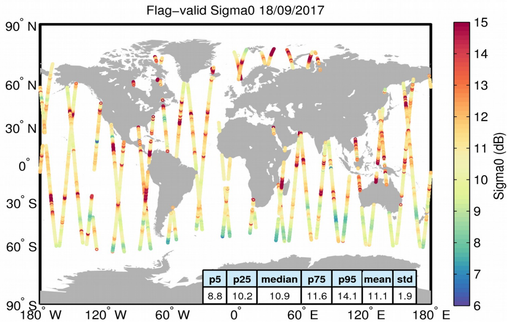
Figure 23. Geographical distribution of flag-valid sigma0 data over oceans and lakes for 18/09/2017. The statistical values shown in the table refer to the sigma0 in dB and are calculated over all measurements shown in the figure.
