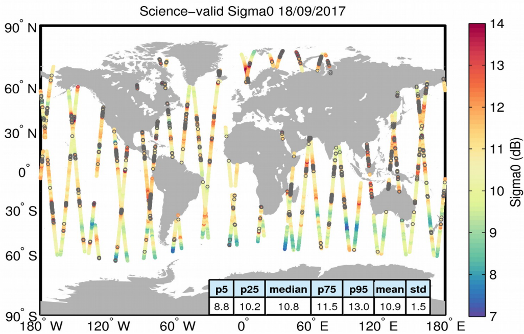
Figure 27. Geographical distribution of science-valid sigma0 data over oceans and lakes for 18/09/2017. The statistical values shown in the table refer to the sigma0 in dB and are calculated over all measurements shown in the figure. Gray circles denote records that have been rejected based on the editing criteria described in Table 4.
