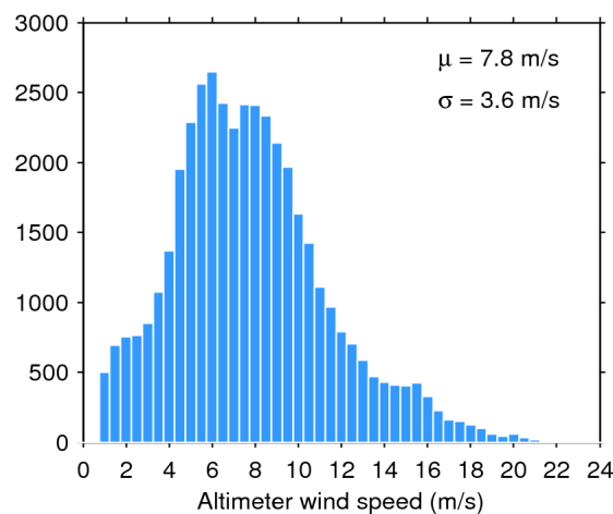
Figure 35. Histogram of science-valid wind over oceans and lakes for 18/09/2017. The mean ( \mu ) and standard deviation ( \sigma ) are also shown. Note that values larger than 24 m/s are excluded from the histogram for the sake of readability but not from the computation of \mu and \sigma .
