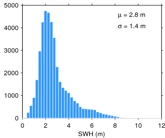
Figure 17. Histogram of flag-valid SWH over oceans and lakes for 18/09/2017. The mean ( \mu ) and standard deviation ( \sigma ) are also shown. Note that values larger than 12 m are excluded from the histogram for the sake of readability but not from the computation of \mu and \sigma .
