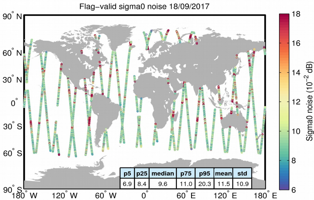
Figure 26. Geographical distribution of flag-valid 20-Hz sigma0 measurement noise over oceans and lakes for 18/09/2017. The statistical values shown in the table refer to the sigma0 noise and are calculated over all measurements shown in the figure.
