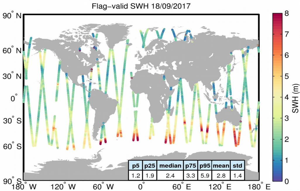
Figure 15. Geographical distribution of flag-valid SWH data over oceans and lakes for 18/09/2017. The statistical values shown in the table refer to the SWH in m and are calculated over all measurements shown in the figure.
