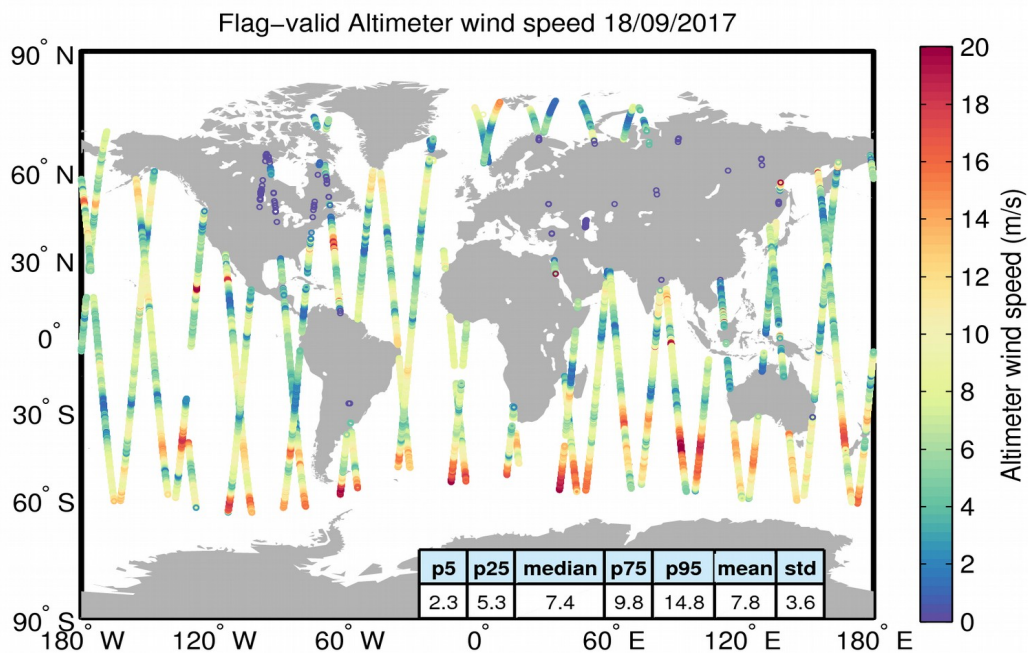
Figure 31. Geographical distribution of flag-valid wind data over oceans and lakes for 18/09/2017. The statistical values shown in the table refer to the wind in m/s and are calculated over all measurements shown in the figure.
