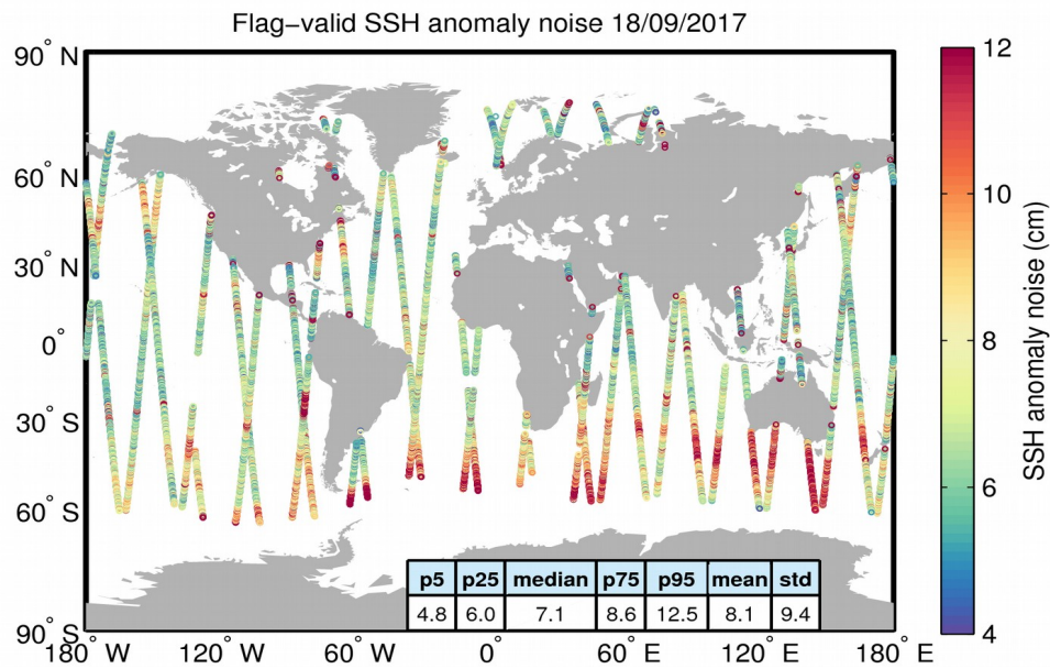
Figure 8. Geographical distribution of flag-valid 20-Hz SSH anomaly measurement noise over oceans and lakes for 18/09/2017. The statistical values shown in the table refer to the SSH anomaly noise and are calculated over all measurements shown in the figure.
