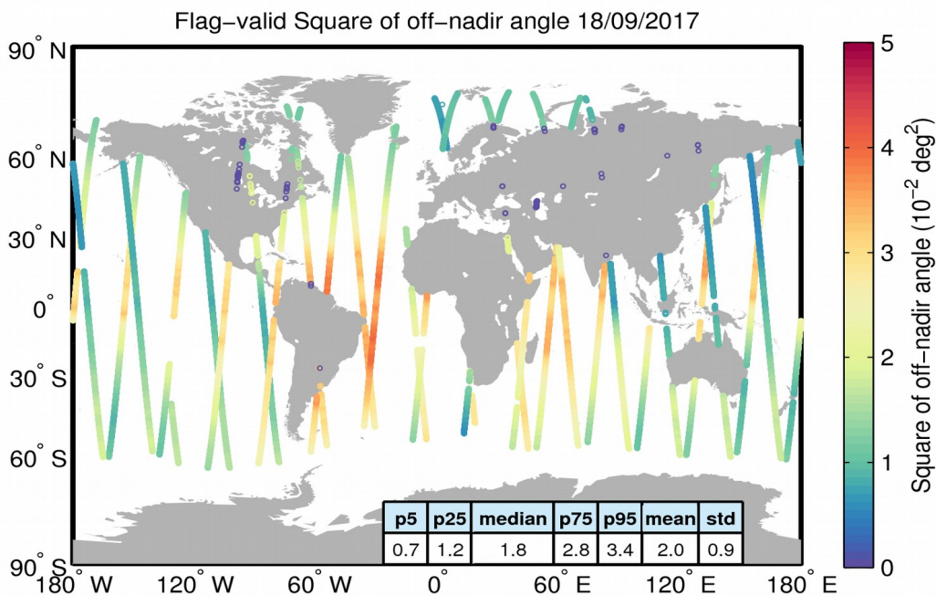
Figure 37. Geographical distribution of flag-valid mispointing data over oceans and lakes for 18/09/2017. The statistical values shown in the table refer to the mispointing in 10^{-2} deg 2 and are calculated over all measurements shown in the figure.
