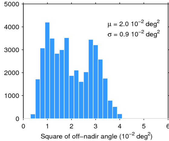
Figure 39. Histogram of flag-valid mispointing over oceans and lakes for 18/09/2017. The mean ( \mu ) and standard deviation ( \sigma ) are also shown. Note that values larger than 6 \cdot 10^{-2} \text{ deg}^2 are excluded from the histogram for the sake of readability but not from the computation of \mu and \sigma .
