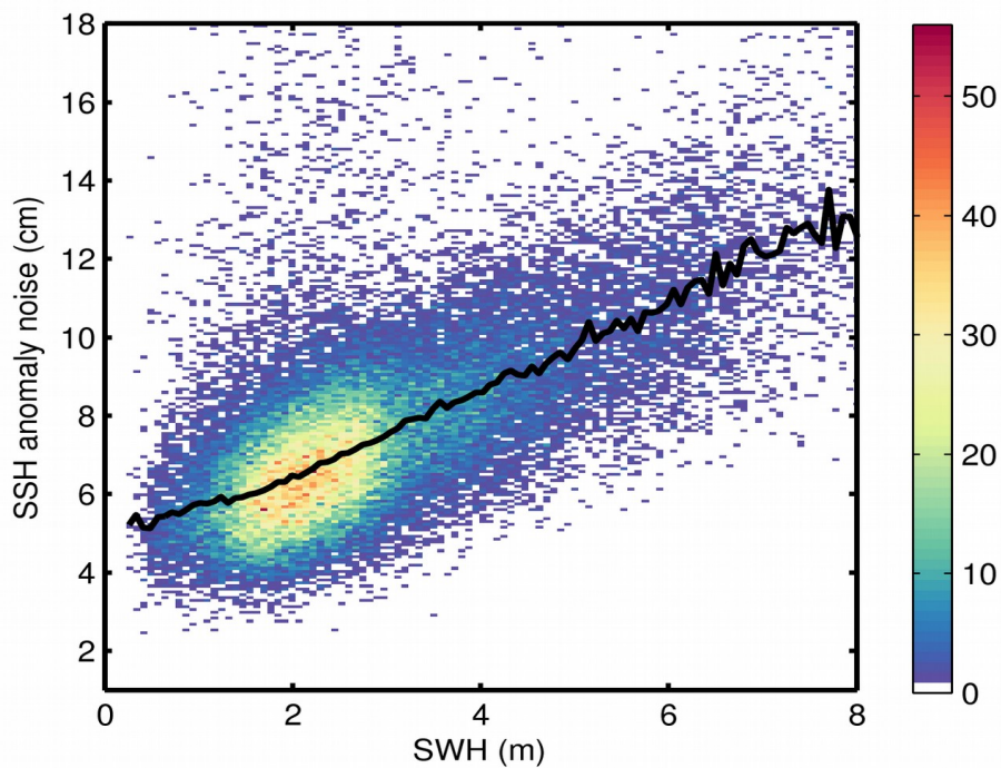
Figure 9. 2D histogram showing flag-valid SSH anomaly noise as a function of SWH for 18/09/2017. The black line denotes the median SSH anomaly noise as a function of SWH.
