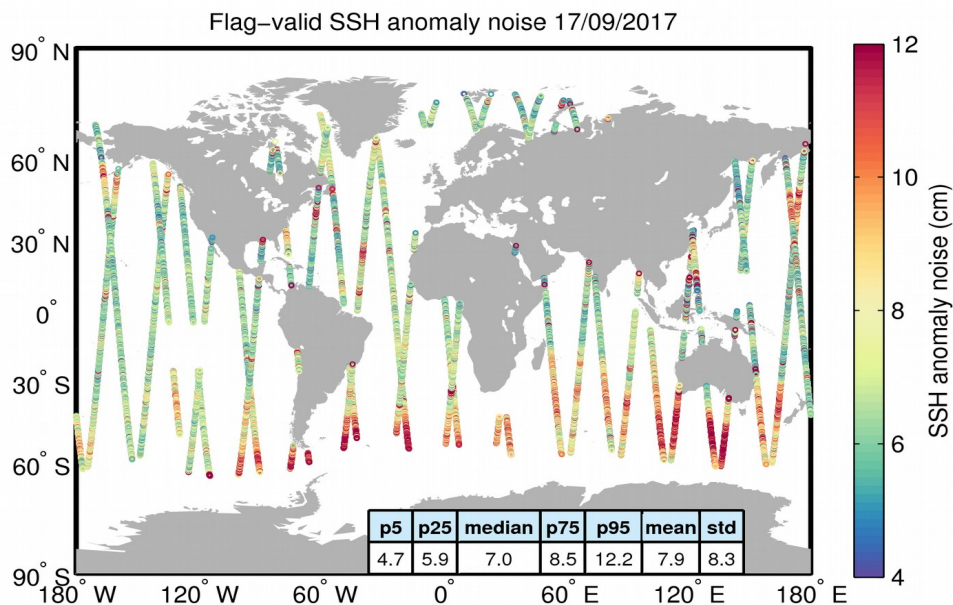
Figure 8. Geographical distribution of flag-valid 20-Hz SSH anomaly measurement noise over oceans and lakes for 17/09/2017. The statistical values shown in the table refer to the SSH anomaly noise and are calculated over all measurements shown in the figure.
