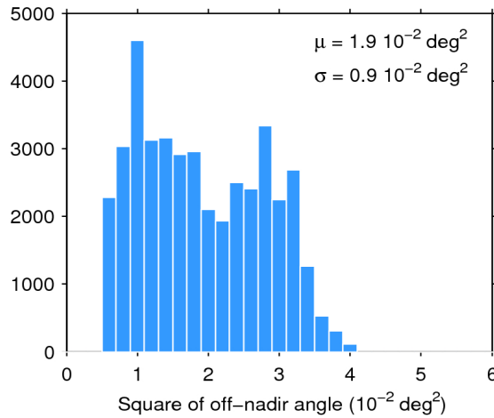
Figure 39. Histogram of flag-valid mispointing over oceans and lakes for 17/09/2017. The mean ( \mu ) and standard deviation ( \sigma ) are also shown. Note that values larger than 6 \cdot 10^{-2} \text{ deg}^2 are excluded from the histogram for the sake of readability but not from the computation of \mu and \sigma .
