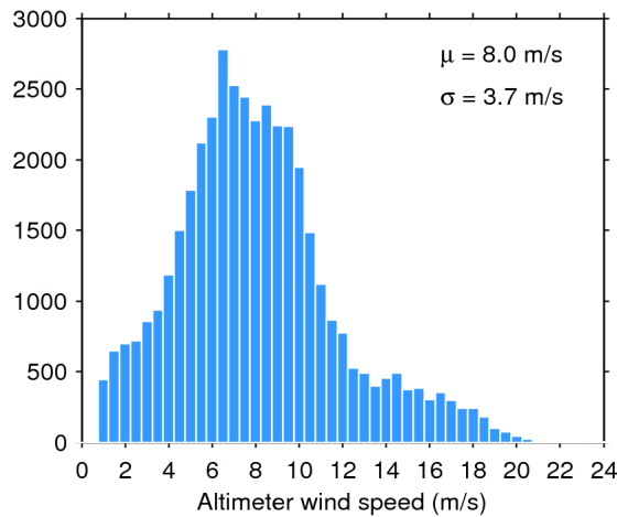
Figure 33. Histogram of flag-valid wind over oceans and lakes for 17/09/2017. The mean ( \mu ) and standard deviation ( \sigma ) are also shown. Note that values larger than 24 m/s are excluded from the histogram for the sake of readability but not from the computation of \mu and \sigma .
