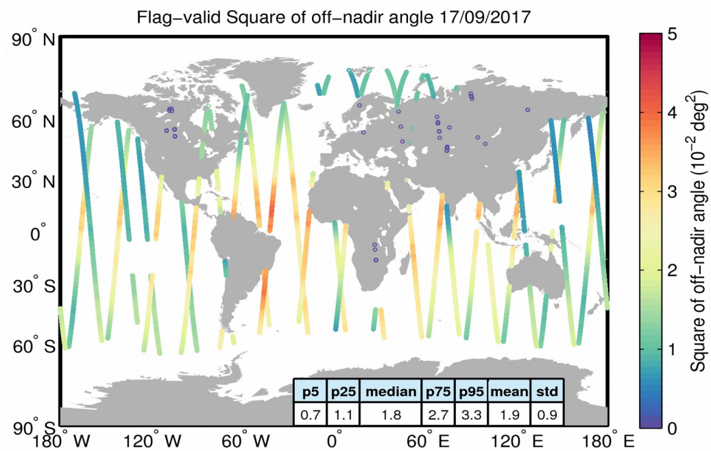
Figure 37. Geographical distribution of flag-valid mispointing data over oceans and lakes for 17/09/2017. The statistical values shown in the table refer to the mispointing in 10^{-2} deg 2 and are calculated over all measurements shown in the figure.
