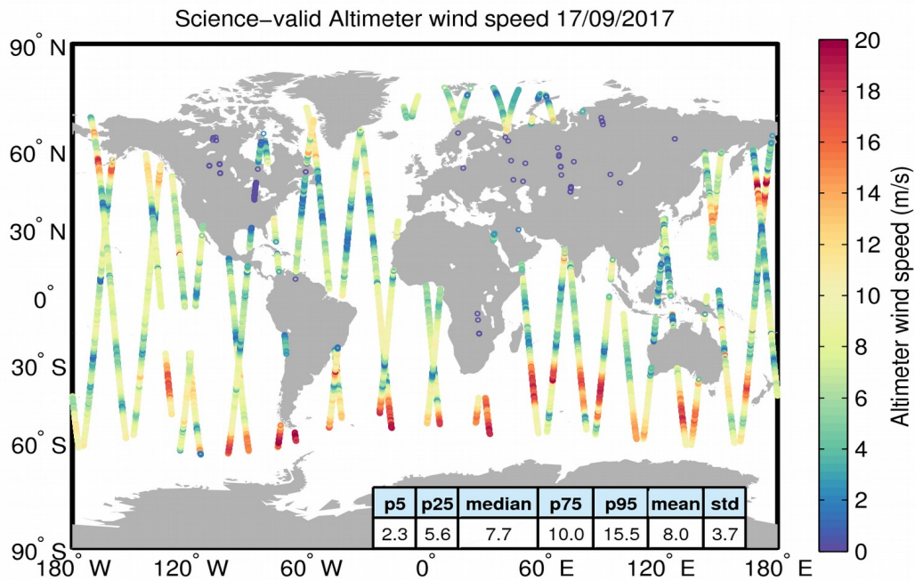
Figure 34. Geographical distribution of science-valid wind data over oceans and lakes for 17/09/2017. The statistical values shown in the table refer to the wind in m/s and are calculated over all measurements shown in the figure. Gray circles denote records that have been rejected based on the editing criteria described in Table 5.
