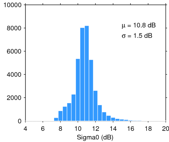
Figure 28. Histogram of science-valid sigma0 over oceans and lakes for 17/09/2017. The mean ( \mu ) and standard deviation ( \sigma ) are also shown. Note that values outside [4 20] dB are excluded from the histogram for the sake of readability but not from the computation of \mu and \sigma .
