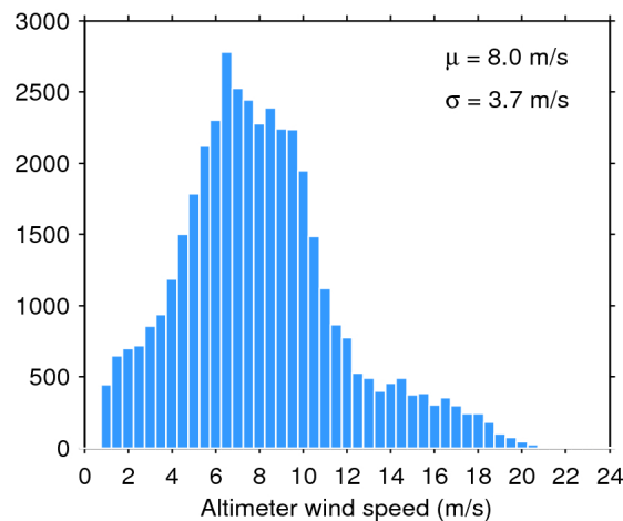
Figure 35. Histogram of science-valid wind over oceans and lakes for 17/09/2017. The mean ( \mu ) and standard deviation ( \sigma ) are also shown. Note that values larger than 24 m/s are excluded from the histogram for the sake of readability but not from the computation of \mu and \sigma .
