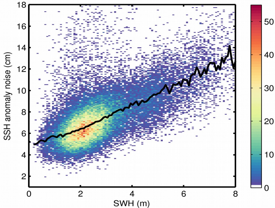
Figure 9. 2D histogram showing flag-valid SSH anomaly noise as a function of SWH for 17/09/2017. The black line denotes the median SSH anomaly noise as a function of SWH.
