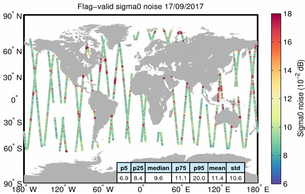
Figure 26. Geographical distribution of flag-valid 20-Hz sigma0 measurement noise over oceans and lakes for 17/09/2017. The statistical values shown in the table refer to the sigma0 noise and are calculated over all measurements shown in the figure.
