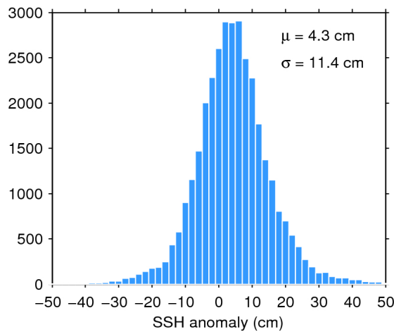
Figure 11. Histogram of science-valid SSH anomaly over oceans and lakes for 17/09/2017. The mean ( \mu ) and standard deviation ( \sigma ) are also shown. Note that values outside [-50 50] cm are excluded from the histogram for the sake of readability but not from the computation of \mu and \sigma .
