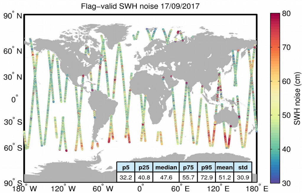
Figure 18. Geographical distribution of flag-valid 20-Hz SWH measurement noise over oceans and lakes for 17/09/2017. The statistical values shown in the table refer to the SWH noise and are calculated over all measurements shown in the figure.
