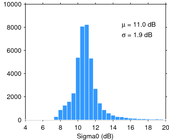
Figure 25. Histogram of flag-valid sigma0 over oceans and lakes for 17/09/2017. The mean ( \mu ) and standard deviation ( \sigma ) are also shown. Note that values outside [4 20] dB are excluded from the histogram for the sake of readability but not from the computation of \mu and \sigma .
