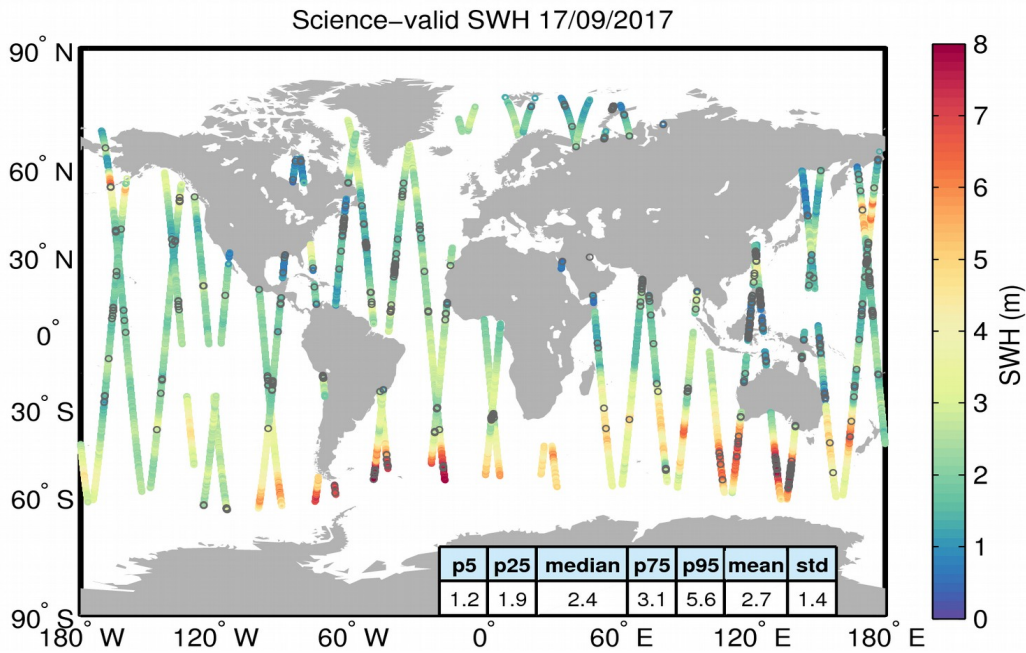
Figure 19. Geographical distribution of science-valid SWH data over oceans and lakes for 17/09/2017. The statistical values shown in the table refer to the SWH in m and are calculated over all measurements shown in the figure. Gray circles denote records that have been rejected based on the editing criteria described in Table 3.
