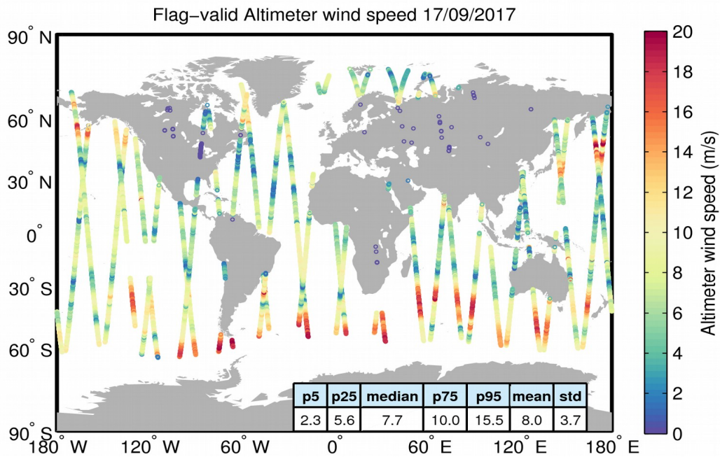
Figure 31. Geographical distribution of flag-valid wind data over oceans and lakes for 17/09/2017. The statistical values shown in the table refer to the wind in m/s and are calculated over all measurements shown in the figure.
