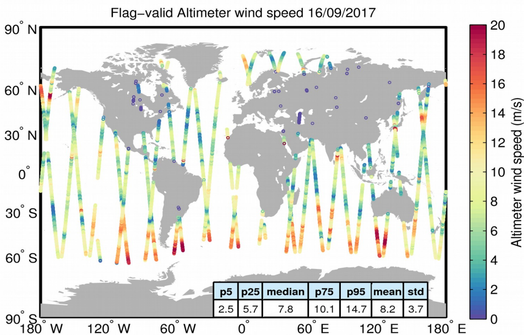
Figure 31. Geographical distribution of flag-valid wind data over oceans and lakes for 16/09/2017. The statistical values shown in the table refer to the wind in m/s and are calculated over all measurements shown in the figure.
