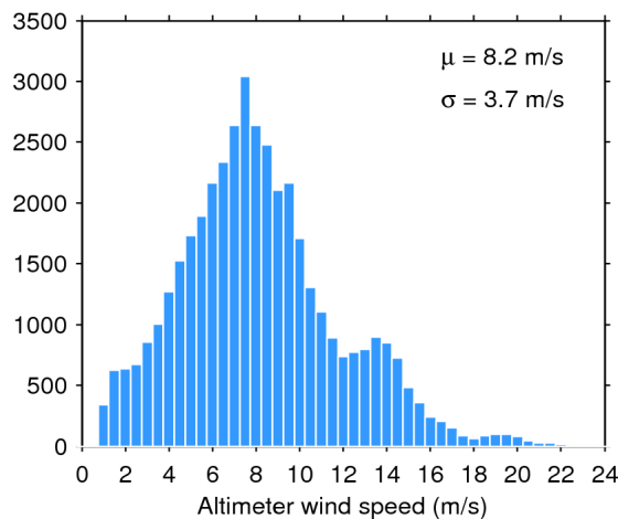
Figure 35. Histogram of science-valid wind over oceans and lakes for 16/09/2017. The mean ( \mu ) and standard deviation ( \sigma ) are also shown. Note that values larger than 24 m/s are excluded from the histogram for the sake of readability but not from the computation of \mu and \sigma .
