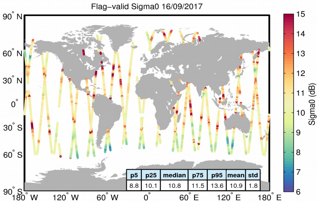
Figure 23. Geographical distribution of flag-valid sigma0 data over oceans and lakes for 16/09/2017. The statistical values shown in the table refer to the sigma0 in dB and are calculated over all measurements shown in the figure.
