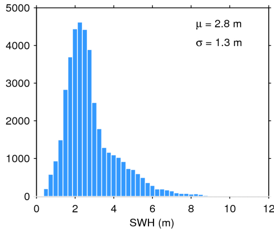
Figure 20. Histogram of science-valid SWH over oceans and lakes for 16/09/2017. The mean ( \mu ) and standard deviation ( \sigma ) are also shown. Note that values larger than 12 m are excluded from the histogram for the sake of readability but not from the computation of \mu and \sigma .
