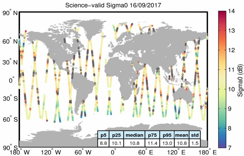
Figure 27. Geographical distribution of science-valid sigma0 data over oceans and lakes for 16/09/2017. The statistical values shown in the table refer to the sigma0 in dB and are calculated over all measurements shown in the figure. Gray circles denote records that have been rejected based on the editing criteria described in Table 4.
