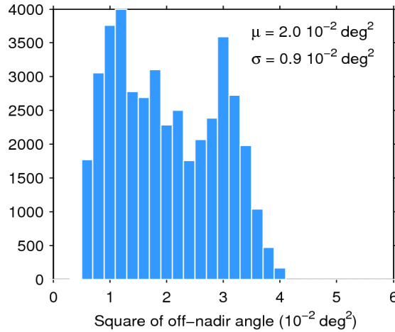
Figure 39. Histogram of flag-valid mispointing over oceans and lakes for 16/09/2017. The mean ( \mu ) and standard deviation ( \sigma ) are also shown. Note that values larger than 6 \cdot 10^{-2} \text{ deg}^2 are excluded from the histogram for the sake of readability but not from the computation of \mu and \sigma .
