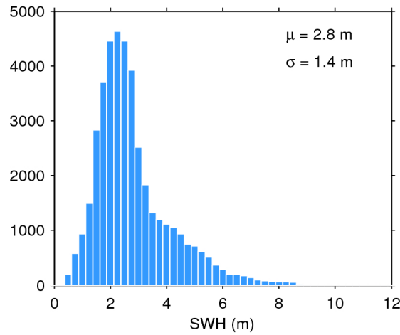
Figure 17. Histogram of flag-valid SWH over oceans and lakes for 16/09/2017. The mean ( \mu ) and standard deviation ( \sigma ) are also shown. Note that values larger than 12 m are excluded from the histogram for the sake of readability but not from the computation of \mu and \sigma .
