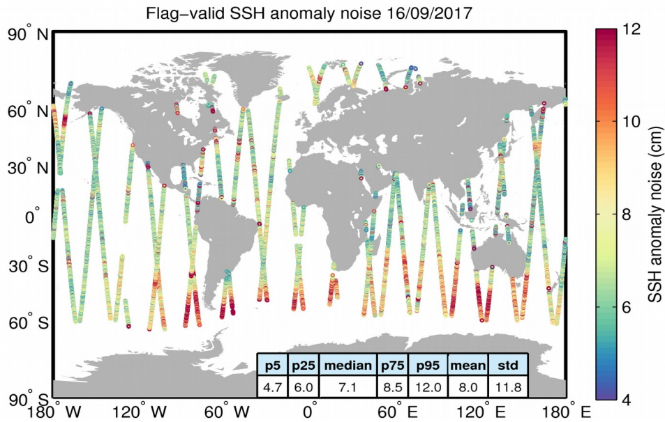
Figure 8. Geographical distribution of flag-valid 20-Hz SSH anomaly measurement noise over oceans and lakes for 16/09/2017. The statistical values shown in the table refer to the SSH anomaly noise and are calculated over all measurements shown in the figure.
