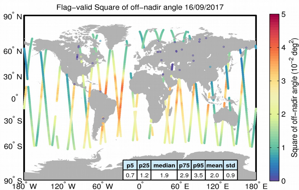
Figure 37. Geographical distribution of flag-valid mispointing data over oceans and lakes for 16/09/2017. The statistical values shown in the table refer to the mispointing in 10^{-2} deg 2 and are calculated over all measurements shown in the figure.
