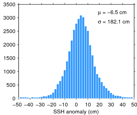
Figure 7. Histogram of flag-valid SSH anomaly over oceans and lakes for 16/09/2017. The mean ( \mu ) and standard deviation ( \sigma ) are also shown. Note that values outside [-50 50] cm are excluded from the histogram for the sake of readability but not from the computation of \mu and \sigma .
