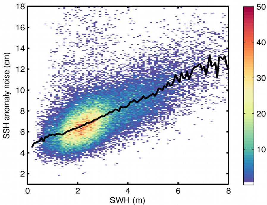
Figure 9. 2D histogram showing flag-valid SSH anomaly noise as a function of SWH for 16/09/2017. The black line denotes the median SSH anomaly noise as a function of SWH.
