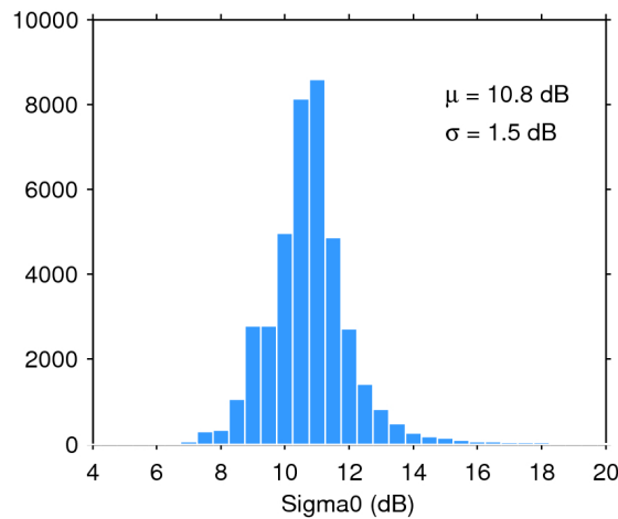
Figure 28. Histogram of science-valid sigma0 over oceans and lakes for 16/09/2017. The mean ( \mu ) and standard deviation ( \sigma ) are also shown. Note that values outside [4 20] dB are excluded from the histogram for the sake of readability but not from the computation of \mu and \sigma .
