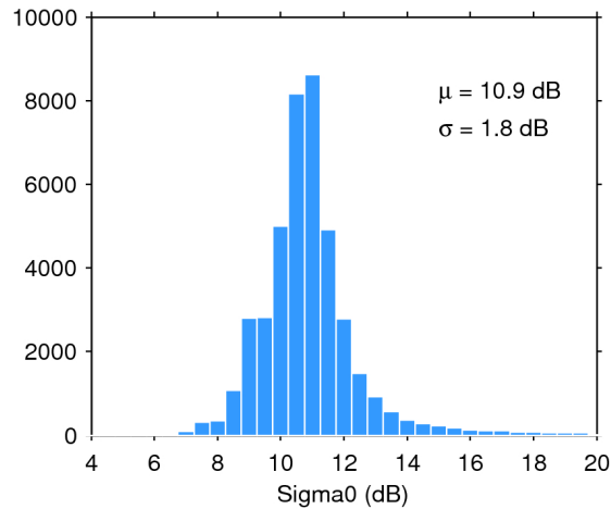
Figure 25. Histogram of flag-valid sigma0 over oceans and lakes for 16/09/2017. The mean ( \mu ) and standard deviation ( \sigma ) are also shown. Note that values outside [4 20] dB are excluded from the histogram for the sake of readability but not from the computation of \mu and \sigma .
