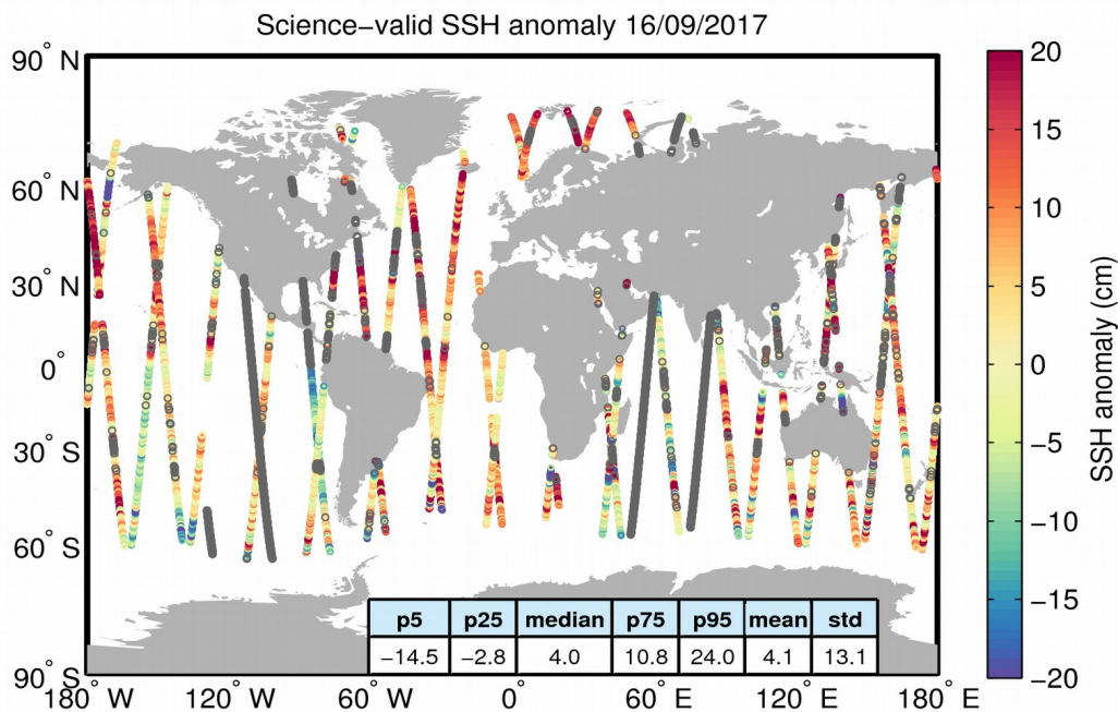
Figure 10. Geographical distribution of science-valid SSH anomaly data over oceans and lakes for 16/09/2017. The statistical values shown in the table refer to the SSH anomaly in cm and are calculated over all measurements shown in the figure. Gray circles denote records that have been rejected based on the editing criteria described in Table 2.
