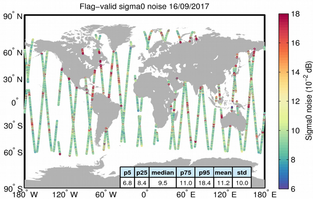
Figure 26. Geographical distribution of flag-valid 20-Hz sigma0 measurement noise over oceans and lakes for 16/09/2017. The statistical values shown in the table refer to the sigma0 noise and are calculated over all measurements shown in the figure.
