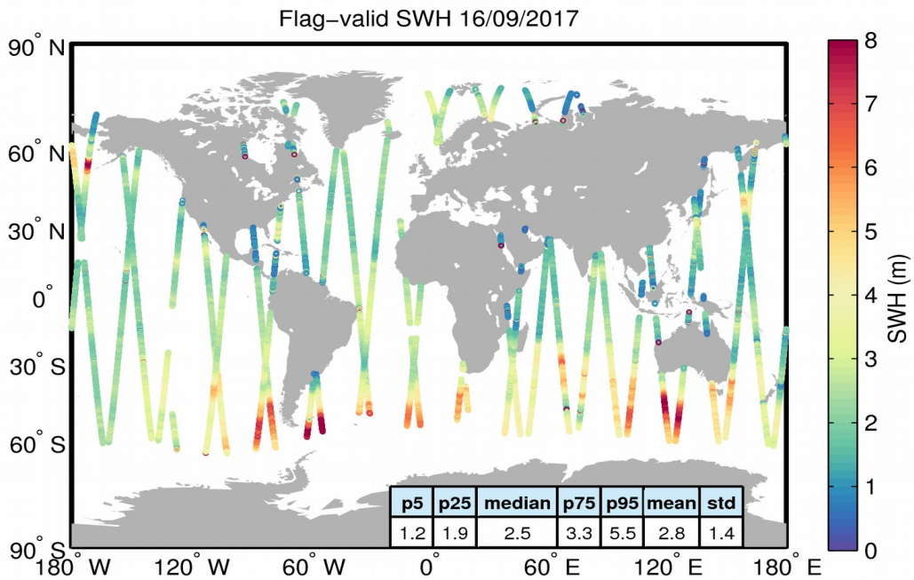
Figure 15. Geographical distribution of flag-valid SWH data over oceans and lakes for 16/09/2017. The statistical values shown in the table refer to the SWH in m and are calculated over all measurements shown in the figure.
