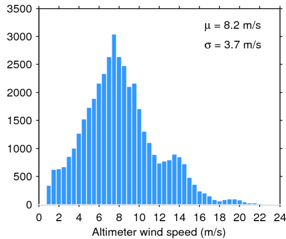
Figure 33. Histogram of flag-valid wind over oceans and lakes for 16/09/2017. The mean ( \mu ) and standard deviation ( \sigma ) are also shown. Note that values larger than 24 m/s are excluded from the histogram for the sake of readability but not from the computation of \mu and \sigma .
