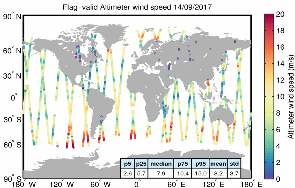
Figure 31. Geographical distribution of flag-valid wind data over oceans and lakes for 14/09/2017. The statistical values shown in the table refer to the wind in m/s and are calculated over all measurements shown in the figure.
