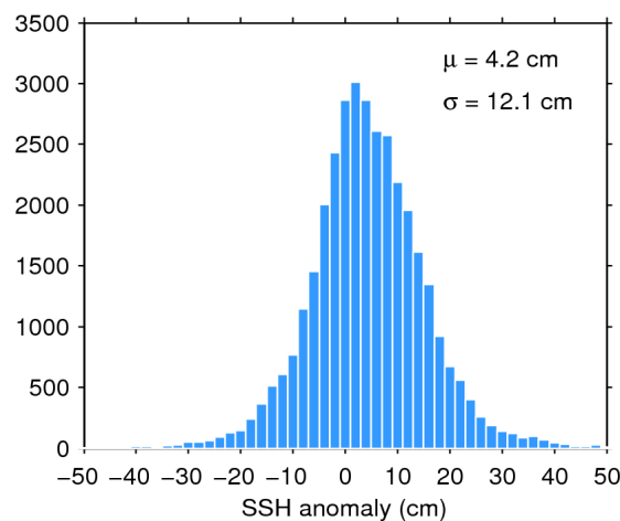
Figure 11. Histogram of science-valid SSH anomaly over oceans and lakes for 14/09/2017. The mean ( \mu ) and standard deviation ( \sigma ) are also shown. Note that values outside [-50 50] cm are excluded from the histogram for the sake of readability but not from the computation of \mu and \sigma .
