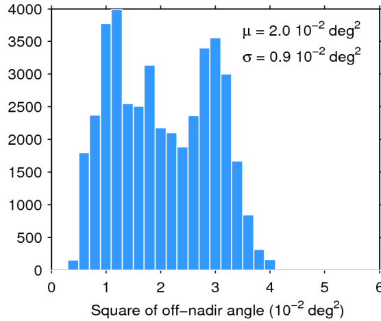
Figure 39. Histogram of flag-valid mispointing over oceans and lakes for 14/09/2017. The mean ( \mu ) and standard deviation ( \sigma ) are also shown. Note that values larger than 6 \cdot 10^{-2} \text{ deg}^2 are excluded from the histogram for the sake of readability but not from the computation of \mu and \sigma .
