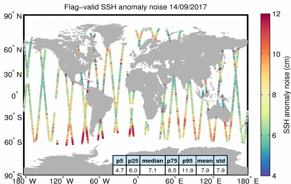
Figure 8. Geographical distribution of flag-valid 20-Hz SSH anomaly measurement noise over oceans and lakes for 14/09/2017. The statistical values shown in the table refer to the SSH anomaly noise and are calculated over all measurements shown in the figure.
