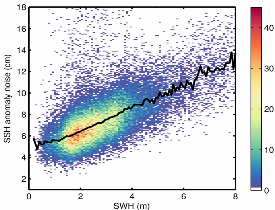
Figure 9. 2D histogram showing flag-valid SSH anomaly noise as a function of SWH for 14/09/2017. The black line denotes the median SSH anomaly noise as a function of SWH.
