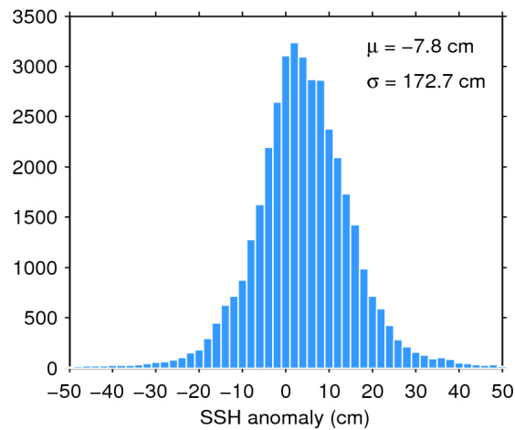
Figure 7. Histogram of flag-valid SSH anomaly over oceans and lakes for 14/09/2017. The mean ( \mu ) and standard deviation ( \sigma ) are also shown. Note that values outside [-50 50] cm are excluded from the histogram for the sake of readability but not from the computation of \mu and \sigma .
