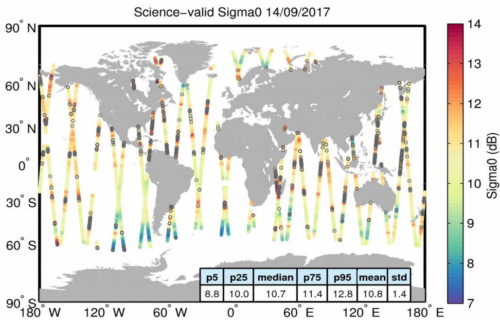
Figure 27. Geographical distribution of science-valid sigma0 data over oceans and lakes for 14/09/2017. The statistical values shown in the table refer to the sigma0 in dB and are calculated over all measurements shown in the figure. Gray circles denote records that have been rejected based on the editing criteria described in Table 4.
