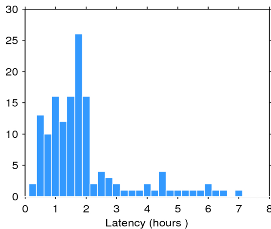
Figure 2. Histogram of the data latency for 14/09/2017. The y-axis denotes the number of files that are made available with a delay of x-hours with respect to the mean time of the records stored in the file.
