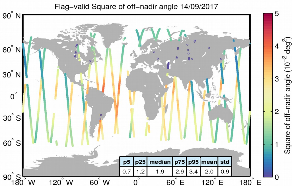
Figure 37. Geographical distribution of flag-valid mispointing data over oceans and lakes for 14/09/2017. The statistical values shown in the table refer to the mispointing in 10^{-2} deg 2 and are calculated over all measurements shown in the figure.
