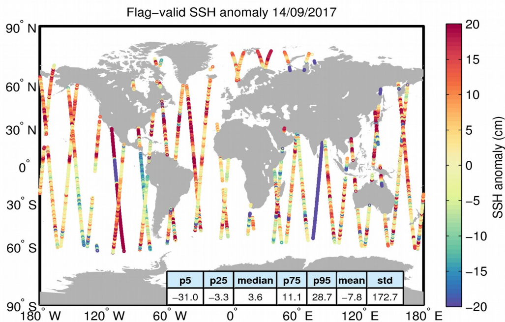
Figure 5. Geographical distribution of flag-valid 1-Hz SSH anomaly data over oceans and lakes for 14/09/2017. The statistical values shown in the table refer to the SSH anomaly in cm and are calculated over all measurements shown in the figure.
