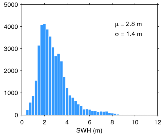
Figure 17. Histogram of flag-valid SWH over oceans and lakes for 14/09/2017. The mean ( \mu ) and standard deviation ( \sigma ) are also shown. Note that values larger than 12 m are excluded from the histogram for the sake of readability but not from the computation of \mu and \sigma .
