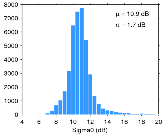
Figure 25. Histogram of flag-valid sigma0 over oceans and lakes for 14/09/2017. The mean ( \mu ) and standard deviation ( \sigma ) are also shown. Note that values outside [4 20] dB are excluded from the histogram for the sake of readability but not from the computation of \mu and \sigma .
