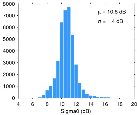
Figure 28. Histogram of science-valid sigma0 over oceans and lakes for 14/09/2017. The mean ( \mu ) and standard deviation ( \sigma ) are also shown. Note that values outside [4 20] dB are excluded from the histogram for the sake of readability but not from the computation of \mu and \sigma .
