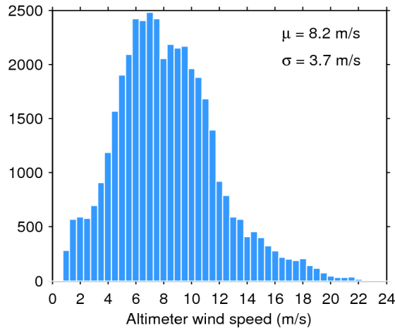
Figure 33. Histogram of flag-valid wind over oceans and lakes for 14/09/2017. The mean ( \mu ) and standard deviation ( \sigma ) are also shown. Note that values larger than 24 m/s are excluded from the histogram for the sake of readability but not from the computation of \mu and \sigma .
