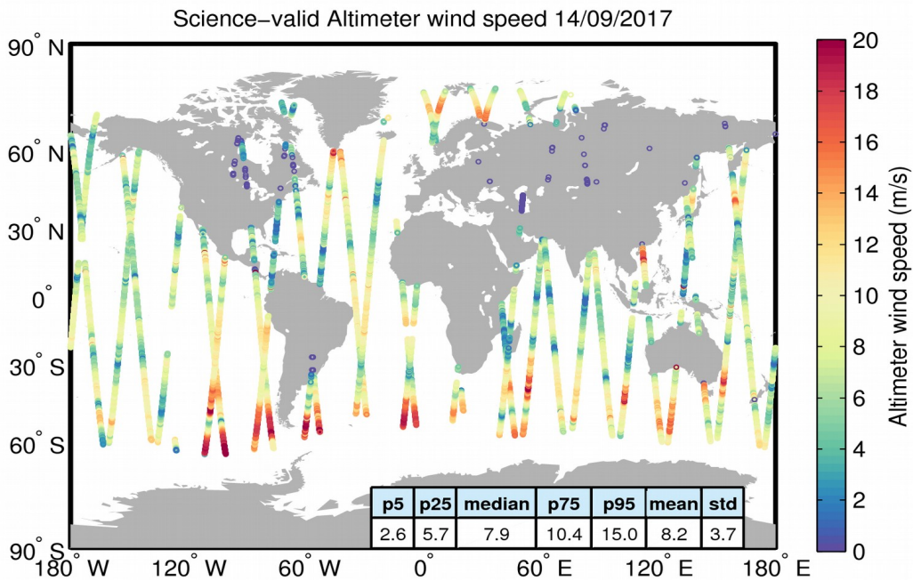
Figure 34. Geographical distribution of science-valid wind data over oceans and lakes for 14/09/2017. The statistical values shown in the table refer to the wind in m/s and are calculated over all measurements shown in the figure. Gray circles denote records that have been rejected based on the editing criteria described in Table 5.
