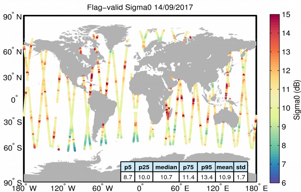
Figure 23. Geographical distribution of flag-valid sigma0 data over oceans and lakes for 14/09/2017. The statistical values shown in the table refer to the sigma0 in dB and are calculated over all measurements shown in the figure.
