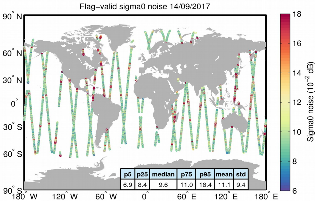
Figure 26. Geographical distribution of flag-valid 20-Hz sigma0 measurement noise over oceans and lakes for 14/09/2017. The statistical values shown in the table refer to the sigma0 noise and are calculated over all measurements shown in the figure.
