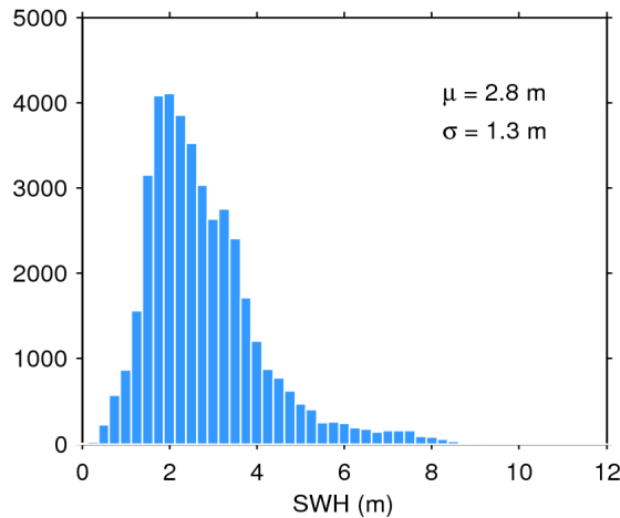
Figure 20. Histogram of science-valid SWH over oceans and lakes for 14/09/2017. The mean ( \mu ) and standard deviation ( \sigma ) are also shown. Note that values larger than 12 m are excluded from the histogram for the sake of readability but not from the computation of \mu and \sigma .
