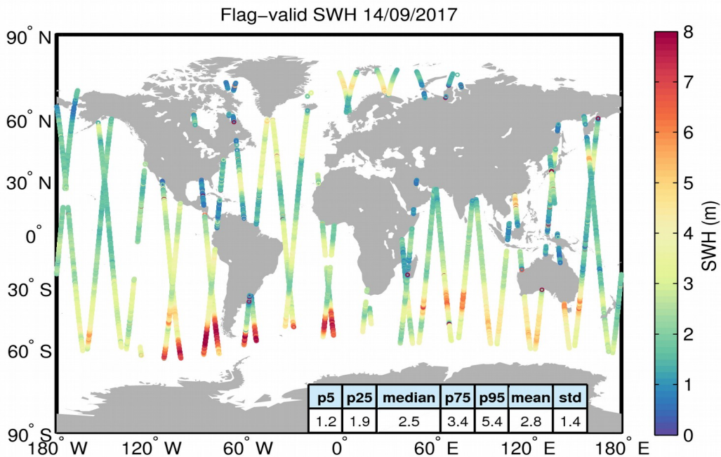
Figure 15. Geographical distribution of flag-valid SWH data over oceans and lakes for 14/09/2017. The statistical values shown in the table refer to the SWH in m and are calculated over all measurements shown in the figure.
