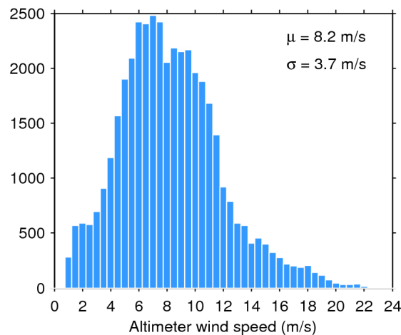
Figure 35. Histogram of science-valid wind over oceans and lakes for 14/09/2017. The mean ( \mu ) and standard deviation ( \sigma ) are also shown. Note that values larger than 24 m/s are excluded from the histogram for the sake of readability but not from the computation of \mu and \sigma .
