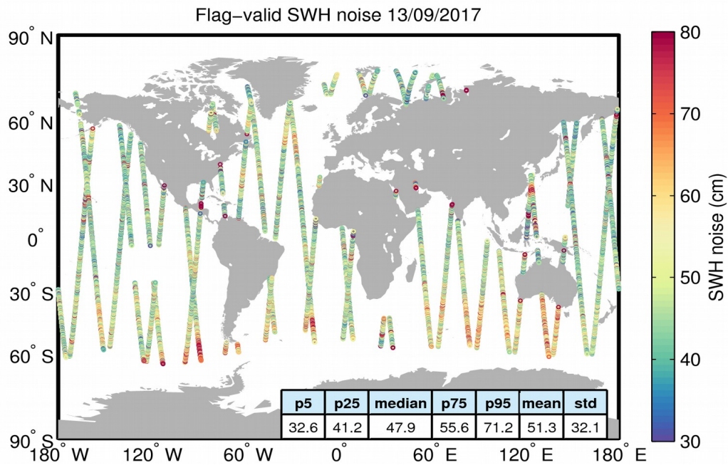
Figure 18. Geographical distribution of flag-valid 20-Hz SWH measurement noise over oceans and lakes for 13/09/2017. The statistical values shown in the table refer to the SWH noise and are calculated over all measurements shown in the figure.
