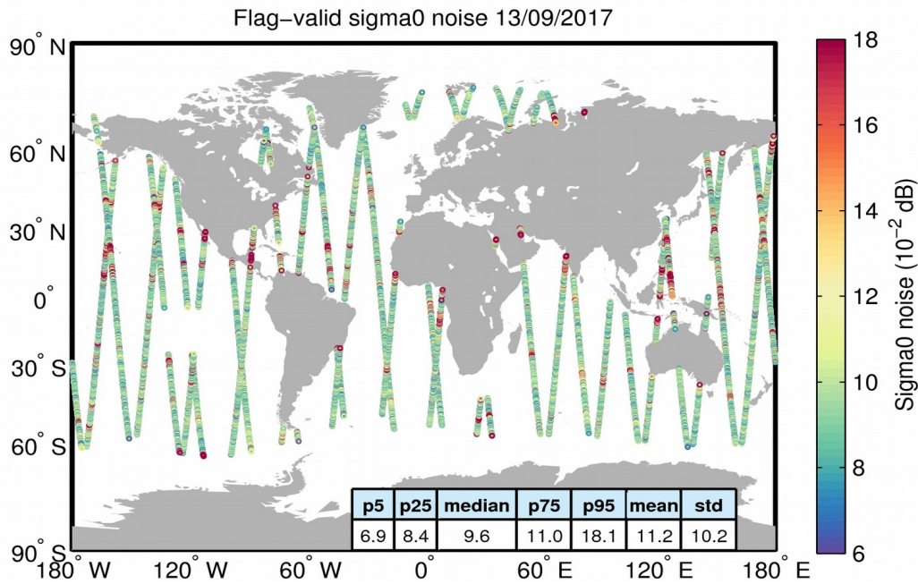
Figure 26. Geographical distribution of flag-valid 20-Hz sigma0 measurement noise over oceans and lakes for 13/09/2017. The statistical values shown in the table refer to the sigma0 noise and are calculated over all measurements shown in the figure.
