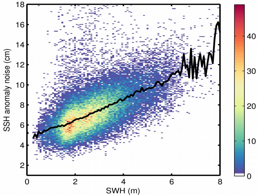
Figure 9. 2D histogram showing flag-valid SSH anomaly noise as a function of SWH for 13/09/2017. The black line denotes the median SSH anomaly noise as a function of SWH.
