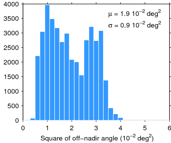
Figure 39. Histogram of flag-valid mispointing over oceans and lakes for 13/09/2017. The mean ( \mu ) and standard deviation ( \sigma ) are also shown. Note that values larger than 6 \times 10^{-2} \text{ deg}^2 are excluded from the histogram for the sake of readability but not from the computation of \mu and \sigma .
