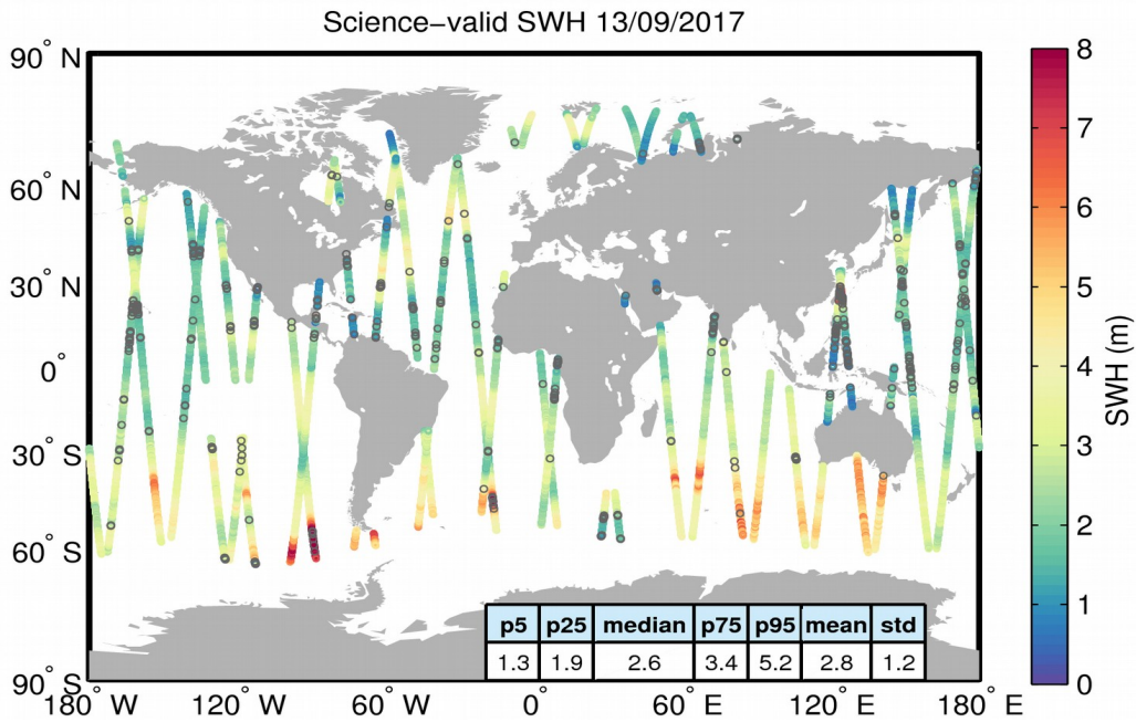
Figure 19. Geographical distribution of science-valid SWH data over oceans and lakes for 13/09/2017. The statistical values shown in the table refer to the SWH in m and are calculated over all measurements shown in the figure. Gray circles denote records that have been rejected based on the editing criteria described in Table 3.
