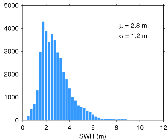
Figure 20. Histogram of science-valid SWH over oceans and lakes for 13/09/2017. The mean ( \mu ) and standard deviation ( \sigma ) are also shown. Note that values larger than 12 m are excluded from the histogram for the sake of readability but not from the computation of \mu and \sigma .
