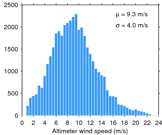
Figure 33. Histogram of flag-valid wind over oceans and lakes for 13/09/2017. The mean ( \mu ) and standard deviation ( \sigma ) are also shown. Note that values larger than 24 m/s are excluded from the histogram for the sake of readability but not from the computation of \mu and \sigma .
