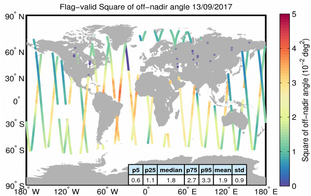
Figure 37. Geographical distribution of flag-valid mispointing data over oceans and lakes for 13/09/2017. The statistical values shown in the table refer to the mispointing in 10^{-2} deg 2 and are calculated over all measurements shown in the figure.
