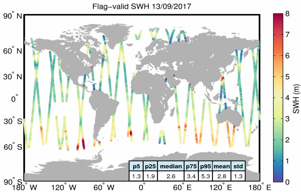
Figure 15. Geographical distribution of flag-valid SWH data over oceans and lakes for 13/09/2017. The statistical values shown in the table refer to the SWH in m and are calculated over all measurements shown in the figure.
