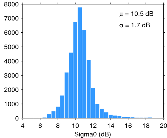
Figure 25. Histogram of flag-valid sigma0 over oceans and lakes for 13/09/2017. The mean ( \mu ) and standard deviation ( \sigma ) are also shown. Note that values outside [4 20] dB are excluded from the histogram for the sake of readability but not from the computation of \mu and \sigma .
