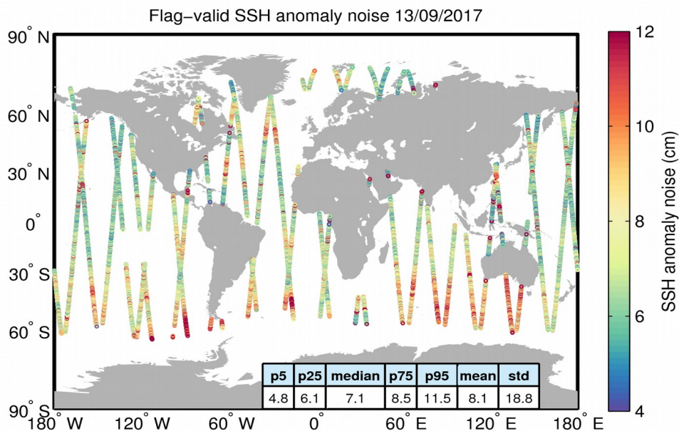
Figure 8. Geographical distribution of flag-valid 20-Hz SSH anomaly measurement noise over oceans and lakes for 13/09/2017. The statistical values shown in the table refer to the SSH anomaly noise and are calculated over all measurements shown in the figure.
