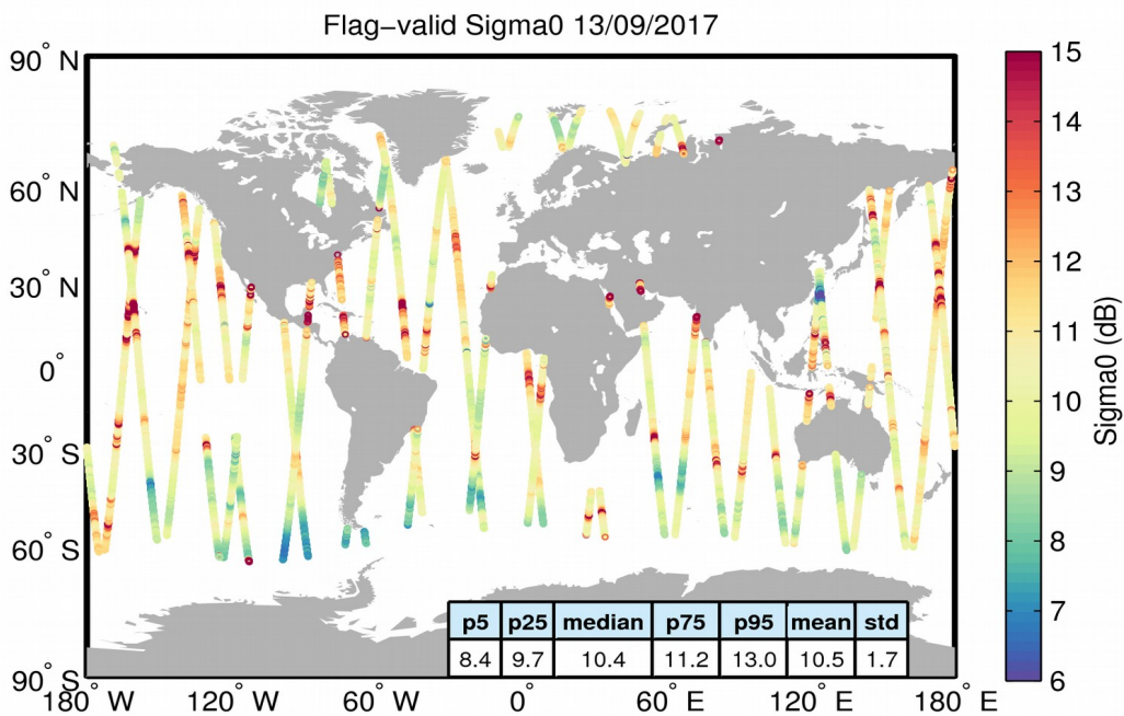
Figure 23. Geographical distribution of flag-valid sigma0 data over oceans and lakes for 13/09/2017. The statistical values shown in the table refer to the sigma0 in dB and are calculated over all measurements shown in the figure.
