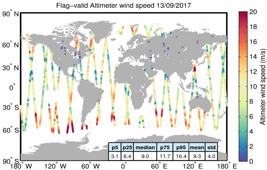
Figure 31. Geographical distribution of flag-valid wind data over oceans and lakes for 13/09/2017. The statistical values shown in the table refer to the wind in m/s and are calculated over all measurements shown in the figure.
