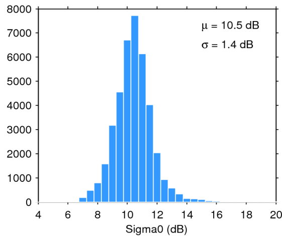
Figure 28. Histogram of science-valid sigma0 over oceans and lakes for 13/09/2017. The mean ( \mu ) and standard deviation ( \sigma ) are also shown. Note that values outside [4 20] dB are excluded from the histogram for the sake of readability but not from the computation of \mu and \sigma .
