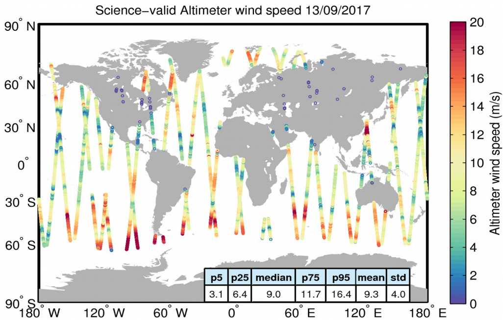
Figure 34. Geographical distribution of science-valid wind data over oceans and lakes for 13/09/2017. The statistical values shown in the table refer to the wind in m/s and are calculated over all measurements shown in the figure. Gray circles denote records that have been rejected based on the editing criteria described in Table 5.
