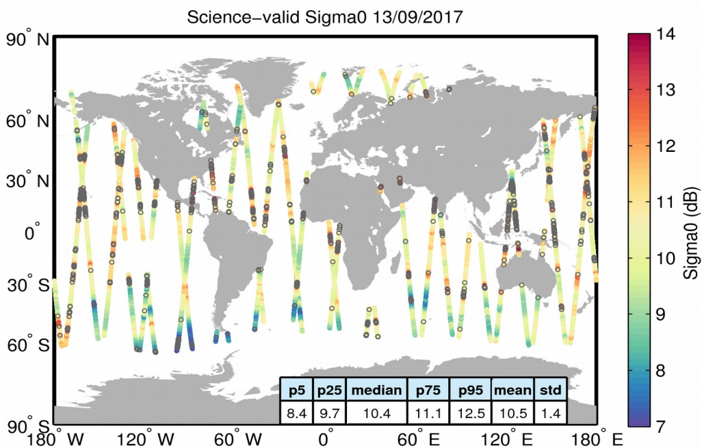
Figure 27. Geographical distribution of science-valid sigma0 data over oceans and lakes for 13/09/2017. The statistical values shown in the table refer to the sigma0 in dB and are calculated over all measurements shown in the figure. Gray circles denote records that have been rejected based on the editing criteria described in Table 4.
