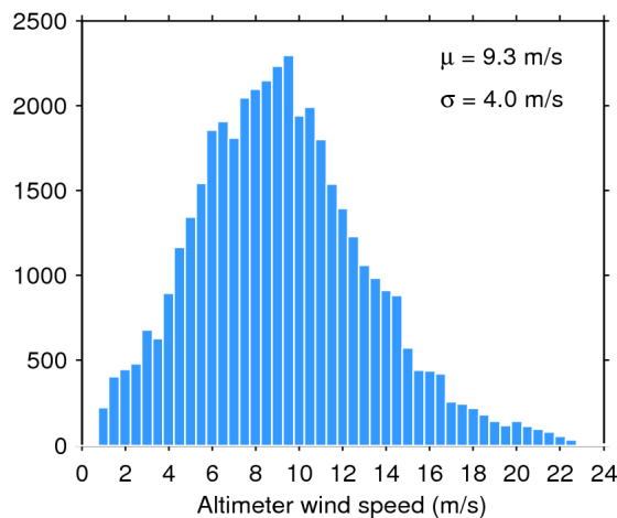
Figure 35. Histogram of science-valid wind over oceans and lakes for 13/09/2017. The mean ( \mu ) and standard deviation ( \sigma ) are also shown. Note that values larger than 24 m/s are excluded from the histogram for the sake of readability but not from the computation of \mu and \sigma .
