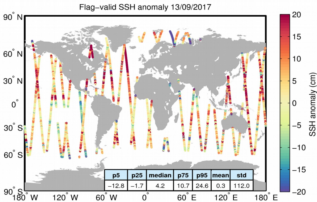
Figure 5. Geographical distribution of flag-valid 1-Hz SSH anomaly data over oceans and lakes for 13/09/2017. The statistical values shown in the table refer to the SSH anomaly in cm and are calculated over all measurements shown in the figure.
