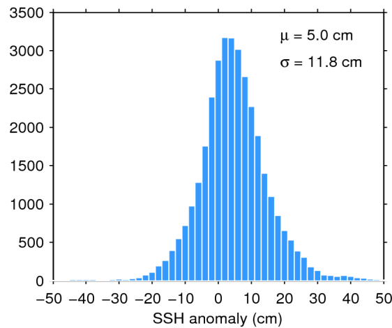
Figure 11. Histogram of science-valid SSH anomaly over oceans and lakes for 13/09/2017. The mean ( \mu ) and standard deviation ( \sigma ) are also shown. Note that values outside [-50 50] cm are excluded from the histogram for the sake of readability but not from the computation of \mu and \sigma .
