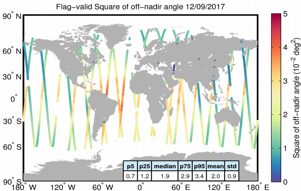
Figure 37. Geographical distribution of flag-valid mispointing data over oceans and lakes for 12/09/2017. The statistical values shown in the table refer to the mispointing in 10^{-2} deg 2 and are calculated over all measurements shown in the figure.
