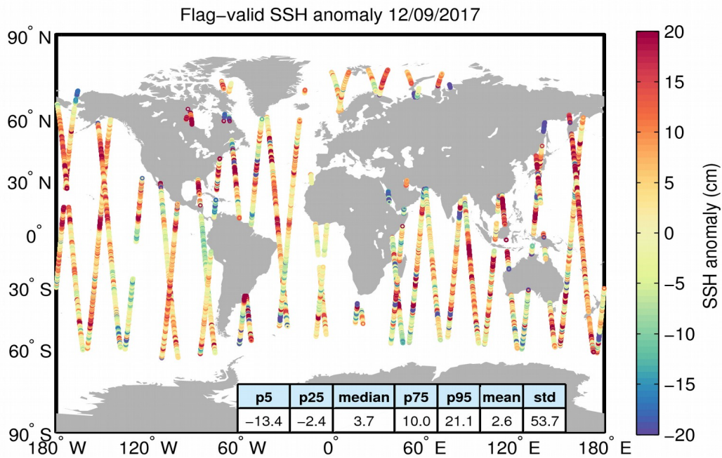
Figure 5. Geographical distribution of flag-valid 1-Hz SSH anomaly data over oceans and lakes for 12/09/2017. The statistical values shown in the table refer to the SSH anomaly in cm and are calculated over all measurements shown in the figure.
