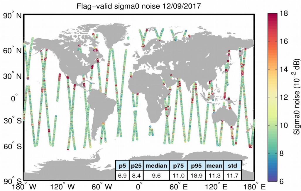
Figure 26. Geographical distribution of flag-valid 20-Hz sigma0 measurement noise over oceans and lakes for 12/09/2017. The statistical values shown in the table refer to the sigma0 noise and are calculated over all measurements shown in the figure.
