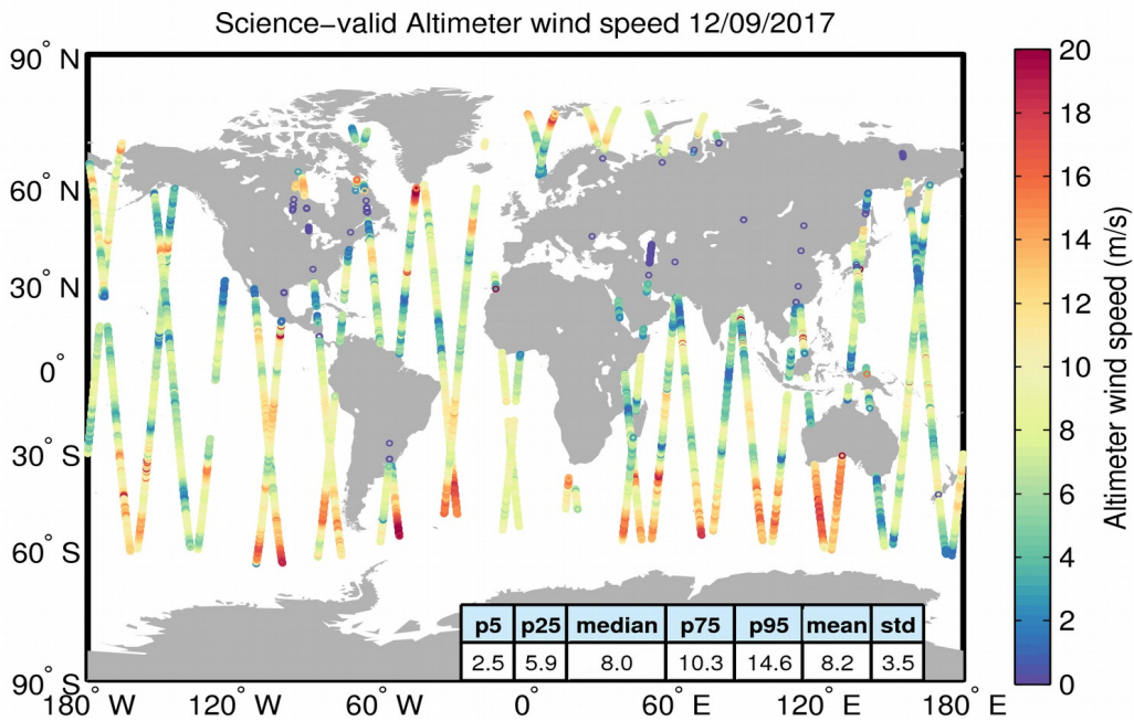
Figure 34. Geographical distribution of science-valid wind data over oceans and lakes for 12/09/2017. The statistical values shown in the table refer to the wind in m/s and are calculated over all measurements shown in the figure. Gray circles denote records that have been rejected based on the editing criteria described in Table 5.
