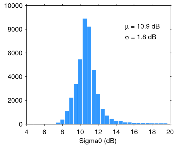
Figure 25. Histogram of flag-valid sigma0 over oceans and lakes for 12/09/2017. The mean ( \mu ) and standard deviation ( \sigma ) are also shown. Note that values outside [4 20] dB are excluded from the histogram for the sake of readability but not from the computation of \mu and \sigma .
