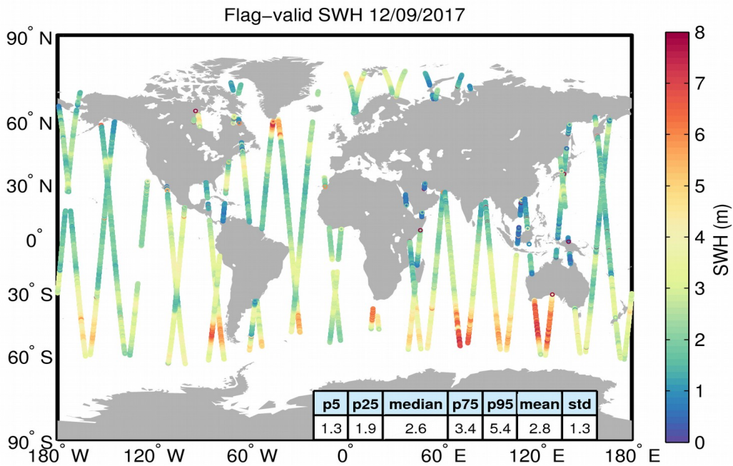
Figure 15. Geographical distribution of flag-valid SWH data over oceans and lakes for 12/09/2017. The statistical values shown in the table refer to the SWH in m and are calculated over all measurements shown in the figure.
