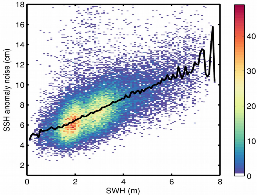
Figure 9. 2D histogram showing flag-valid SSH anomaly noise as a function of SWH for 12/09/2017. The black line denotes the median SSH anomaly noise as a function of SWH.
