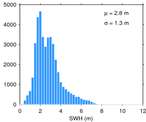
Figure 17. Histogram of flag-valid SWH over oceans and lakes for 12/09/2017. The mean ( \mu ) and standard deviation ( \sigma ) are also shown. Note that values larger than 12 m are excluded from the histogram for the sake of readability but not from the computation of \mu and \sigma .
