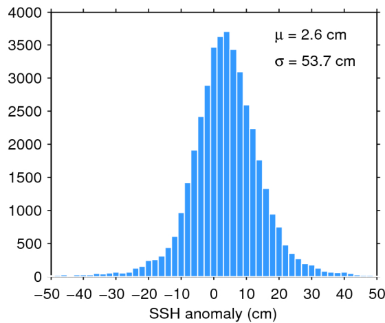
Figure 7. Histogram of flag-valid SSH anomaly over oceans and lakes for 12/09/2017. The mean ( \mu ) and standard deviation ( \sigma ) are also shown. Note that values outside [-50 50] cm are excluded from the histogram for the sake of readability but not from the computation of \mu and \sigma .
