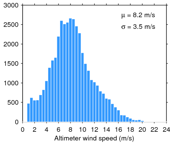
Figure 33. Histogram of flag-valid wind over oceans and lakes for 12/09/2017. The mean ( \mu ) and standard deviation ( \sigma ) are also shown. Note that values larger than 24 m/s are excluded from the histogram for the sake of readability but not from the computation of \mu and \sigma .
