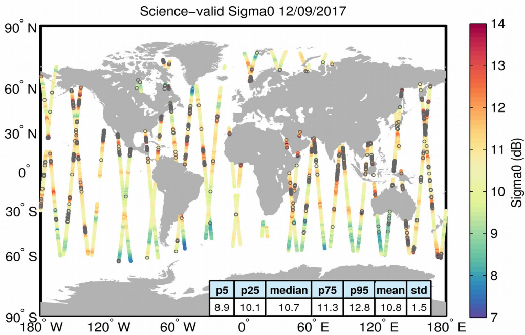
Figure 27. Geographical distribution of science-valid sigma0 data over oceans and lakes for 12/09/2017. The statistical values shown in the table refer to the sigma0 in dB and are calculated over all measurements shown in the figure. Gray circles denote records that have been rejected based on the editing criteria described in Table 4.
