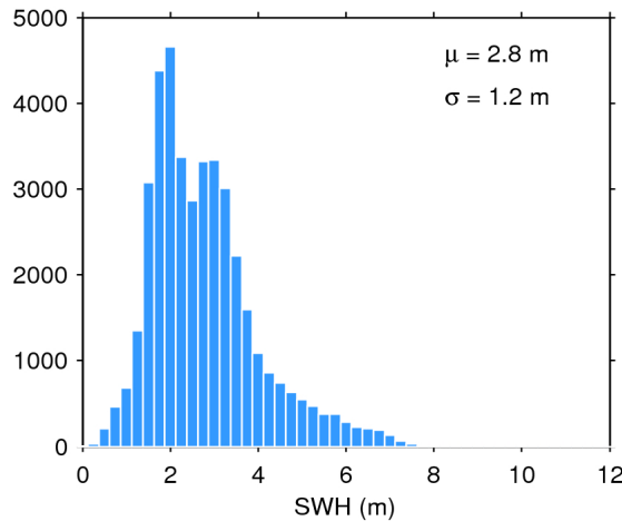
Figure 20. Histogram of science-valid SWH over oceans and lakes for 12/09/2017. The mean ( \mu ) and standard deviation ( \sigma ) are also shown. Note that values larger than 12 m are excluded from the histogram for the sake of readability but not from the computation of \mu and \sigma .
