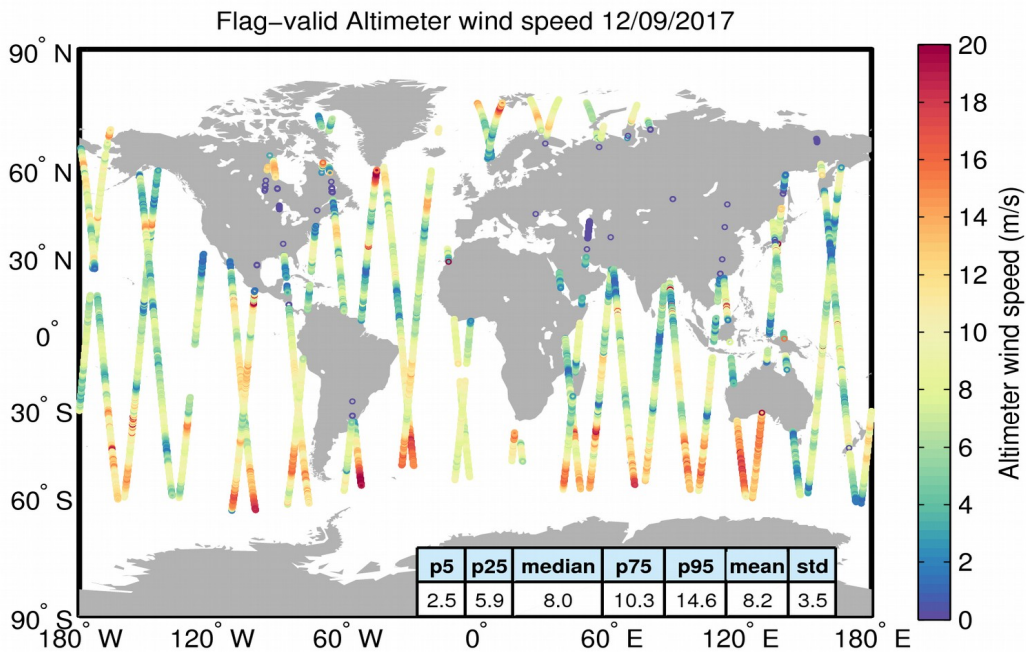
Figure 31. Geographical distribution of flag-valid wind data over oceans and lakes for 12/09/2017. The statistical values shown in the table refer to the wind in m/s and are calculated over all measurements shown in the figure.
