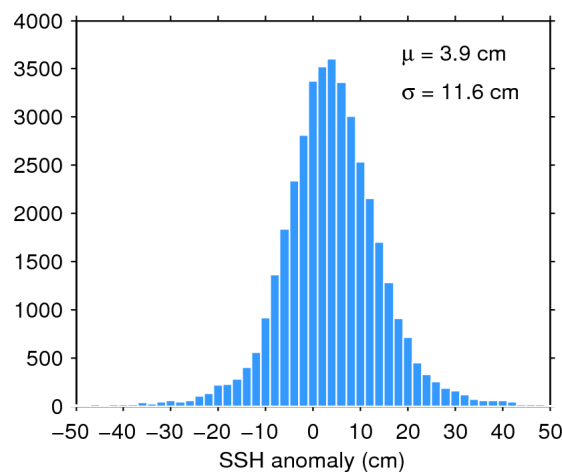
Figure 11. Histogram of science-valid SSH anomaly over oceans and lakes for 12/09/2017. The mean ( \mu ) and standard deviation ( \sigma ) are also shown. Note that values outside [-50 50] cm are excluded from the histogram for the sake of readability but not from the computation of \mu and \sigma .
