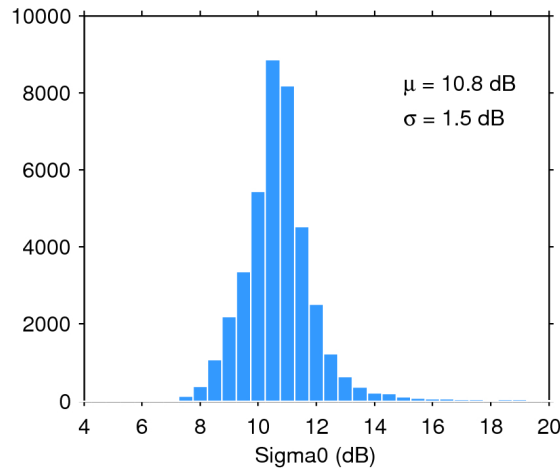
Figure 28. Histogram of science-valid sigma0 over oceans and lakes for 12/09/2017. The mean ( \mu ) and standard deviation ( \sigma ) are also shown. Note that values outside [4 20] dB are excluded from the histogram for the sake of readability but not from the computation of \mu and \sigma .
