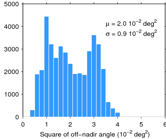
Figure 39. Histogram of flag-valid mispointing over oceans and lakes for 12/09/2017. The mean ( \mu ) and standard deviation ( \sigma ) are also shown. Note that values larger than 6 \cdot 10^{-2} \text{ deg}^2 are excluded from the histogram for the sake of readability but not from the computation of \mu and \sigma .
