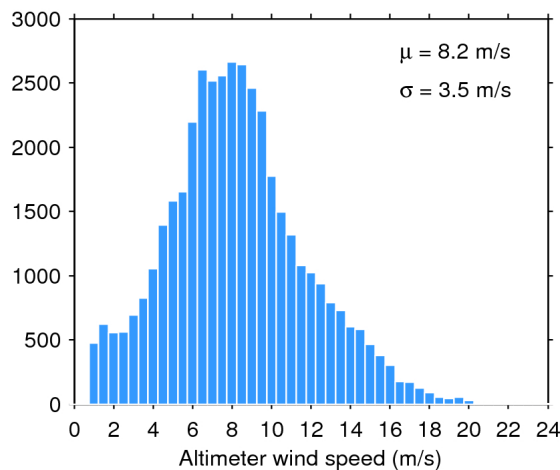
Figure 35. Histogram of science-valid wind over oceans and lakes for 12/09/2017. The mean ( \mu ) and standard deviation ( \sigma ) are also shown. Note that values larger than 24 m/s are excluded from the histogram for the sake of readability but not from the computation of \mu and \sigma .
