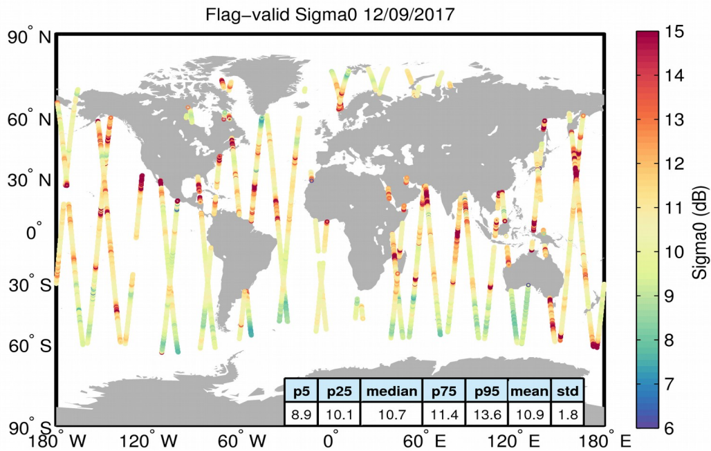
Figure 23. Geographical distribution of flag-valid sigma0 data over oceans and lakes for 12/09/2017. The statistical values shown in the table refer to the sigma0 in dB and are calculated over all measurements shown in the figure.
