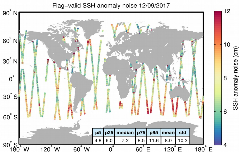
Figure 8. Geographical distribution of flag-valid 20-Hz SSH anomaly measurement noise over oceans and lakes for 12/09/2017. The statistical values shown in the table refer to the SSH anomaly noise and are calculated over all measurements shown in the figure.
