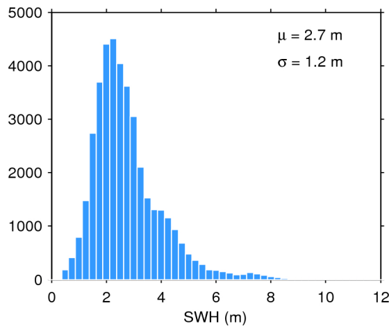
Figure 20. Histogram of science-valid SWH over oceans and lakes for 11/09/2017. The mean ( \mu ) and standard deviation ( \sigma ) are also shown. Note that values larger than 12 m are excluded from the histogram for the sake of readability but not from the computation of \mu and \sigma .
