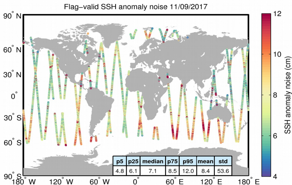
Figure 8. Geographical distribution of flag-valid 20-Hz SSH anomaly measurement noise over oceans and lakes for 11/09/2017. The statistical values shown in the table refer to the SSH anomaly noise and are calculated over all measurements shown in the figure.
