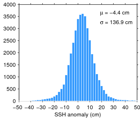
Figure 7. Histogram of flag-valid SSH anomaly over oceans and lakes for 11/09/2017. The mean ( \mu ) and standard deviation ( \sigma ) are also shown. Note that values outside [-50\ 50] cm are excluded from the histogram for the sake of readability but not from the computation of \mu and \sigma .
