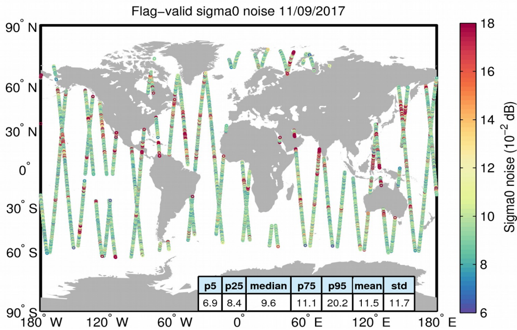
Figure 26. Geographical distribution of flag-valid 20-Hz sigma0 measurement noise over oceans and lakes for 11/09/2017. The statistical values shown in the table refer to the sigma0 noise and are calculated over all measurements shown in the figure.
