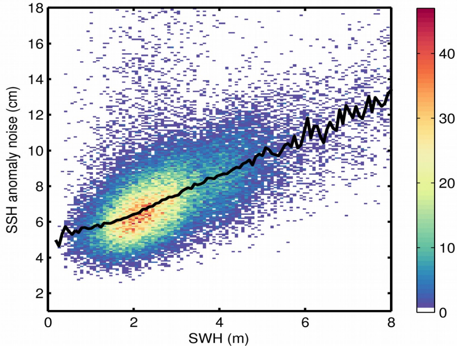
Figure 9. 2D histogram showing flag-valid SSH anomaly noise as a function of SWH for 11/09/2017. The black line denotes the median SSH anomaly noise as a function of SWH.
