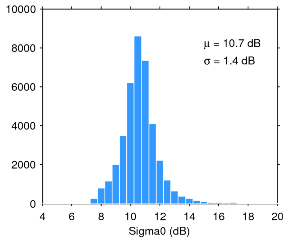
Figure 28. Histogram of science-valid sigma0 over oceans and lakes for 11/09/2017. The mean ( \mu ) and standard deviation ( \sigma ) are also shown. Note that values outside [4 20] dB are excluded from the histogram for the sake of readability but not from the computation of \mu and \sigma .
