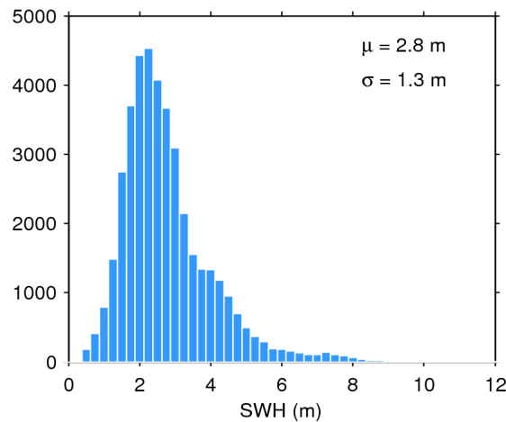
Figure 17. Histogram of flag-valid SWH over oceans and lakes for 11/09/2017. The mean ( \mu ) and standard deviation ( \sigma ) are also shown. Note that values larger than 12 m are excluded from the histogram for the sake of readability but not from the computation of \mu and \sigma .
