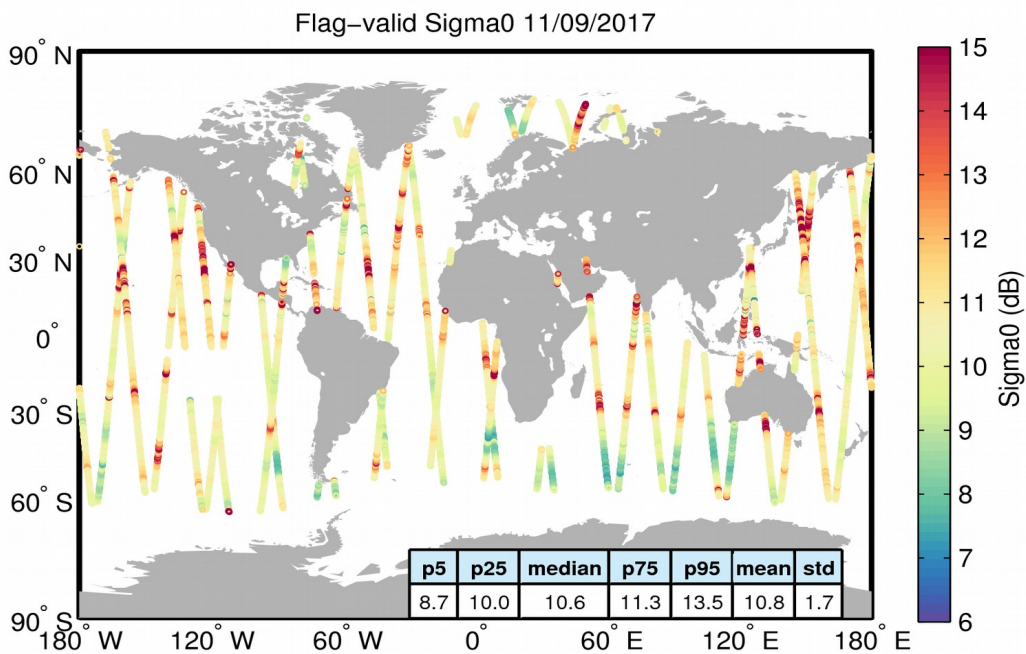
Figure 23. Geographical distribution of flag-valid sigma0 data over oceans and lakes for 11/09/2017. The statistical values shown in the table refer to the sigma0 in dB and are calculated over all measurements shown in the figure.
