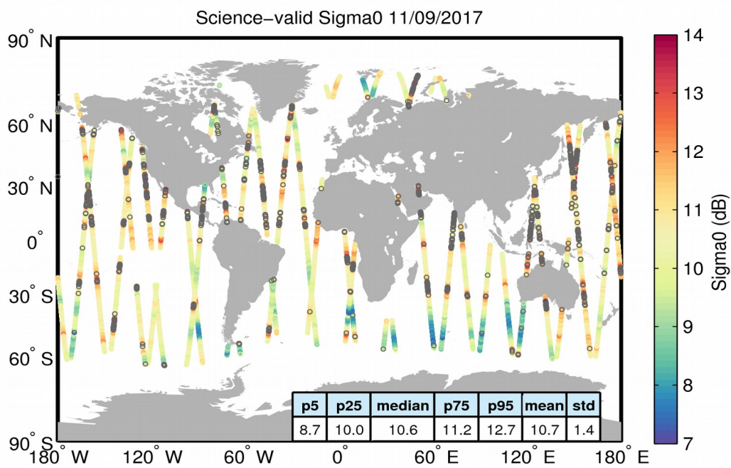
Figure 27. Geographical distribution of science-valid sigma0 data over oceans and lakes for 11/09/2017. The statistical values shown in the table refer to the sigma0 in dB and are calculated over all measurements shown in the figure. Gray circles denote records that have been rejected based on the editing criteria described in Table 4.
