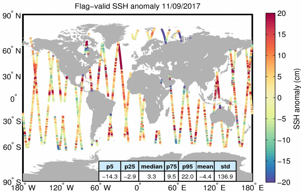
Figure 5. Geographical distribution of flag-valid 1-Hz SSH anomaly data over oceans and lakes for 11/09/2017. The statistical values shown in the table refer to the SSH anomaly in cm and are calculated over all measurements shown in the figure.
