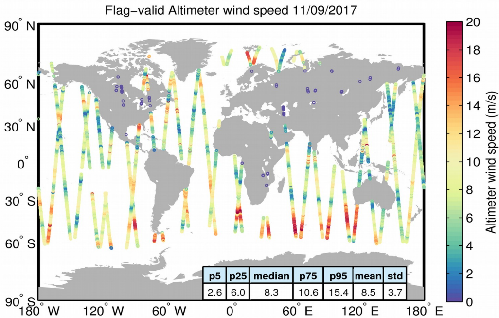
Figure 31. Geographical distribution of flag-valid wind data over oceans and lakes for 11/09/2017. The statistical values shown in the table refer to the wind in m/s and are calculated over all measurements shown in the figure.
