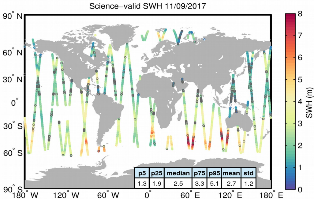
Figure 19. Geographical distribution of science-valid SWH data over oceans and lakes for 11/09/2017. The statistical values shown in the table refer to the SWH in m and are calculated over all measurements shown in the figure. Gray circles denote records that have been rejected based on the editing criteria described in Table 3.
