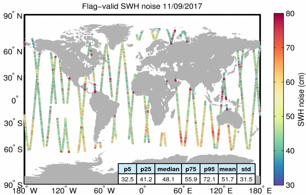
Figure 18. Geographical distribution of flag-valid 20-Hz SWH measurement noise over oceans and lakes for 11/09/2017. The statistical values shown in the table refer to the SWH noise and are calculated over all measurements shown in the figure.
