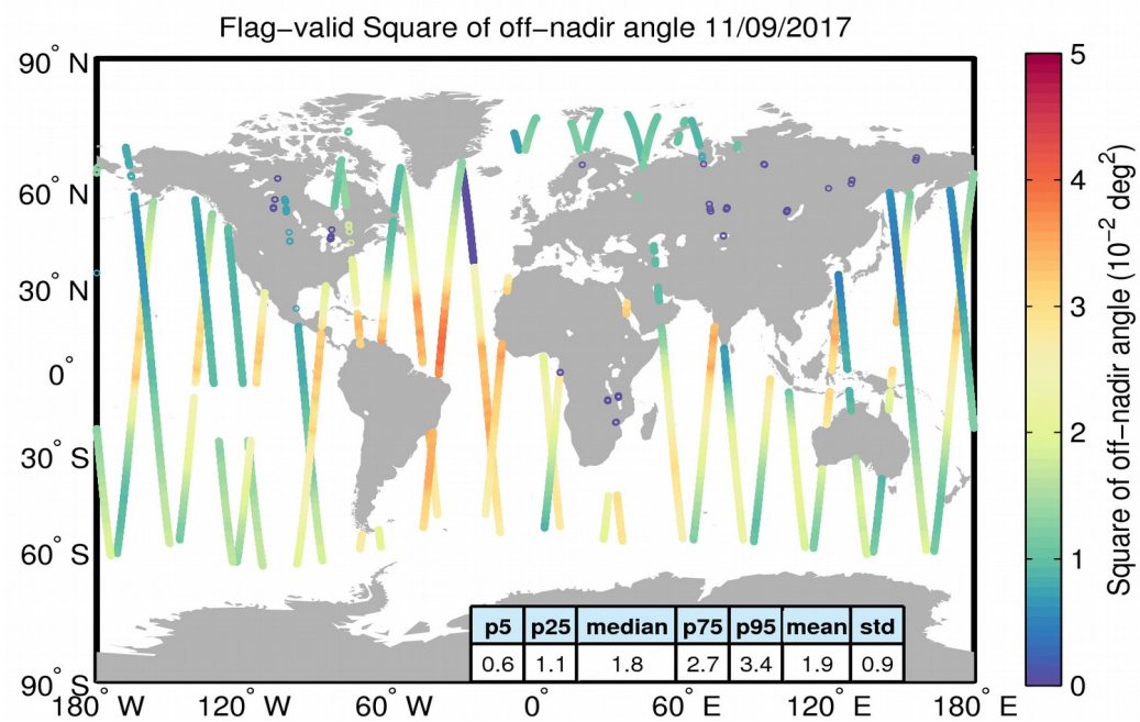
Figure 37. Geographical distribution of flag-valid mispointing data over oceans and lakes for 11/09/2017. The statistical values shown in the table refer to the mispointing in 10^{-2} deg 2 and are calculated over all measurements shown in the figure.
