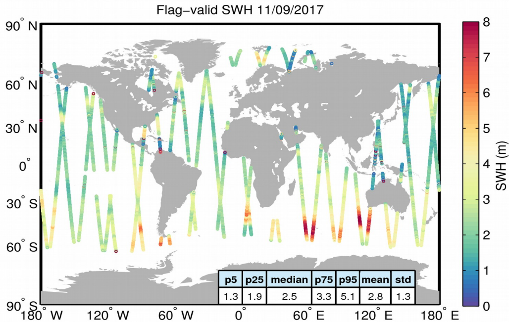
Figure 15. Geographical distribution of flag-valid SWH data over oceans and lakes for 11/09/2017. The statistical values shown in the table refer to the SWH in m and are calculated over all measurements shown in the figure.
