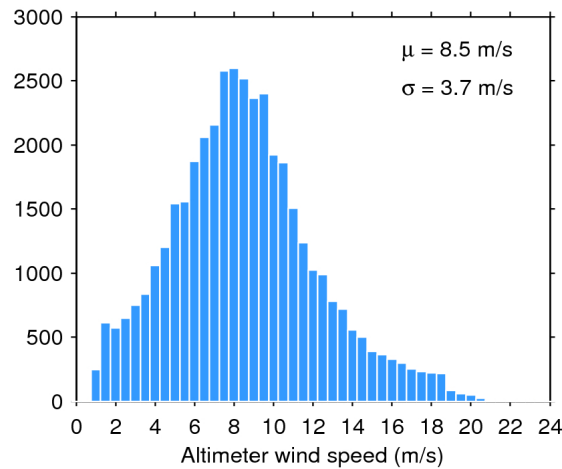
Figure 33. Histogram of flag-valid wind over oceans and lakes for 11/09/2017. The mean ( \mu ) and standard deviation ( \sigma ) are also shown. Note that values larger than 24 m/s are excluded from the histogram for the sake of readability but not from the computation of \mu and \sigma .
