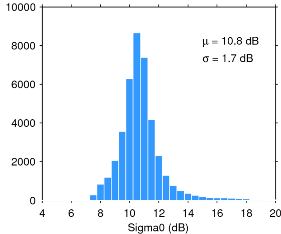
Figure 25. Histogram of flag-valid sigma0 over oceans and lakes for 11/09/2017. The mean ( \mu ) and standard deviation ( \sigma ) are also shown. Note that values outside [4 20] dB are excluded from the histogram for the sake of readability but not from the computation of \mu and \sigma .
