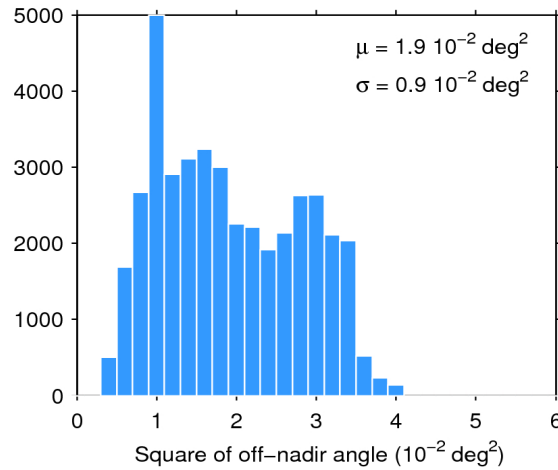
Figure 39. Histogram of flag-valid mispointing over oceans and lakes for 11/09/2017. The mean ( \mu ) and standard deviation ( \sigma ) are also shown. Note that values larger than 6 \cdot 10^{-2} \text{ deg}^2 are excluded from the histogram for the sake of readability but not from the computation of \mu and \sigma .
