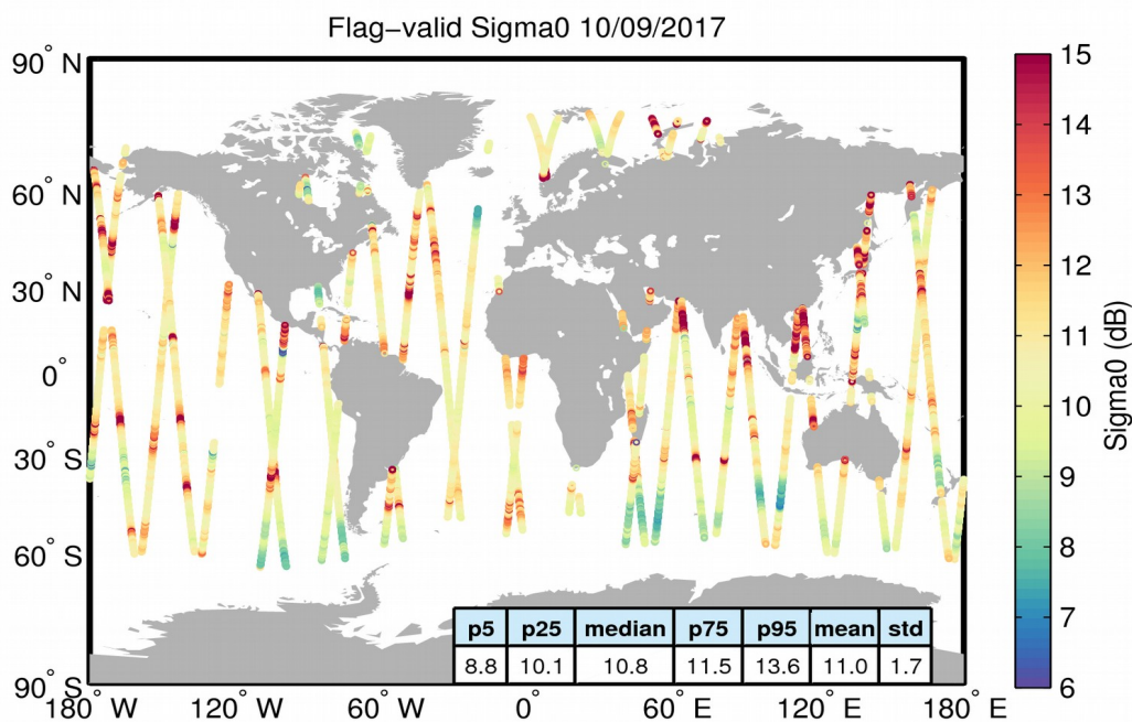
Figure 23. Geographical distribution of flag-valid sigma0 data over oceans and lakes for 10/09/2017. The statistical values shown in the table refer to the sigma0 in dB and are calculated over all measurements shown in the figure.
