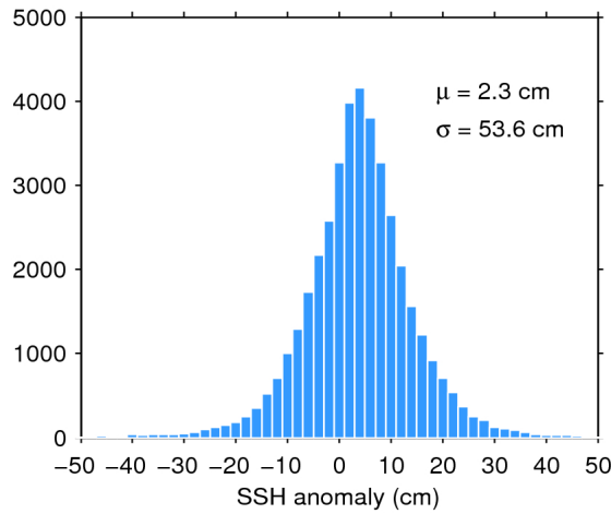
Figure 7. Histogram of flag-valid SSH anomaly over oceans and lakes for 10/09/2017. The mean ( \mu ) and standard deviation ( \sigma ) are also shown. Note that values outside [-50\ 50] cm are excluded from the histogram for the sake of readability but not from the computation of \mu and \sigma .
