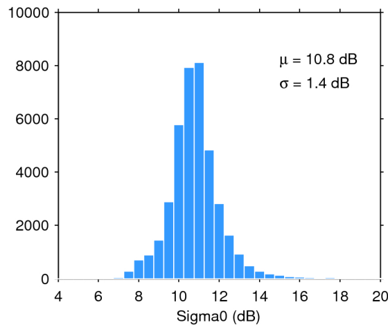
Figure 28. Histogram of science-valid sigma0 over oceans and lakes for 10/09/2017. The mean ( \mu ) and standard deviation ( \sigma ) are also shown. Note that values outside [4 20] dB are excluded from the histogram for the sake of readability but not from the computation of \mu and \sigma .
