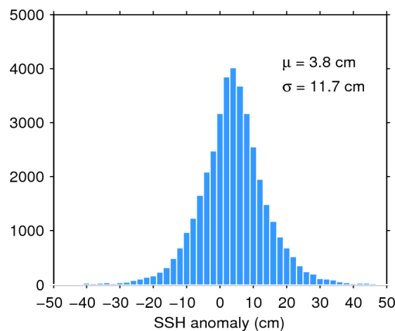
Figure 11. Histogram of science-valid SSH anomaly over oceans and lakes for 10/09/2017. The mean ( \mu ) and standard deviation ( \sigma ) are also shown. Note that values outside [-50 50] cm are excluded from the histogram for the sake of readability but not from the computation of \mu and \sigma .
