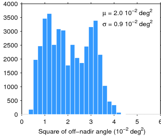
Figure 39. Histogram of flag-valid mispointing over oceans and lakes for 10/09/2017. The mean ( \mu ) and standard deviation ( \sigma ) are also shown. Note that values larger than 6 \cdot 10^{-2} \text{ deg}^2 are excluded from the histogram for the sake of readability but not from the computation of \mu and \sigma .
