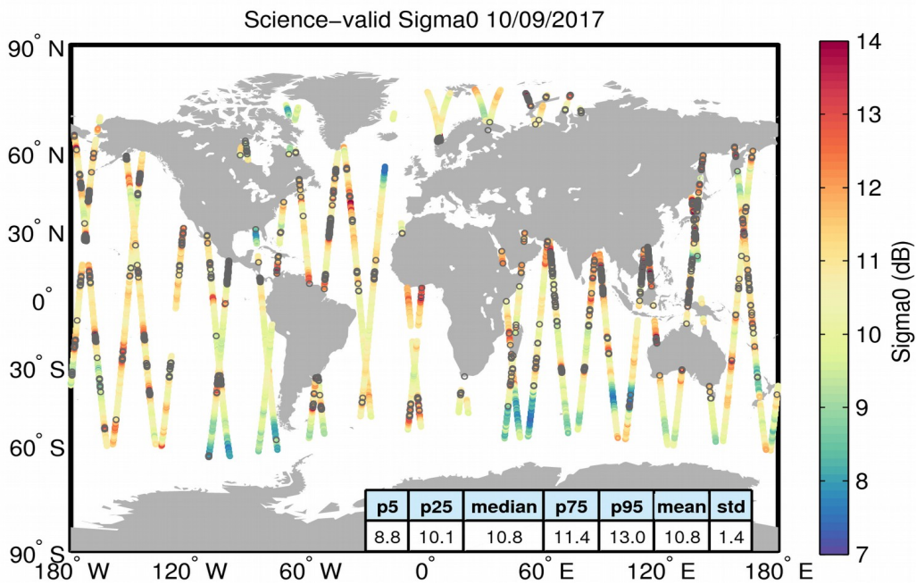
Figure 27. Geographical distribution of science-valid sigma0 data over oceans and lakes for 10/09/2017. The statistical values shown in the table refer to the sigma0 in dB and are calculated over all measurements shown in the figure. Gray circles denote records that have been rejected based on the editing criteria described in Table 4.
