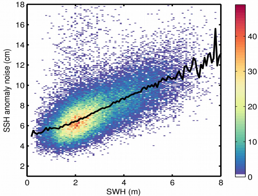
Figure 9. 2D histogram showing flag-valid SSH anomaly noise as a function of SWH for 10/09/2017. The black line denotes the median SSH anomaly noise as a function of SWH.
