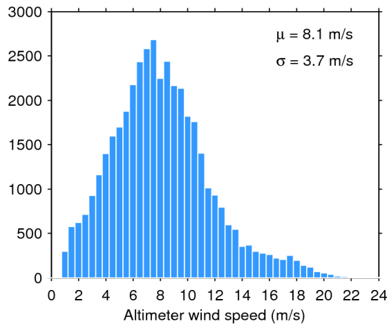
Figure 33. Histogram of flag-valid wind over oceans and lakes for 10/09/2017. The mean ( \mu ) and standard deviation ( \sigma ) are also shown. Note that values larger than 24 m/s are excluded from the histogram for the sake of readability but not from the computation of \mu and \sigma .
