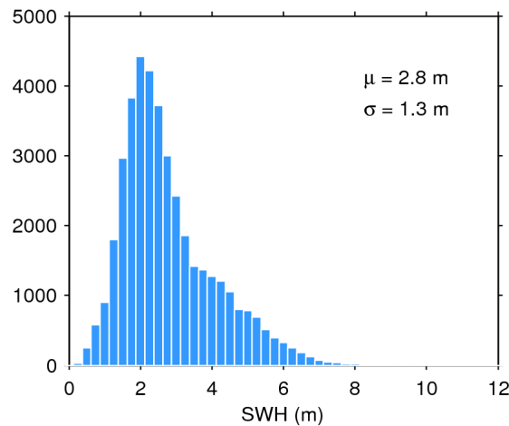
Figure 20. Histogram of science-valid SWH over oceans and lakes for 10/09/2017. The mean ( \mu ) and standard deviation ( \sigma ) are also shown. Note that values larger than 12 m are excluded from the histogram for the sake of readability but not from the computation of \mu and \sigma .
