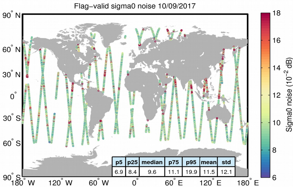
Figure 26. Geographical distribution of flag-valid 20-Hz sigma0 measurement noise over oceans and lakes for 10/09/2017. The statistical values shown in the table refer to the sigma0 noise and are calculated over all measurements shown in the figure.
