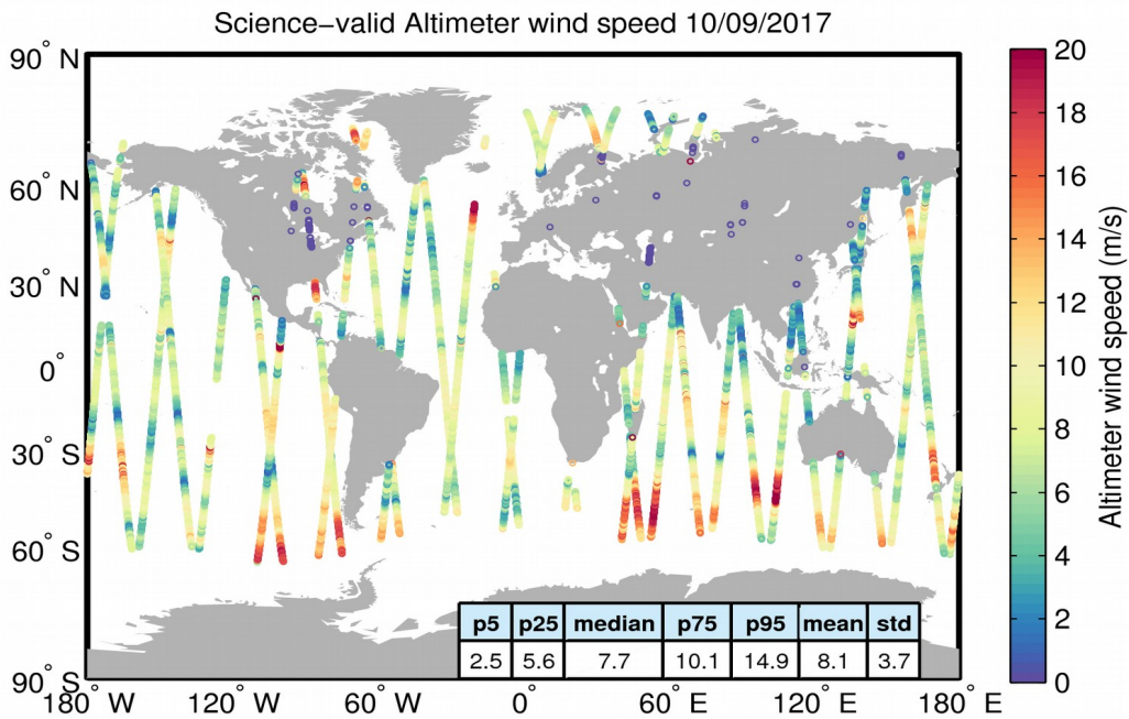
Figure 34. Geographical distribution of science-valid wind data over oceans and lakes for 10/09/2017. The statistical values shown in the table refer to the wind in m/s and are calculated over all measurements shown in the figure. Gray circles denote records that have been rejected based on the editing criteria described in Table 5.
