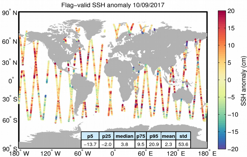
Figure 5. Geographical distribution of flag-valid 1-Hz SSH anomaly data over oceans and lakes for 10/09/2017. The statistical values shown in the table refer to the SSH anomaly in cm and are calculated over all measurements shown in the figure.
