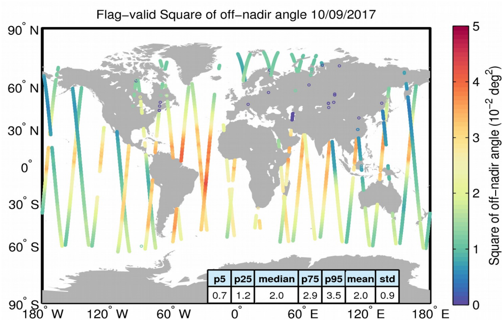
Figure 37. Geographical distribution of flag-valid mispointing data over oceans and lakes for 10/09/2017. The statistical values shown in the table refer to the mispointing in 10^{-2} deg 2 and are calculated over all measurements shown in the figure.
