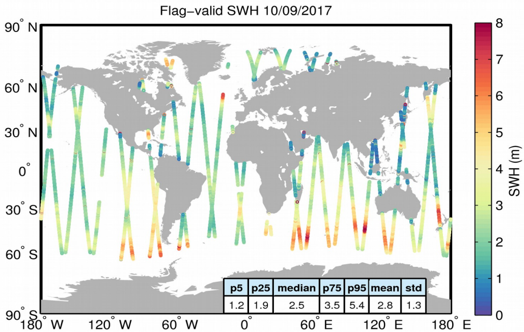
Figure 15. Geographical distribution of flag-valid SWH data over oceans and lakes for 10/09/2017. The statistical values shown in the table refer to the SWH in m and are calculated over all measurements shown in the figure.
