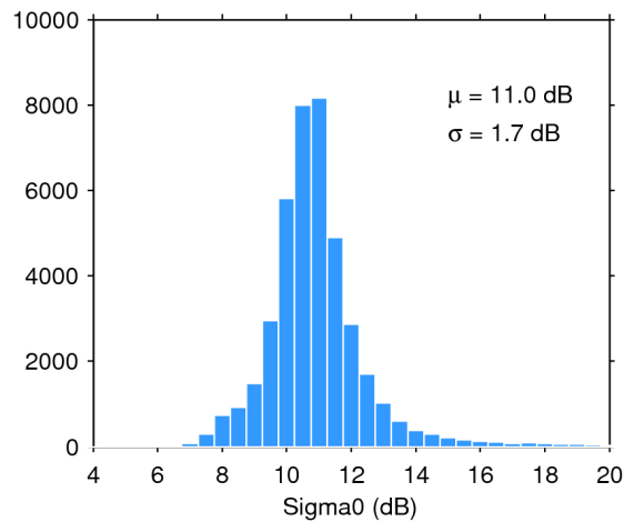
Figure 25. Histogram of flag-valid sigma0 over oceans and lakes for 10/09/2017. The mean ( \mu ) and standard deviation ( \sigma ) are also shown. Note that values outside [4 20] dB are excluded from the histogram for the sake of readability but not from the computation of \mu and \sigma .
