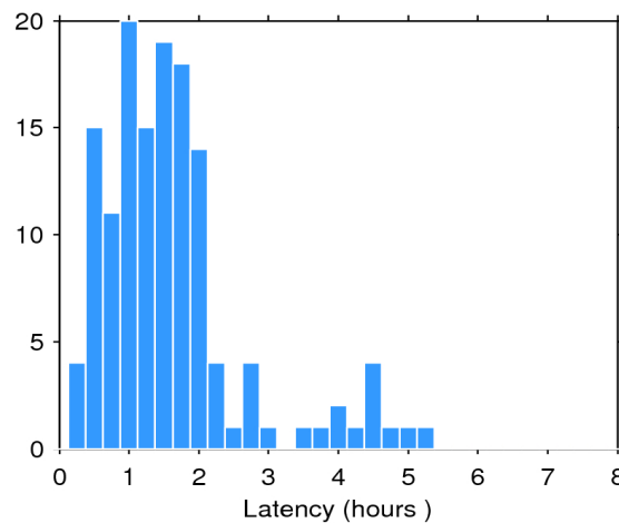
Figure 2. Histogram of the data latency for 10/09/2017. The y-axis denotes the number of files that are made available with a delay of x-hours with respect to the mean time of the records stored in the file.
