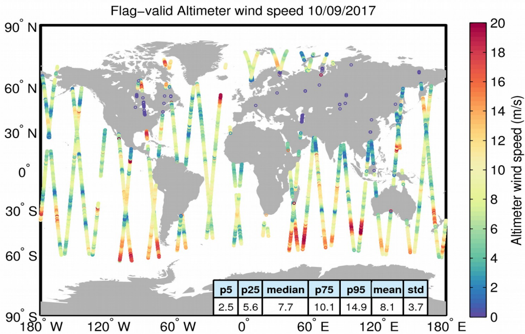
Figure 31. Geographical distribution of flag-valid wind data over oceans and lakes for 10/09/2017. The statistical values shown in the table refer to the wind in m/s and are calculated over all measurements shown in the figure.
