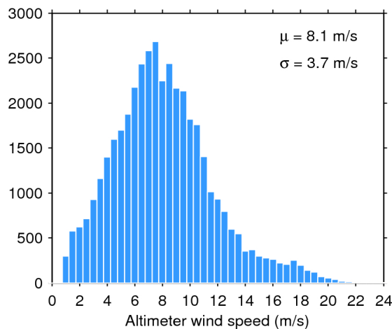
Figure 35. Histogram of science-valid wind over oceans and lakes for 10/09/2017. The mean ( \mu ) and standard deviation ( \sigma ) are also shown. Note that values larger than 24 m/s are excluded from the histogram for the sake of readability but not from the computation of \mu and \sigma .
