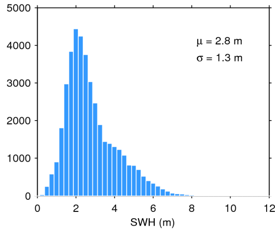
Figure 17. Histogram of flag-valid SWH over oceans and lakes for 10/09/2017. The mean ( \mu ) and standard deviation ( \sigma ) are also shown. Note that values larger than 12 m are excluded from the histogram for the sake of readability but not from the computation of \mu and \sigma .
