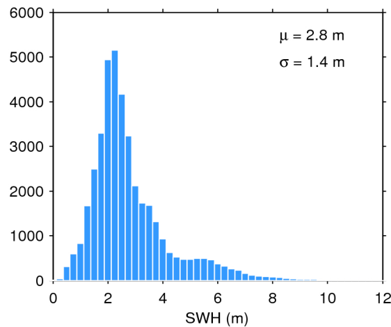
Figure 20. Histogram of science-valid SWH over oceans and lakes for 08/09/2017. The mean ( \mu ) and standard deviation ( \sigma ) are also shown. Note that values larger than 12 m are excluded from the histogram for the sake of readability but not from the computation of \mu and \sigma .
