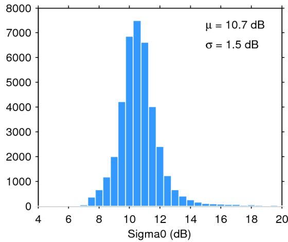
Figure 28. Histogram of science-valid sigma0 over oceans and lakes for 08/09/2017. The mean ( \mu ) and standard deviation ( \sigma ) are also shown. Note that values outside [4 20] dB are excluded from the histogram for the sake of readability but not from the computation of \mu and \sigma .
