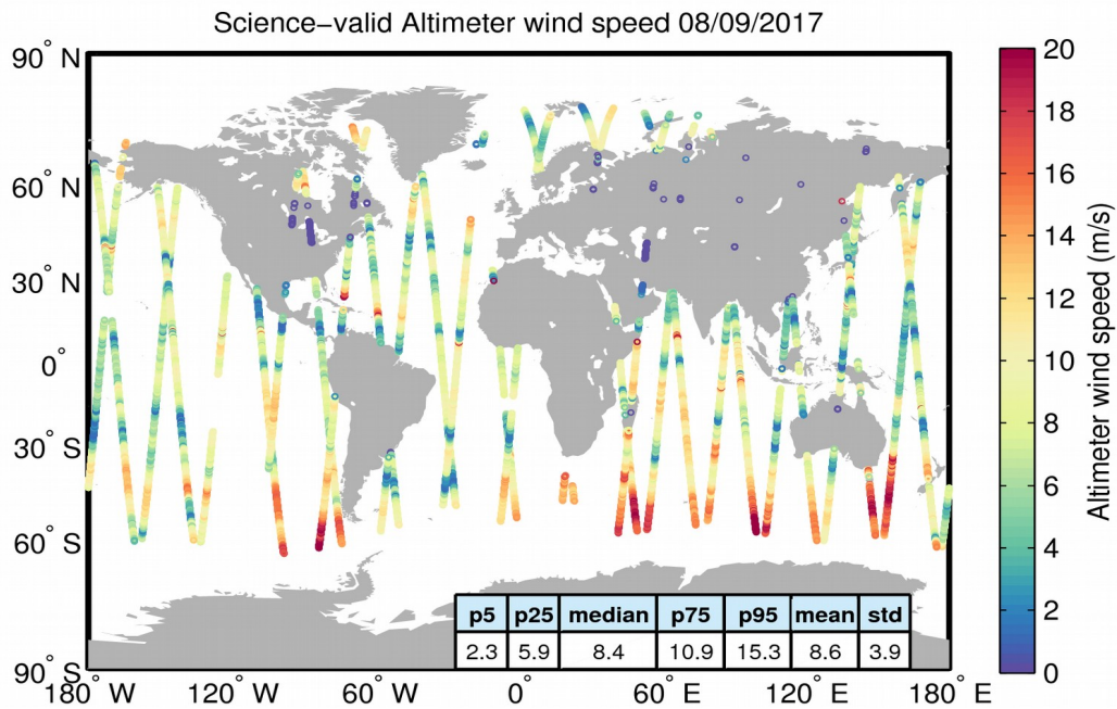
Figure 34. Geographical distribution of science-valid wind data over oceans and lakes for 08/09/2017. The statistical values shown in the table refer to the wind in m/s and are calculated over all measurements shown in the figure. Gray circles denote records that have been rejected based on the editing criteria described in Table 5.
