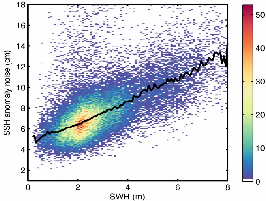
Figure 9. 2D histogram showing flag-valid SSH anomaly noise as a function of SWH for 08/09/2017. The black line denotes the median SSH anomaly noise as a function of SWH.
