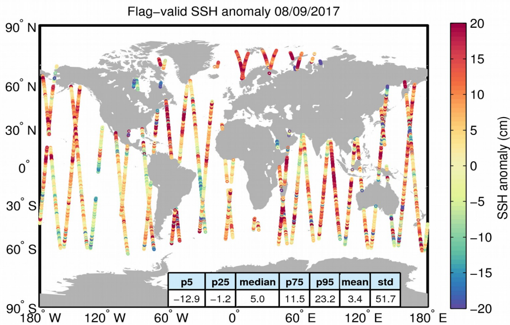
Figure 5. Geographical distribution of flag-valid 1-Hz SSH anomaly data over oceans and lakes for 08/09/2017. The statistical values shown in the table refer to the SSH anomaly in cm and are calculated over all measurements shown in the figure.
