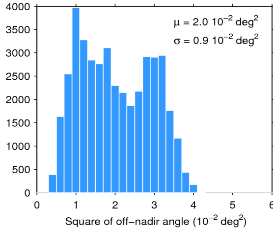
Figure 39. Histogram of flag-valid mispointing over oceans and lakes for 08/09/2017. The mean ( \mu ) and standard deviation ( \sigma ) are also shown. Note that values larger than 6 \cdot 10^{-2} \text{ deg}^2 are excluded from the histogram for the sake of readability but not from the computation of \mu and \sigma .
