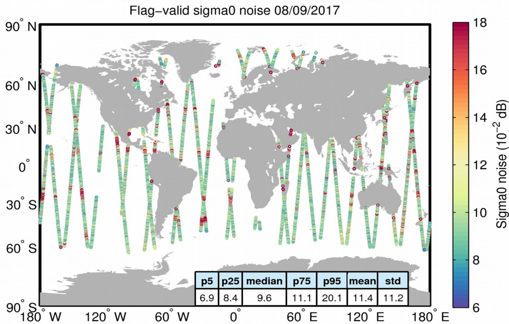
Figure 26. Geographical distribution of flag-valid 20-Hz sigma0 measurement noise over oceans and lakes for 08/09/2017. The statistical values shown in the table refer to the sigma0 noise and are calculated over all measurements shown in the figure.
