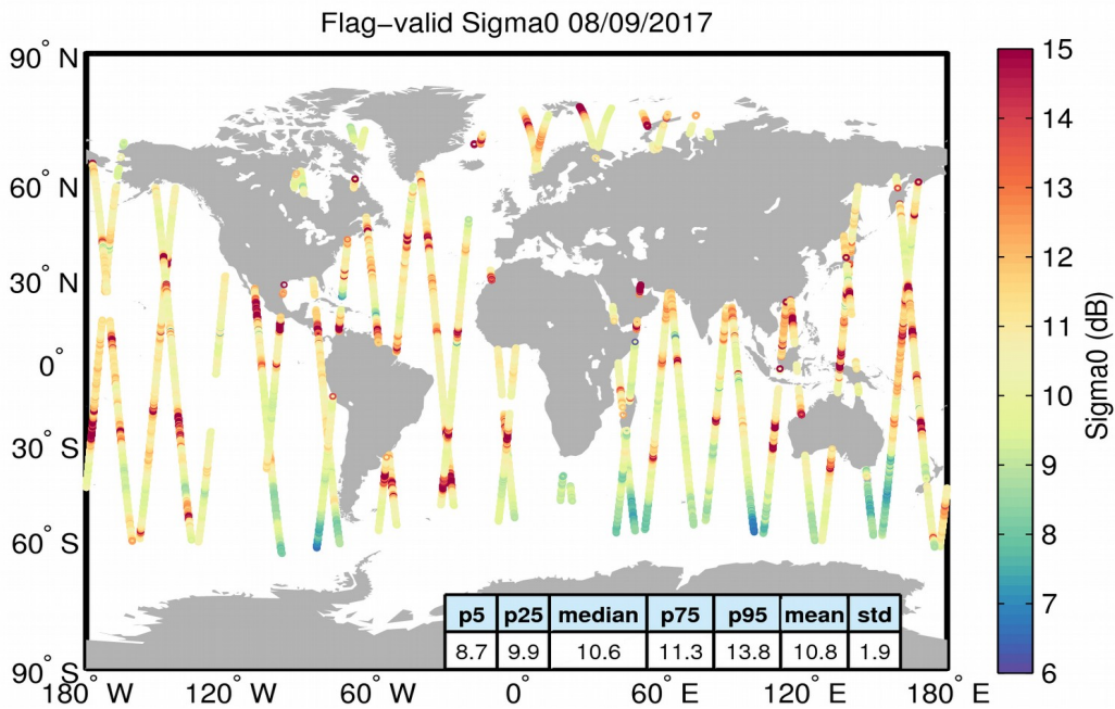
Figure 23. Geographical distribution of flag-valid sigma0 data over oceans and lakes for 08/09/2017. The statistical values shown in the table refer to the sigma0 in dB and are calculated over all measurements shown in the figure.
