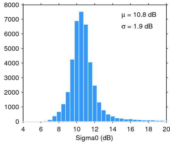
Figure 25. Histogram of flag-valid sigma0 over oceans and lakes for 08/09/2017. The mean ( \mu ) and standard deviation ( \sigma ) are also shown. Note that values outside [4 20] dB are excluded from the histogram for the sake of readability but not from the computation of \mu and \sigma .
