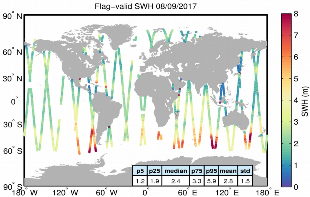
Figure 15. Geographical distribution of flag-valid SWH data over oceans and lakes for 08/09/2017. The statistical values shown in the table refer to the SWH in m and are calculated over all measurements shown in the figure.
