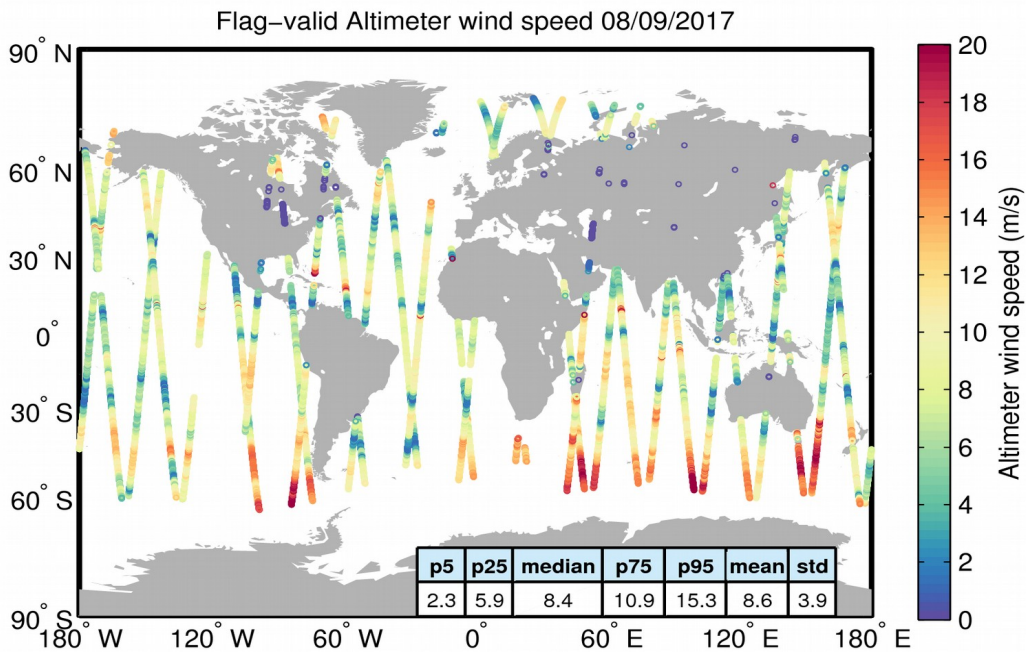
Figure 31. Geographical distribution of flag-valid wind data over oceans and lakes for 08/09/2017. The statistical values shown in the table refer to the wind in m/s and are calculated over all measurements shown in the figure.
