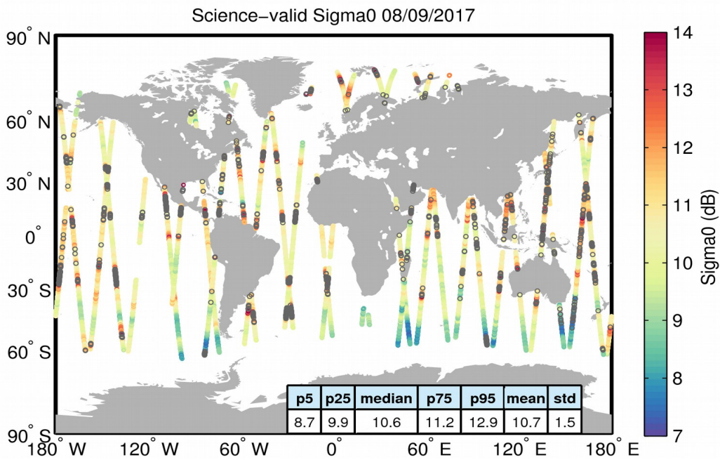
Figure 27. Geographical distribution of science-valid sigma0 data over oceans and lakes for 08/09/2017. The statistical values shown in the table refer to the sigma0 in dB and are calculated over all measurements shown in the figure. Gray circles denote records that have been rejected based on the editing criteria described in Table 4.
