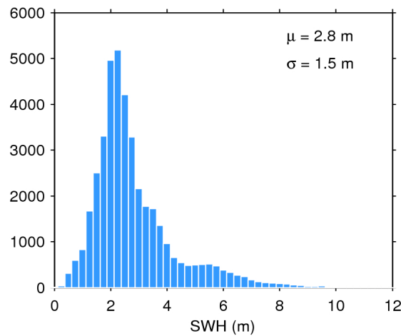
Figure 17. Histogram of flag-valid SWH over oceans and lakes for 08/09/2017. The mean ( \mu ) and standard deviation ( \sigma ) are also shown. Note that values larger than 12 m are excluded from the histogram for the sake of readability but not from the computation of \mu and \sigma .
