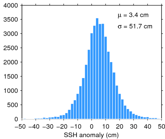
Figure 7. Histogram of flag-valid SSH anomaly over oceans and lakes for 08/09/2017. The mean ( \mu ) and standard deviation ( \sigma ) are also shown. Note that values outside [-50 50] cm are excluded from the histogram for the sake of readability but not from the computation of \mu and \sigma .
