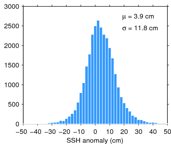
Figure 11. Histogram of science-valid SSH anomaly over oceans and lakes for 07/09/2017. The mean ( \mu ) and standard deviation ( \sigma ) are also shown. Note that values outside [-50 50] cm are excluded from the histogram for the sake of readability but not from the computation of \mu and \sigma .
