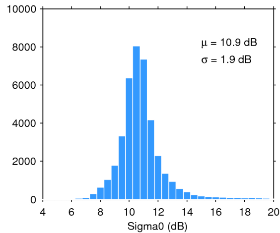
Figure 25. Histogram of flag-valid sigma0 over oceans and lakes for 07/09/2017. The mean ( \mu ) and standard deviation ( \sigma ) are also shown. Note that values outside [4 20] dB are excluded from the histogram for the sake of readability but not from the computation of \mu and \sigma .
