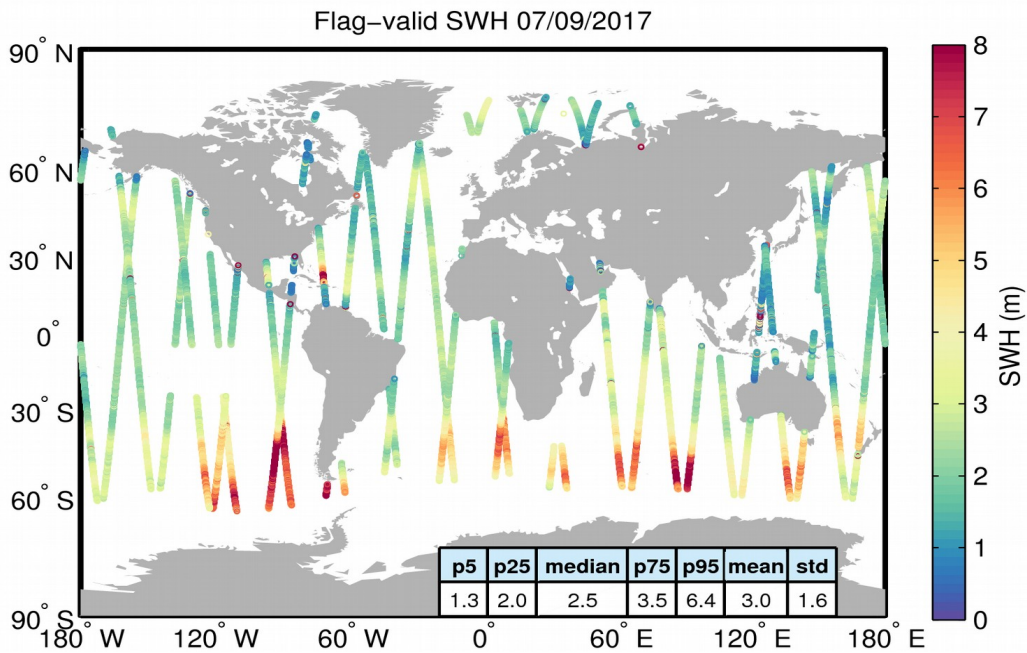
Figure 15. Geographical distribution of flag-valid SWH data over oceans and lakes for 07/09/2017. The statistical values shown in the table refer to the SWH in m and are calculated over all measurements shown in the figure.
