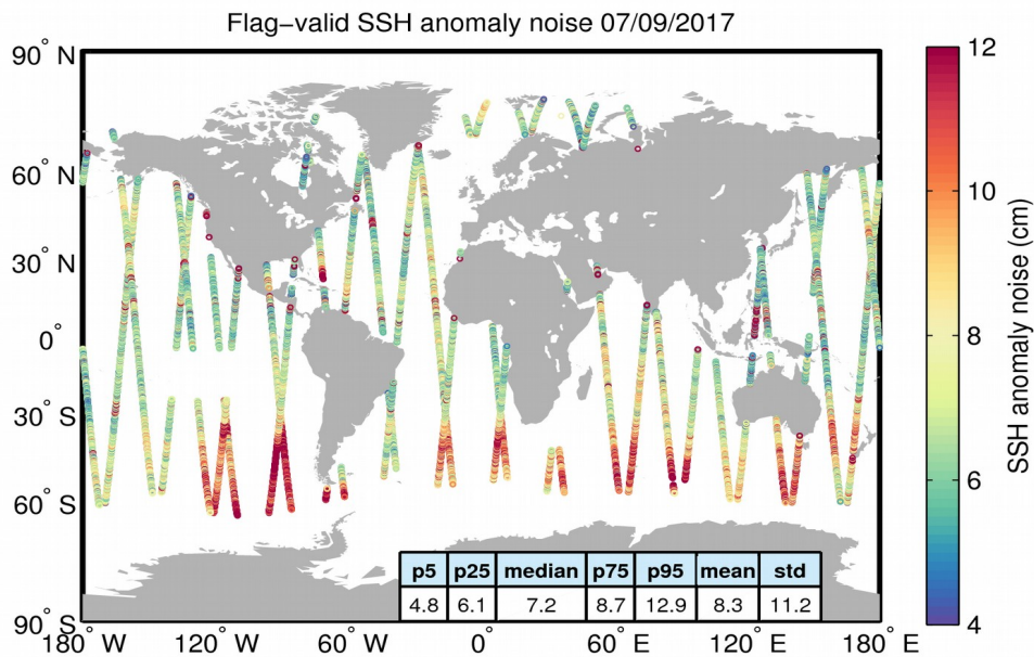
Figure 8. Geographical distribution of flag-valid 20-Hz SSH anomaly measurement noise over oceans and lakes for 07/09/2017. The statistical values shown in the table refer to the SSH anomaly noise and are calculated over all measurements shown in the figure.
