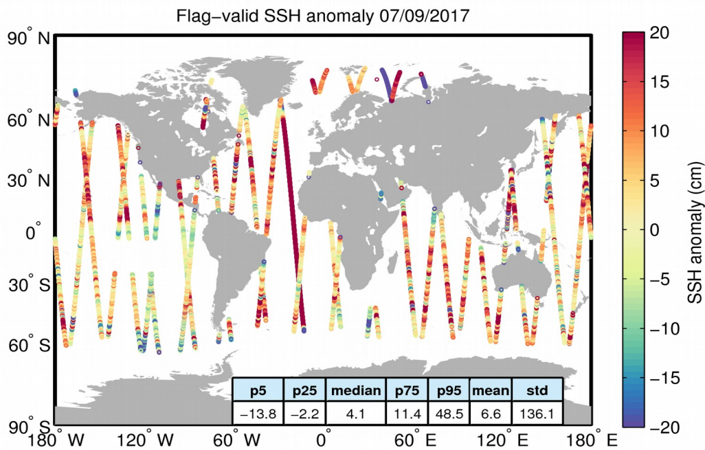
Figure 5. Geographical distribution of flag-valid 1-Hz SSH anomaly data over oceans and lakes for 07/09/2017. The statistical values shown in the table refer to the SSH anomaly in cm and are calculated over all measurements shown in the figure.
