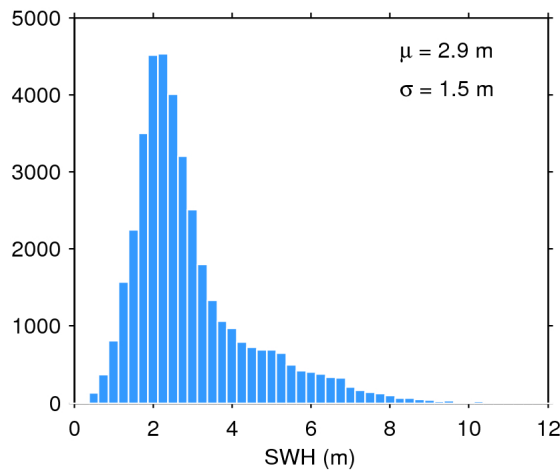
Figure 20. Histogram of science-valid SWH over oceans and lakes for 07/09/2017. The mean ( \mu ) and standard deviation ( \sigma ) are also shown. Note that values larger than 12 m are excluded from the histogram for the sake of readability but not from the computation of \mu and \sigma .
