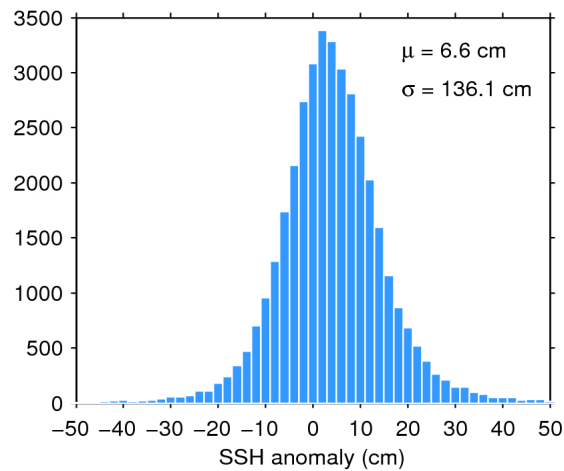
Figure 7. Histogram of flag-valid SSH anomaly over oceans and lakes for 07/09/2017. The mean ( \mu ) and standard deviation ( \sigma ) are also shown. Note that values outside [-50 50] cm are excluded from the histogram for the sake of readability but not from the computation of \mu and \sigma .
