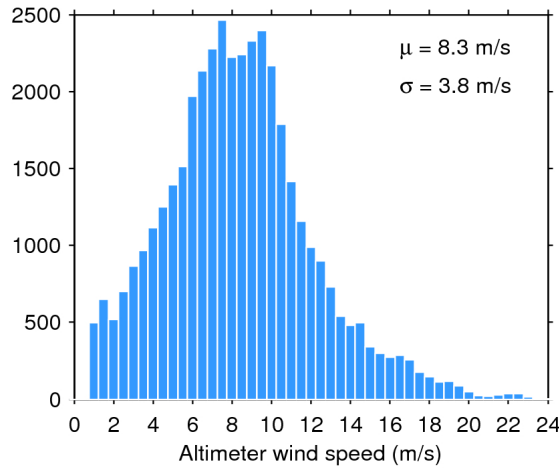
Figure 33. Histogram of flag-valid wind over oceans and lakes for 07/09/2017. The mean ( \mu ) and standard deviation ( \sigma ) are also shown. Note that values larger than 24 m/s are excluded from the histogram for the sake of readability but not from the computation of \mu and \sigma .
