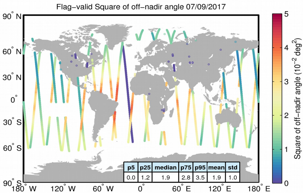
Figure 37. Geographical distribution of flag-valid mispointing data over oceans and lakes for 07/09/2017. The statistical values shown in the table refer to the mispointing in 10^{-2} deg 2 and are calculated over all measurements shown in the figure.
