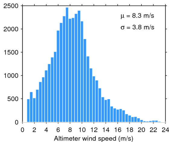
Figure 35. Histogram of science-valid wind over oceans and lakes for 07/09/2017. The mean ( \mu ) and standard deviation ( \sigma ) are also shown. Note that values larger than 24 m/s are excluded from the histogram for the sake of readability but not from the computation of \mu and \sigma .
