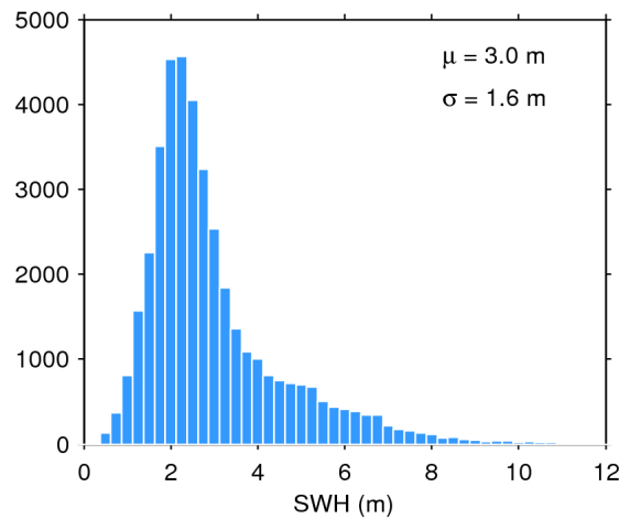
Figure 17. Histogram of flag-valid SWH over oceans and lakes for 07/09/2017. The mean ( \mu ) and standard deviation ( \sigma ) are also shown. Note that values larger than 12 m are excluded from the histogram for the sake of readability but not from the computation of \mu and \sigma .
