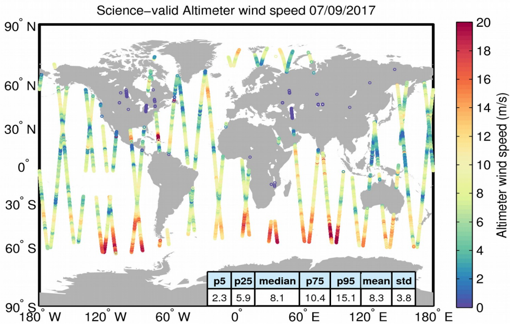
Figure 34. Geographical distribution of science-valid wind data over oceans and lakes for 07/09/2017. The statistical values shown in the table refer to the wind in m/s and are calculated over all measurements shown in the figure. Gray circles denote records that have been rejected based on the editing criteria described in Table 5.
