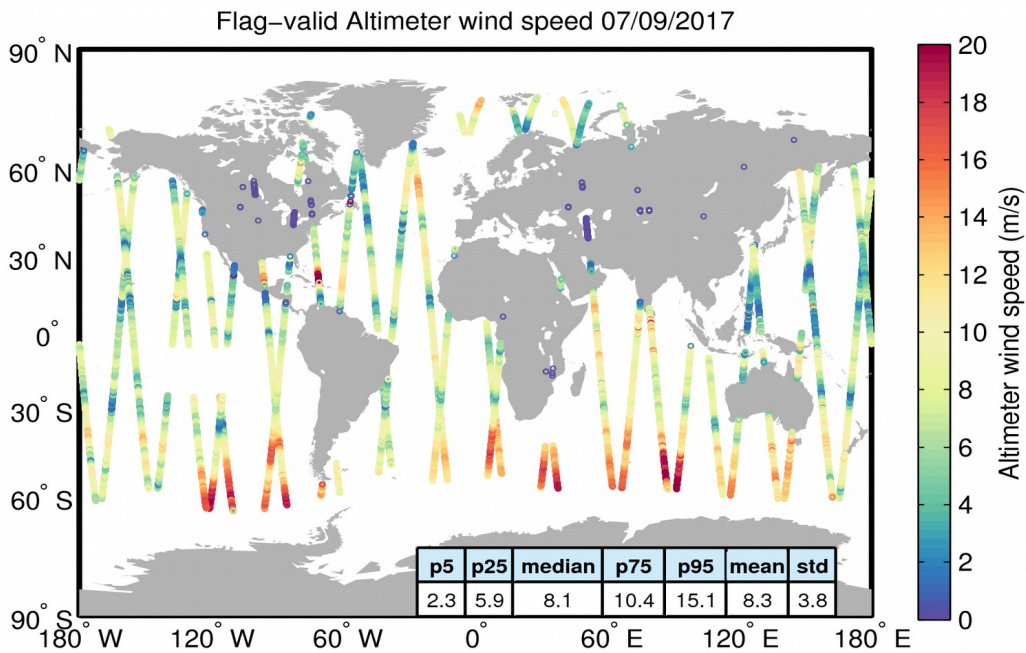
Figure 31. Geographical distribution of flag-valid wind data over oceans and lakes for 07/09/2017. The statistical values shown in the table refer to the wind in m/s and are calculated over all measurements shown in the figure.
