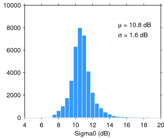
Figure 28. Histogram of science-valid sigma0 over oceans and lakes for 07/09/2017. The mean ( \mu ) and standard deviation ( \sigma ) are also shown. Note that values outside [4 20] dB are excluded from the histogram for the sake of readability but not from the computation of \mu and \sigma .
