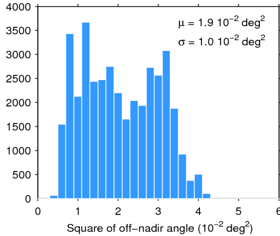
Figure 39. Histogram of flag-valid mispointing over oceans and lakes for 07/09/2017. The mean ( \mu ) and standard deviation ( \sigma ) are also shown. Note that values larger than 6 \cdot 10^{-2} \text{ deg}^2 are excluded from the histogram for the sake of readability but not from the computation of \mu and \sigma .
