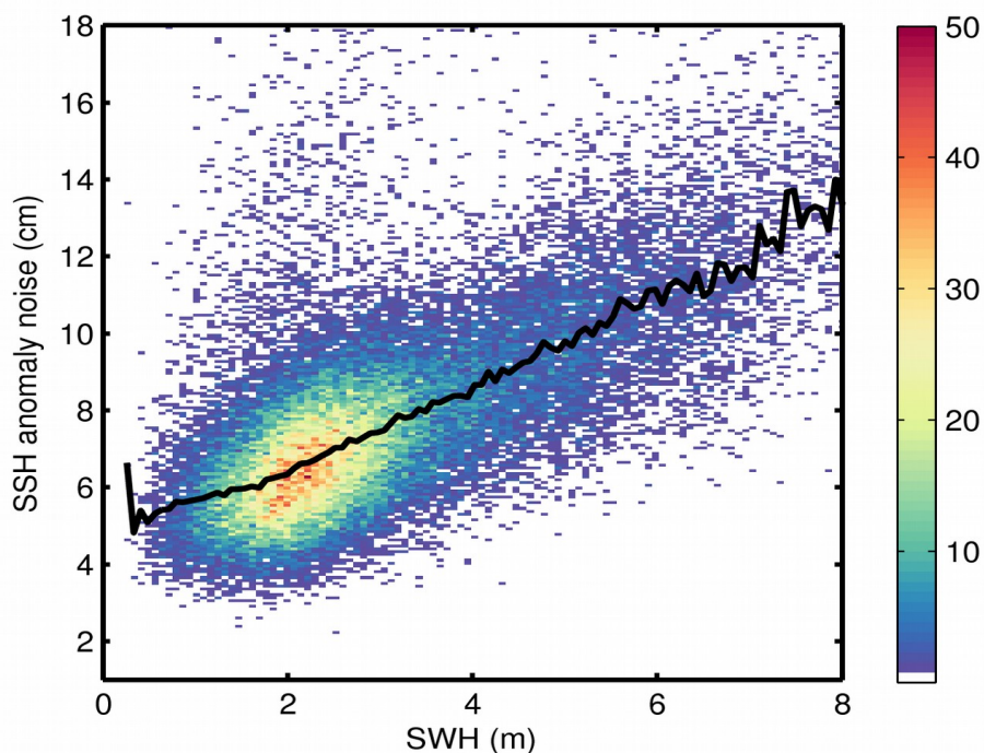
Figure 9. 2D histogram showing flag-valid SSH anomaly noise as a function of SWH for 07/09/2017. The black line denotes the median SSH anomaly noise as a function of SWH.
