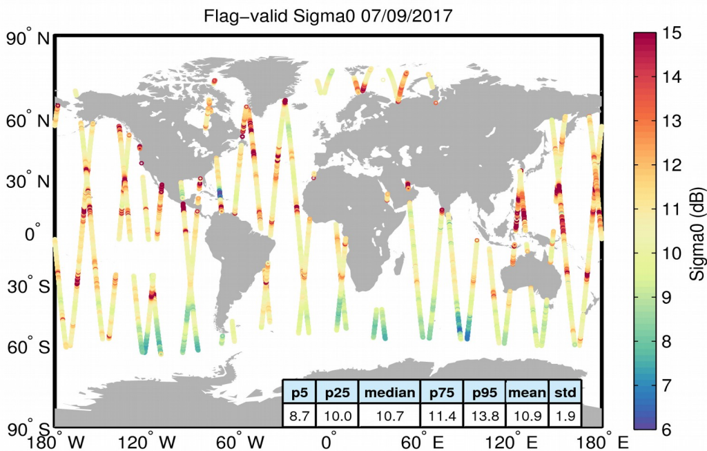
Figure 23. Geographical distribution of flag-valid sigma0 data over oceans and lakes for 07/09/2017. The statistical values shown in the table refer to the sigma0 in dB and are calculated over all measurements shown in the figure.
