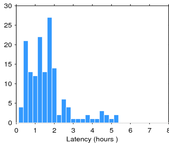
Figure 2. Histogram of the data latency for 07/09/2017. The y-axis denotes the number of files that are made available with a delay of x-hours with respect to the mean time of the records stored in the file.
