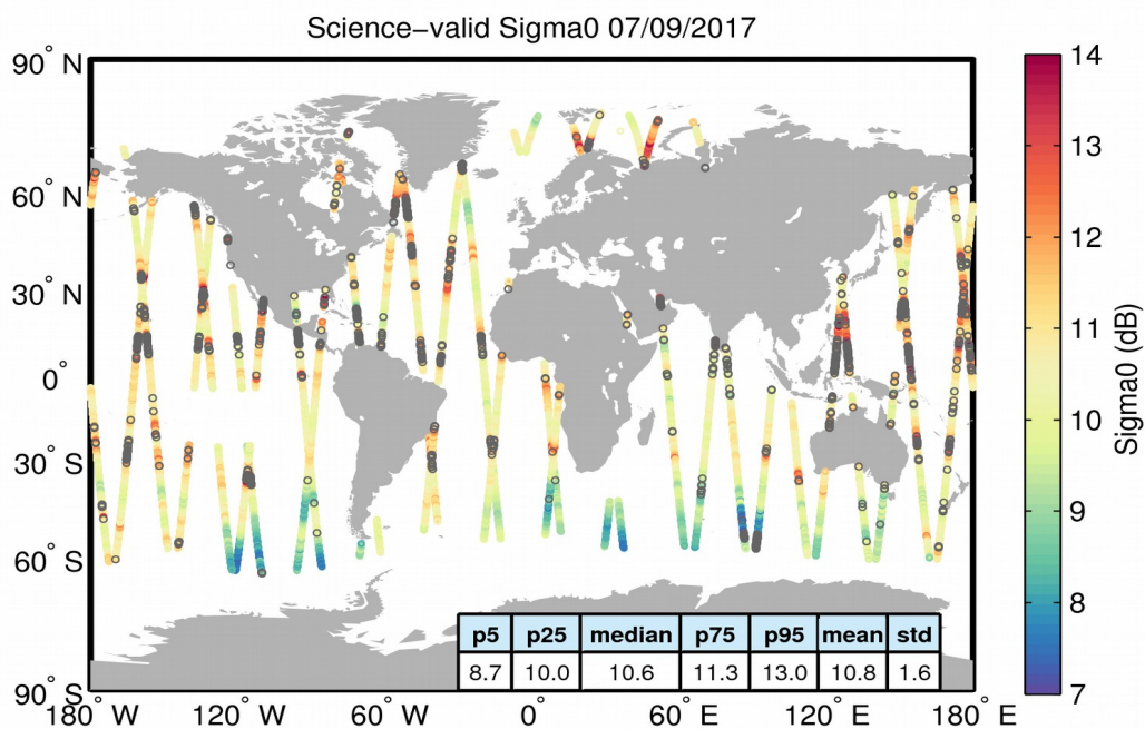
Figure 27. Geographical distribution of science-valid sigma0 data over oceans and lakes for 07/09/2017. The statistical values shown in the table refer to the sigma0 in dB and are calculated over all measurements shown in the figure. Gray circles denote records that have been rejected based on the editing criteria described in Table 4.
