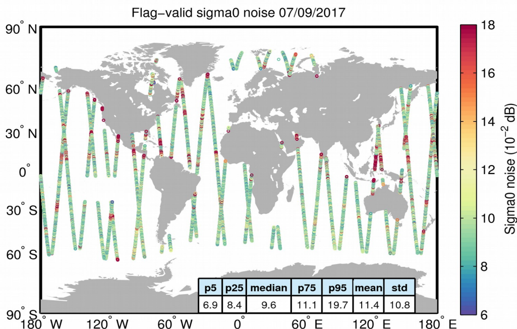
Figure 26. Geographical distribution of flag-valid 20-Hz sigma0 measurement noise over oceans and lakes for 07/09/2017. The statistical values shown in the table refer to the sigma0 noise and are calculated over all measurements shown in the figure.
