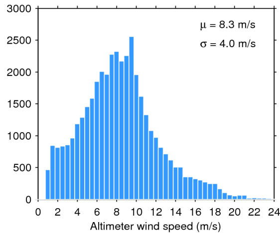
Figure 33. Histogram of flag-valid wind over oceans and lakes for 05/09/2017. The mean ( \mu ) and standard deviation ( \sigma ) are also shown. Note that values larger than 24 m/s are excluded from the histogram for the sake of readability but not from the computation of \mu and \sigma .
