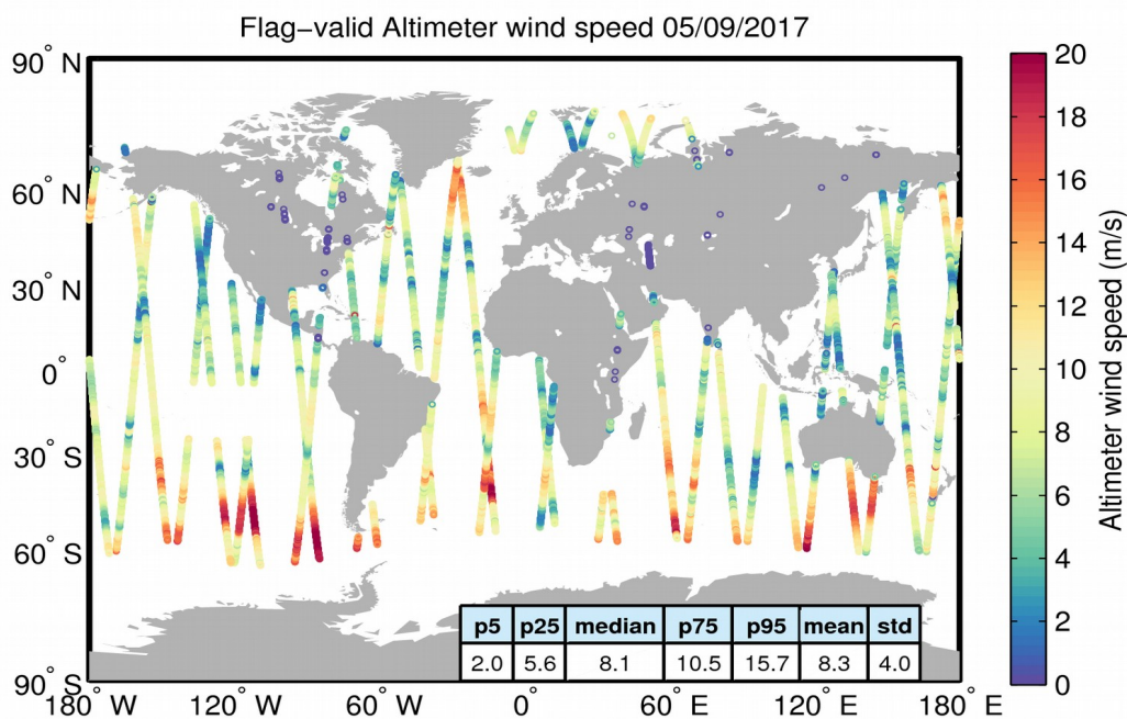
Figure 31. Geographical distribution of flag-valid wind data over oceans and lakes for 05/09/2017. The statistical values shown in the table refer to the wind in m/s and are calculated over all measurements shown in the figure.
