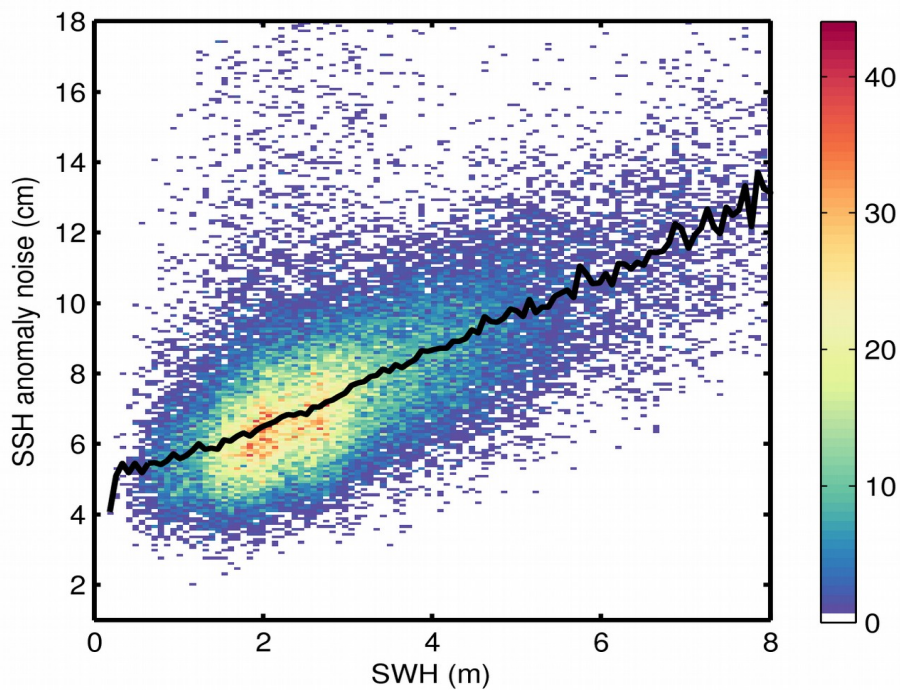
Figure 9. 2D histogram showing flag-valid SSH anomaly noise as a function of SWH for 05/09/2017. The black line denotes the median SSH anomaly noise as a function of SWH.
