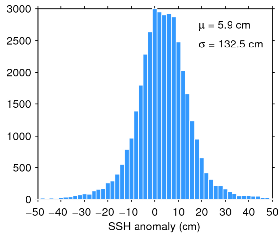
Figure 7. Histogram of flag-valid SSH anomaly over oceans and lakes for 05/09/2017. The mean ( \mu ) and standard deviation ( \sigma ) are also shown. Note that values outside [-50 50] cm are excluded from the histogram for the sake of readability but not from the computation of \mu and \sigma .
