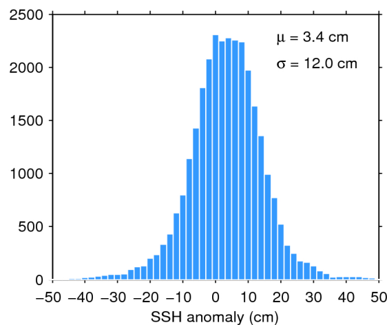
Figure 11. Histogram of science-valid SSH anomaly over oceans and lakes for 05/09/2017. The mean ( \mu ) and standard deviation ( \sigma ) are also shown. Note that values outside [-50 50] cm are excluded from the histogram for the sake of readability but not from the computation of \mu and \sigma .
