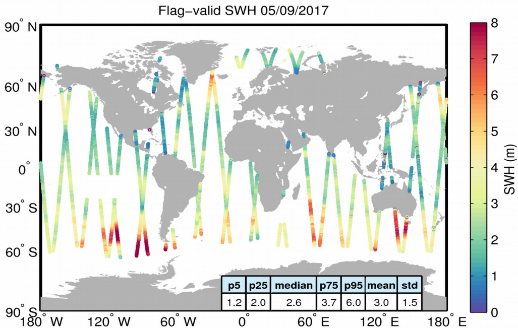
Figure 15. Geographical distribution of flag-valid SWH data over oceans and lakes for 05/09/2017. The statistical values shown in the table refer to the SWH in m and are calculated over all measurements shown in the figure.
