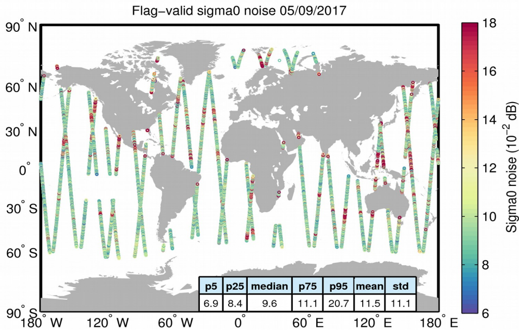
Figure 26. Geographical distribution of flag-valid 20-Hz sigma0 measurement noise over oceans and lakes for 05/09/2017. The statistical values shown in the table refer to the sigma0 noise and are calculated over all measurements shown in the figure.
