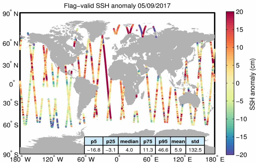
Figure 5. Geographical distribution of flag-valid 1-Hz SSH anomaly data over oceans and lakes for 05/09/2017. The statistical values shown in the table refer to the SSH anomaly in cm and are calculated over all measurements shown in the figure.
