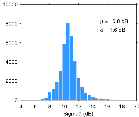
Figure 28. Histogram of science-valid sigma0 over oceans and lakes for 05/09/2017. The mean ( \mu ) and standard deviation ( \sigma ) are also shown. Note that values outside [4 20] dB are excluded from the histogram for the sake of readability but not from the computation of \mu and \sigma .
