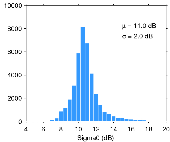
Figure 25. Histogram of flag-valid sigma0 over oceans and lakes for 05/09/2017. The mean ( \mu ) and standard deviation ( \sigma ) are also shown. Note that values outside [4 20] dB are excluded from the histogram for the sake of readability but not from the computation of \mu and \sigma .
