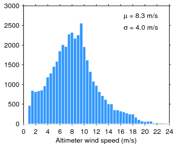
Figure 35. Histogram of science-valid wind over oceans and lakes for 05/09/2017. The mean ( \mu ) and standard deviation ( \sigma ) are also shown. Note that values larger than 24 m/s are excluded from the histogram for the sake of readability but not from the computation of \mu and \sigma .
