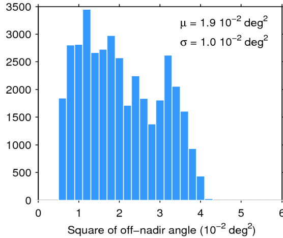
Figure 39. Histogram of flag-valid mispointing over oceans and lakes for 05/09/2017. The mean ( \mu ) and standard deviation ( \sigma ) are also shown. Note that values larger than 6 \cdot 10^{-2} \text{ deg}^2 are excluded from the histogram for the sake of readability but not from the computation of \mu and \sigma .
