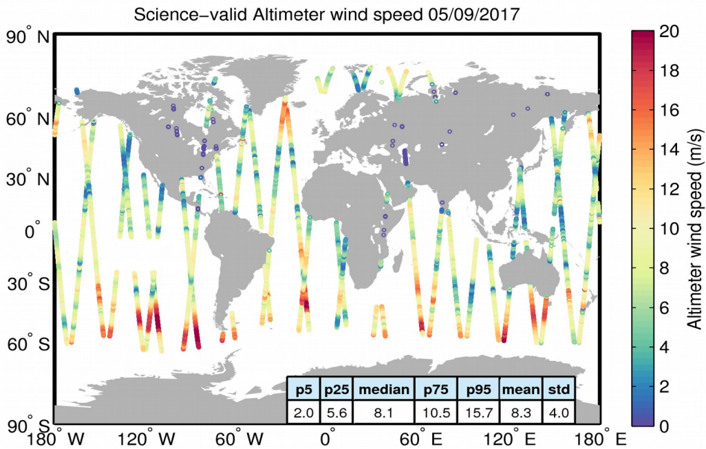
Figure 34. Geographical distribution of science-valid wind data over oceans and lakes for 05/09/2017. The statistical values shown in the table refer to the wind in m/s and are calculated over all measurements shown in the figure. Gray circles denote records that have been rejected based on the editing criteria described in Table 5.
