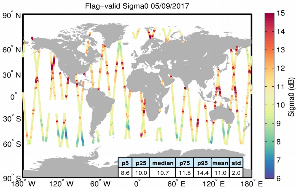
Figure 23. Geographical distribution of flag-valid sigma0 data over oceans and lakes for 05/09/2017. The statistical values shown in the table refer to the sigma0 in dB and are calculated over all measurements shown in the figure.
