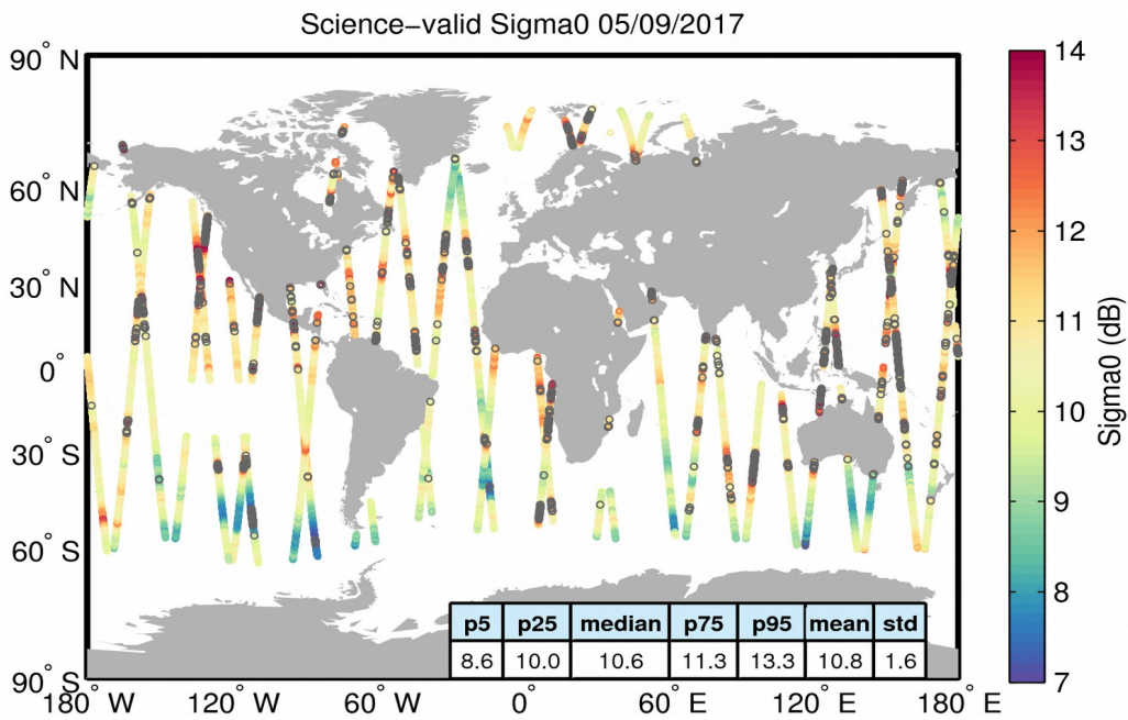
Figure 27. Geographical distribution of science-valid sigma0 data over oceans and lakes for 05/09/2017. The statistical values shown in the table refer to the sigma0 in dB and are calculated over all measurements shown in the figure. Gray circles denote records that have been rejected based on the editing criteria described in Table 4.
