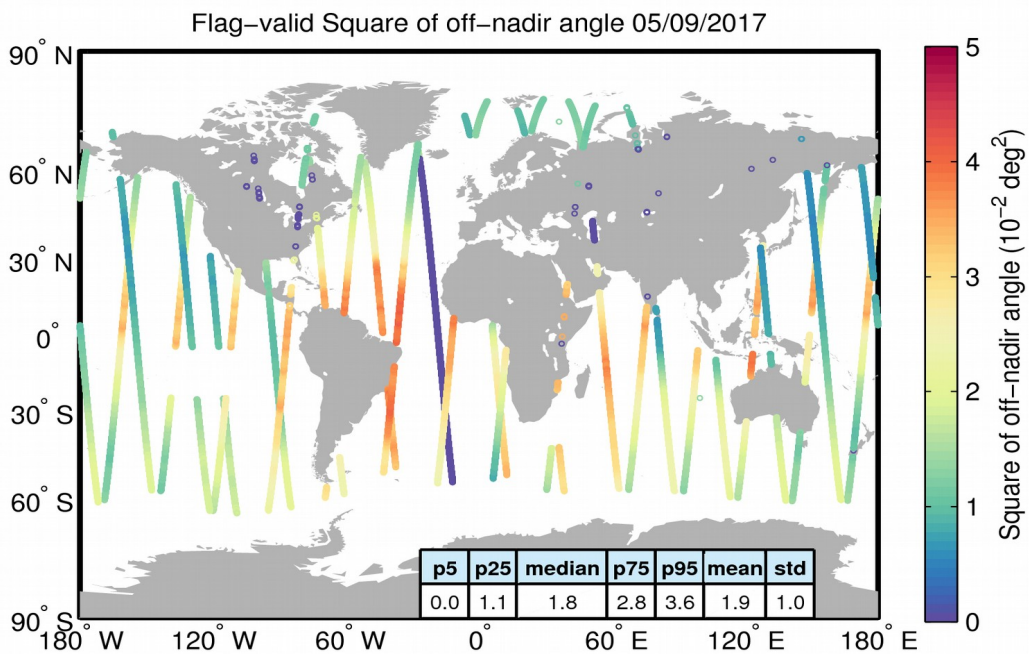
Figure 37. Geographical distribution of flag-valid mispointing data over oceans and lakes for 05/09/2017. The statistical values shown in the table refer to the mispointing in 10^{-2} deg 2 and are calculated over all measurements shown in the figure.
