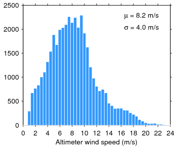
Figure 33. Histogram of flag-valid wind over oceans and lakes for 03/09/2017. The mean ( \mu ) and standard deviation ( \sigma ) are also shown. Note that values larger than 24 m/s are excluded from the histogram for the sake of readability but not from the computation of \mu and \sigma .
