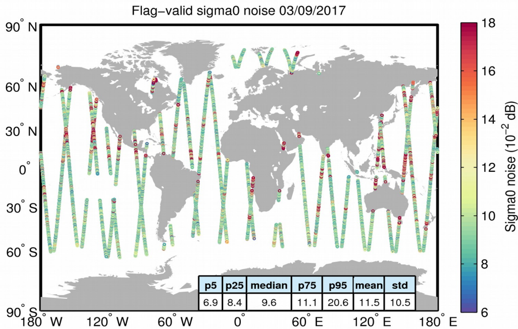
Figure 26. Geographical distribution of flag-valid 20-Hz sigma0 measurement noise over oceans and lakes for 03/09/2017. The statistical values shown in the table refer to the sigma0 noise and are calculated over all measurements shown in the figure.
