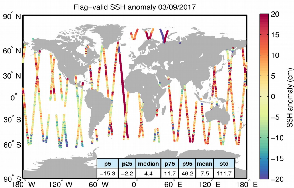
Figure 5. Geographical distribution of flag-valid 1-Hz SSH anomaly data over oceans and lakes for 03/09/2017. The statistical values shown in the table refer to the SSH anomaly in cm and are calculated over all measurements shown in the figure.
