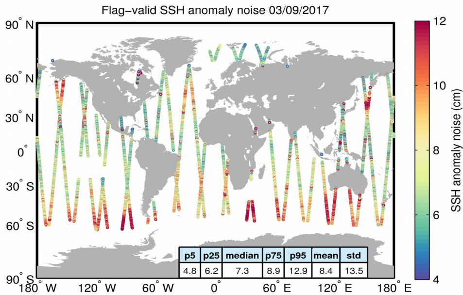
Figure 8. Geographical distribution of flag-valid 20-Hz SSH anomaly measurement noise over oceans and lakes for 03/09/2017. The statistical values shown in the table refer to the SSH anomaly noise and are calculated over all measurements shown in the figure.
