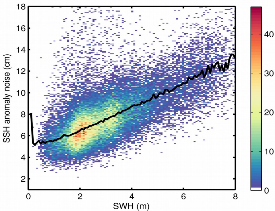
Figure 9. 2D histogram showing flag-valid SSH anomaly noise as a function of SWH for 03/09/2017. The black line denotes the median SSH anomaly noise as a function of SWH.
