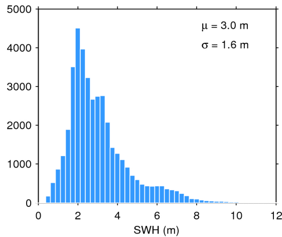
Figure 17. Histogram of flag-valid SWH over oceans and lakes for 03/09/2017. The mean ( \mu ) and standard deviation ( \sigma ) are also shown. Note that values larger than 12 m are excluded from the histogram for the sake of readability but not from the computation of \mu and \sigma .
