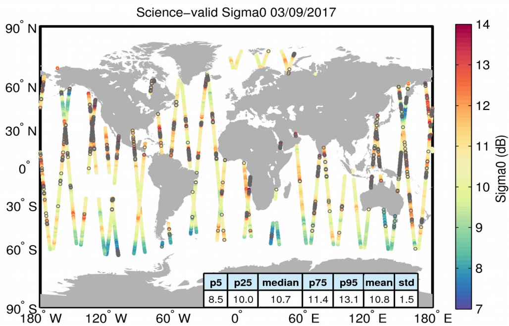
Figure 27. Geographical distribution of science-valid sigma0 data over oceans and lakes for 03/09/2017. The statistical values shown in the table refer to the sigma0 in dB and are calculated over all measurements shown in the figure. Gray circles denote records that have been rejected based on the editing criteria described in Table 4.
