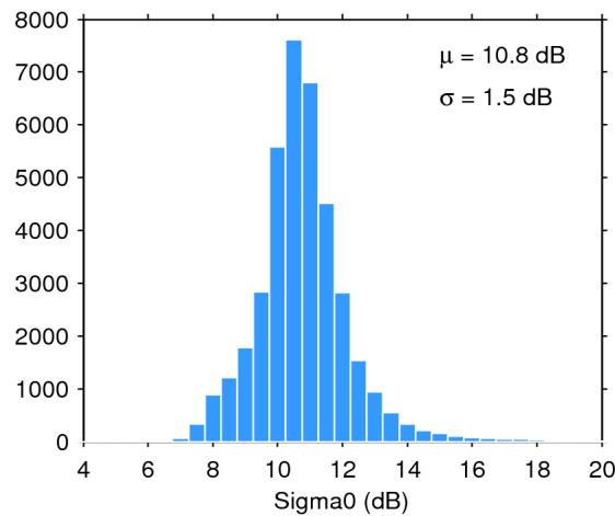
Figure 28. Histogram of science-valid sigma0 over oceans and lakes for 03/09/2017. The mean ( \mu ) and standard deviation ( \sigma ) are also shown. Note that values outside [4 20] dB are excluded from the histogram for the sake of readability but not from the computation of \mu and \sigma .
