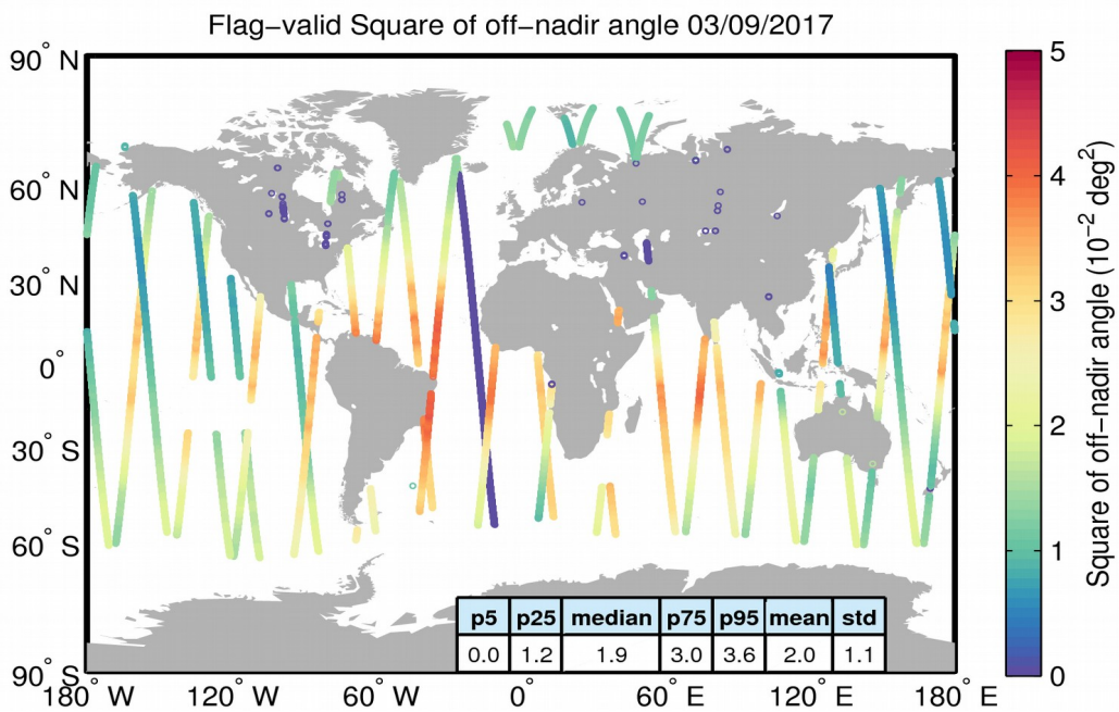
Figure 37. Geographical distribution of flag-valid mispointing data over oceans and lakes for 03/09/2017. The statistical values shown in the table refer to the mispointing in 10^{-2} deg 2 and are calculated over all measurements shown in the figure.
