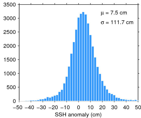
Figure 7. Histogram of flag-valid SSH anomaly over oceans and lakes for 03/09/2017. The mean ( \mu ) and standard deviation ( \sigma ) are also shown. Note that values outside [-50 50] cm are excluded from the histogram for the sake of readability but not from the computation of \mu and \sigma .
