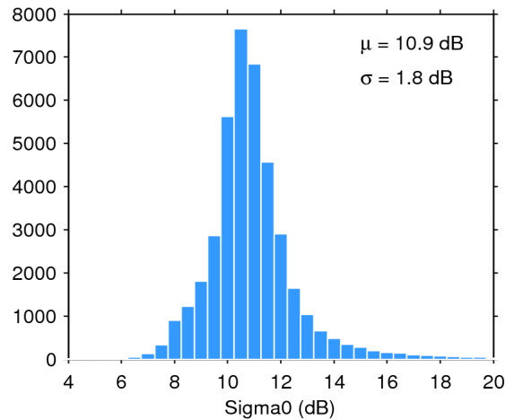
Figure 25. Histogram of flag-valid sigma0 over oceans and lakes for 03/09/2017. The mean ( \mu ) and standard deviation ( \sigma ) are also shown. Note that values outside [4 20] dB are excluded from the histogram for the sake of readability but not from the computation of \mu and \sigma .
