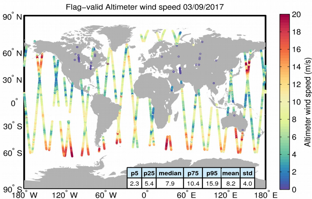
Figure 31. Geographical distribution of flag-valid wind data over oceans and lakes for 03/09/2017. The statistical values shown in the table refer to the wind in m/s and are calculated over all measurements shown in the figure.
