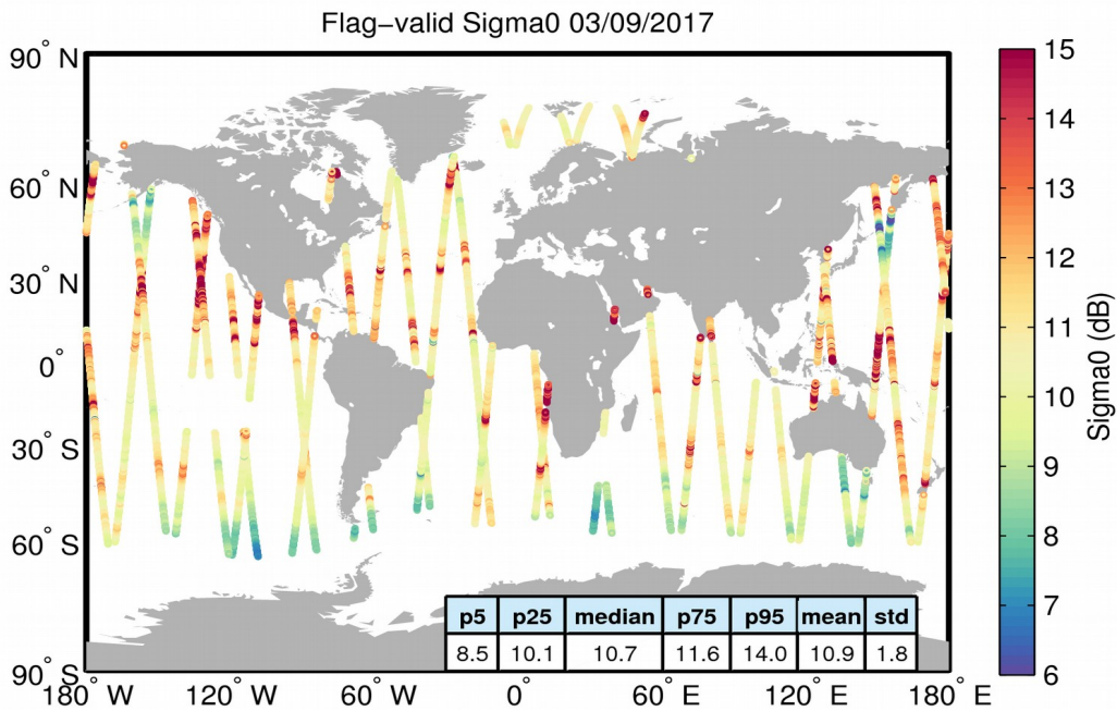
Figure 23. Geographical distribution of flag-valid sigma0 data over oceans and lakes for 03/09/2017. The statistical values shown in the table refer to the sigma0 in dB and are calculated over all measurements shown in the figure.
