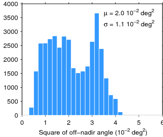
Figure 39. Histogram of flag-valid mispointing over oceans and lakes for 03/09/2017. The mean ( \mu ) and standard deviation ( \sigma ) are also shown. Note that values larger than 6 \cdot 10^{-2} \text{ deg}^2 are excluded from the histogram for the sake of readability but not from the computation of \mu and \sigma .
