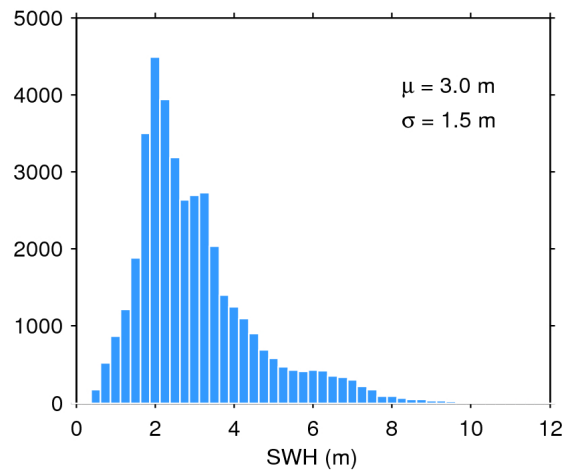
Figure 20. Histogram of science-valid SWH over oceans and lakes for 03/09/2017. The mean ( \mu ) and standard deviation ( \sigma ) are also shown. Note that values larger than 12 m are excluded from the histogram for the sake of readability but not from the computation of \mu and \sigma .
