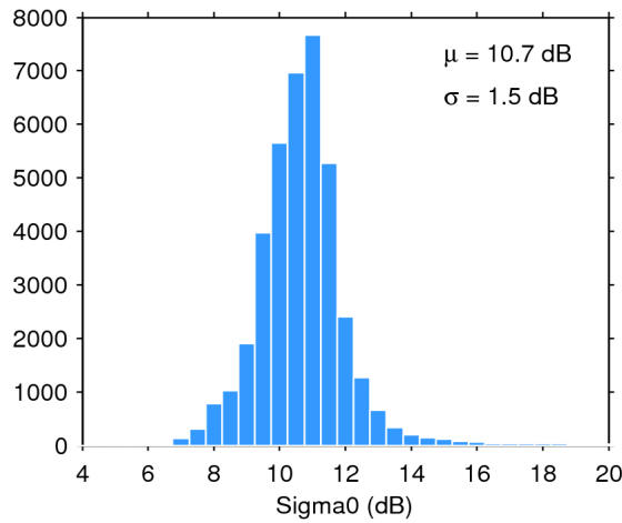
Figure 28. Histogram of science-valid sigma0 over oceans and lakes for 02/09/2017. The mean ( \mu ) and standard deviation ( \sigma ) are also shown. Note that values outside [4 20] dB are excluded from the histogram for the sake of readability but not from the computation of \mu and \sigma .
