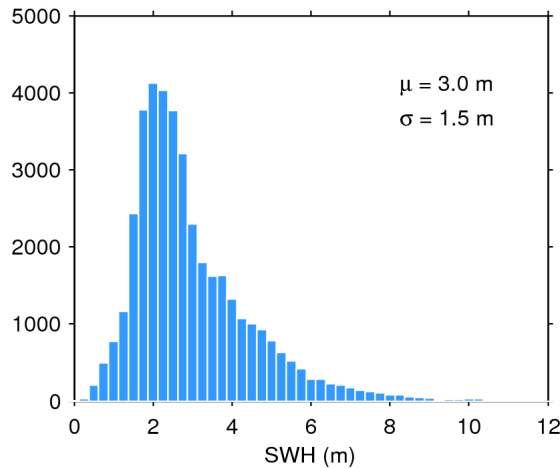
Figure 20. Histogram of science-valid SWH over oceans and lakes for 02/09/2017. The mean ( \mu ) and standard deviation ( \sigma ) are also shown. Note that values larger than 12 m are excluded from the histogram for the sake of readability but not from the computation of \mu and \sigma .
