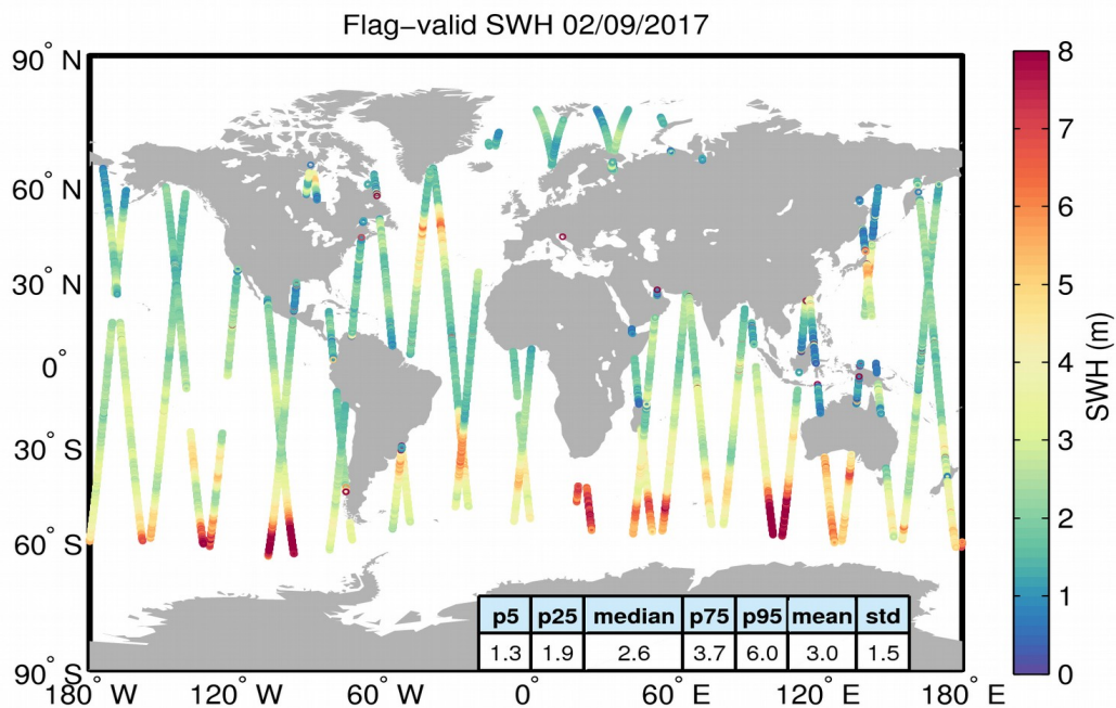
Figure 15. Geographical distribution of flag-valid SWH data over oceans and lakes for 02/09/2017. The statistical values shown in the table refer to the SWH in m and are calculated over all measurements shown in the figure.
