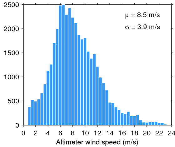
Figure 33. Histogram of flag-valid wind over oceans and lakes for 02/09/2017. The mean ( \mu ) and standard deviation ( \sigma ) are also shown. Note that values larger than 24 m/s are excluded from the histogram for the sake of readability but not from the computation of \mu and \sigma .
