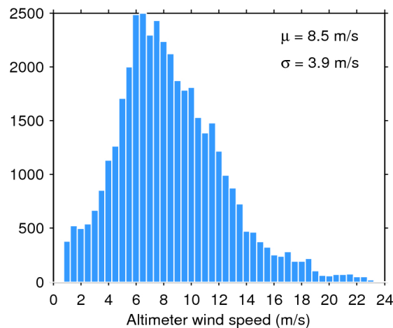
Figure 35. Histogram of science-valid wind over oceans and lakes for 02/09/2017. The mean ( \mu ) and standard deviation ( \sigma ) are also shown. Note that values larger than 24 m/s are excluded from the histogram for the sake of readability but not from the computation of \mu and \sigma .
