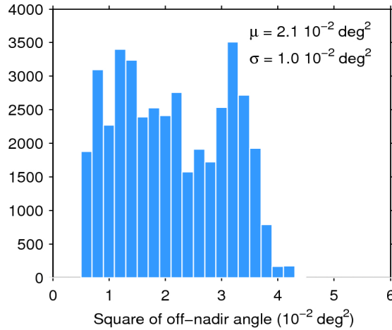
Figure 39. Histogram of flag-valid mispointing over oceans and lakes for 02/09/2017. The mean ( \mu ) and standard deviation ( \sigma ) are also shown. Note that values larger than 6 \cdot 10^{-2} \text{ deg}^2 are excluded from the histogram for the sake of readability but not from the computation of \mu and \sigma .
