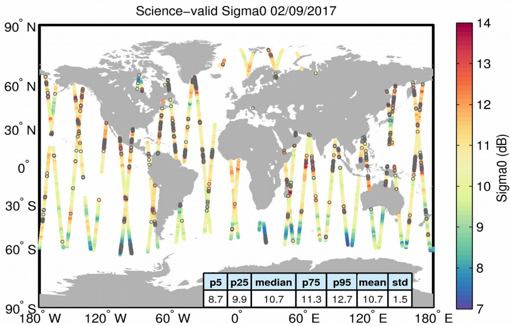
Figure 27. Geographical distribution of science-valid sigma0 data over oceans and lakes for 02/09/2017. The statistical values shown in the table refer to the sigma0 in dB and are calculated over all measurements shown in the figure. Gray circles denote records that have been rejected based on the editing criteria described in Table 4.
