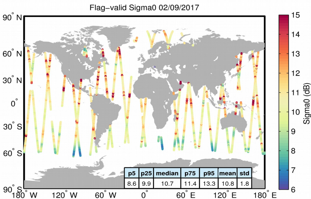
Figure 23. Geographical distribution of flag-valid sigma0 data over oceans and lakes for 02/09/2017. The statistical values shown in the table refer to the sigma0 in dB and are calculated over all measurements shown in the figure.
