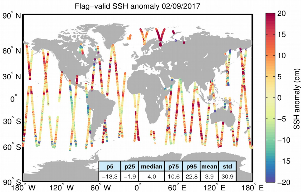
Figure 5. Geographical distribution of flag-valid 1-Hz SSH anomaly data over oceans and lakes for 02/09/2017. The statistical values shown in the table refer to the SSH anomaly in cm and are calculated over all measurements shown in the figure.
