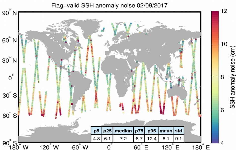
Figure 8. Geographical distribution of flag-valid 20-Hz SSH anomaly measurement noise over oceans and lakes for 02/09/2017. The statistical values shown in the table refer to the SSH anomaly noise and are calculated over all measurements shown in the figure.
