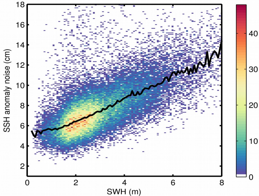
Figure 9. 2D histogram showing flag-valid SSH anomaly noise as a function of SWH for 02/09/2017. The black line denotes the median SSH anomaly noise as a function of SWH.
