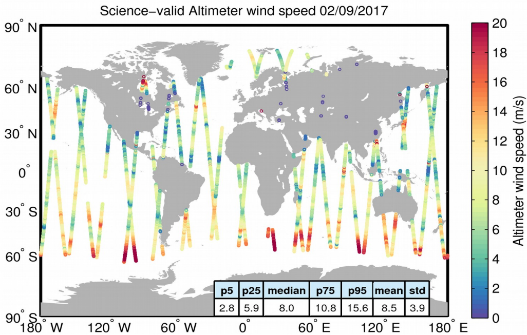
Figure 34. Geographical distribution of science-valid wind data over oceans and lakes for 02/09/2017. The statistical values shown in the table refer to the wind in m/s and are calculated over all measurements shown in the figure. Gray circles denote records that have been rejected based on the editing criteria described in Table 5.
