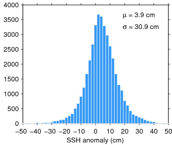
Figure 7. Histogram of flag-valid SSH anomaly over oceans and lakes for 02/09/2017. The mean ( \mu ) and standard deviation ( \sigma ) are also shown. Note that values outside [-50 50] cm are excluded from the histogram for the sake of readability but not from the computation of \mu and \sigma .
