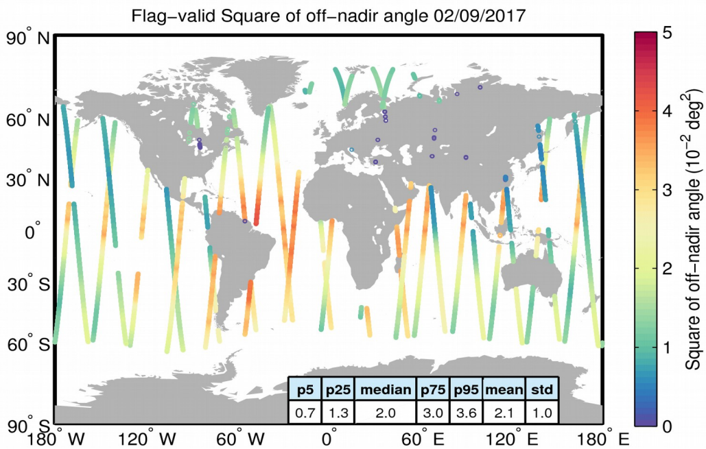
Figure 37. Geographical distribution of flag-valid mispointing data over oceans and lakes for 02/09/2017. The statistical values shown in the table refer to the mispointing in 10^{-2} deg 2 and are calculated over all measurements shown in the figure.
