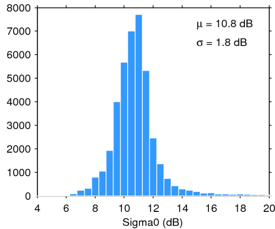
Figure 25. Histogram of flag-valid sigma0 over oceans and lakes for 02/09/2017. The mean ( \mu ) and standard deviation ( \sigma ) are also shown. Note that values outside [4 20] dB are excluded from the histogram for the sake of readability but not from the computation of \mu and \sigma .
