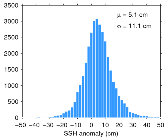
Figure 11. Histogram of science-valid SSH anomaly over oceans and lakes for 01/09/2017. The mean ( \mu ) and standard deviation ( \sigma ) are also shown. Note that values outside [-50 50] cm are excluded from the histogram for the sake of readability but not from the computation of \mu and \sigma .
