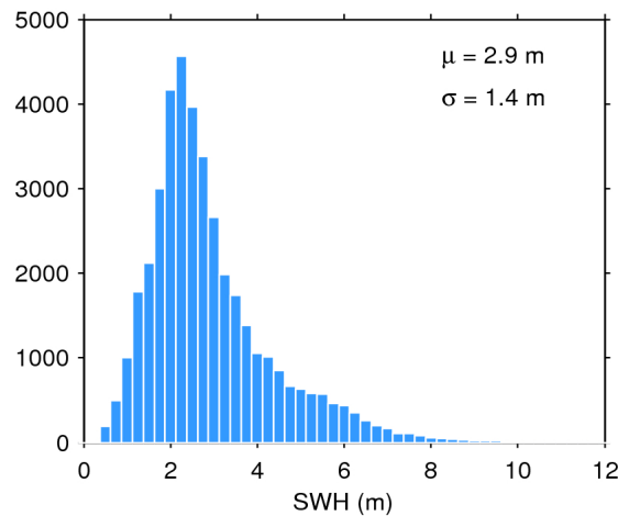
Figure 20. Histogram of science-valid SWH over oceans and lakes for 01/09/2017. The mean ( \mu ) and standard deviation ( \sigma ) are also shown. Note that values larger than 12 m are excluded from the histogram for the sake of readability but not from the computation of \mu and \sigma .
