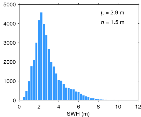
Figure 17. Histogram of flag-valid SWH over oceans and lakes for 01/09/2017. The mean ( \mu ) and standard deviation ( \sigma ) are also shown. Note that values larger than 12 m are excluded from the histogram for the sake of readability but not from the computation of \mu and \sigma .
