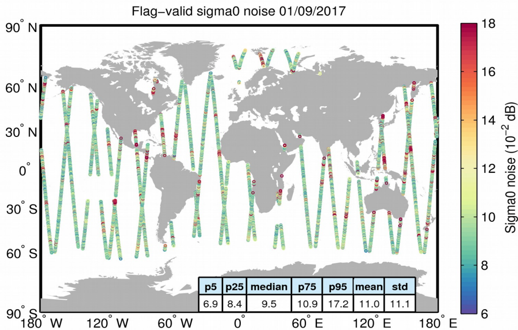
Figure 26. Geographical distribution of flag-valid 20-Hz sigma0 measurement noise over oceans and lakes for 01/09/2017. The statistical values shown in the table refer to the sigma0 noise and are calculated over all measurements shown in the figure.
