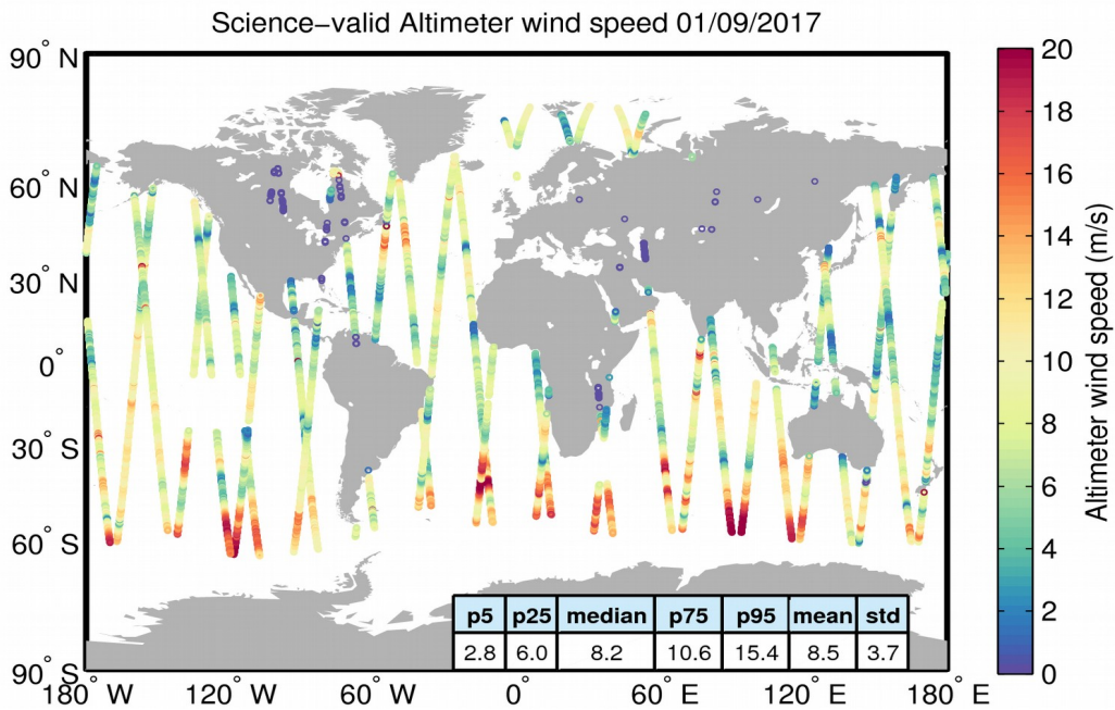
Figure 34. Geographical distribution of science-valid wind data over oceans and lakes for 01/09/2017. The statistical values shown in the table refer to the wind in m/s and are calculated over all measurements shown in the figure. Gray circles denote records that have been rejected based on the editing criteria described in Table 5.
