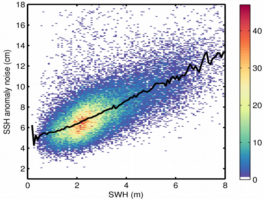
Figure 9. 2D histogram showing flag-valid SSH anomaly noise as a function of SWH for 01/09/2017. The black line denotes the median SSH anomaly noise as a function of SWH.
