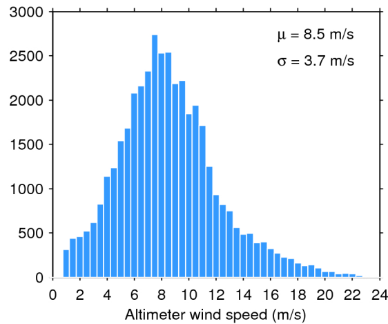
Figure 33. Histogram of flag-valid wind over oceans and lakes for 01/09/2017. The mean ( \mu ) and standard deviation ( \sigma ) are also shown. Note that values larger than 24 m/s are excluded from the histogram for the sake of readability but not from the computation of \mu and \sigma .
