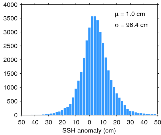
Figure 7. Histogram of flag-valid SSH anomaly over oceans and lakes for 01/09/2017. The mean ( \mu ) and standard deviation ( \sigma ) are also shown. Note that values outside [-50 50] cm are excluded from the histogram for the sake of readability but not from the computation of \mu and \sigma .
