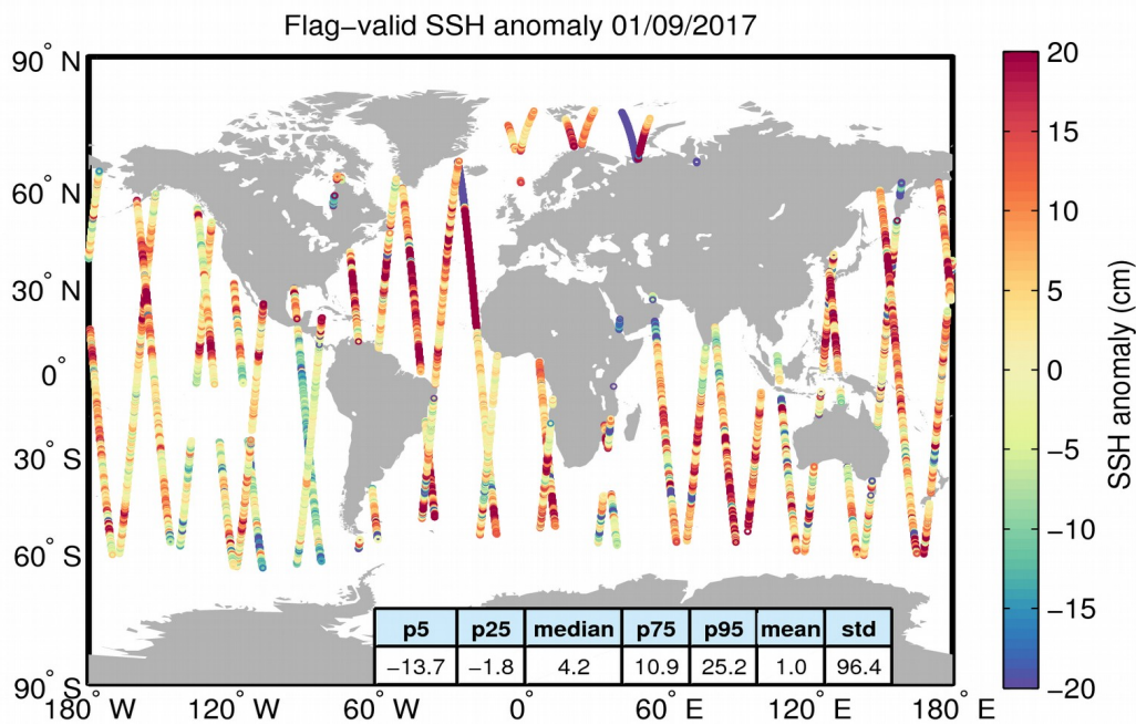
Figure 5. Geographical distribution of flag-valid 1-Hz SSH anomaly data over oceans and lakes for 01/09/2017. The statistical values shown in the table refer to the SSH anomaly in cm and are calculated over all measurements shown in the figure.
