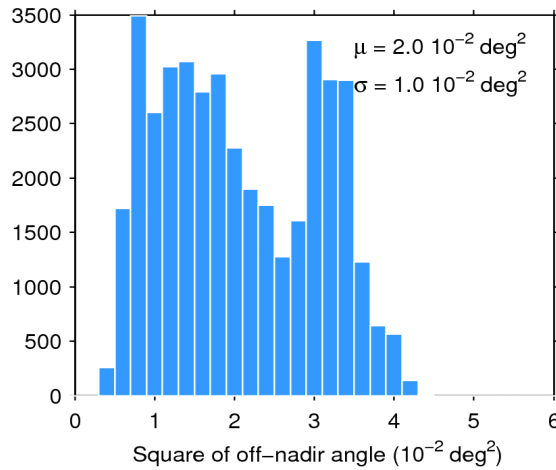
Figure 39. Histogram of flag-valid mispointing over oceans and lakes for 01/09/2017. The mean ( \mu ) and standard deviation ( \sigma ) are also shown. Note that values larger than 6 \cdot 10^{-2} \text{ deg}^2 are excluded from the histogram for the sake of readability but not from the computation of \mu and \sigma .
