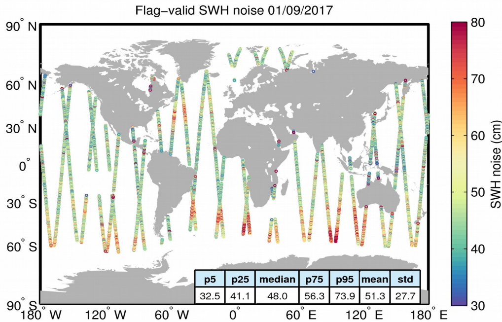
Figure 18. Geographical distribution of flag-valid 20-Hz SWH measurement noise over oceans and lakes for 01/09/2017. The statistical values shown in the table refer to the SWH noise and are calculated over all measurements shown in the figure.
