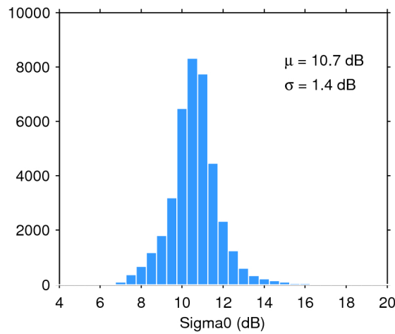
Figure 28. Histogram of science-valid sigma0 over oceans and lakes for 01/09/2017. The mean ( \mu ) and standard deviation ( \sigma ) are also shown. Note that values outside [4 20] dB are excluded from the histogram for the sake of readability but not from the computation of \mu and \sigma .
