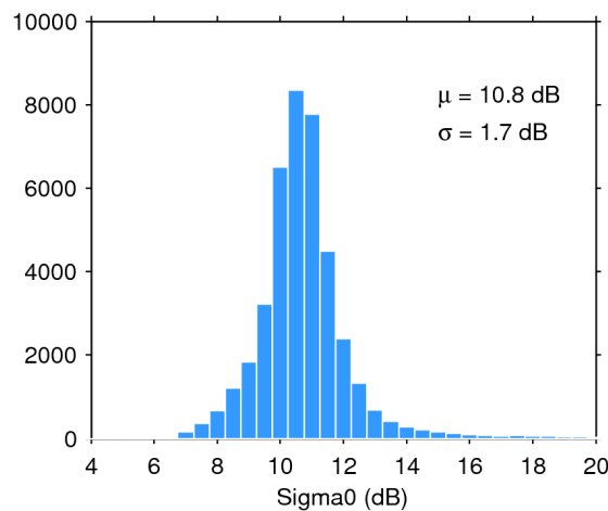
Figure 25. Histogram of flag-valid sigma0 over oceans and lakes for 01/09/2017. The mean ( \mu ) and standard deviation ( \sigma ) are also shown. Note that values outside [4 20] dB are excluded from the histogram for the sake of readability but not from the computation of \mu and \sigma .
