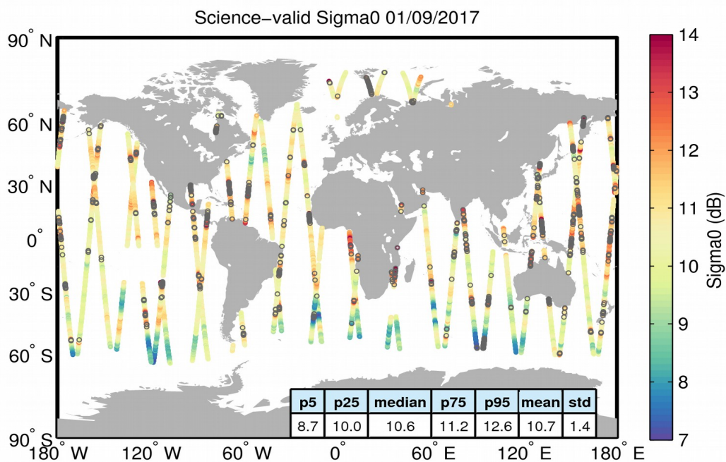
Figure 27. Geographical distribution of science-valid sigma0 data over oceans and lakes for 01/09/2017. The statistical values shown in the table refer to the sigma0 in dB and are calculated over all measurements shown in the figure. Gray circles denote records that have been rejected based on the editing criteria described in Table 4.
