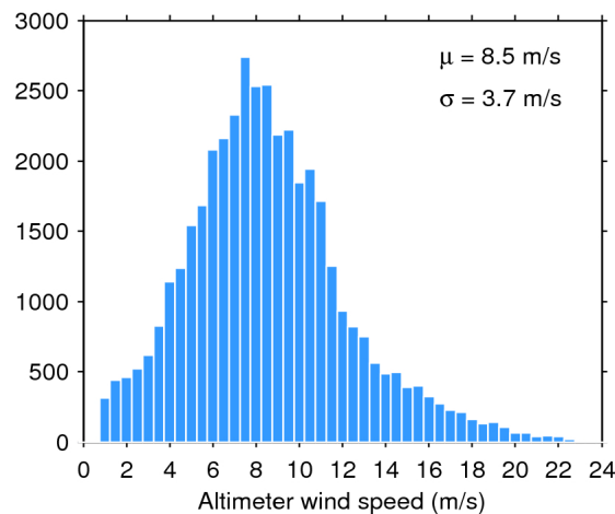
Figure 35. Histogram of science-valid wind over oceans and lakes for 01/09/2017. The mean ( \mu ) and standard deviation ( \sigma ) are also shown. Note that values larger than 24 m/s are excluded from the histogram for the sake of readability but not from the computation of \mu and \sigma .
