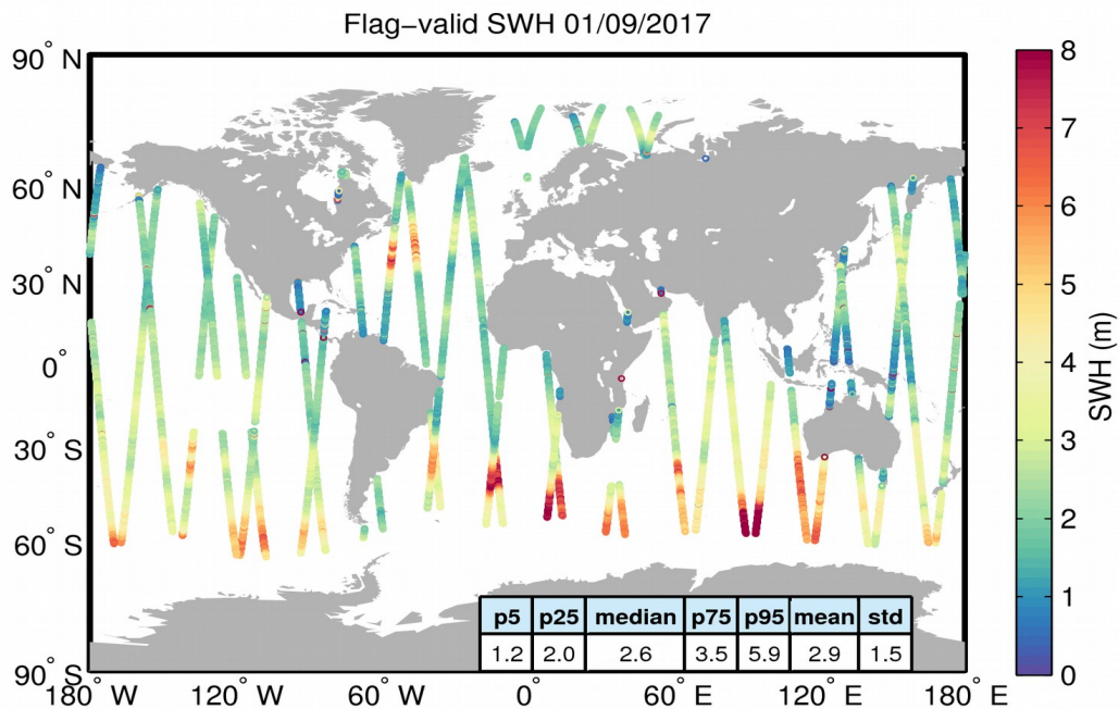
Figure 15. Geographical distribution of flag-valid SWH data over oceans and lakes for 01/09/2017. The statistical values shown in the table refer to the SWH in m and are calculated over all measurements shown in the figure.
