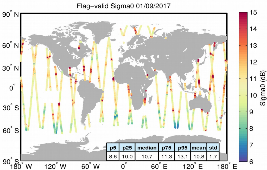
Figure 23. Geographical distribution of flag-valid sigma0 data over oceans and lakes for 01/09/2017. The statistical values shown in the table refer to the sigma0 in dB and are calculated over all measurements shown in the figure.
