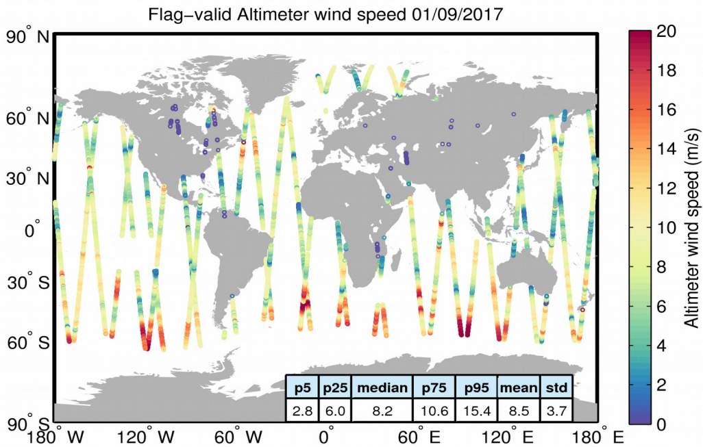
Figure 31. Geographical distribution of flag-valid wind data over oceans and lakes for 01/09/2017. The statistical values shown in the table refer to the wind in m/s and are calculated over all measurements shown in the figure.
