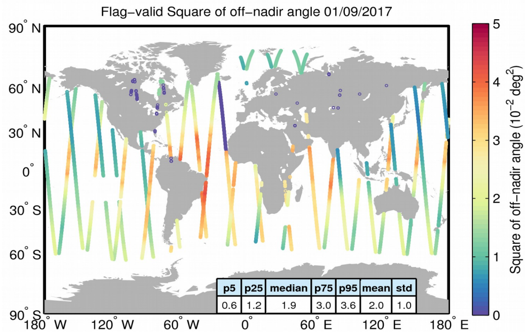
Figure 37. Geographical distribution of flag-valid mispointing data over oceans and lakes for 01/09/2017. The statistical values shown in the table refer to the mispointing in 10^{-2} \text{ deg}^2 and are calculated over all measurements shown in the figure.
