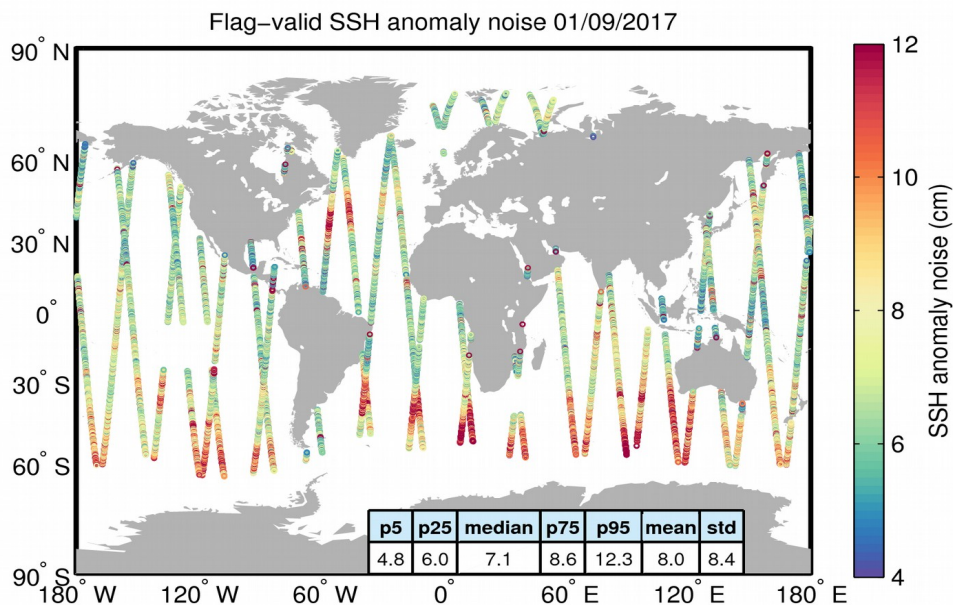
Figure 8. Geographical distribution of flag-valid 20-Hz SSH anomaly measurement noise over oceans and lakes for 01/09/2017. The statistical values shown in the table refer to the SSH anomaly noise and are calculated over all measurements shown in the figure.
