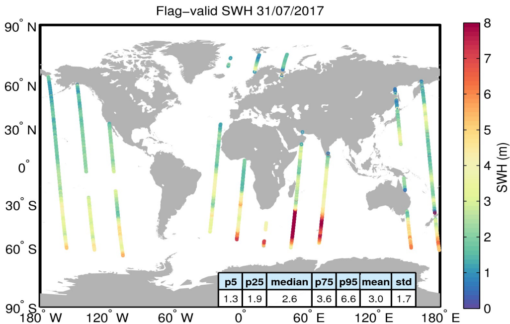
Figure 15. Geographical distribution of flag-valid SWH data over oceans and lakes for 31/07/2017. The statistical values shown in the table refer to the SWH in m and are calculated over all measurements shown in the figure.
