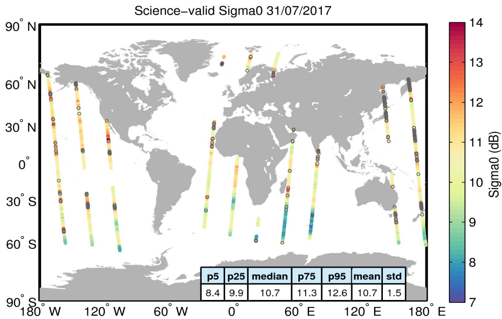
Figure 27. Geographical distribution of science-valid sigma0 data over oceans and lakes for 31/07/2017. The statistical values shown in the table refer to the sigma0 in dB and are calculated over all measurements shown in the figure. Gray circles denote records that have been rejected based on the editing criteria described in Table 4.
