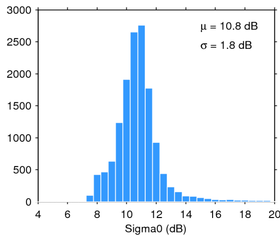
Figure 25. Histogram of flag-valid sigma0 over oceans and lakes for 31/07/2017. The mean ( \mu ) and standard deviation ( \sigma ) are also shown. Note that values outside [4 20] dB are excluded from the histogram for the sake of readability but not from the computation of \mu and \sigma .
