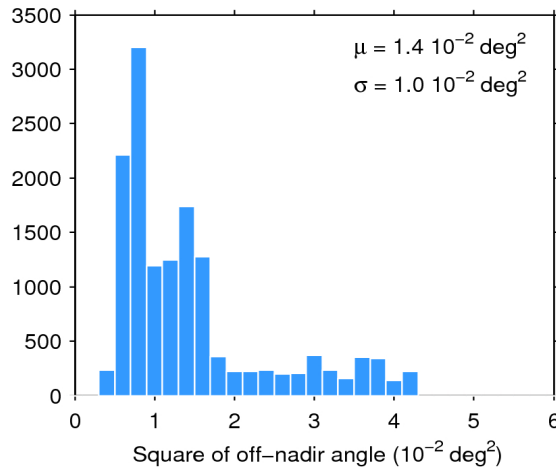
Figure 39. Histogram of flag-valid mispointing over oceans and lakes for 31/07/2017. The mean ( \mu ) and standard deviation ( \sigma ) are also shown. Note that values larger than 6 \cdot 10^{-2} \text{ deg}^2 are excluded from the histogram for the sake of readability but not from the computation of \mu and \sigma .
