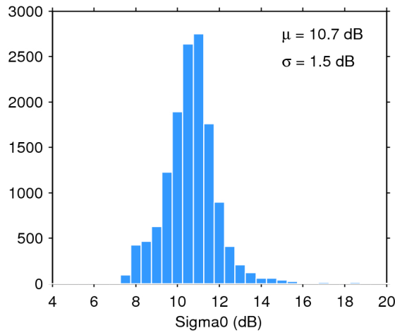
Figure 28. Histogram of science-valid sigma0 over oceans and lakes for 31/07/2017. The mean ( \mu ) and standard deviation ( \sigma ) are also shown. Note that values outside [4 20] dB are excluded from the histogram for the sake of readability but not from the computation of \mu and \sigma .
