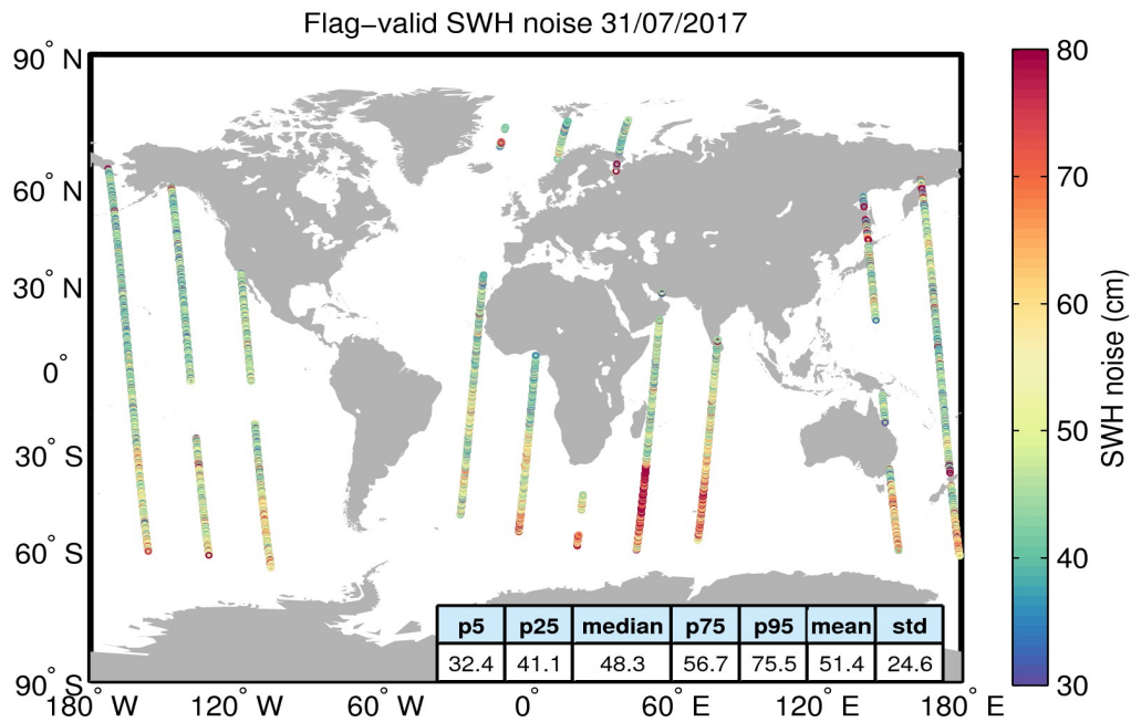
Figure 18. Geographical distribution of flag-valid 20-Hz SWH measurement noise over oceans and lakes for 31/07/2017. The statistical values shown in the table refer to the SWH noise and are calculated over all measurements shown in the figure.
