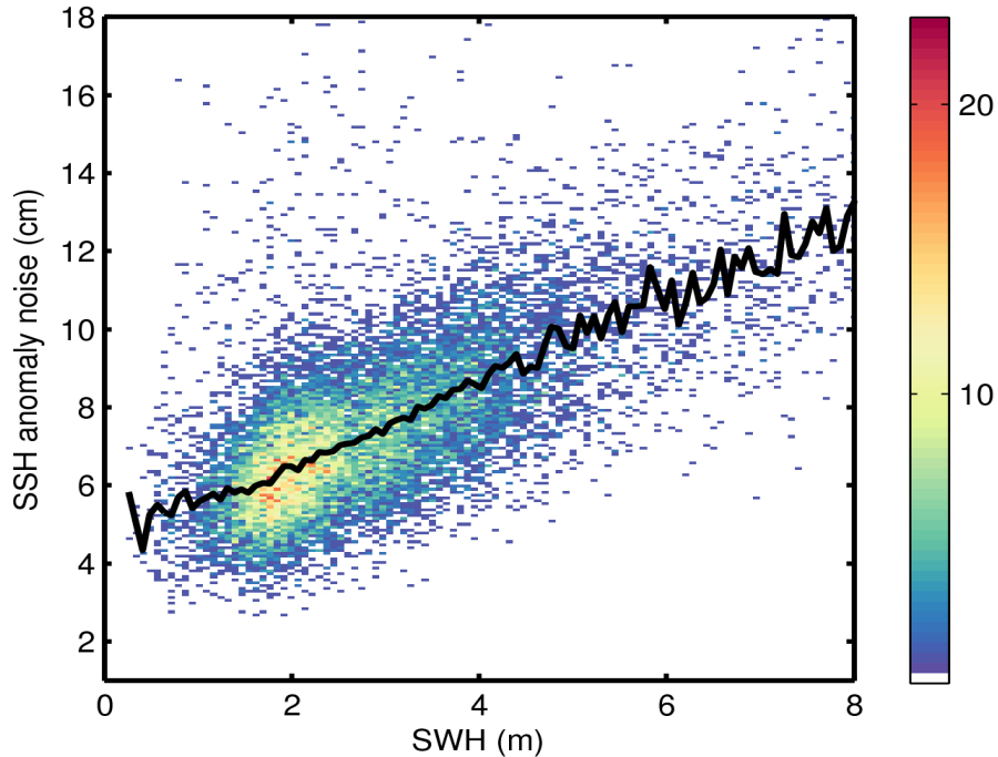
Figure 9. 2D histogram showing flag-valid SSH anomaly noise as a function of SWH for 31/07/2017. The black line denotes the median SSH anomaly noise as a function of SWH.
