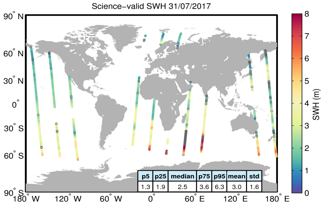
Figure 19. Geographical distribution of science-valid SWH data over oceans and lakes for 31/07/2017. The statistical values shown in the table refer to the SWH in m and are calculated over all measurements shown in the figure. Gray circles denote records that have been rejected based on the editing criteria described in Table 3.
