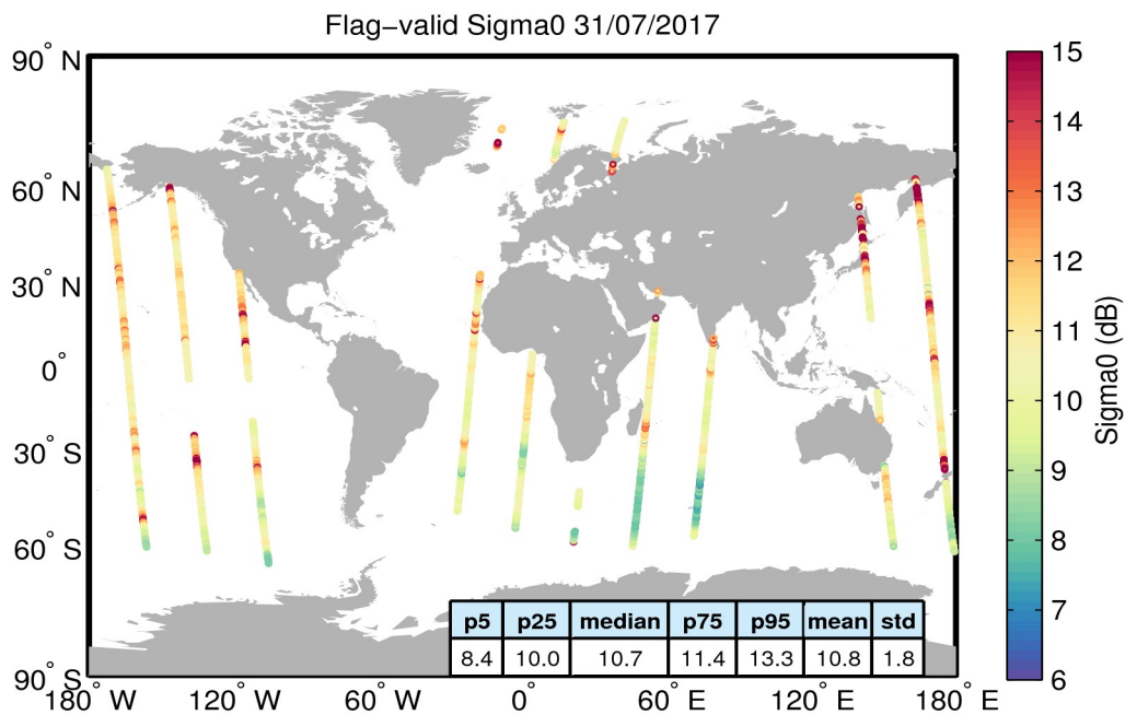
Figure 23. Geographical distribution of flag-valid sigma0 data over oceans and lakes for 31/07/2017. The statistical values shown in the table refer to the sigma0 in dB and are calculated over all measurements shown in the figure.
