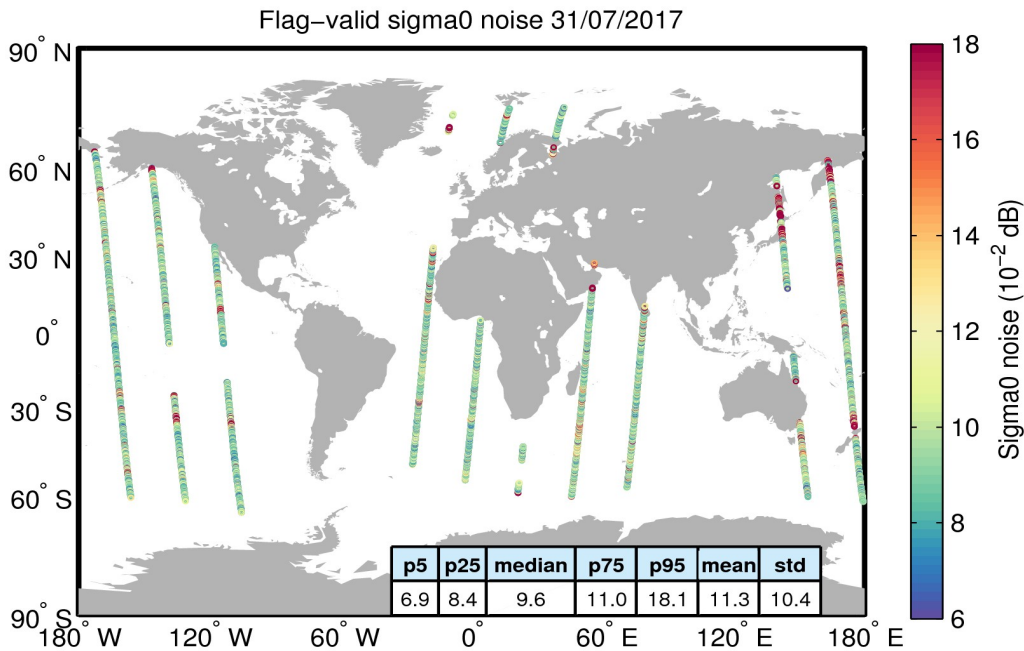
Figure 26. Geographical distribution of flag-valid 20-Hz sigma0 measurement noise over oceans and lakes for 31/07/2017. The statistical values shown in the table refer to the sigma0 noise and are calculated over all measurements shown in the figure.
