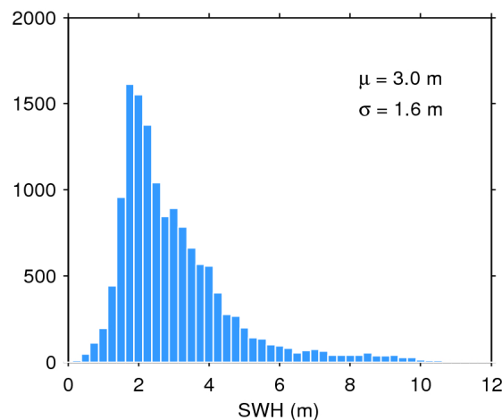
Figure 20. Histogram of science-valid SWH over oceans and lakes for 31/07/2017. The mean ( \mu ) and standard deviation ( \sigma ) are also shown. Note that values larger than 12 m are excluded from the histogram for the sake of readability but not from the computation of \mu and \sigma .
