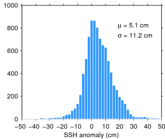
Figure 11. Histogram of science-valid SSH anomaly over oceans and lakes for 31/07/2017. The mean ( \mu ) and standard deviation ( \sigma ) are also shown. Note that values outside [-50 50] cm are excluded from the histogram for the sake of readability but not from the computation of \mu and \sigma .
