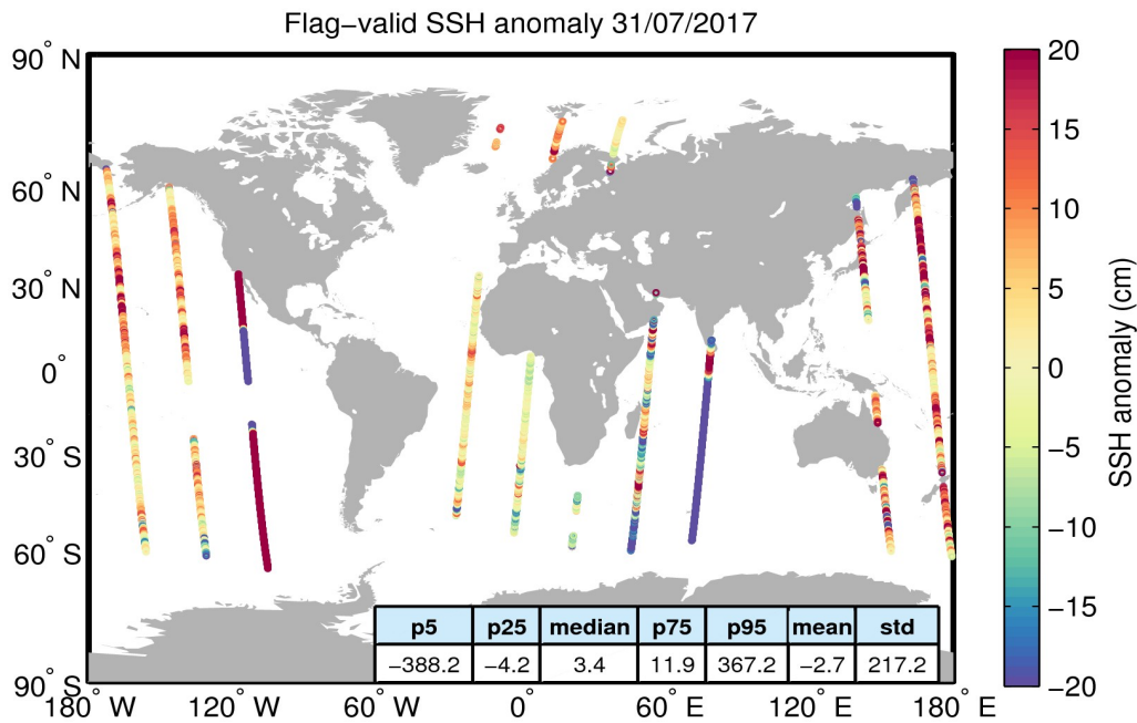
Figure 5. Geographical distribution of flag-valid 1-Hz SSH anomaly data over oceans and lakes for 31/07/2017. The statistical values shown in the table refer to the SSH anomaly in cm and are calculated over all measurements shown in the figure.
