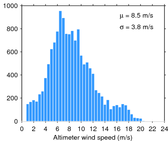
Figure 35. Histogram of science-valid wind over oceans and lakes for 31/07/2017. The mean ( \mu ) and standard deviation ( \sigma ) are also shown. Note that values larger than 24 m/s are excluded from the histogram for the sake of readability but not from the computation of \mu and \sigma .
