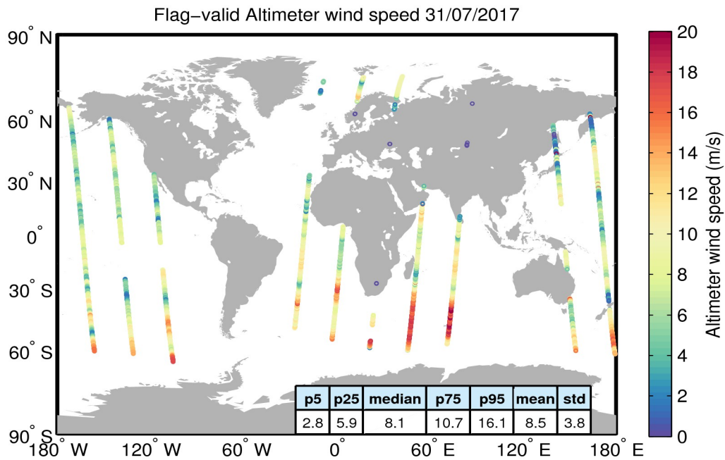
Figure 31. Geographical distribution of flag-valid wind data over oceans and lakes for 31/07/2017. The statistical values shown in the table refer to the wind in m/s and are calculated over all measurements shown in the figure.
