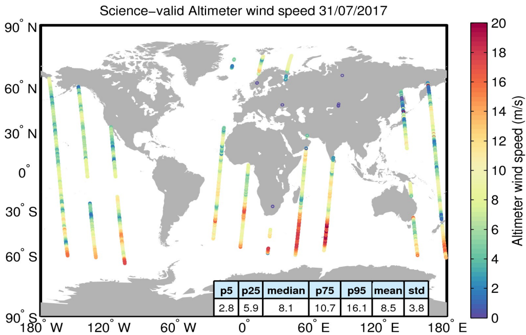
Figure 34. Geographical distribution of science-valid wind data over oceans and lakes for 31/07/2017. The statistical values shown in the table refer to the wind in m/s and are calculated over all measurements shown in the figure. Gray circles denote records that have been rejected based on the editing criteria described in Table 5.
