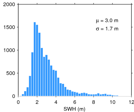
Figure 17. Histogram of flag-valid SWH over oceans and lakes for 31/07/2017. The mean ( \mu ) and standard deviation ( \sigma ) are also shown. Note that values larger than 12 m are excluded from the histogram for the sake of readability but not from the computation of \mu and \sigma .
