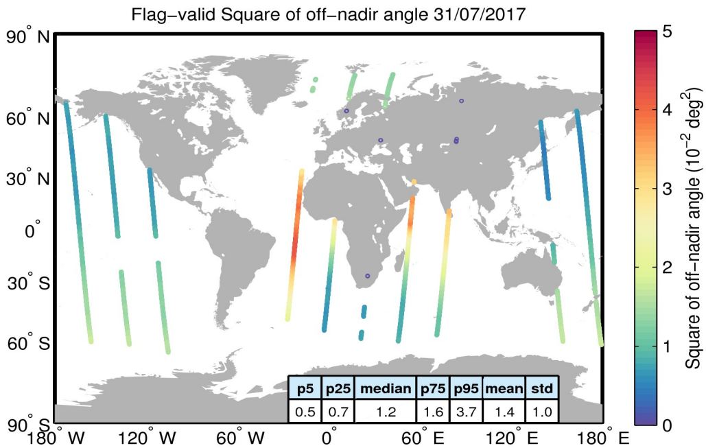
Figure 37. Geographical distribution of flag-valid mispointing data over oceans and lakes for 31/07/2017. The statistical values shown in the table refer to the mispointing in 10^{-2} deg 2 and are calculated over all measurements shown in the figure.
