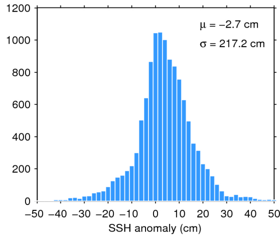
Figure 7. Histogram of flag-valid SSH anomaly over oceans and lakes for 31/07/2017. The mean ( \mu ) and standard deviation ( \sigma ) are also shown. Note that values outside [-50 50] cm are excluded from the histogram for the sake of readability but not from the computation of \mu and \sigma .
