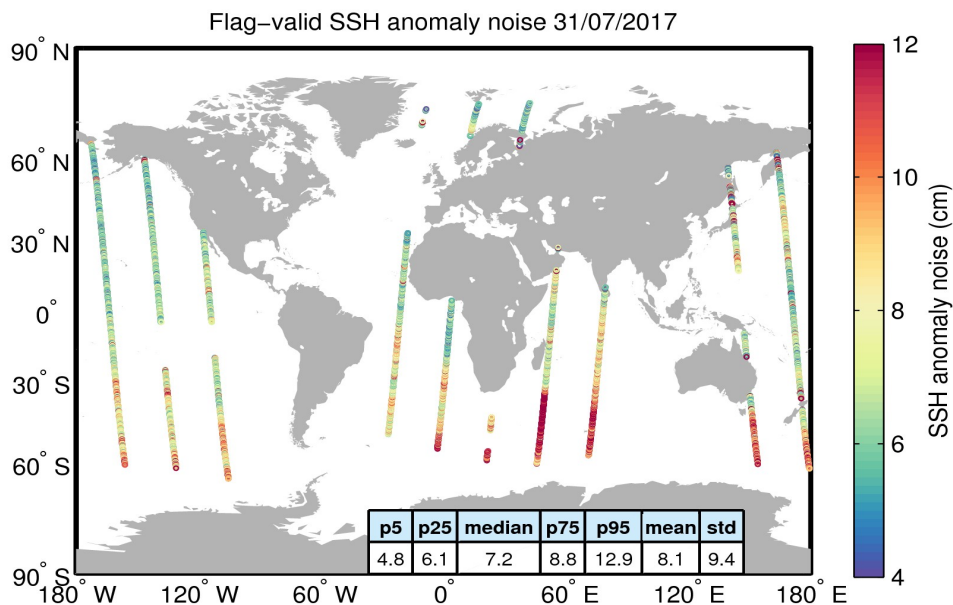
Figure 8. Geographical distribution of flag-valid 20-Hz SSH anomaly measurement noise over oceans and lakes for 31/07/2017. The statistical values shown in the table refer to the SSH anomaly noise and are calculated over all measurements shown in the figure.
