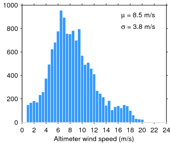
Figure 33. Histogram of flag-valid wind over oceans and lakes for 31/07/2017. The mean ( \mu ) and standard deviation ( \sigma ) are also shown. Note that values larger than 24 m/s are excluded from the histogram for the sake of readability but not from the computation of \mu and \sigma .
