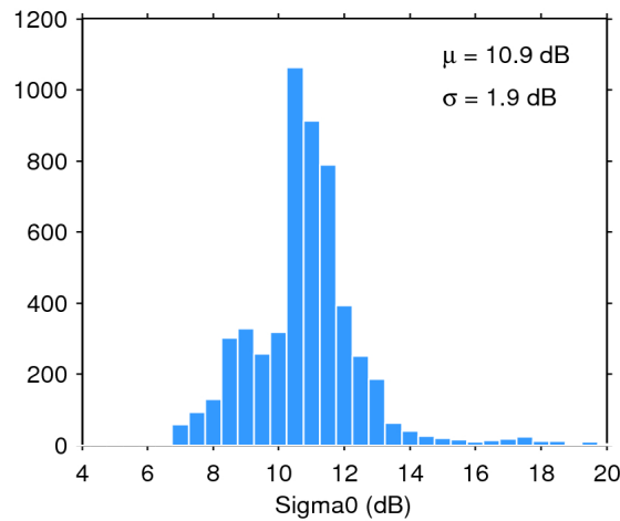
Figure 28. Histogram of science-valid sigma0 over oceans and lakes for 30/07/2017. The mean ( \mu ) and standard deviation ( \sigma ) are also shown. Note that values outside [4 20] dB are excluded from the histogram for the sake of readability but not from the computation of \mu and \sigma .
