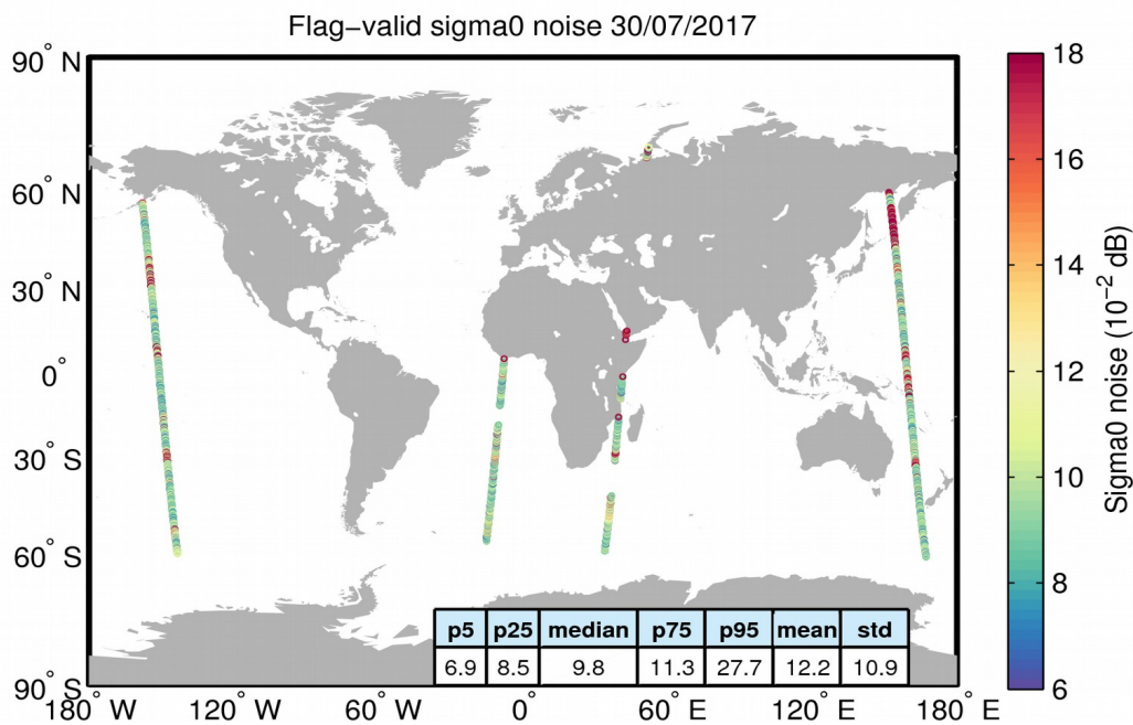
Figure 26. Geographical distribution of flag-valid 20-Hz sigma0 measurement noise over oceans and lakes for 30/07/2017. The statistical values shown in the table refer to the sigma0 noise and are calculated over all measurements shown in the figure.
