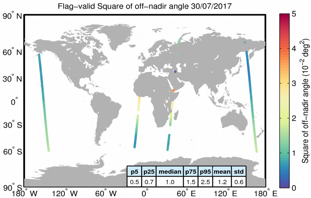
Figure 37. Geographical distribution of flag-valid mispointing data over oceans and lakes for 30/07/2017. The statistical values shown in the table refer to the mispointing in 10^{-2} deg 2 and are calculated over all measurements shown in the figure.
