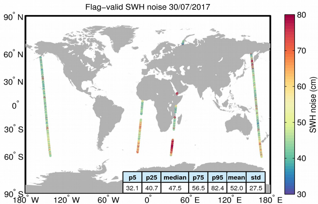
Figure 18. Geographical distribution of flag-valid 20-Hz SWH measurement noise over oceans and lakes for 30/07/2017. The statistical values shown in the table refer to the SWH noise and are calculated over all measurements shown in the figure.
