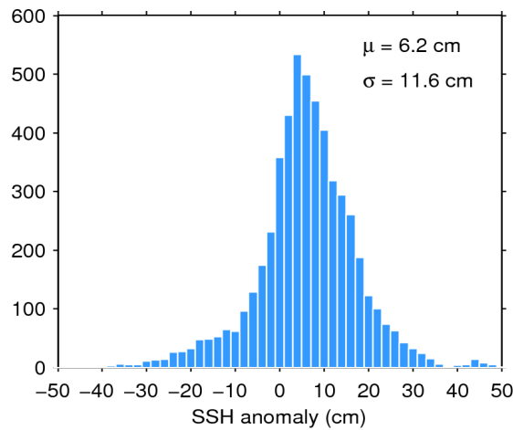
Figure 11. Histogram of science-valid SSH anomaly over oceans and lakes for 30/07/2017. The mean ( \mu ) and standard deviation ( \sigma ) are also shown. Note that values outside [-50 50] cm are excluded from the histogram for the sake of readability but not from the computation of \mu and \sigma .
