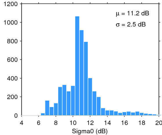
Figure 25. Histogram of flag-valid sigma0 over oceans and lakes for 30/07/2017. The mean ( \mu ) and standard deviation ( \sigma ) are also shown. Note that values outside [4 20] dB are excluded from the histogram for the sake of readability but not from the computation of \mu and \sigma .
