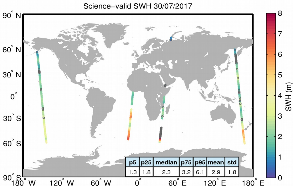
Figure 19. Geographical distribution of science-valid SWH data over oceans and lakes for 30/07/2017. The statistical values shown in the table refer to the SWH in m and are calculated over all measurements shown in the figure. Gray circles denote records that have been rejected based on the editing criteria described in Table 3.
