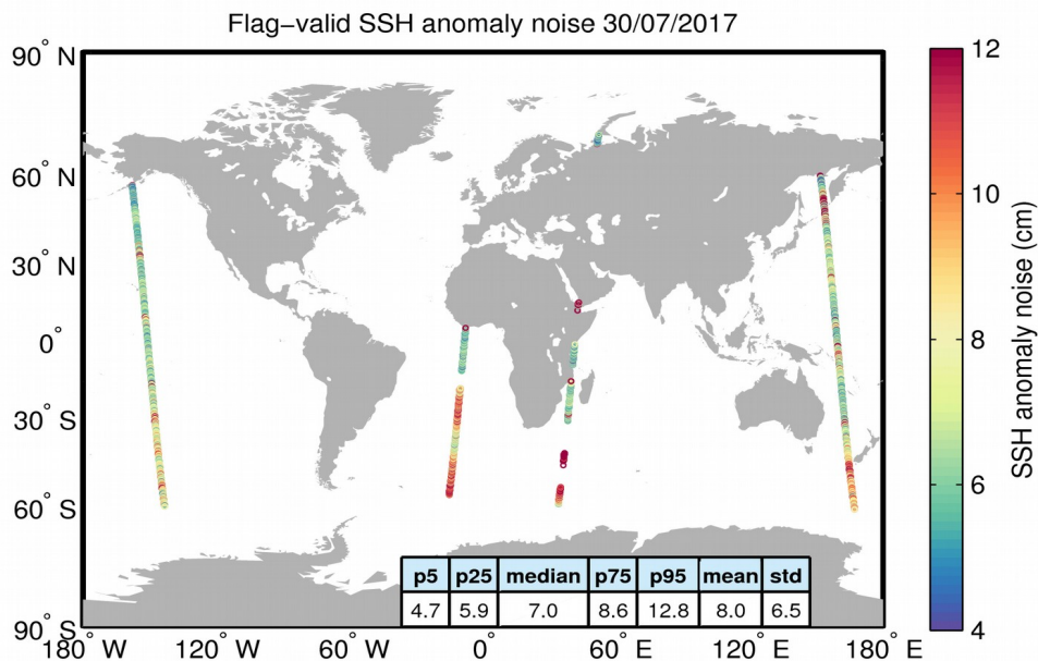
Figure 8. Geographical distribution of flag-valid 20-Hz SSH anomaly measurement noise over oceans and lakes for 30/07/2017. The statistical values shown in the table refer to the SSH anomaly noise and are calculated over all measurements shown in the figure.
