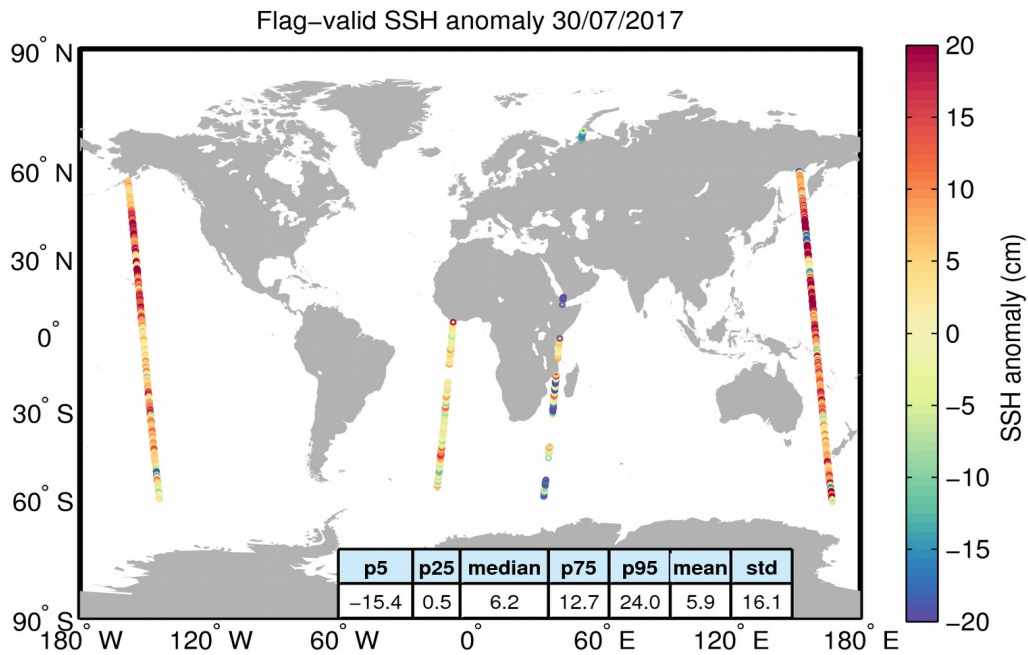
Figure 5. Geographical distribution of flag-valid 1-Hz SSH anomaly data over oceans and lakes for 30/07/2017. The statistical values shown in the table refer to the SSH anomaly in cm and are calculated over all measurements shown in the figure.
