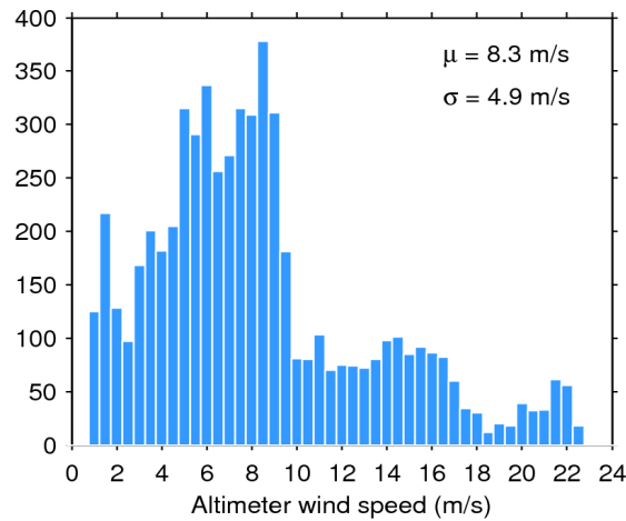
Figure 33. Histogram of flag-valid wind over oceans and lakes for 30/07/2017. The mean ( \mu ) and standard deviation ( \sigma ) are also shown. Note that values larger than 24 m/s are excluded from the histogram for the sake of readability but not from the computation of \mu and \sigma .
