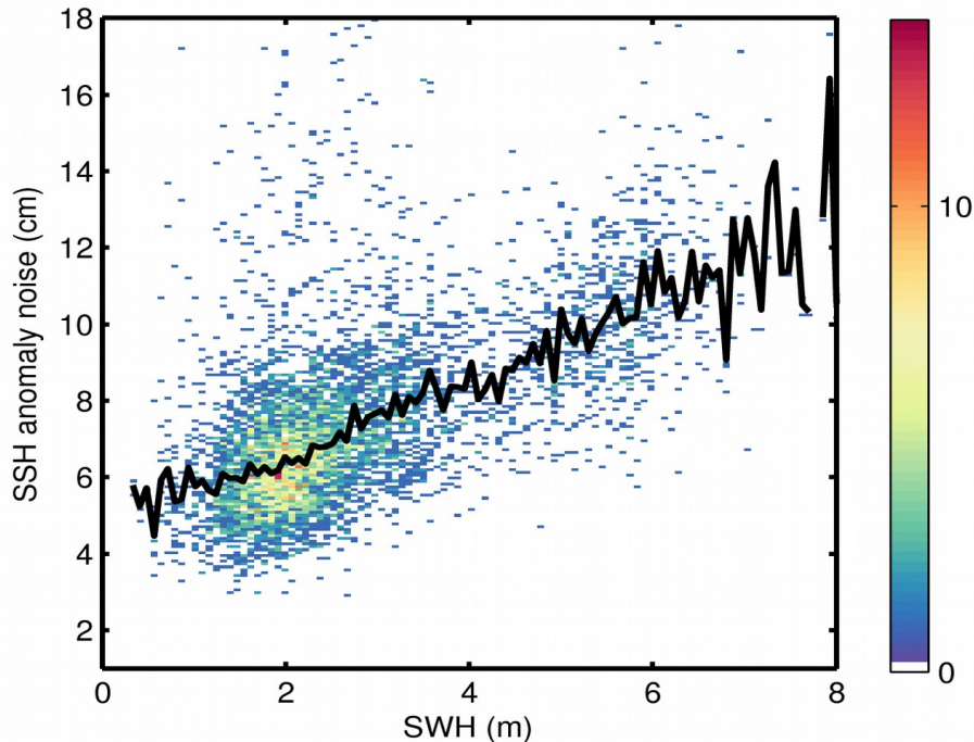
Figure 9. 2D histogram showing flag-valid SSH anomaly noise as a function of SWH for 30/07/2017. The black line denotes the median SSH anomaly noise as a function of SWH.
