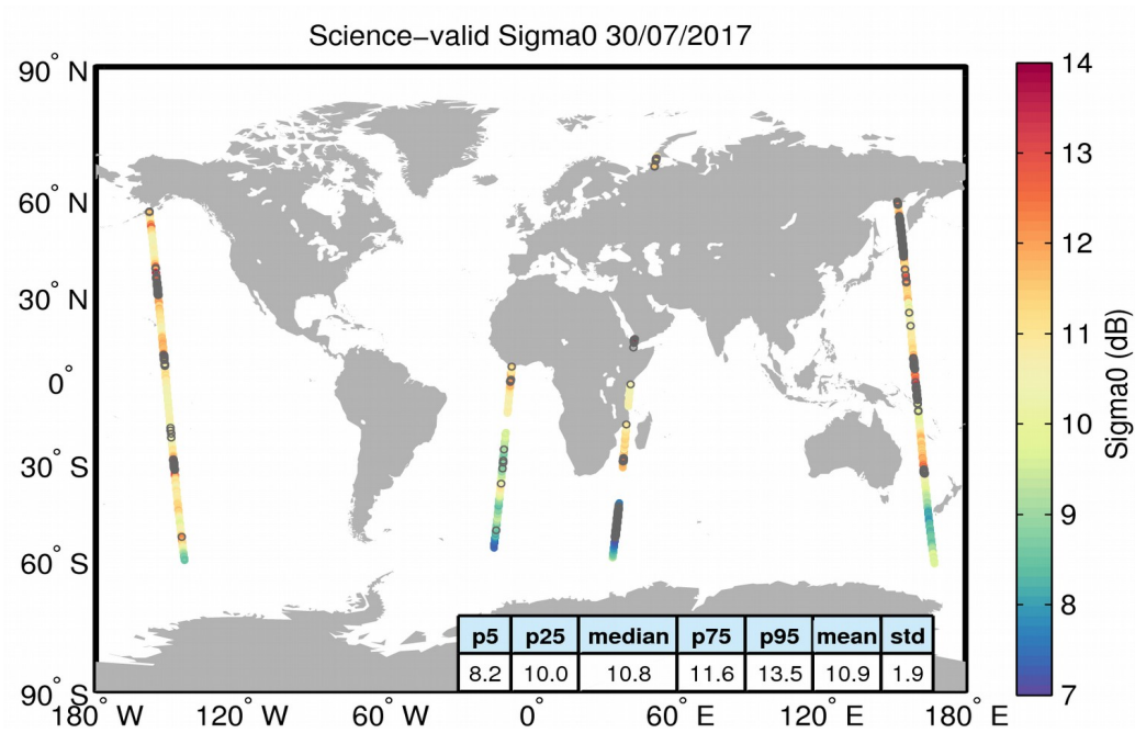
Figure 27. Geographical distribution of science-valid sigma0 data over oceans and lakes for 30/07/2017. The statistical values shown in the table refer to the sigma0 in dB and are calculated over all measurements shown in the figure. Gray circles denote records that have been rejected based on the editing criteria described in Table 4.
