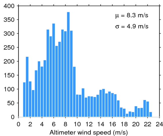
Figure 35. Histogram of science-valid wind over oceans and lakes for 30/07/2017. The mean ( \mu ) and standard deviation ( \sigma ) are also shown. Note that values larger than 24 m/s are excluded from the histogram for the sake of readability but not from the computation of \mu and \sigma .
