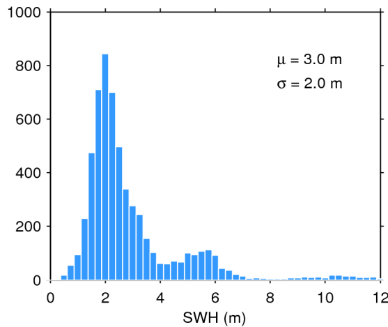
Figure 17. Histogram of flag-valid SWH over oceans and lakes for 30/07/2017. The mean ( \mu ) and standard deviation ( \sigma ) are also shown. Note that values larger than 12 m are excluded from the histogram for the sake of readability but not from the computation of \mu and \sigma .
