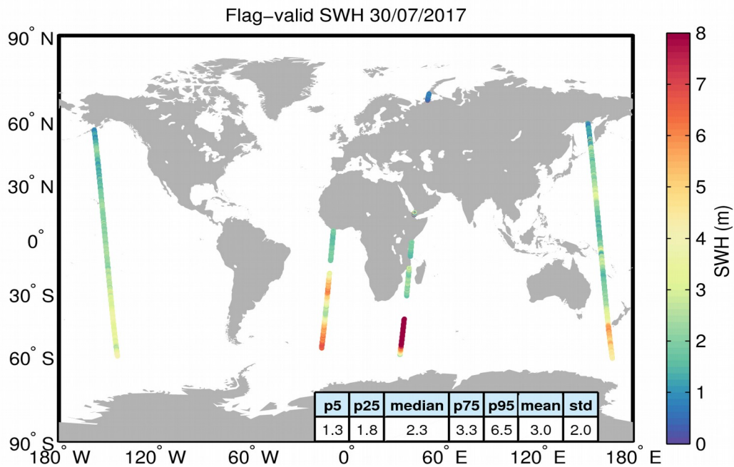
Figure 15. Geographical distribution of flag-valid SWH data over oceans and lakes for 30/07/2017. The statistical values shown in the table refer to the SWH in m and are calculated over all measurements shown in the figure.
