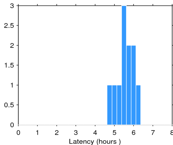
Figure 2. Histogram of the data latency for 30/07/2017. The y-axis denotes the number of files that are made available with a delay of x-hours with respect to the mean time of the records stored in the file.
