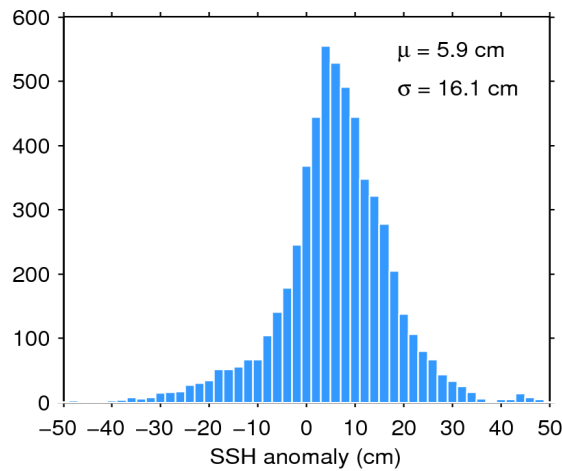
Figure 7. Histogram of flag-valid SSH anomaly over oceans and lakes for 30/07/2017. The mean ( \mu ) and standard deviation ( \sigma ) are also shown. Note that values outside [-50 50] cm are excluded from the histogram for the sake of readability but not from the computation of \mu and \sigma .
