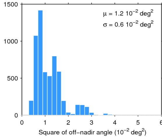
Figure 39. Histogram of flag-valid mispointing over oceans and lakes for 30/07/2017. The mean ( \mu ) and standard deviation ( \sigma ) are also shown. Note that values larger than 6 \cdot 10^{-2} \text{ deg}^2 are excluded from the histogram for the sake of readability but not from the computation of \mu and \sigma .
