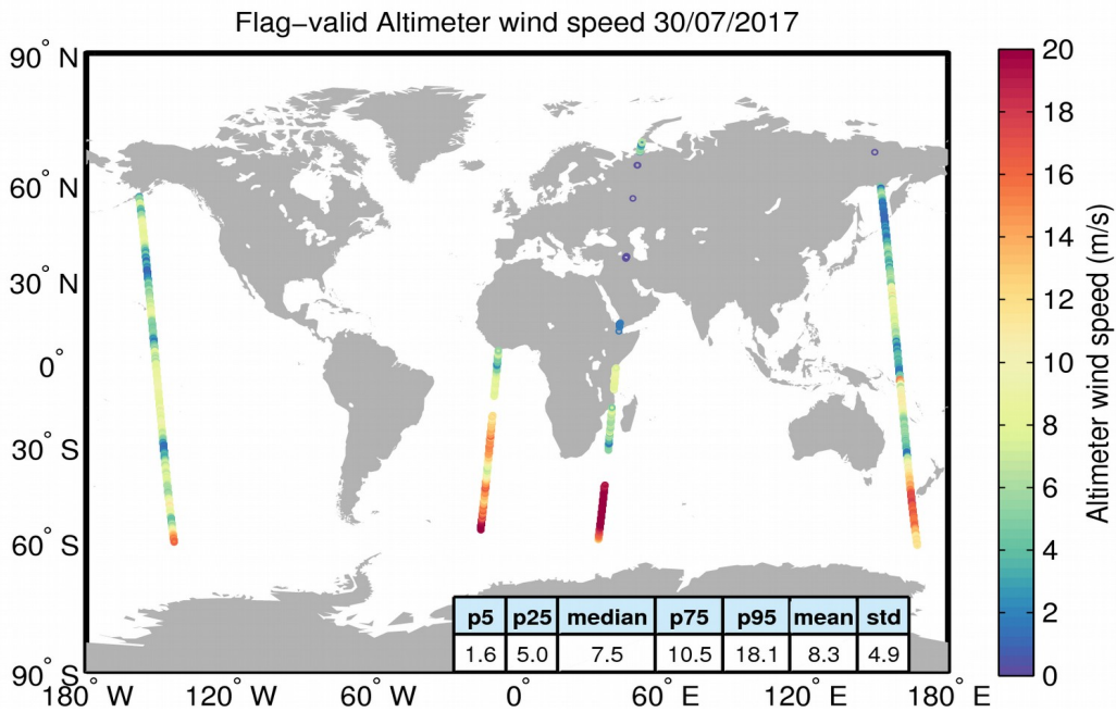
Figure 31. Geographical distribution of flag-valid wind data over oceans and lakes for 30/07/2017. The statistical values shown in the table refer to the wind in m/s and are calculated over all measurements shown in the figure.
