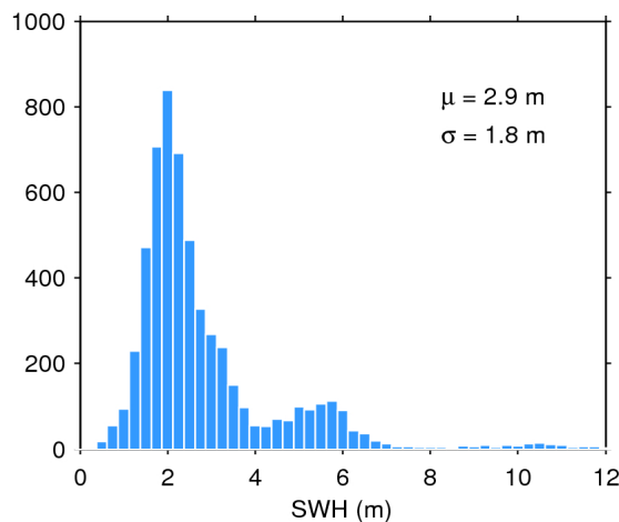
Figure 20. Histogram of science-valid SWH over oceans and lakes for 30/07/2017. The mean ( \mu ) and standard deviation ( \sigma ) are also shown. Note that values larger than 12 m are excluded from the histogram for the sake of readability but not from the computation of \mu and \sigma .
