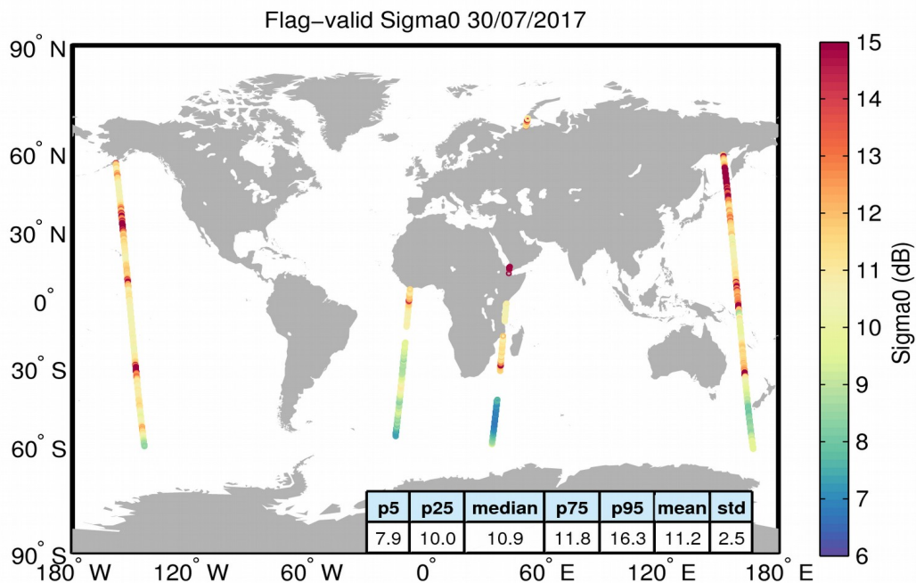
Figure 23. Geographical distribution of flag-valid sigma0 data over oceans and lakes for 30/07/2017. The statistical values shown in the table refer to the sigma0 in dB and are calculated over all measurements shown in the figure.
