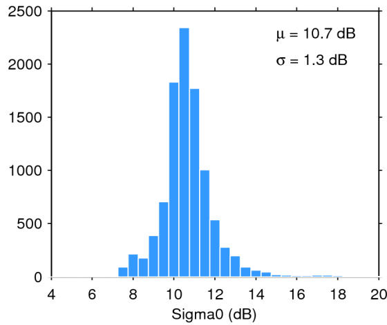
Figure 28. Histogram of science-valid sigma0 over oceans and lakes for 28/07/2017. The mean ( \mu ) and standard deviation ( \sigma ) are also shown. Note that values outside [4 20] dB are excluded from the histogram for the sake of readability but not from the computation of \mu and \sigma .
