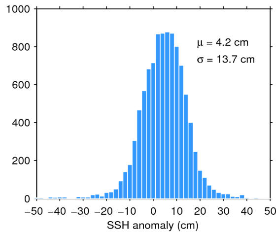
Figure 7. Histogram of flag-valid SSH anomaly over oceans and lakes for 28/07/2017. The mean ( \mu ) and standard deviation ( \sigma ) are also shown. Note that values outside [-50 50] cm are excluded from the histogram for the sake of readability but not from the computation of \mu and \sigma .
