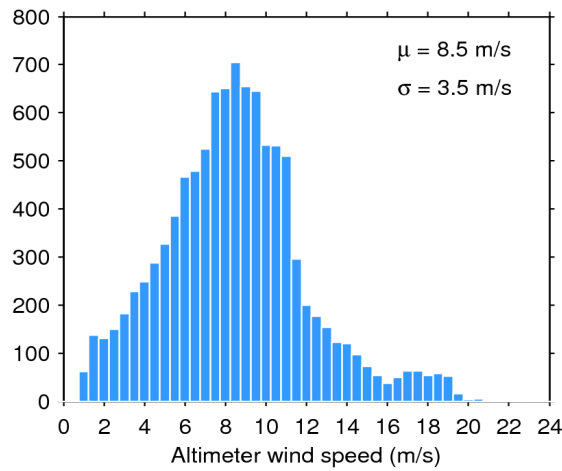
Figure 33. Histogram of flag-valid wind over oceans and lakes for 28/07/2017. The mean ( \mu ) and standard deviation ( \sigma ) are also shown. Note that values larger than 24 m/s are excluded from the histogram for the sake of readability but not from the computation of \mu and \sigma .
