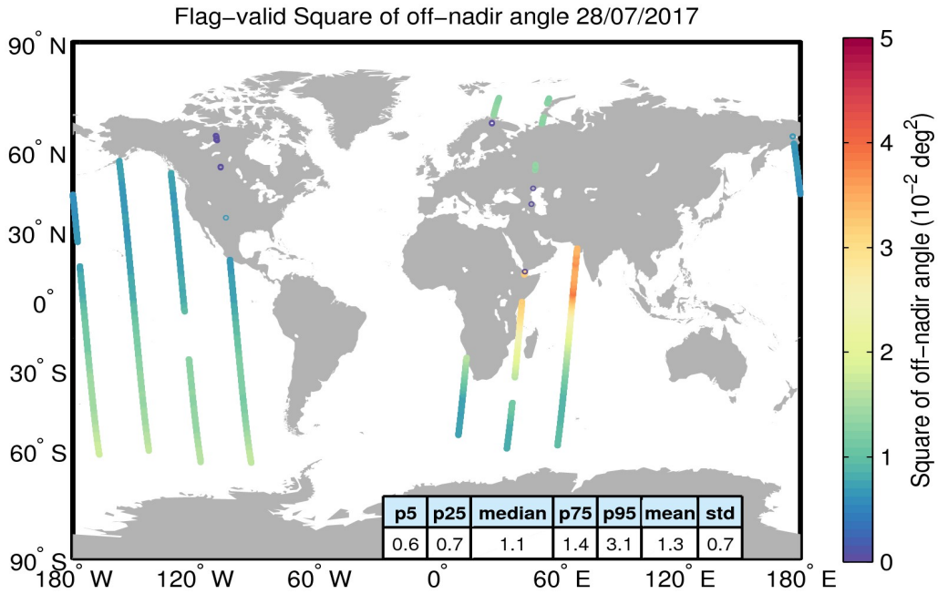
Figure 37. Geographical distribution of flag-valid mispointing data over oceans and lakes for 28/07/2017. The statistical values shown in the table refer to the mispointing in 10^{-2} deg 2 and are calculated over all measurements shown in the figure.
