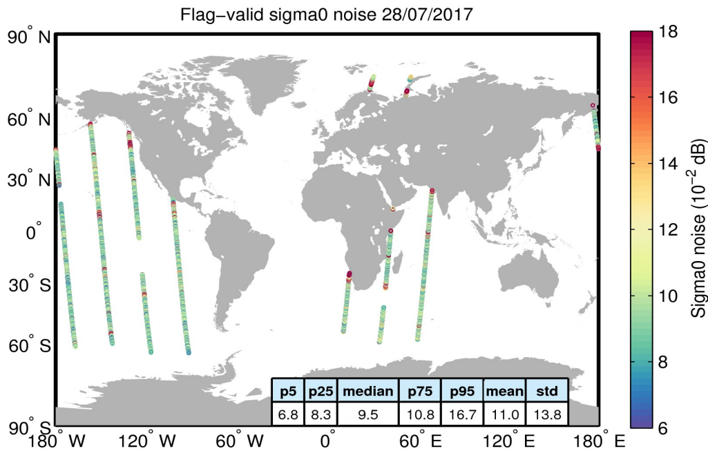
Figure 26. Geographical distribution of flag-valid 20-Hz sigma0 measurement noise over oceans and lakes for 28/07/2017. The statistical values shown in the table refer to the sigma0 noise and are calculated over all measurements shown in the figure.
