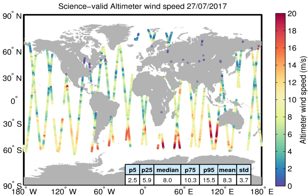
Figure 34. Geographical distribution of science-valid wind data over oceans and lakes for 27/07/2017. The statistical values shown in the table refer to the wind in m/s and are calculated over all measurements shown in the figure. Gray circles denote records that have been rejected based on the editing criteria described in Table 5.
