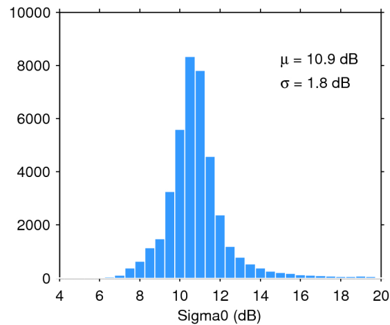
Figure 25. Histogram of flag-valid sigma0 over oceans and lakes for 27/07/2017. The mean ( \mu ) and standard deviation ( \sigma ) are also shown. Note that values outside [4 20] dB are excluded from the histogram for the sake of readability but not from the computation of \mu and \sigma .
