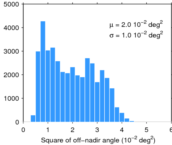
Figure 39. Histogram of flag-valid mispointing over oceans and lakes for 27/07/2017. The mean ( \mu ) and standard deviation ( \sigma ) are also shown. Note that values larger than 6 \cdot 10^{-2} \text{ deg}^2 are excluded from the histogram for the sake of readability but not from the computation of \mu and \sigma .
