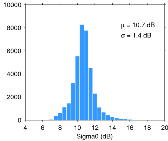
Figure 28. Histogram of science-valid sigma0 over oceans and lakes for 27/07/2017. The mean ( \mu ) and standard deviation ( \sigma ) are also shown. Note that values outside [4 20] dB are excluded from the histogram for the sake of readability but not from the computation of \mu and \sigma .
