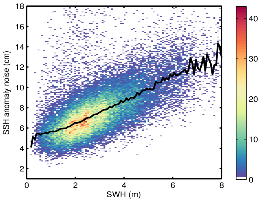
Figure 9. 2D histogram showing flag-valid SSH anomaly noise as a function of SWH for 27/07/2017. The black line denotes the median SSH anomaly noise as a function of SWH.
