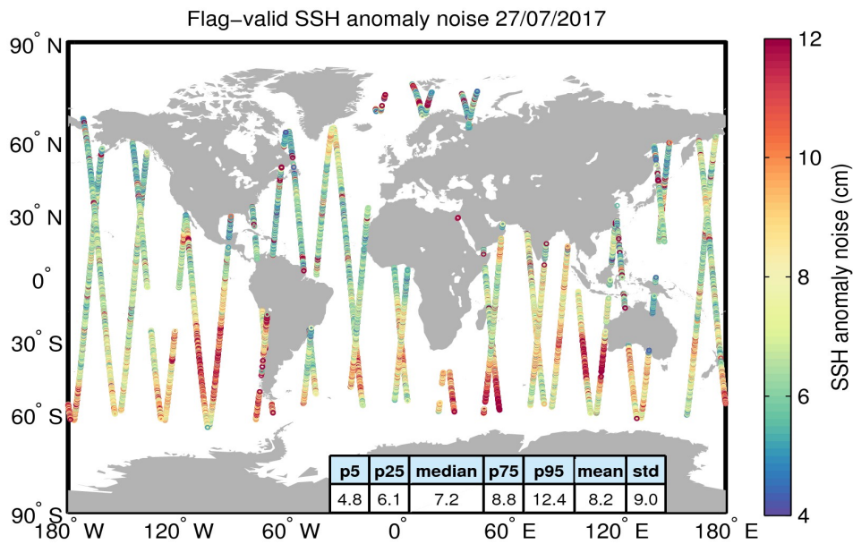
Figure 8. Geographical distribution of flag-valid 20-Hz SSH anomaly measurement noise over oceans and lakes for 27/07/2017. The statistical values shown in the table refer to the SSH anomaly noise and are calculated over all measurements shown in the figure.
