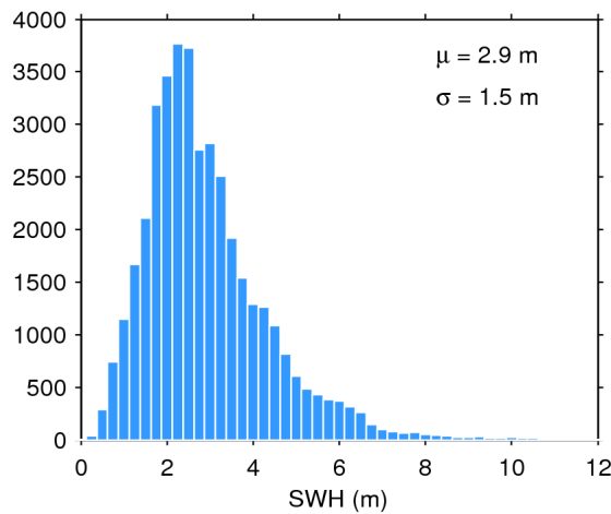
Figure 17. Histogram of flag-valid SWH over oceans and lakes for 27/07/2017. The mean ( \mu ) and standard deviation ( \sigma ) are also shown. Note that values larger than 12 m are excluded from the histogram for the sake of readability but not from the computation of \mu and \sigma .
