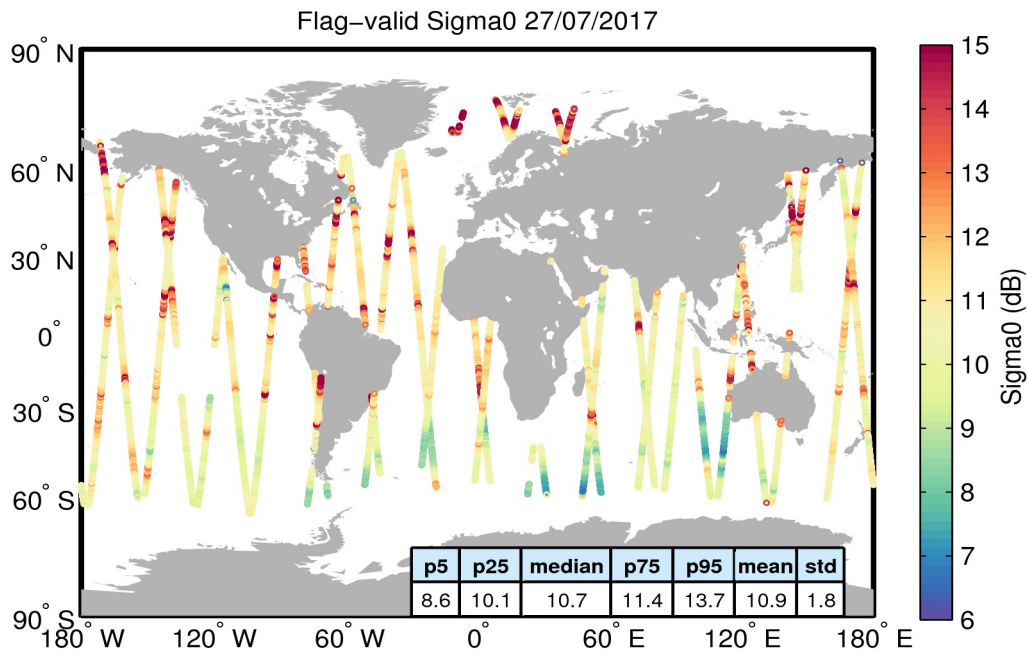
Figure 23. Geographical distribution of flag-valid sigma0 data over oceans and lakes for 27/07/2017. The statistical values shown in the table refer to the sigma0 in dB and are calculated over all measurements shown in the figure.
