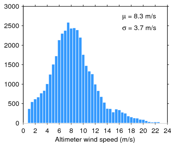
Figure 35. Histogram of science-valid wind over oceans and lakes for 27/07/2017. The mean ( \mu ) and standard deviation ( \sigma ) are also shown. Note that values larger than 24 m/s are excluded from the histogram for the sake of readability but not from the computation of \mu and \sigma .
