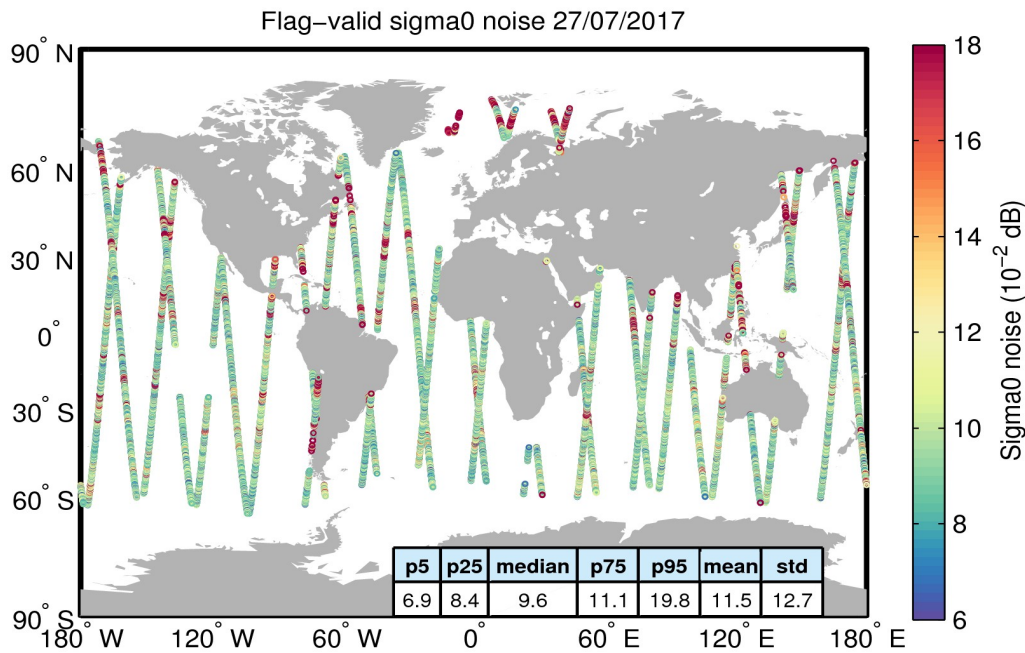
Figure 26. Geographical distribution of flag-valid 20-Hz sigma0 measurement noise over oceans and lakes for 27/07/2017. The statistical values shown in the table refer to the sigma0 noise and are calculated over all measurements shown in the figure.
