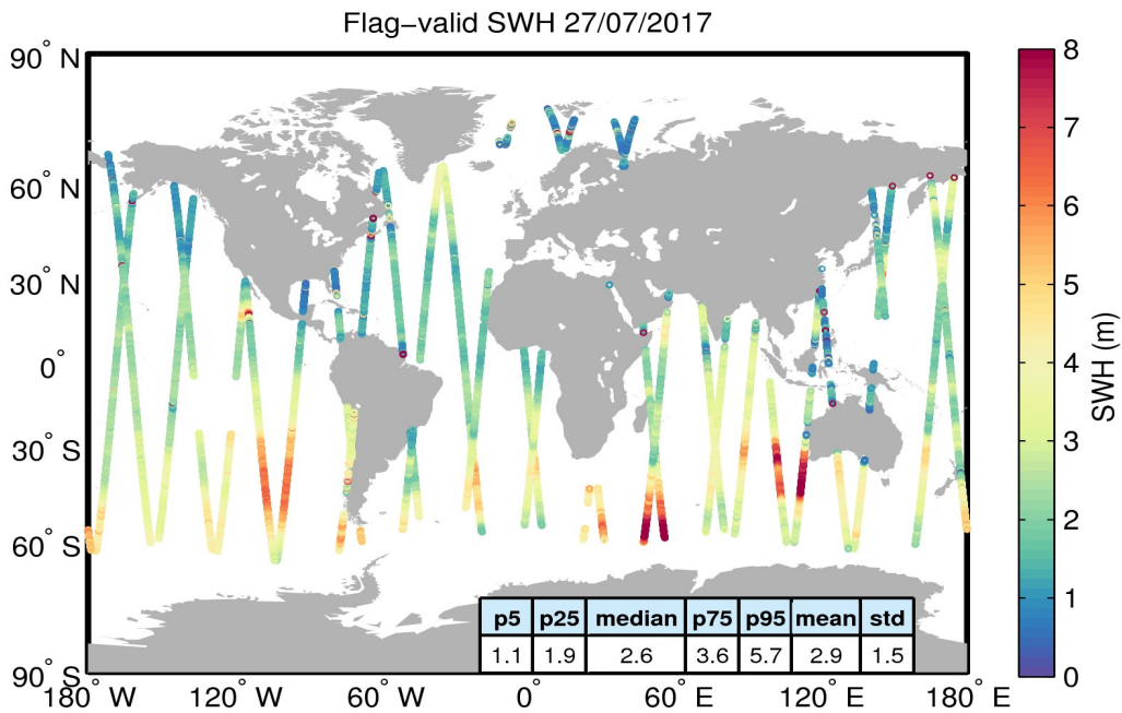
Figure 15. Geographical distribution of flag-valid SWH data over oceans and lakes for 27/07/2017. The statistical values shown in the table refer to the SWH in m and are calculated over all measurements shown in the figure.
