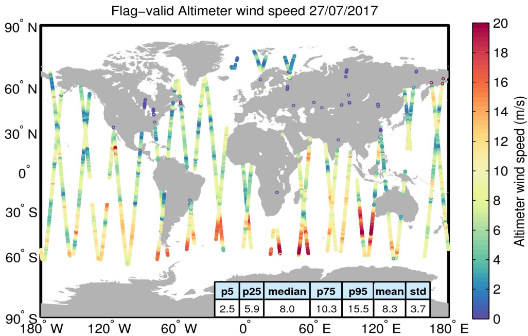
Figure 31. Geographical distribution of flag-valid wind data over oceans and lakes for 27/07/2017. The statistical values shown in the table refer to the wind in m/s and are calculated over all measurements shown in the figure.
