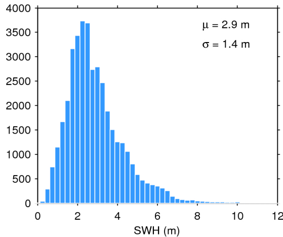
Figure 20. Histogram of science-valid SWH over oceans and lakes for 27/07/2017. The mean ( \mu ) and standard deviation ( \sigma ) are also shown. Note that values larger than 12 m are excluded from the histogram for the sake of readability but not from the computation of \mu and \sigma .
