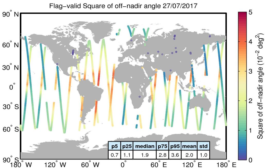
Figure 37. Geographical distribution of flag-valid mispointing data over oceans and lakes for 27/07/2017. The statistical values shown in the table refer to the mispointing in 10^{-2} deg 2 and are calculated over all measurements shown in the figure.
