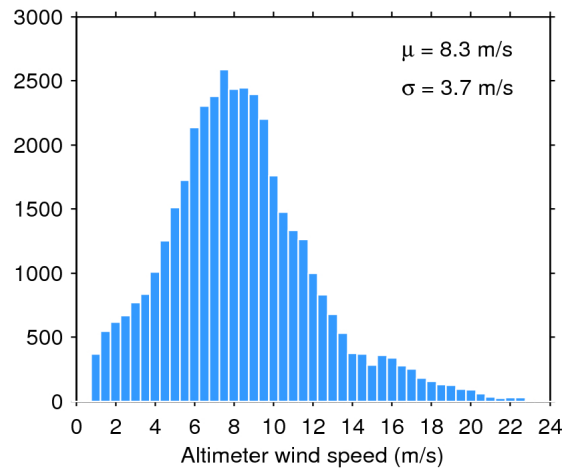
Figure 33. Histogram of flag-valid wind over oceans and lakes for 27/07/2017. The mean ( \mu ) and standard deviation ( \sigma ) are also shown. Note that values larger than 24 m/s are excluded from the histogram for the sake of readability but not from the computation of \mu and \sigma .
