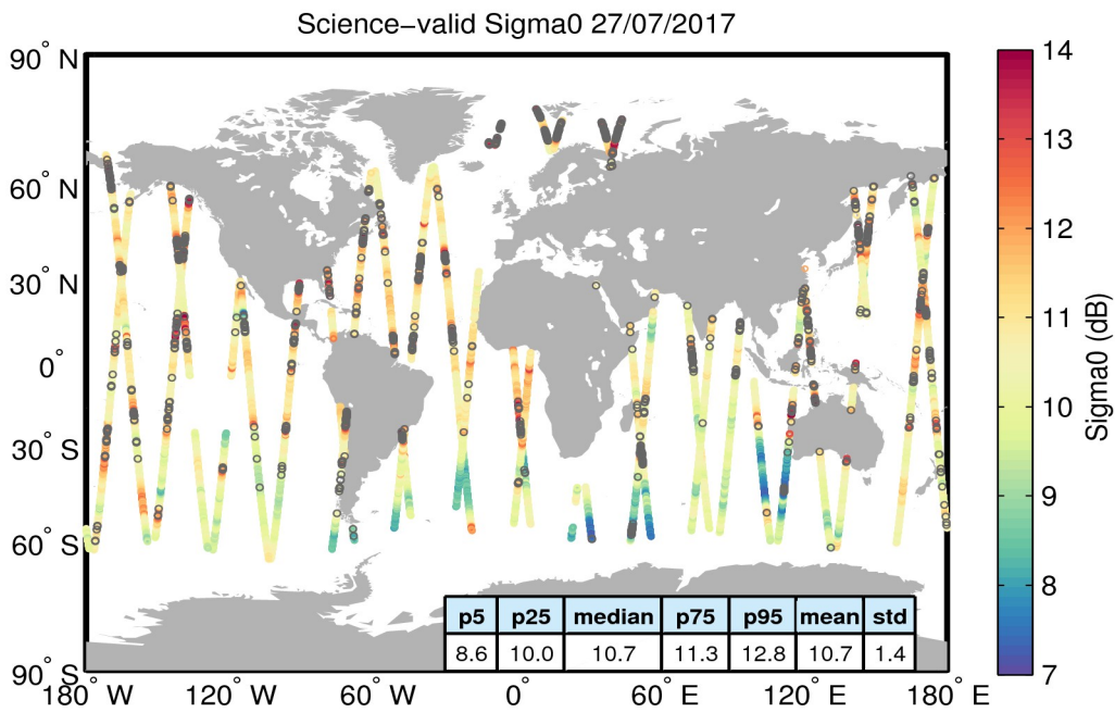
Figure 27. Geographical distribution of science-valid sigma0 data over oceans and lakes for 27/07/2017. The statistical values shown in the table refer to the sigma0 in dB and are calculated over all measurements shown in the figure. Gray circles denote records that have been rejected based on the editing criteria described in Table 4.
