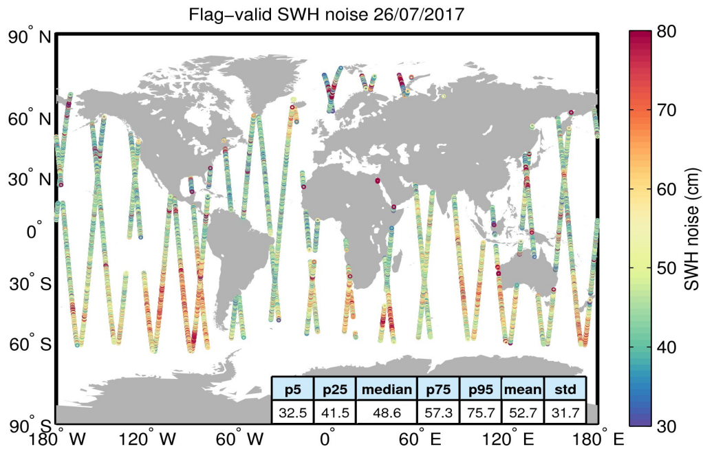
Figure 18. Geographical distribution of flag-valid 20-Hz SWH measurement noise over oceans and lakes for 26/07/2017. The statistical values shown in the table refer to the SWH noise and are calculated over all measurements shown in the figure.
