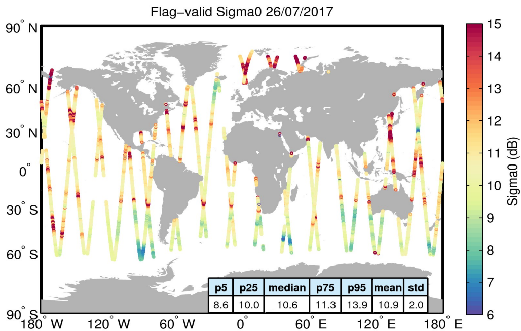
Figure 23. Geographical distribution of flag-valid sigma0 data over oceans and lakes for 26/07/2017. The statistical values shown in the table refer to the sigma0 in dB and are calculated over all measurements shown in the figure.
