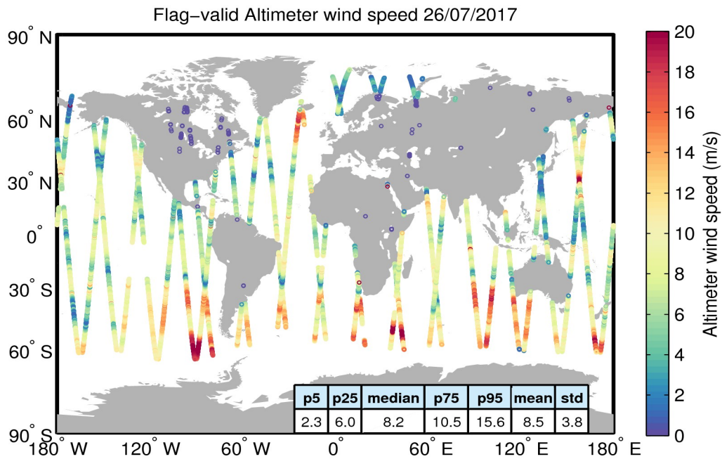
Figure 31. Geographical distribution of flag-valid wind data over oceans and lakes for 26/07/2017. The statistical values shown in the table refer to the wind in m/s and are calculated over all measurements shown in the figure.
