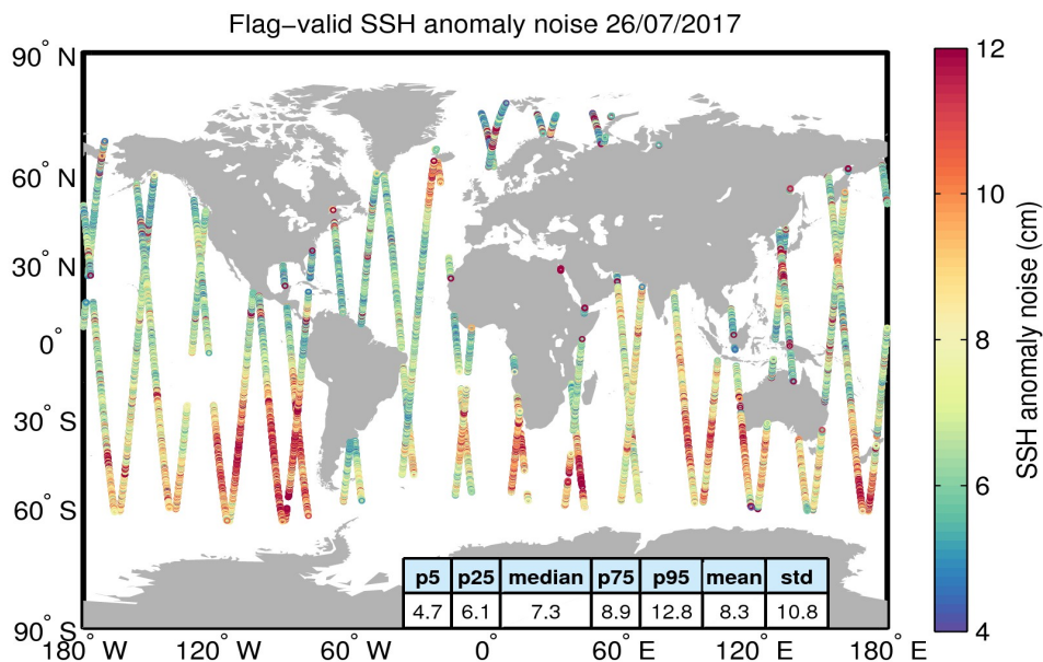
Figure 8. Geographical distribution of flag-valid 20-Hz SSH anomaly measurement noise over oceans and lakes for 26/07/2017. The statistical values shown in the table refer to the SSH anomaly noise and are calculated over all measurements shown in the figure.
