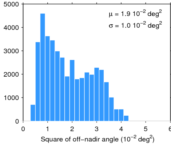
Figure 39. Histogram of flag-valid mispointing over oceans and lakes for 26/07/2017. The mean ( \mu ) and standard deviation ( \sigma ) are also shown. Note that values larger than 6 \cdot 10^{-2} \text{ deg}^2 are excluded from the histogram for the sake of readability but not from the computation of \mu and \sigma .
