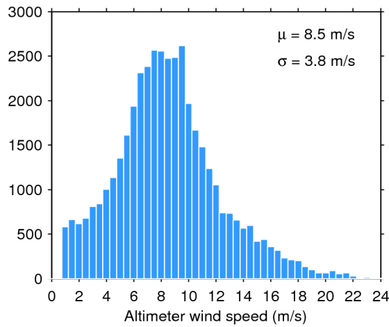
Figure 33. Histogram of flag-valid wind over oceans and lakes for 26/07/2017. The mean ( \mu ) and standard deviation ( \sigma ) are also shown. Note that values larger than 24 m/s are excluded from the histogram for the sake of readability but not from the computation of \mu and \sigma .
