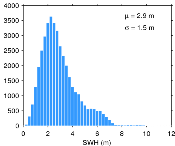
Figure 20. Histogram of science-valid SWH over oceans and lakes for 26/07/2017. The mean ( \mu ) and standard deviation ( \sigma ) are also shown. Note that values larger than 12 m are excluded from the histogram for the sake of readability but not from the computation of \mu and \sigma .
