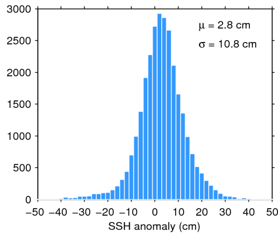
Figure 11. Histogram of science-valid SSH anomaly over oceans and lakes for 26/07/2017. The mean ( \mu ) and standard deviation ( \sigma ) are also shown. Note that values outside [-50 50] cm are excluded from the histogram for the sake of readability but not from the computation of \mu and \sigma .
