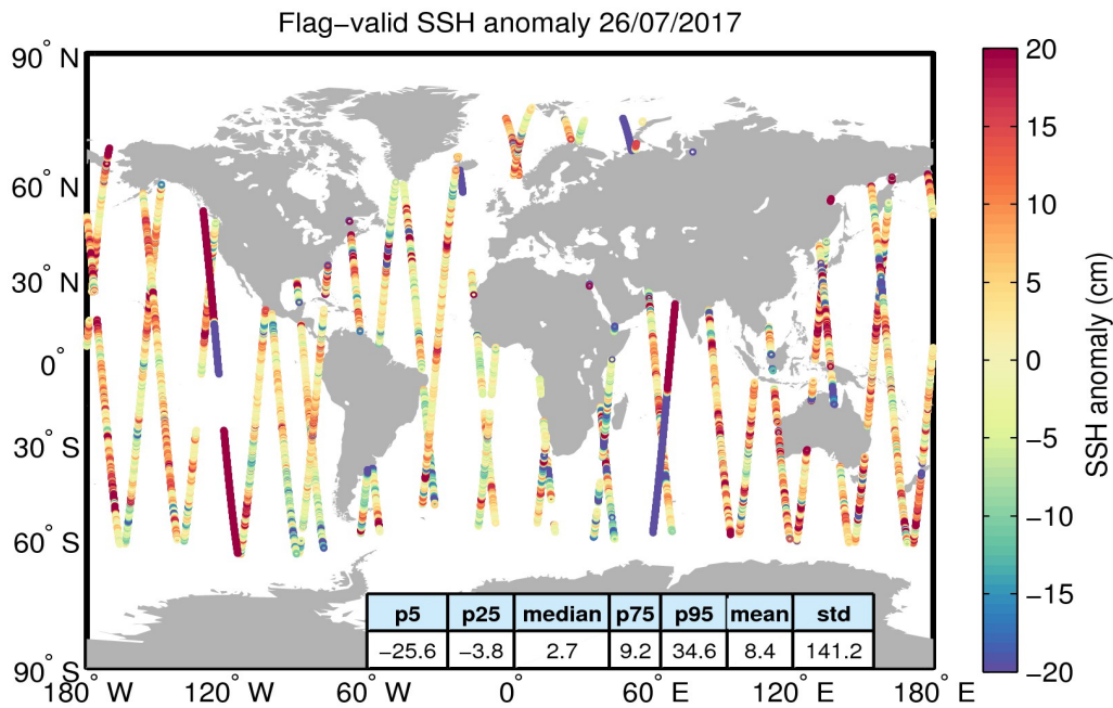
Figure 5. Geographical distribution of flag-valid 1-Hz SSH anomaly data over oceans and lakes for 26/07/2017. The statistical values shown in the table refer to the SSH anomaly in cm and are calculated over all measurements shown in the figure.
