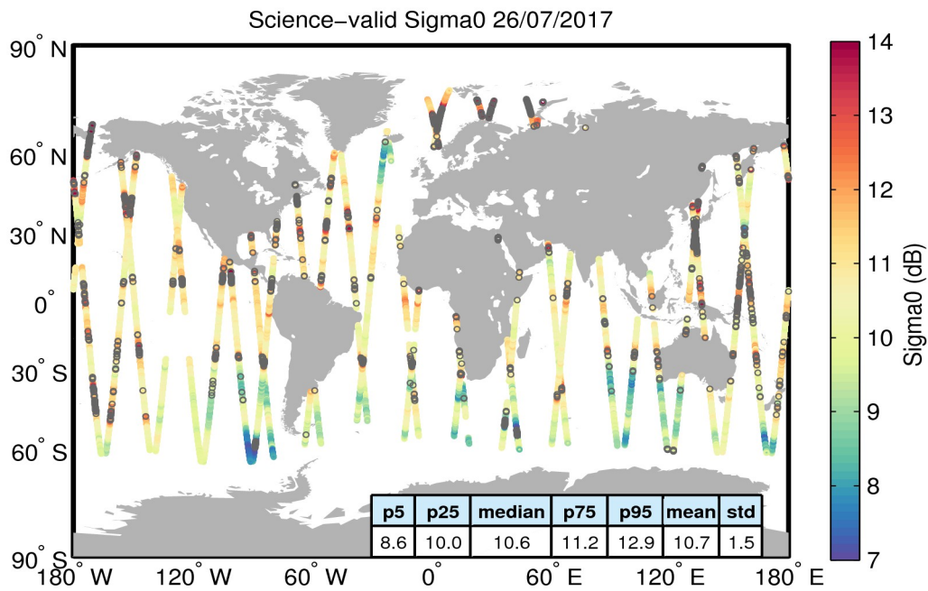
Figure 27. Geographical distribution of science-valid sigma0 data over oceans and lakes for 26/07/2017. The statistical values shown in the table refer to the sigma0 in dB and are calculated over all measurements shown in the figure. Gray circles denote records that have been rejected based on the editing criteria described in Table 4.
