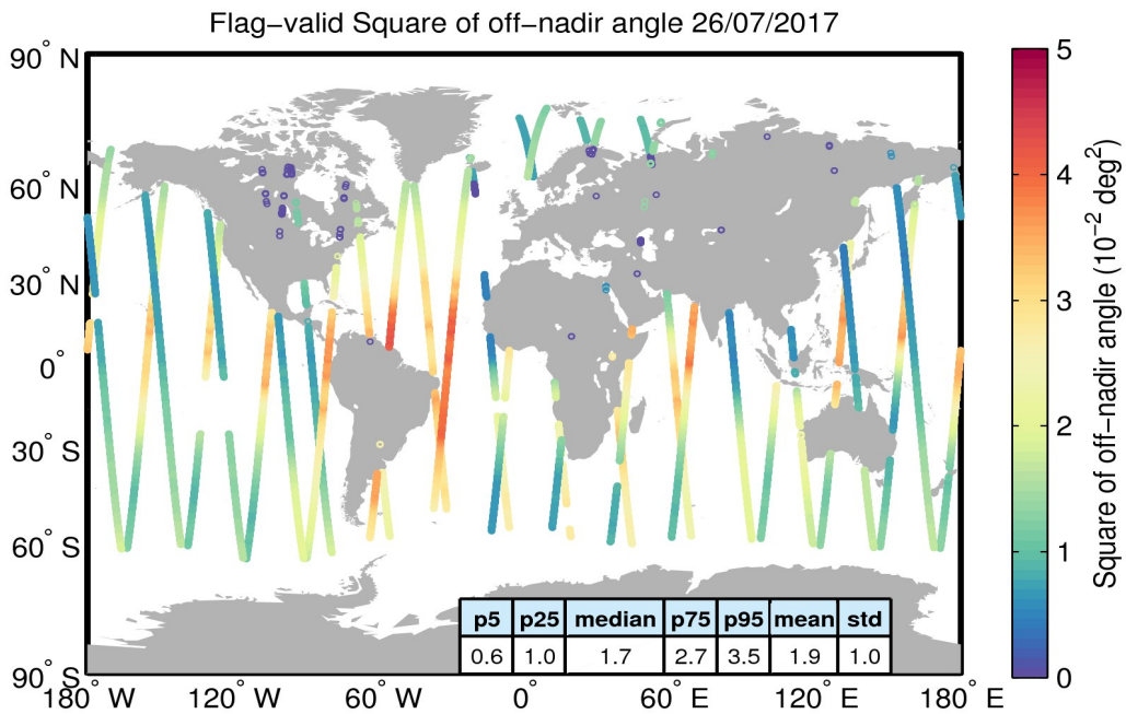
Figure 37. Geographical distribution of flag-valid mispointing data over oceans and lakes for 26/07/2017. The statistical values shown in the table refer to the mispointing in 10^{-2} deg 2 and are calculated over all measurements shown in the figure.
