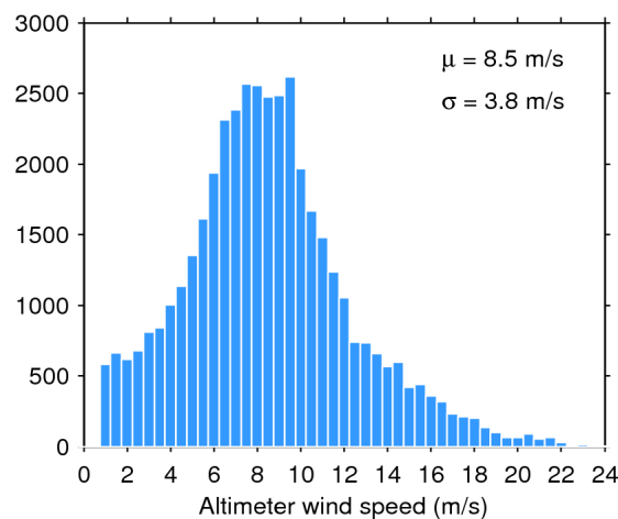
Figure 35. Histogram of science-valid wind over oceans and lakes for 26/07/2017. The mean ( \mu ) and standard deviation ( \sigma ) are also shown. Note that values larger than 24 m/s are excluded from the histogram for the sake of readability but not from the computation of \mu and \sigma .
