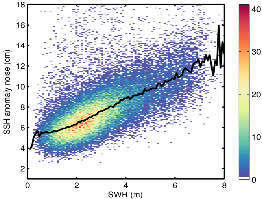
Figure 9. 2D histogram showing flag-valid SSH anomaly noise as a function of SWH for 26/07/2017. The black line denotes the median SSH anomaly noise as a function of SWH.
