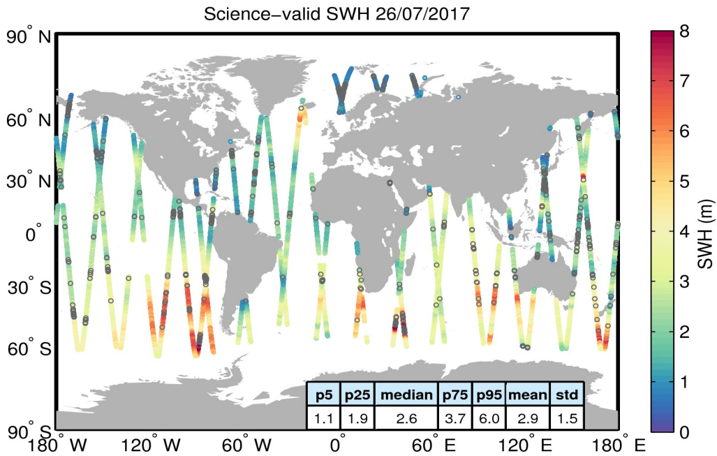
Figure 19. Geographical distribution of science-valid SWH data over oceans and lakes for 26/07/2017. The statistical values shown in the table refer to the SWH in m and are calculated over all measurements shown in the figure. Gray circles denote records that have been rejected based on the editing criteria described in Table 3.
