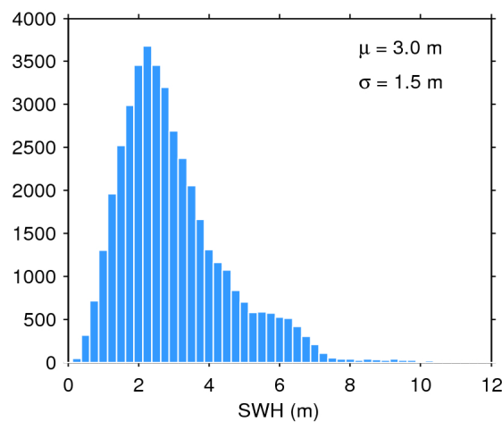
Figure 17. Histogram of flag-valid SWH over oceans and lakes for 26/07/2017. The mean ( \mu ) and standard deviation ( \sigma ) are also shown. Note that values larger than 12 m are excluded from the histogram for the sake of readability but not from the computation of \mu and \sigma .
