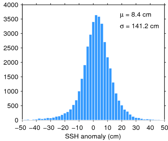
Figure 7. Histogram of flag-valid SSH anomaly over oceans and lakes for 26/07/2017. The mean ( \mu ) and standard deviation ( \sigma ) are also shown. Note that values outside [-50 50] cm are excluded from the histogram for the sake of readability but not from the computation of \mu and \sigma .
