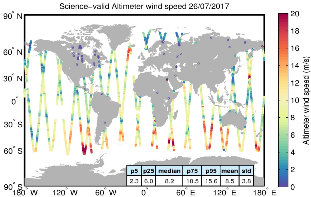
Figure 34. Geographical distribution of science-valid wind data over oceans and lakes for 26/07/2017. The statistical values shown in the table refer to the wind in m/s and are calculated over all measurements shown in the figure. Gray circles denote records that have been rejected based on the editing criteria described in Table 5.
