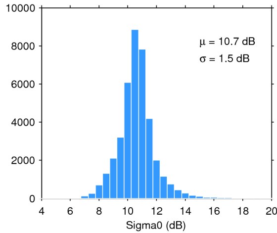
Figure 28. Histogram of science-valid sigma0 over oceans and lakes for 26/07/2017. The mean ( \mu ) and standard deviation ( \sigma ) are also shown. Note that values outside [4 20] dB are excluded from the histogram for the sake of readability but not from the computation of \mu and \sigma .
