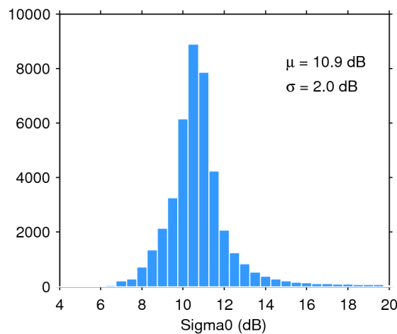
Figure 25. Histogram of flag-valid sigma0 over oceans and lakes for 26/07/2017. The mean ( \mu ) and standard deviation ( \sigma ) are also shown. Note that values outside [4 20] dB are excluded from the histogram for the sake of readability but not from the computation of \mu and \sigma .
