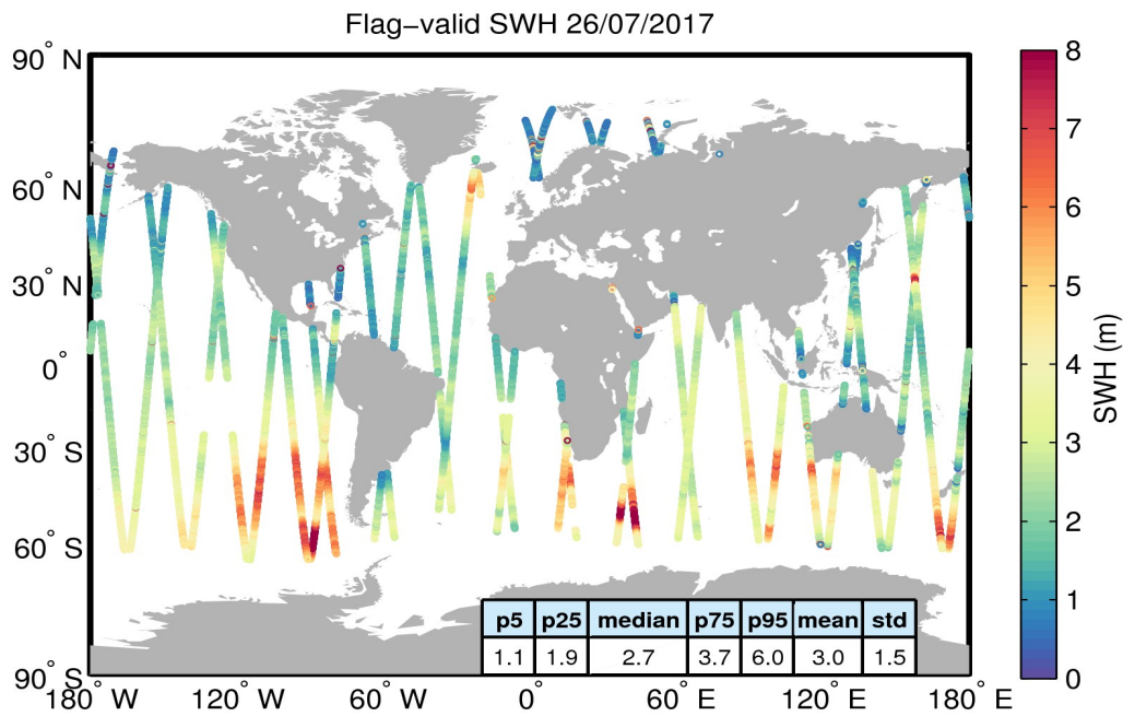
Figure 15. Geographical distribution of flag-valid SWH data over oceans and lakes for 26/07/2017. The statistical values shown in the table refer to the SWH in m and are calculated over all measurements shown in the figure.
