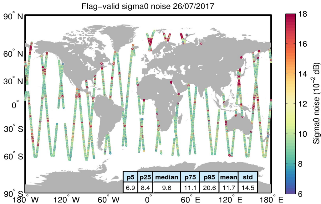
Figure 26. Geographical distribution of flag-valid 20-Hz sigma0 measurement noise over oceans and lakes for 26/07/2017. The statistical values shown in the table refer to the sigma0 noise and are calculated over all measurements shown in the figure.
