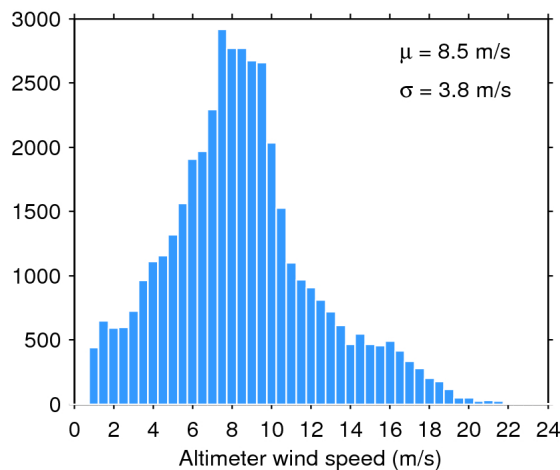
Figure 35. Histogram of science-valid wind over oceans and lakes for 24/07/2017. The mean ( \mu ) and standard deviation ( \sigma ) are also shown. Note that values larger than 24 m/s are excluded from the histogram for the sake of readability but not from the computation of \mu and \sigma .
