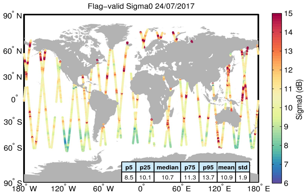
Figure 23. Geographical distribution of flag-valid sigma0 data over oceans and lakes for 24/07/2017. The statistical values shown in the table refer to the sigma0 in dB and are calculated over all measurements shown in the figure.
