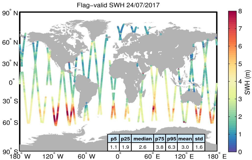
Figure 15. Geographical distribution of flag-valid SWH data over oceans and lakes for 24/07/2017. The statistical values shown in the table refer to the SWH in m and are calculated over all measurements shown in the figure.
