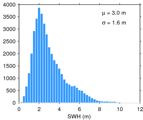
Figure 17. Histogram of flag-valid SWH over oceans and lakes for 24/07/2017. The mean ( \mu ) and standard deviation ( \sigma ) are also shown. Note that values larger than 12 m are excluded from the histogram for the sake of readability but not from the computation of \mu and \sigma .
