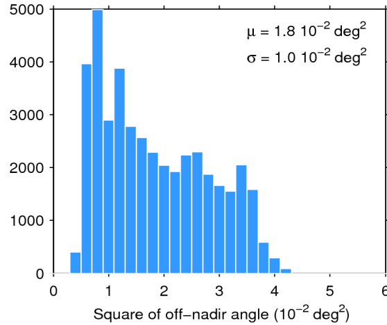
Figure 39. Histogram of flag-valid mispointing over oceans and lakes for 24/07/2017. The mean ( \mu ) and standard deviation ( \sigma ) are also shown. Note that values larger than 6 \cdot 10^{-2} \text{ deg}^2 are excluded from the histogram for the sake of readability but not from the computation of \mu and \sigma .
