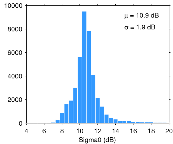
Figure 25. Histogram of flag-valid sigma0 over oceans and lakes for 24/07/2017. The mean ( \mu ) and standard deviation ( \sigma ) are also shown. Note that values outside [4 20] dB are excluded from the histogram for the sake of readability but not from the computation of \mu and \sigma .
