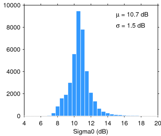
Figure 28. Histogram of science-valid sigma0 over oceans and lakes for 24/07/2017. The mean ( \mu ) and standard deviation ( \sigma ) are also shown. Note that values outside [4 20] dB are excluded from the histogram for the sake of readability but not from the computation of \mu and \sigma .
