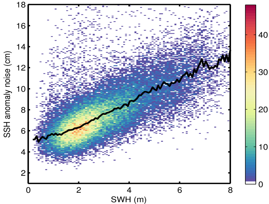
Figure 9. 2D histogram showing flag-valid SSH anomaly noise as a function of SWH for 24/07/2017. The black line denotes the median SSH anomaly noise as a function of SWH.
