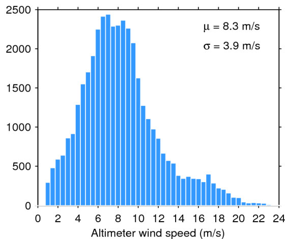
Figure 35. Histogram of science-valid wind over oceans and lakes for 23/07/2017. The mean ( \mu ) and standard deviation ( \sigma ) are also shown. Note that values larger than 24 m/s are excluded from the histogram for the sake of readability but not from the computation of \mu and \sigma .
