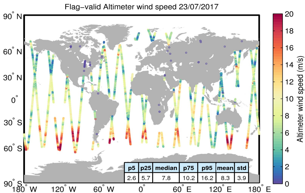
Figure 31. Geographical distribution of flag-valid wind data over oceans and lakes for 23/07/2017. The statistical values shown in the table refer to the wind in m/s and are calculated over all measurements shown in the figure.
