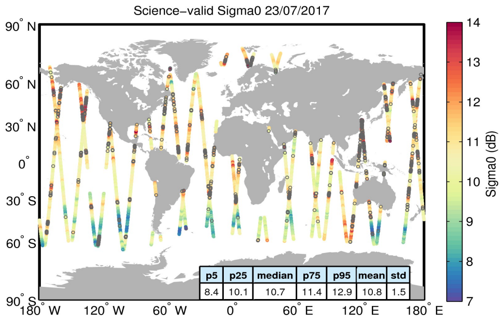
Figure 27. Geographical distribution of science-valid sigma0 data over oceans and lakes for 23/07/2017. The statistical values shown in the table refer to the sigma0 in dB and are calculated over all measurements shown in the figure. Gray circles denote records that have been rejected based on the editing criteria described in Table 4.
