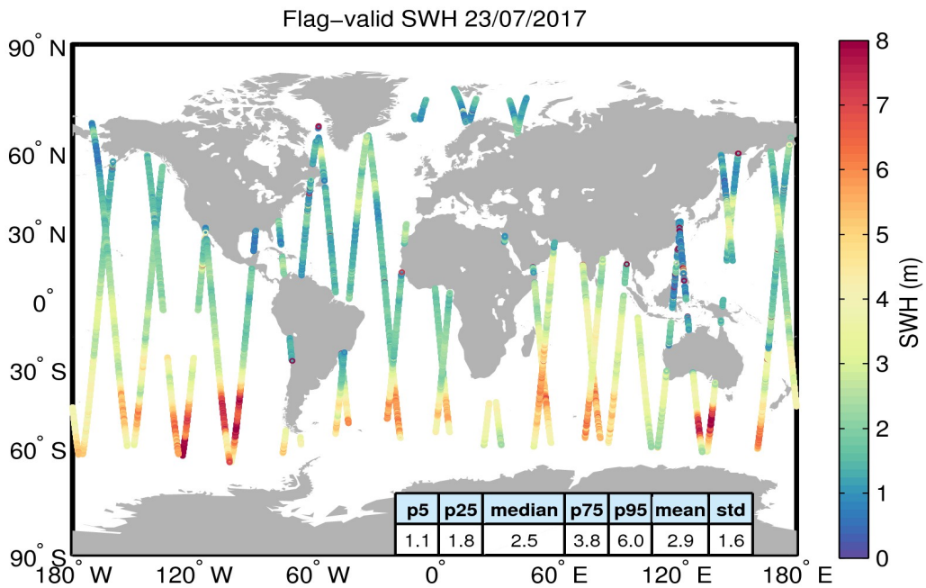
Figure 15. Geographical distribution of flag-valid SWH data over oceans and lakes for 23/07/2017. The statistical values shown in the table refer to the SWH in m and are calculated over all measurements shown in the figure.
