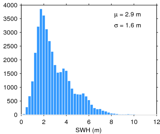
Figure 17. Histogram of flag-valid SWH over oceans and lakes for 23/07/2017. The mean ( \mu ) and standard deviation ( \sigma ) are also shown. Note that values larger than 12 m are excluded from the histogram for the sake of readability but not from the computation of \mu and \sigma .
