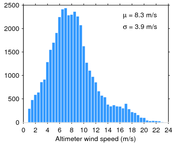
Figure 33. Histogram of flag-valid wind over oceans and lakes for 23/07/2017. The mean ( \mu ) and standard deviation ( \sigma ) are also shown. Note that values larger than 24 m/s are excluded from the histogram for the sake of readability but not from the computation of \mu and \sigma .
