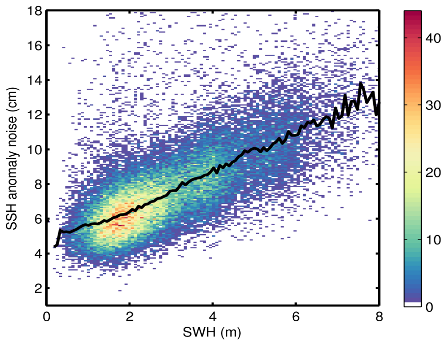
Figure 9. 2D histogram showing flag-valid SSH anomaly noise as a function of SWH for 23/07/2017. The black line denotes the median SSH anomaly noise as a function of SWH.
