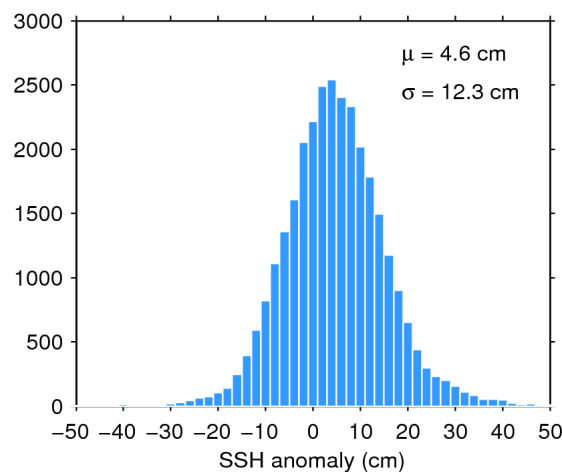
Figure 11. Histogram of science-valid SSH anomaly over oceans and lakes for 23/07/2017. The mean ( \mu ) and standard deviation ( \sigma ) are also shown. Note that values outside [-50 50] cm are excluded from the histogram for the sake of readability but not from the computation of \mu and \sigma .
