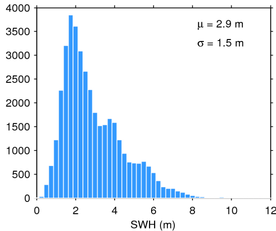
Figure 20. Histogram of science-valid SWH over oceans and lakes for 23/07/2017. The mean ( \mu ) and standard deviation ( \sigma ) are also shown. Note that values larger than 12 m are excluded from the histogram for the sake of readability but not from the computation of \mu and \sigma .
