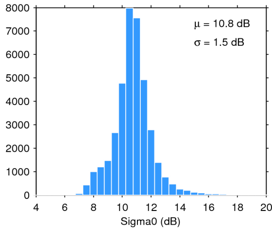
Figure 28. Histogram of science-valid sigma0 over oceans and lakes for 23/07/2017. The mean ( \mu ) and standard deviation ( \sigma ) are also shown. Note that values outside [4 20] dB are excluded from the histogram for the sake of readability but not from the computation of \mu and \sigma .
