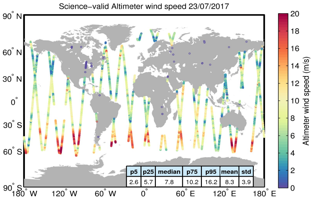
Figure 34. Geographical distribution of science-valid wind data over oceans and lakes for 23/07/2017. The statistical values shown in the table refer to the wind in m/s and are calculated over all measurements shown in the figure. Gray circles denote records that have been rejected based on the editing criteria described in Table 5.
