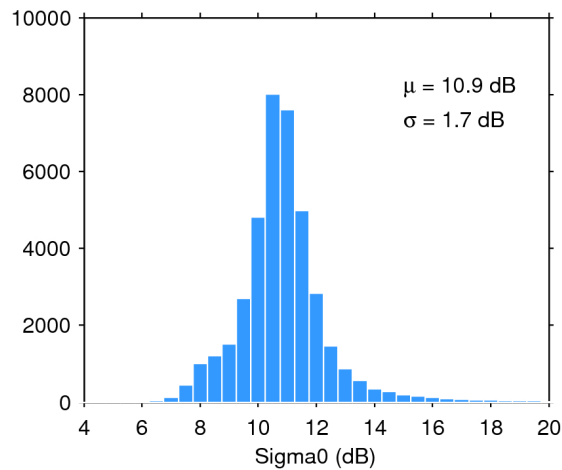
Figure 25. Histogram of flag-valid sigma0 over oceans and lakes for 23/07/2017. The mean ( \mu ) and standard deviation ( \sigma ) are also shown. Note that values outside [4 20] dB are excluded from the histogram for the sake of readability but not from the computation of \mu and \sigma .
