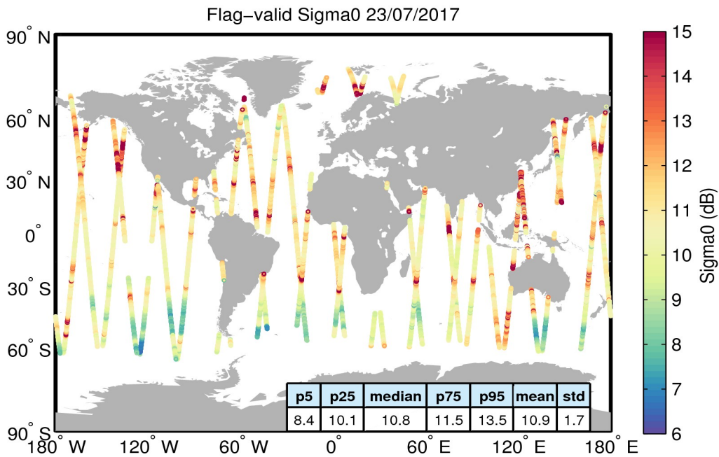
Figure 23. Geographical distribution of flag-valid sigma0 data over oceans and lakes for 23/07/2017. The statistical values shown in the table refer to the sigma0 in dB and are calculated over all measurements shown in the figure.
