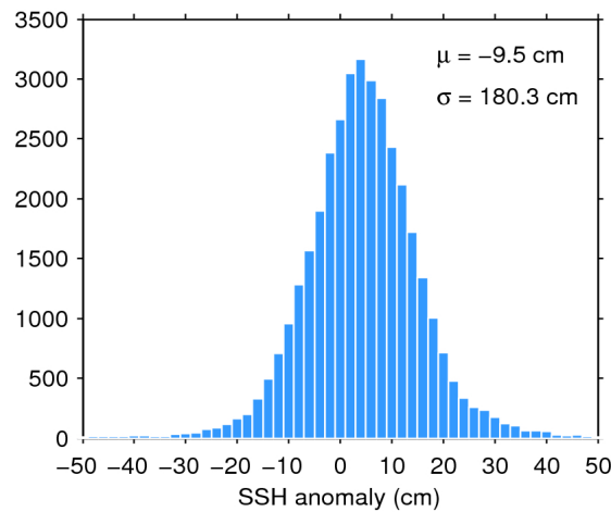
Figure 7. Histogram of flag-valid SSH anomaly over oceans and lakes for 23/07/2017. The mean ( \mu ) and standard deviation ( \sigma ) are also shown. Note that values outside [-50 50] cm are excluded from the histogram for the sake of readability but not from the computation of \mu and \sigma .
