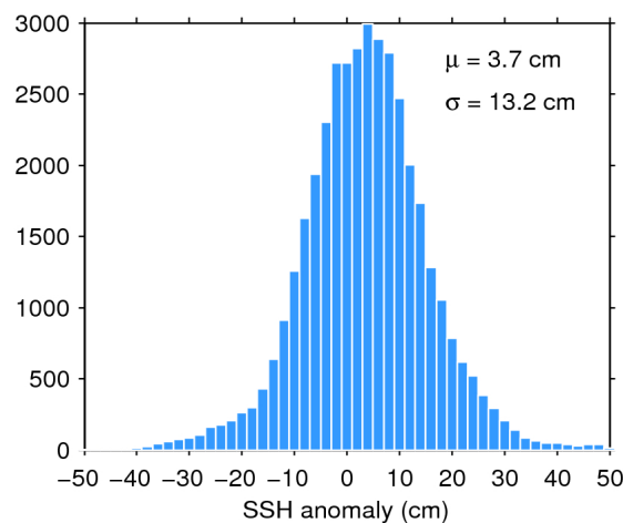
Figure 11. Histogram of science-valid SSH anomaly over oceans and lakes for 22/07/2017. The mean ( \mu ) and standard deviation ( \sigma ) are also shown. Note that values outside [-50 50] cm are excluded from the histogram for the sake of readability but not from the computation of \mu and \sigma .
