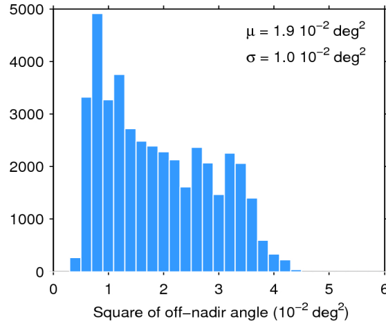
Figure 39. Histogram of flag-valid mispointing over oceans and lakes for 22/07/2017. The mean ( \mu ) and standard deviation ( \sigma ) are also shown. Note that values larger than 6 \cdot 10^{-2} \text{ deg}^2 are excluded from the histogram for the sake of readability but not from the computation of \mu and \sigma .
