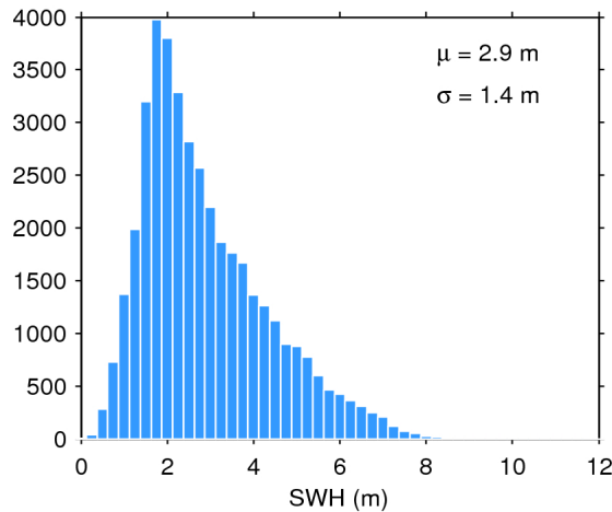
Figure 20. Histogram of science-valid SWH over oceans and lakes for 22/07/2017. The mean ( \mu ) and standard deviation ( \sigma ) are also shown. Note that values larger than 12 m are excluded from the histogram for the sake of readability but not from the computation of \mu and \sigma .
