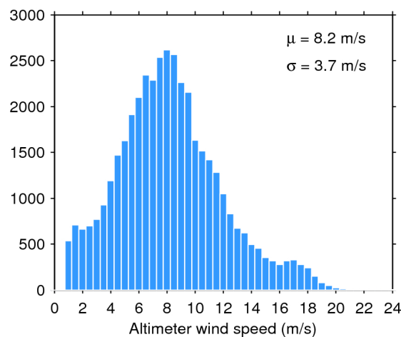
Figure 35. Histogram of science-valid wind over oceans and lakes for 22/07/2017. The mean ( \mu ) and standard deviation ( \sigma ) are also shown. Note that values larger than 24 m/s are excluded from the histogram for the sake of readability but not from the computation of \mu and \sigma .
