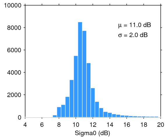
Figure 25. Histogram of flag-valid sigma0 over oceans and lakes for 22/07/2017. The mean ( \mu ) and standard deviation ( \sigma ) are also shown. Note that values outside [4 20] dB are excluded from the histogram for the sake of readability but not from the computation of \mu and \sigma .
