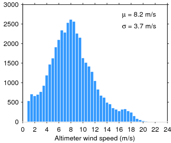
Figure 33. Histogram of flag-valid wind over oceans and lakes for 22/07/2017. The mean ( \mu ) and standard deviation ( \sigma ) are also shown. Note that values larger than 24 m/s are excluded from the histogram for the sake of readability but not from the computation of \mu and \sigma .
