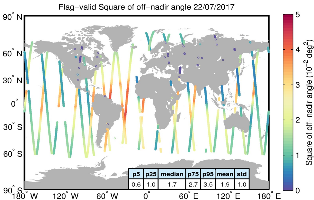
Figure 37. Geographical distribution of flag-valid mispointing data over oceans and lakes for 22/07/2017. The statistical values shown in the table refer to the mispointing in 10^{-2} deg 2 and are calculated over all measurements shown in the figure.
