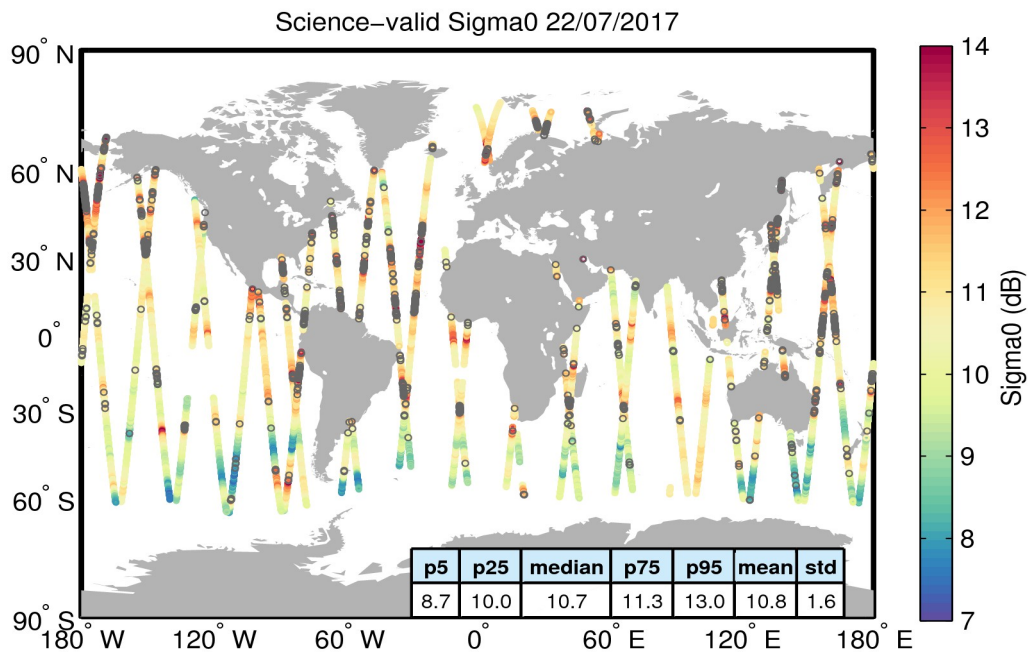
Figure 27. Geographical distribution of science-valid sigma0 data over oceans and lakes for 22/07/2017. The statistical values shown in the table refer to the sigma0 in dB and are calculated over all measurements shown in the figure. Gray circles denote records that have been rejected based on the editing criteria described in Table 4.
