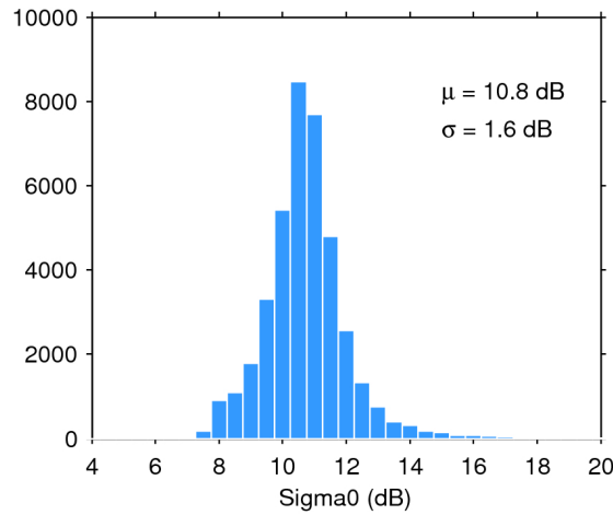
Figure 28. Histogram of science-valid sigma0 over oceans and lakes for 22/07/2017. The mean ( \mu ) and standard deviation ( \sigma ) are also shown. Note that values outside [4 20] dB are excluded from the histogram for the sake of readability but not from the computation of \mu and \sigma .
