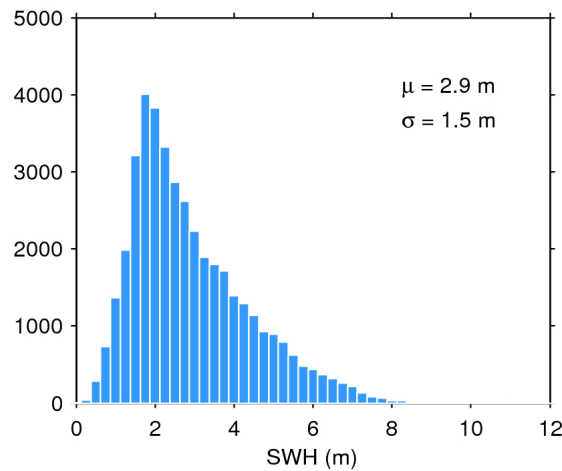
Figure 17. Histogram of flag-valid SWH over oceans and lakes for 22/07/2017. The mean ( \mu ) and standard deviation ( \sigma ) are also shown. Note that values larger than 12 m are excluded from the histogram for the sake of readability but not from the computation of \mu and \sigma .
