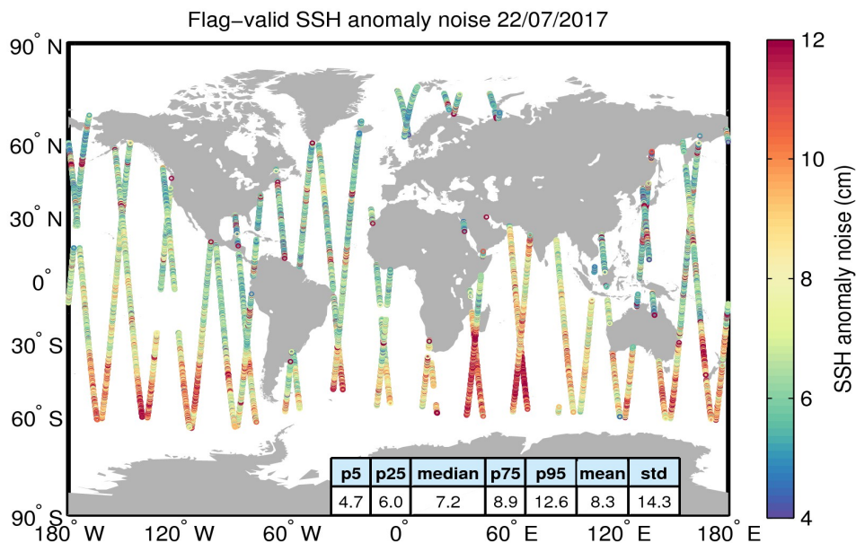
Figure 8. Geographical distribution of flag-valid 20-Hz SSH anomaly measurement noise over oceans and lakes for 22/07/2017. The statistical values shown in the table refer to the SSH anomaly noise and are calculated over all measurements shown in the figure.
