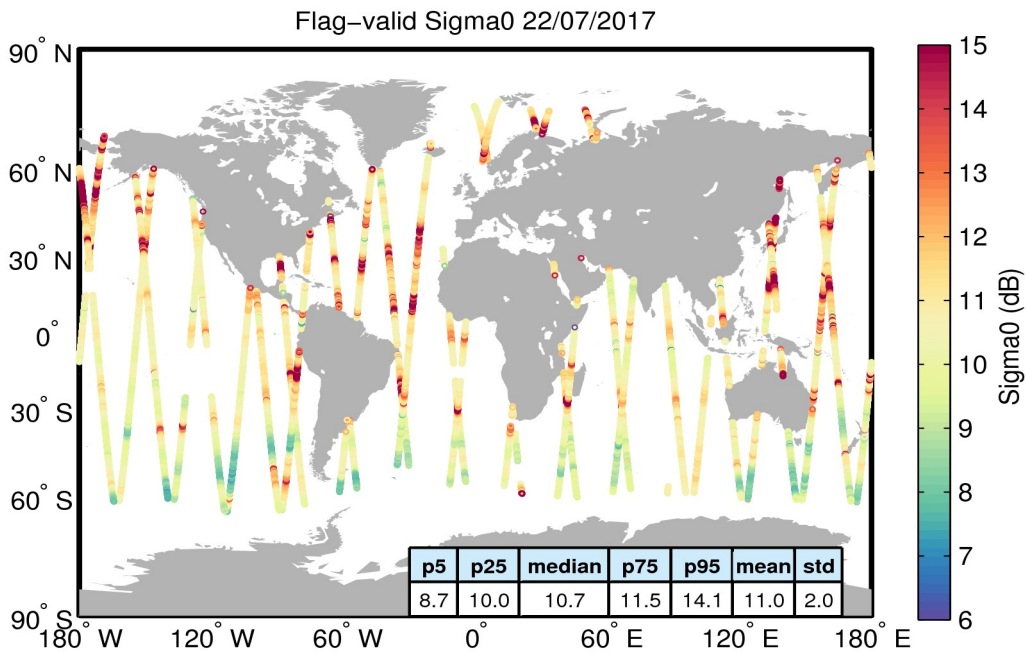
Figure 23. Geographical distribution of flag-valid sigma0 data over oceans and lakes for 22/07/2017. The statistical values shown in the table refer to the sigma0 in dB and are calculated over all measurements shown in the figure.
