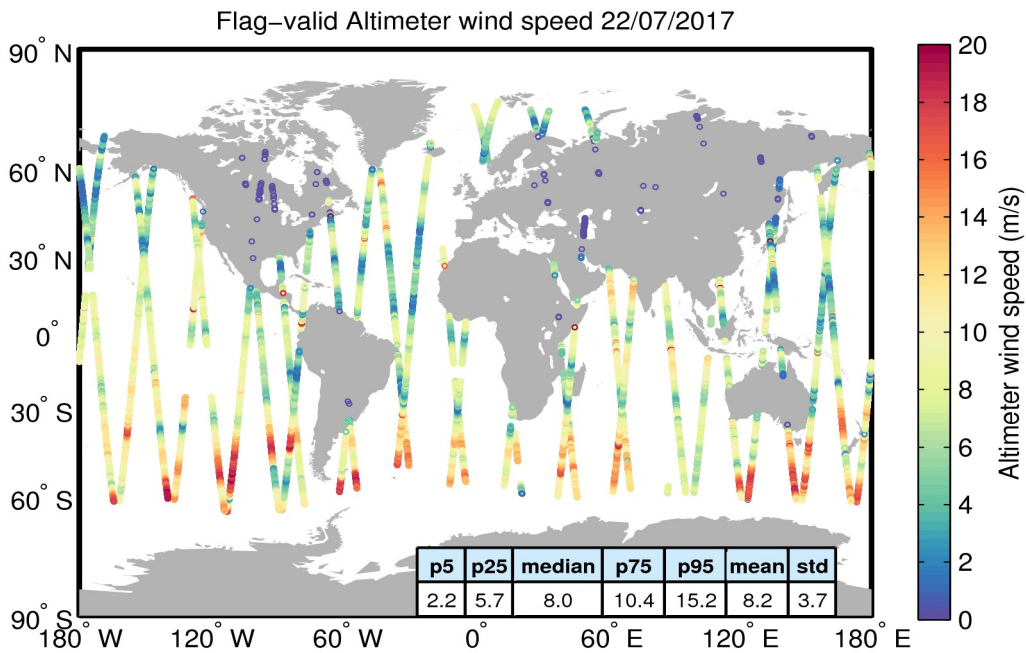
Figure 31. Geographical distribution of flag-valid wind data over oceans and lakes for 22/07/2017. The statistical values shown in the table refer to the wind in m/s and are calculated over all measurements shown in the figure.
