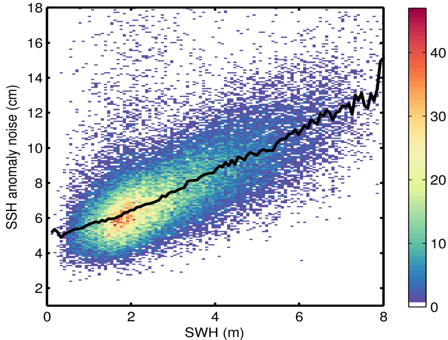
Figure 9. 2D histogram showing flag-valid SSH anomaly noise as a function of SWH for 22/07/2017. The black line denotes the median SSH anomaly noise as a function of SWH.
