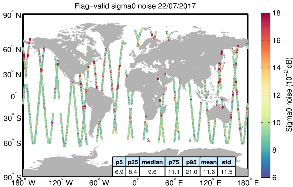
Figure 26. Geographical distribution of flag-valid 20-Hz sigma0 measurement noise over oceans and lakes for 22/07/2017. The statistical values shown in the table refer to the sigma0 noise and are calculated over all measurements shown in the figure.
