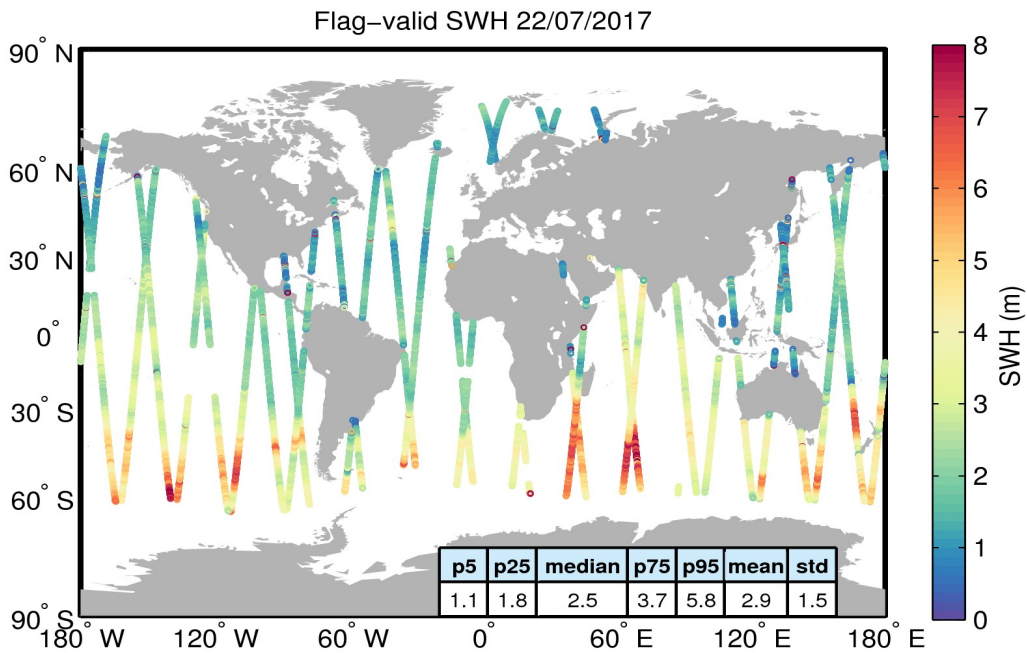
Figure 15. Geographical distribution of flag-valid SWH data over oceans and lakes for 22/07/2017. The statistical values shown in the table refer to the SWH in m and are calculated over all measurements shown in the figure.
