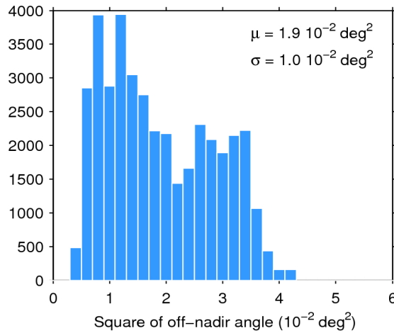
Figure 39. Histogram of flag-valid mispointing over oceans and lakes for 21/07/2017. The mean ( \mu ) and standard deviation ( \sigma ) are also shown. Note that values larger than 6 \cdot 10^{-2} \text{ deg}^2 are excluded from the histogram for the sake of readability but not from the computation of \mu and \sigma .
