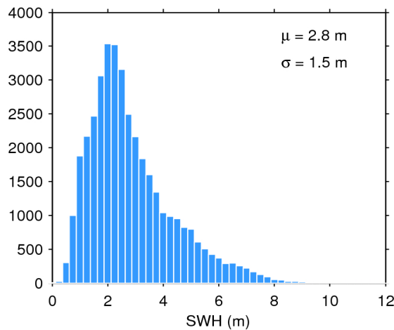
Figure 20. Histogram of science-valid SWH over oceans and lakes for 21/07/2017. The mean ( \mu ) and standard deviation ( \sigma ) are also shown. Note that values larger than 12 m are excluded from the histogram for the sake of readability but not from the computation of \mu and \sigma .
