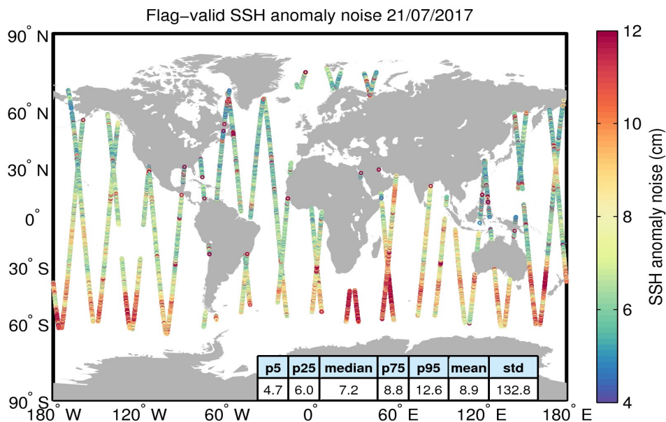
Figure 8. Geographical distribution of flag-valid 20-Hz SSH anomaly measurement noise over oceans and lakes for 21/07/2017. The statistical values shown in the table refer to the SSH anomaly noise and are calculated over all measurements shown in the figure.
