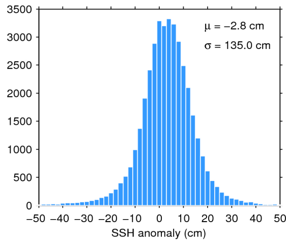
Figure 7. Histogram of flag-valid SSH anomaly over oceans and lakes for 21/07/2017. The mean ( \mu ) and standard deviation ( \sigma ) are also shown. Note that values outside [-50\ 50] cm are excluded from the histogram for the sake of readability but not from the computation of \mu and \sigma .
