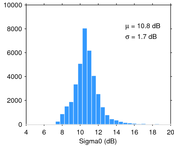
Figure 28. Histogram of science-valid sigma0 over oceans and lakes for 21/07/2017. The mean ( \mu ) and standard deviation ( \sigma ) are also shown. Note that values outside [4 20] dB are excluded from the histogram for the sake of readability but not from the computation of \mu and \sigma .
