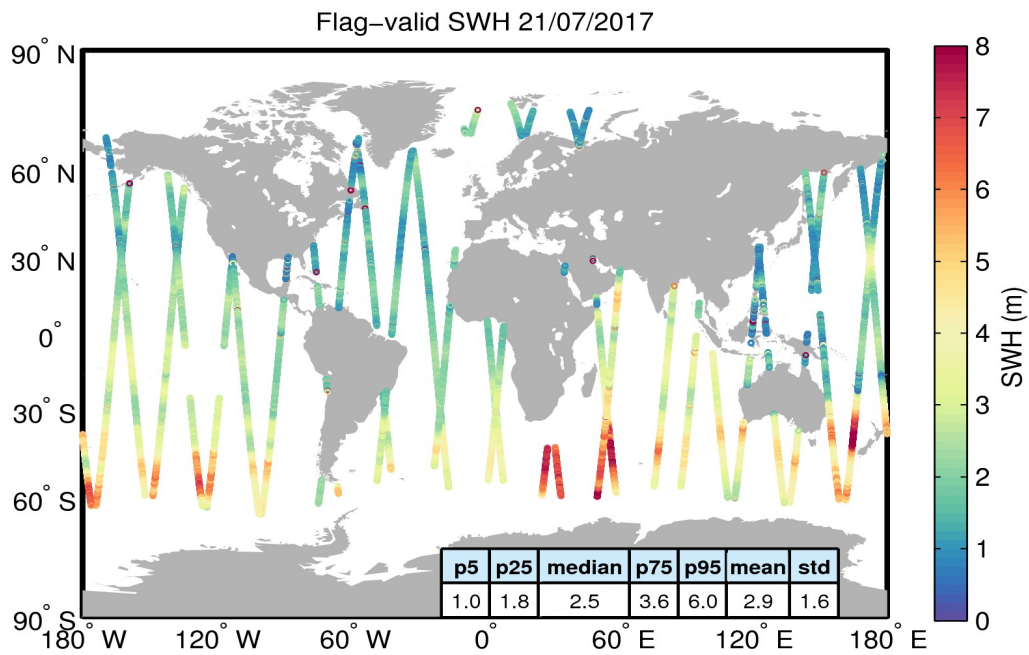
Figure 15. Geographical distribution of flag-valid SWH data over oceans and lakes for 21/07/2017. The statistical values shown in the table refer to the SWH in m and are calculated over all measurements shown in the figure.
