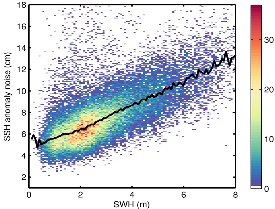
Figure 9. 2D histogram showing flag-valid SSH anomaly noise as a function of SWH for 21/07/2017. The black line denotes the median SSH anomaly noise as a function of SWH.
