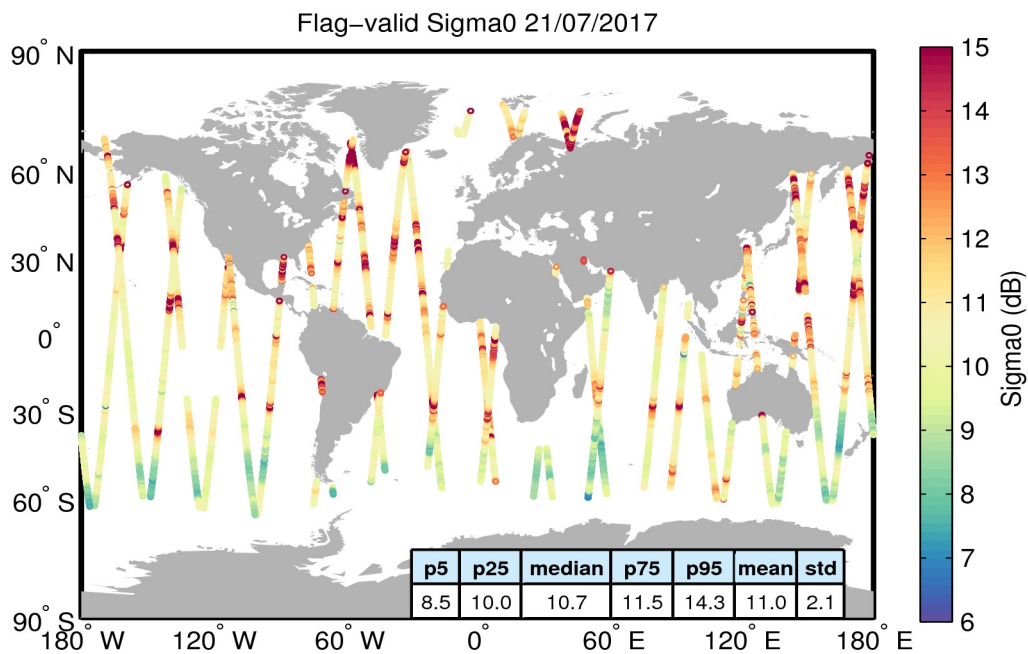
Figure 23. Geographical distribution of flag-valid sigma0 data over oceans and lakes for 21/07/2017. The statistical values shown in the table refer to the sigma0 in dB and are calculated over all measurements shown in the figure.
