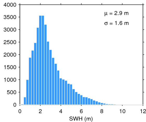
Figure 17. Histogram of flag-valid SWH over oceans and lakes for 21/07/2017. The mean ( \mu ) and standard deviation ( \sigma ) are also shown. Note that values larger than 12 m are excluded from the histogram for the sake of readability but not from the computation of \mu and \sigma .
