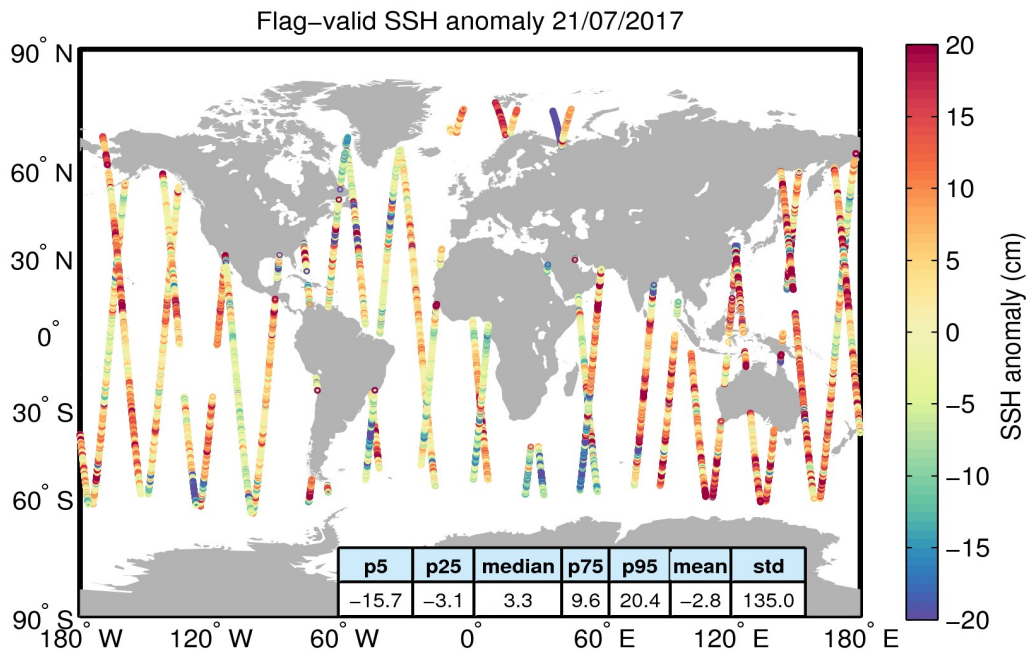
Figure 5. Geographical distribution of flag-valid 1-Hz SSH anomaly data over oceans and lakes for 21/07/2017. The statistical values shown in the table refer to the SSH anomaly in cm and are calculated over all measurements shown in the figure.
