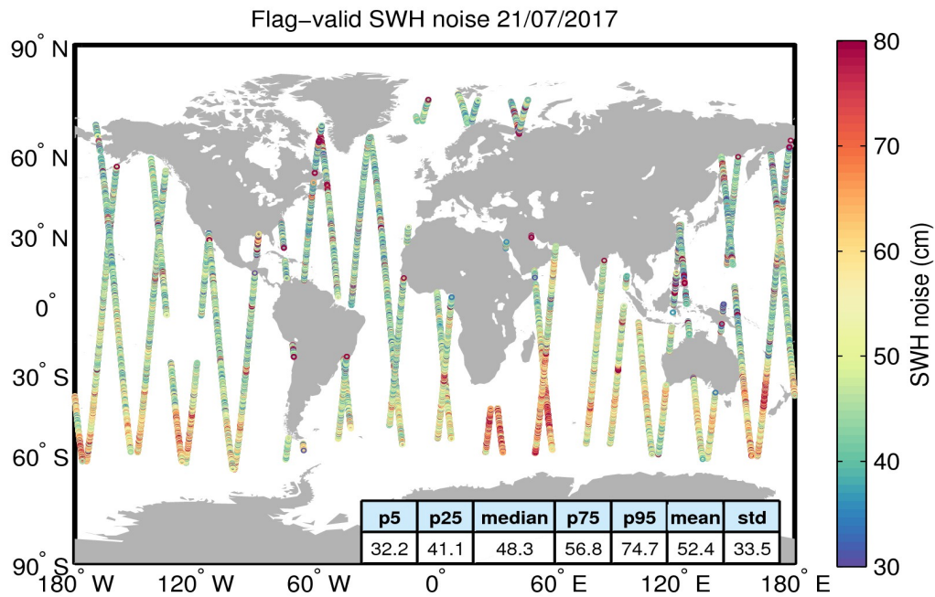
Figure 18. Geographical distribution of flag-valid 20-Hz SWH measurement noise over oceans and lakes for 21/07/2017. The statistical values shown in the table refer to the SWH noise and are calculated over all measurements shown in the figure.
