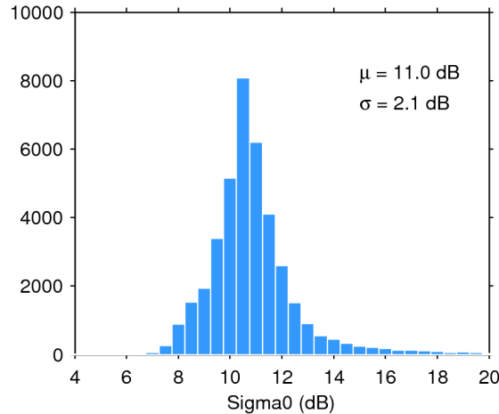
Figure 25. Histogram of flag-valid sigma0 over oceans and lakes for 21/07/2017. The mean ( \mu ) and standard deviation ( \sigma ) are also shown. Note that values outside [4 20] dB are excluded from the histogram for the sake of readability but not from the computation of \mu and \sigma .
