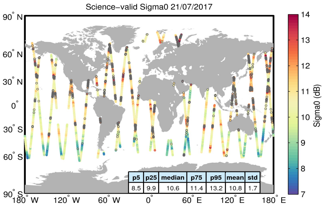
Figure 27. Geographical distribution of science-valid sigma0 data over oceans and lakes for 21/07/2017. The statistical values shown in the table refer to the sigma0 in dB and are calculated over all measurements shown in the figure. Gray circles denote records that have been rejected based on the editing criteria described in Table 4.
