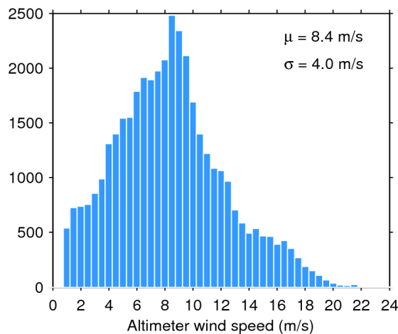
Figure 35. Histogram of science-valid wind over oceans and lakes for 21/07/2017. The mean ( \mu ) and standard deviation ( \sigma ) are also shown. Note that values larger than 24 m/s are excluded from the histogram for the sake of readability but not from the computation of \mu and \sigma .
