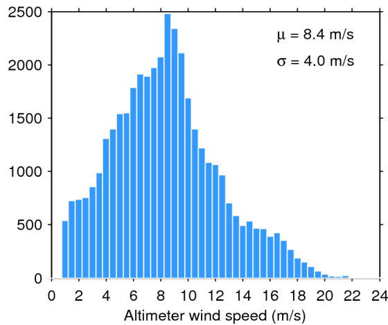
Figure 33. Histogram of flag-valid wind over oceans and lakes for 21/07/2017. The mean ( \mu ) and standard deviation ( \sigma ) are also shown. Note that values larger than 24 m/s are excluded from the histogram for the sake of readability but not from the computation of \mu and \sigma .
