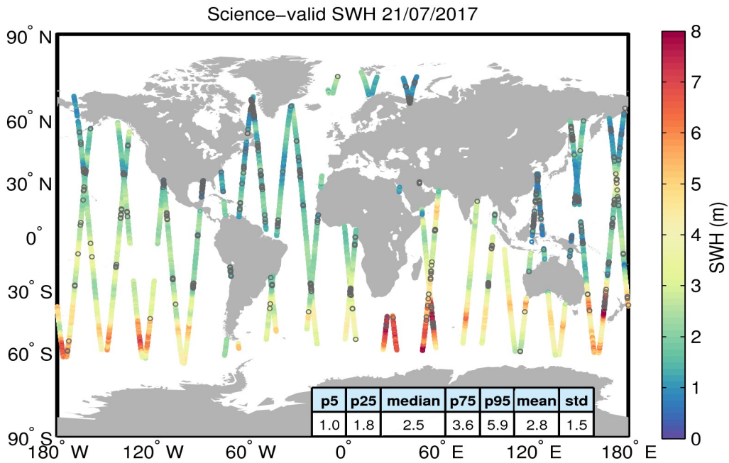
Figure 19. Geographical distribution of science-valid SWH data over oceans and lakes for 21/07/2017. The statistical values shown in the table refer to the SWH in m and are calculated over all measurements shown in the figure. Gray circles denote records that have been rejected based on the editing criteria described in Table 3.
