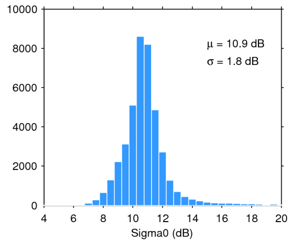
Figure 25. Histogram of flag-valid sigma0 over oceans and lakes for 20/07/2017. The mean ( \mu ) and standard deviation ( \sigma ) are also shown. Note that values outside [4 20] dB are excluded from the histogram for the sake of readability but not from the computation of \mu and \sigma .
