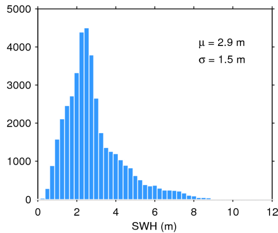
Figure 17. Histogram of flag-valid SWH over oceans and lakes for 20/07/2017. The mean ( \mu ) and standard deviation ( \sigma ) are also shown. Note that values larger than 12 m are excluded from the histogram for the sake of readability but not from the computation of \mu and \sigma .
