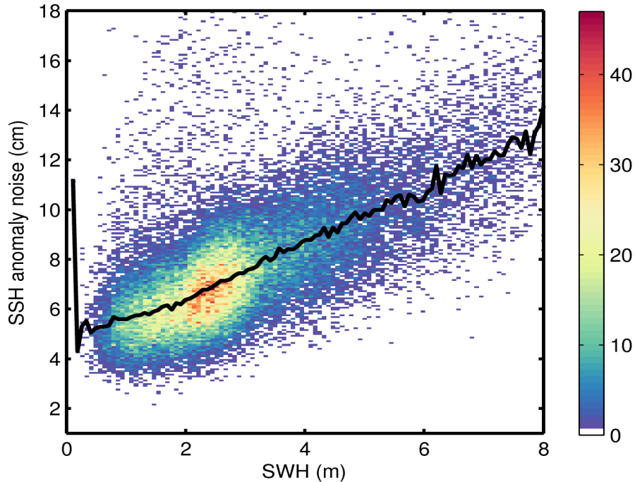
Figure 9. 2D histogram showing flag-valid SSH anomaly noise as a function of SWH for 20/07/2017. The black line denotes the median SSH anomaly noise as a function of SWH.
