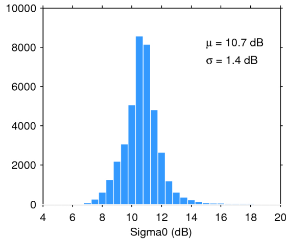
Figure 28. Histogram of science-valid sigma0 over oceans and lakes for 20/07/2017. The mean ( \mu ) and standard deviation ( \sigma ) are also shown. Note that values outside [4 20] dB are excluded from the histogram for the sake of readability but not from the computation of \mu and \sigma .
