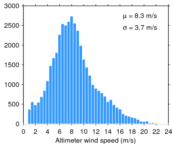
Figure 35. Histogram of science-valid wind over oceans and lakes for 20/07/2017. The mean ( \mu ) and standard deviation ( \sigma ) are also shown. Note that values larger than 24 m/s are excluded from the histogram for the sake of readability but not from the computation of \mu and \sigma .
