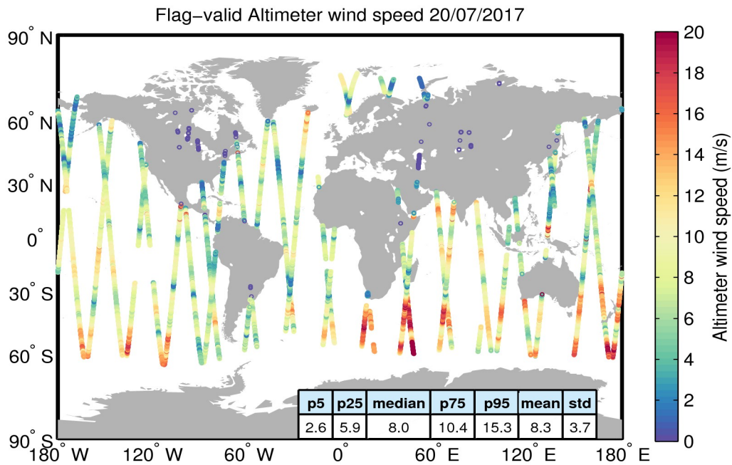
Figure 31. Geographical distribution of flag-valid wind data over oceans and lakes for 20/07/2017. The statistical values shown in the table refer to the wind in m/s and are calculated over all measurements shown in the figure.
