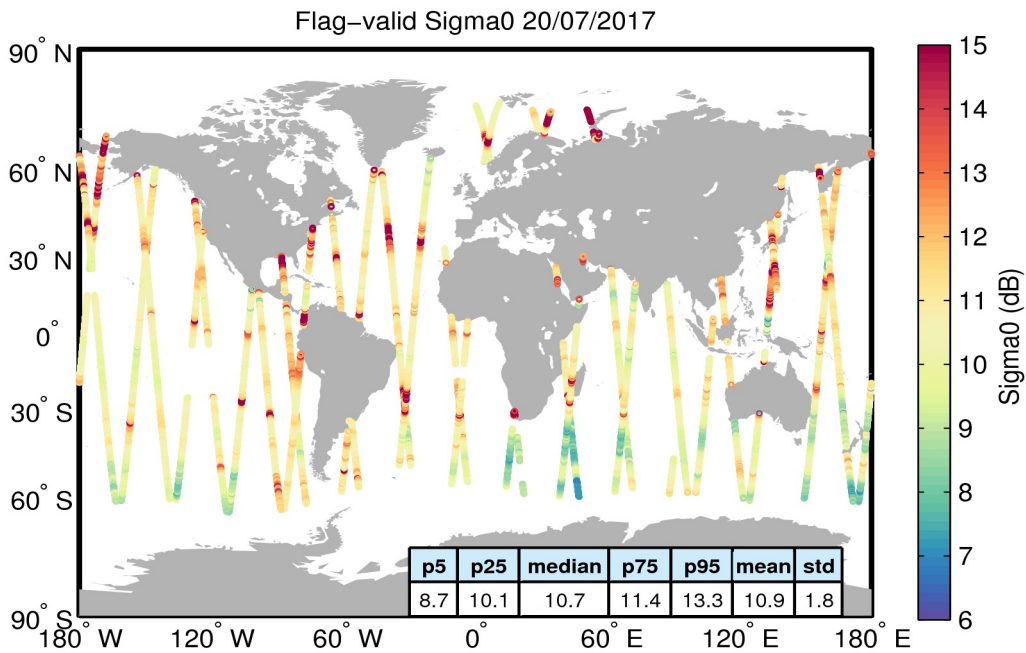
Figure 23. Geographical distribution of flag-valid sigma0 data over oceans and lakes for 20/07/2017. The statistical values shown in the table refer to the sigma0 in dB and are calculated over all measurements shown in the figure.
