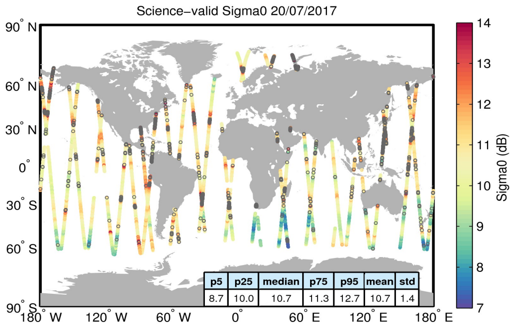
Figure 27. Geographical distribution of science-valid sigma0 data over oceans and lakes for 20/07/2017. The statistical values shown in the table refer to the sigma0 in dB and are calculated over all measurements shown in the figure. Gray circles denote records that have been rejected based on the editing criteria described in Table 4.
