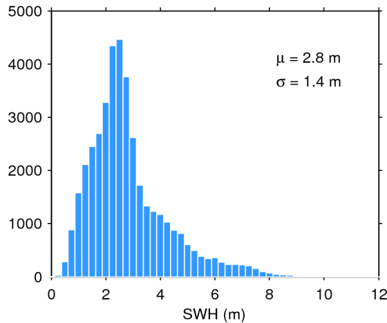
Figure 20. Histogram of science-valid SWH over oceans and lakes for 20/07/2017. The mean ( \mu ) and standard deviation ( \sigma ) are also shown. Note that values larger than 12 m are excluded from the histogram for the sake of readability but not from the computation of \mu and \sigma .
