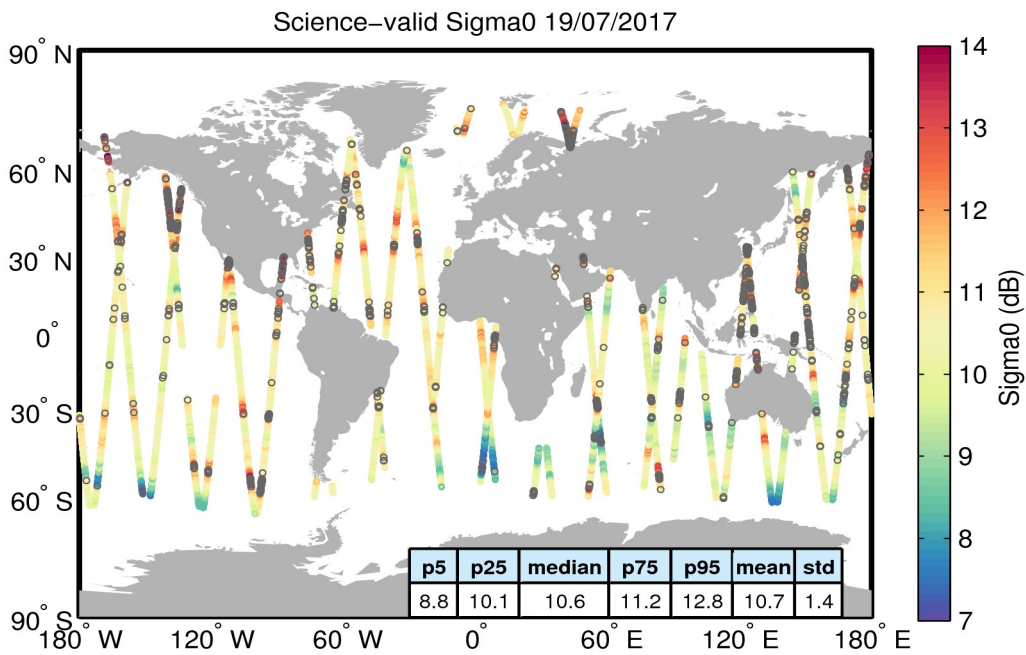
Figure 27. Geographical distribution of science-valid sigma0 data over oceans and lakes for 19/07/2017. The statistical values shown in the table refer to the sigma0 in dB and are calculated over all measurements shown in the figure. Gray circles denote records that have been rejected based on the editing criteria described in Table 4.
