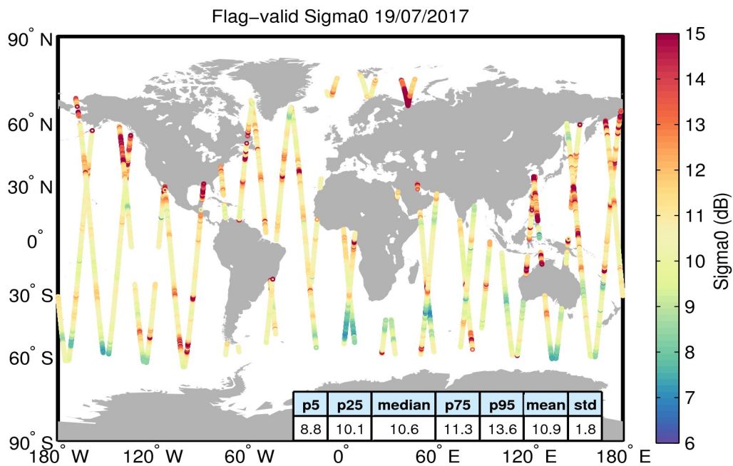
Figure 23. Geographical distribution of flag-valid sigma0 data over oceans and lakes for 19/07/2017. The statistical values shown in the table refer to the sigma0 in dB and are calculated over all measurements shown in the figure.
