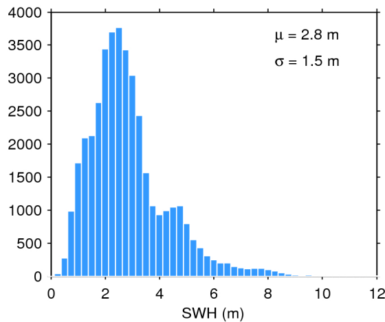
Figure 17. Histogram of flag-valid SWH over oceans and lakes for 19/07/2017. The mean ( \mu ) and standard deviation ( \sigma ) are also shown. Note that values larger than 12 m are excluded from the histogram for the sake of readability but not from the computation of \mu and \sigma .
