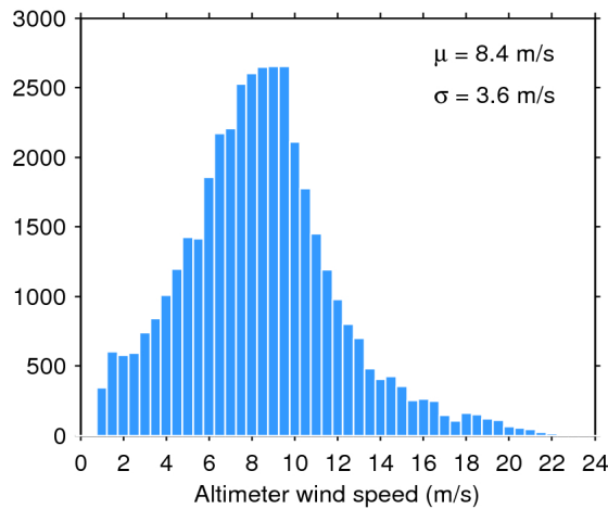
Figure 33. Histogram of flag-valid wind over oceans and lakes for 19/07/2017. The mean ( \mu ) and standard deviation ( \sigma ) are also shown. Note that values larger than 24 m/s are excluded from the histogram for the sake of readability but not from the computation of \mu and \sigma .
