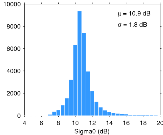
Figure 25. Histogram of flag-valid sigma0 over oceans and lakes for 19/07/2017. The mean ( \mu ) and standard deviation ( \sigma ) are also shown. Note that values outside [4 20] dB are excluded from the histogram for the sake of readability but not from the computation of \mu and \sigma .
