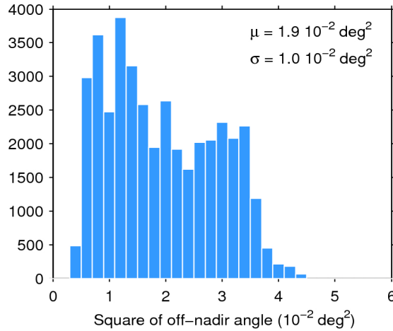
Figure 39. Histogram of flag-valid mispointing over oceans and lakes for 19/07/2017. The mean ( \mu ) and standard deviation ( \sigma ) are also shown. Note that values larger than 6 \cdot 10^{-2} \text{ deg}^2 are excluded from the histogram for the sake of readability but not from the computation of \mu and \sigma .
