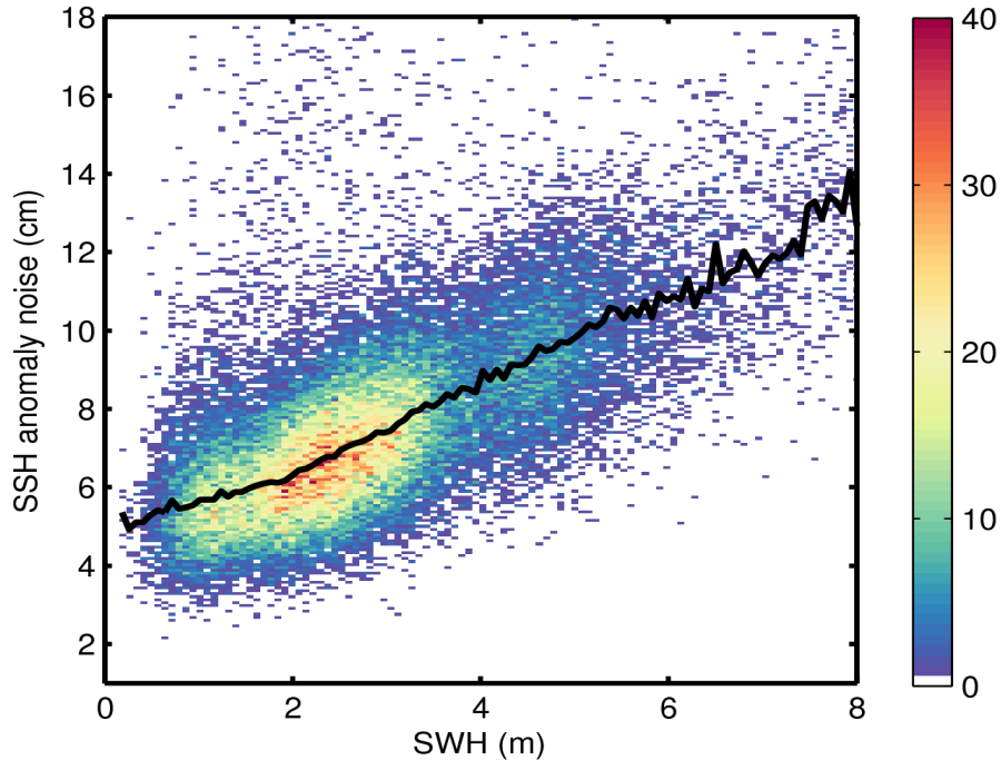
Figure 9. 2D histogram showing flag-valid SSH anomaly noise as a function of SWH for 19/07/2017. The black line denotes the median SSH anomaly noise as a function of SWH.
