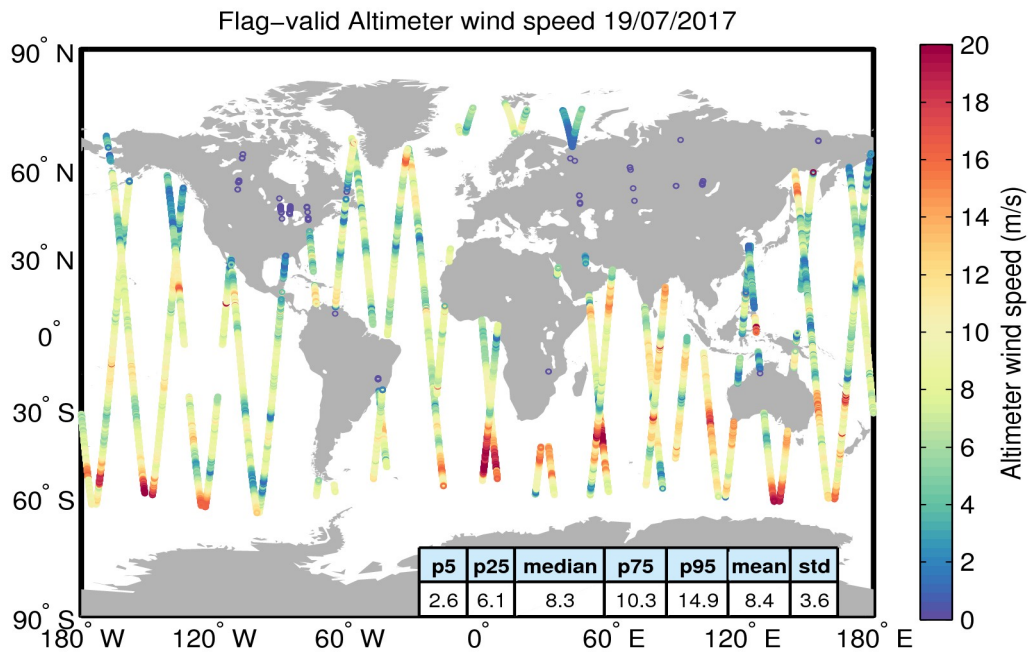
Figure 31. Geographical distribution of flag-valid wind data over oceans and lakes for 19/07/2017. The statistical values shown in the table refer to the wind in m/s and are calculated over all measurements shown in the figure.
