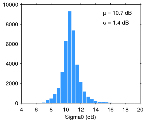
Figure 28. Histogram of science-valid sigma0 over oceans and lakes for 19/07/2017. The mean ( \mu ) and standard deviation ( \sigma ) are also shown. Note that values outside [4 20] dB are excluded from the histogram for the sake of readability but not from the computation of \mu and \sigma .
