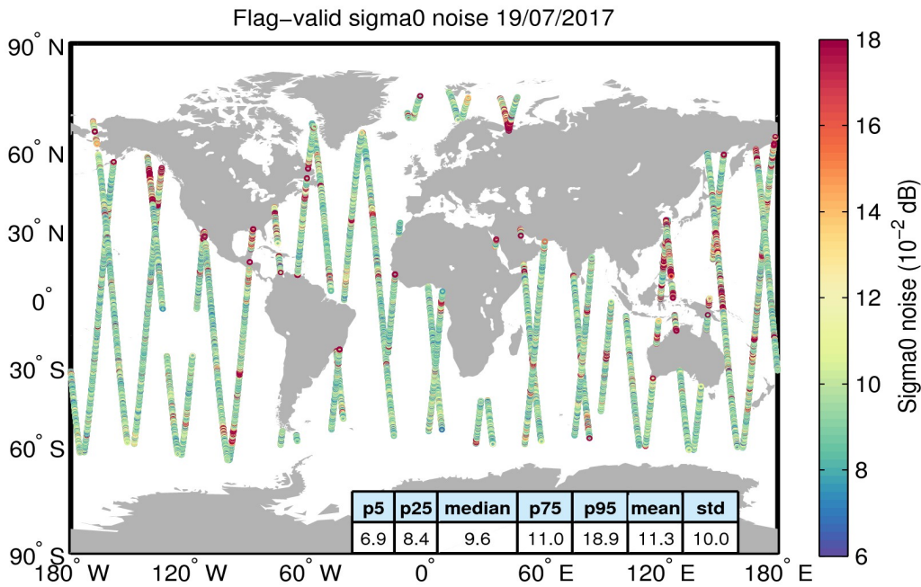
Figure 26. Geographical distribution of flag-valid 20-Hz sigma0 measurement noise over oceans and lakes for 19/07/2017. The statistical values shown in the table refer to the sigma0 noise and are calculated over all measurements shown in the figure.
