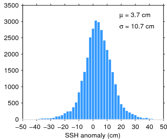
Figure 11. Histogram of science-valid SSH anomaly over oceans and lakes for 19/07/2017. The mean ( \mu ) and standard deviation ( \sigma ) are also shown. Note that values outside [-50 50] cm are excluded from the histogram for the sake of readability but not from the computation of \mu and \sigma .
