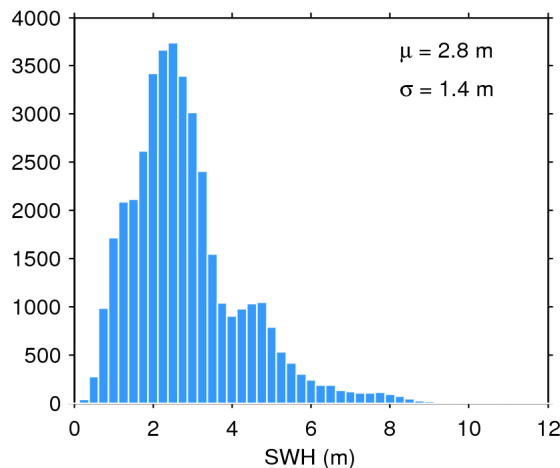
Figure 20. Histogram of science-valid SWH over oceans and lakes for 19/07/2017. The mean ( \mu ) and standard deviation ( \sigma ) are also shown. Note that values larger than 12 m are excluded from the histogram for the sake of readability but not from the computation of \mu and \sigma .
