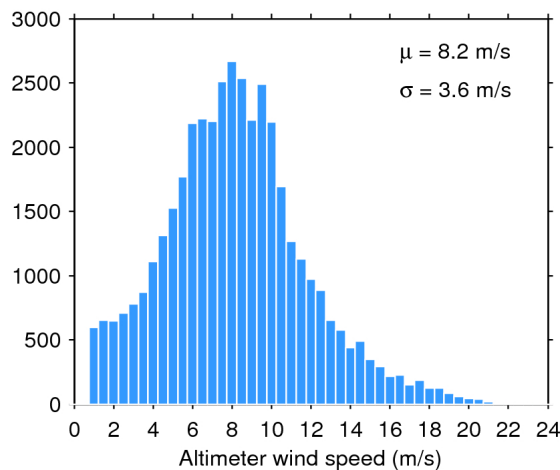
Figure 35. Histogram of science-valid wind over oceans and lakes for 18/07/2017. The mean ( \mu ) and standard deviation ( \sigma ) are also shown. Note that values larger than 24 m/s are excluded from the histogram for the sake of readability but not from the computation of \mu and \sigma .
