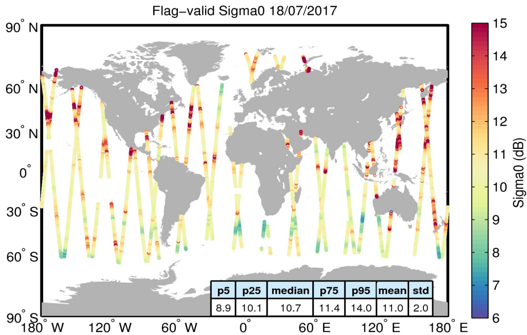
Figure 23. Geographical distribution of flag-valid sigma0 data over oceans and lakes for 18/07/2017. The statistical values shown in the table refer to the sigma0 in dB and are calculated over all measurements shown in the figure.
