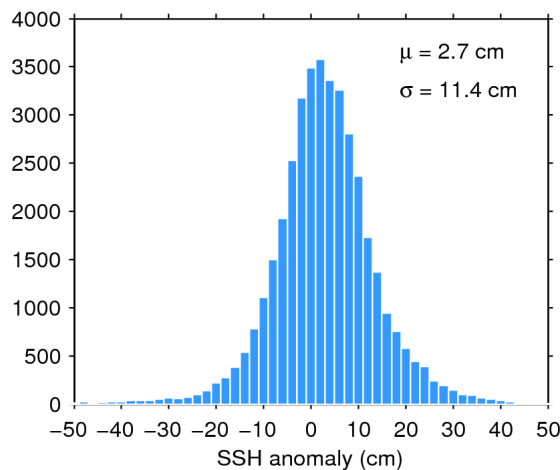
Figure 11. Histogram of science-valid SSH anomaly over oceans and lakes for 18/07/2017. The mean ( \mu ) and standard deviation ( \sigma ) are also shown. Note that values outside [-50 50] cm are excluded from the histogram for the sake of readability but not from the computation of \mu and \sigma .
