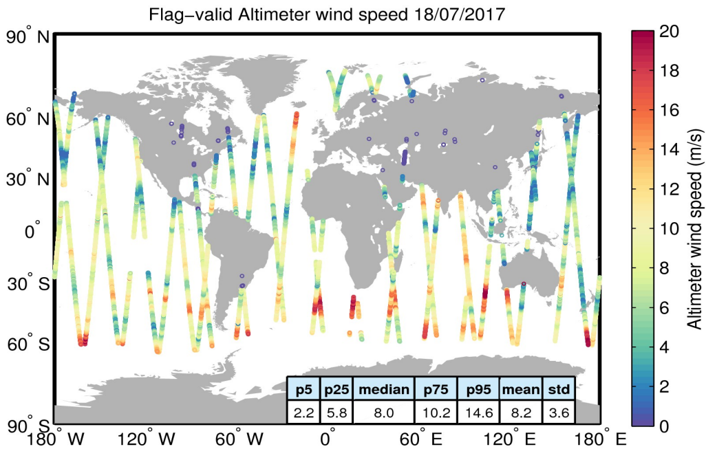
Figure 31. Geographical distribution of flag-valid wind data over oceans and lakes for 18/07/2017. The statistical values shown in the table refer to the wind in m/s and are calculated over all measurements shown in the figure.
