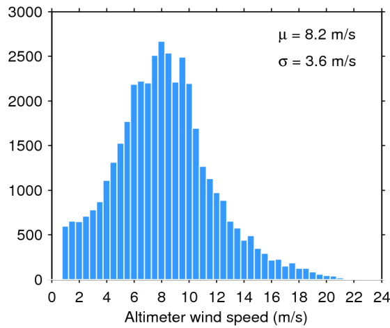
Figure 33. Histogram of flag-valid wind over oceans and lakes for 18/07/2017. The mean ( \mu ) and standard deviation ( \sigma ) are also shown. Note that values larger than 24 m/s are excluded from the histogram for the sake of readability but not from the computation of \mu and \sigma .
