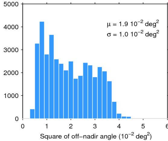
Figure 39. Histogram of flag-valid mispointing over oceans and lakes for 18/07/2017. The mean ( \mu ) and standard deviation ( \sigma ) are also shown. Note that values larger than 6 \cdot 10^{-2} \text{ deg}^2 are excluded from the histogram for the sake of readability but not from the computation of \mu and \sigma .
