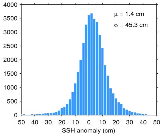
Figure 7. Histogram of flag-valid SSH anomaly over oceans and lakes for 18/07/2017. The mean ( \mu ) and standard deviation ( \sigma ) are also shown. Note that values outside [-50 50] cm are excluded from the histogram for the sake of readability but not from the computation of \mu and \sigma .
