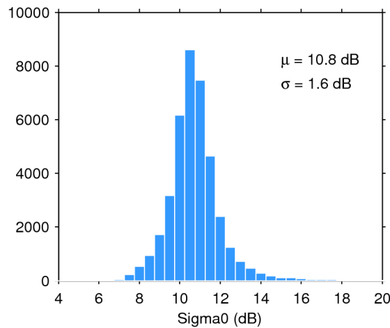
Figure 28. Histogram of science-valid sigma0 over oceans and lakes for 18/07/2017. The mean ( \mu ) and standard deviation ( \sigma ) are also shown. Note that values outside [4 20] dB are excluded from the histogram for the sake of readability but not from the computation of \mu and \sigma .
