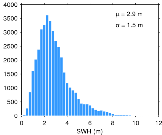
Figure 20. Histogram of science-valid SWH over oceans and lakes for 18/07/2017. The mean ( \mu ) and standard deviation ( \sigma ) are also shown. Note that values larger than 12 m are excluded from the histogram for the sake of readability but not from the computation of \mu and \sigma .
