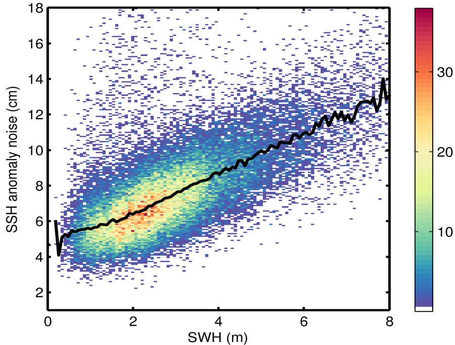
Figure 9. 2D histogram showing flag-valid SSH anomaly noise as a function of SWH for 18/07/2017. The black line denotes the median SSH anomaly noise as a function of SWH.
