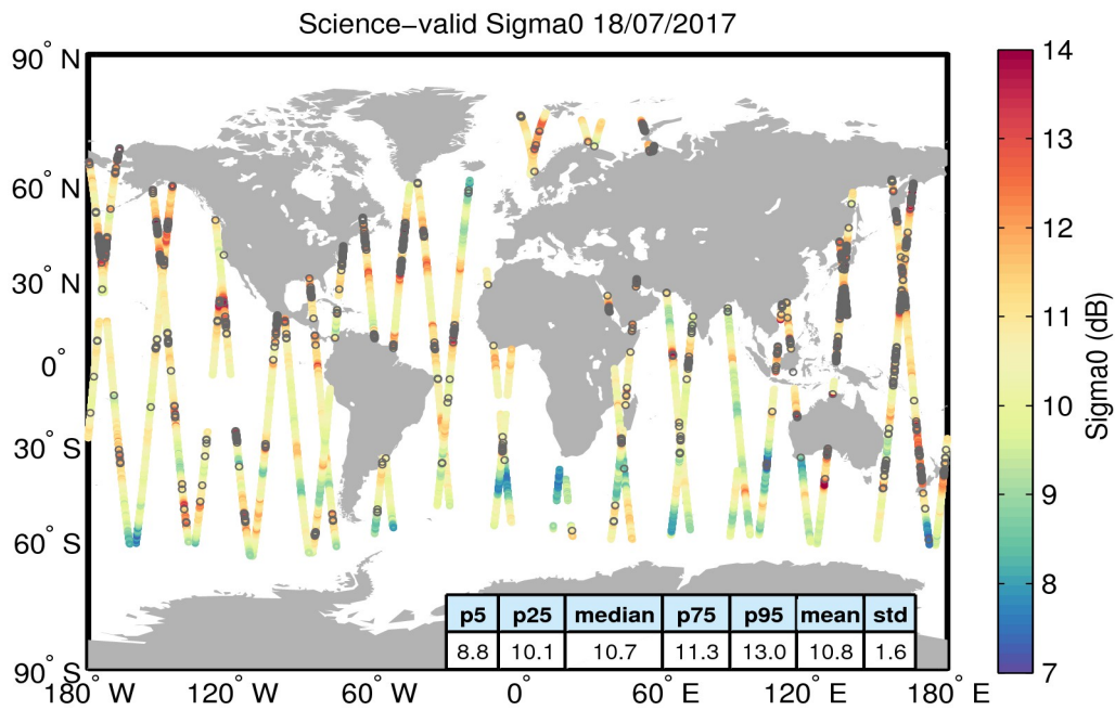
Figure 27. Geographical distribution of science-valid sigma0 data over oceans and lakes for 18/07/2017. The statistical values shown in the table refer to the sigma0 in dB and are calculated over all measurements shown in the figure. Gray circles denote records that have been rejected based on the editing criteria described in Table 4.
