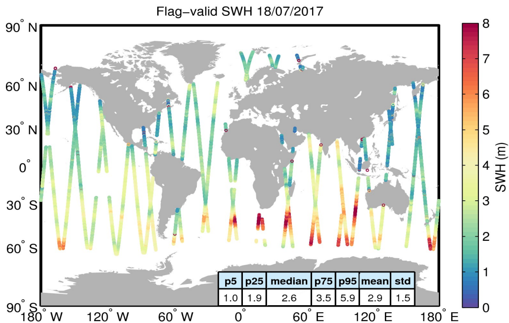
Figure 15. Geographical distribution of flag-valid SWH data over oceans and lakes for 18/07/2017. The statistical values shown in the table refer to the SWH in m and are calculated over all measurements shown in the figure.
