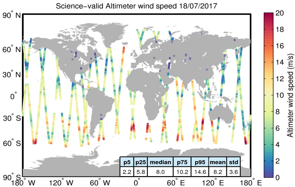
Figure 34. Geographical distribution of science-valid wind data over oceans and lakes for 18/07/2017. The statistical values shown in the table refer to the wind in m/s and are calculated over all measurements shown in the figure. Gray circles denote records that have been rejected based on the editing criteria described in Table 5.
