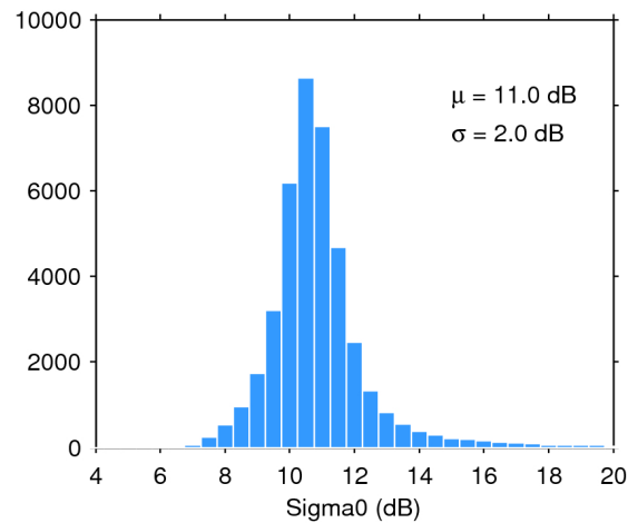
Figure 25. Histogram of flag-valid sigma0 over oceans and lakes for 18/07/2017. The mean ( \mu ) and standard deviation ( \sigma ) are also shown. Note that values outside [4 20] dB are excluded from the histogram for the sake of readability but not from the computation of \mu and \sigma .
