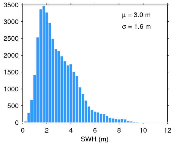
Figure 20. Histogram of science-valid SWH over oceans and lakes for 16/07/2017. The mean ( \mu ) and standard deviation ( \sigma ) are also shown. Note that values larger than 12 m are excluded from the histogram for the sake of readability but not from the computation of \mu and \sigma .
