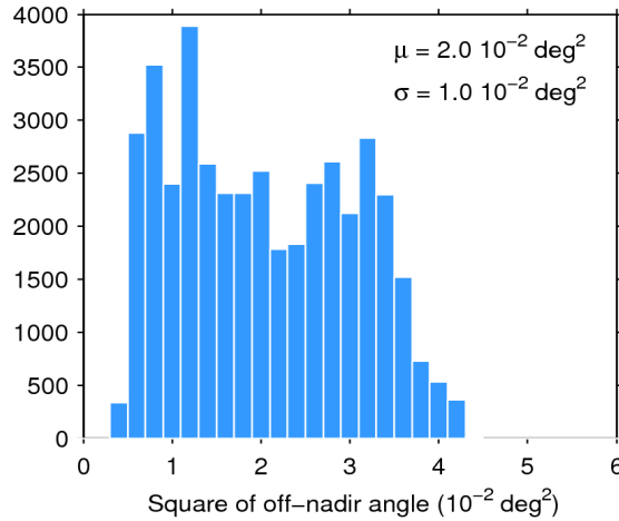
Figure 39. Histogram of flag-valid mispointing over oceans and lakes for 16/07/2017. The mean ( \mu ) and standard deviation ( \sigma ) are also shown. Note that values larger than 6 \cdot 10^{-2} \text{ deg}^2 are excluded from the histogram for the sake of readability but not from the computation of \mu and \sigma .
