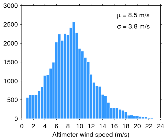
Figure 35. Histogram of science-valid wind over oceans and lakes for 16/07/2017. The mean ( \mu ) and standard deviation ( \sigma ) are also shown. Note that values larger than 24 m/s are excluded from the histogram for the sake of readability but not from the computation of \mu and \sigma .
