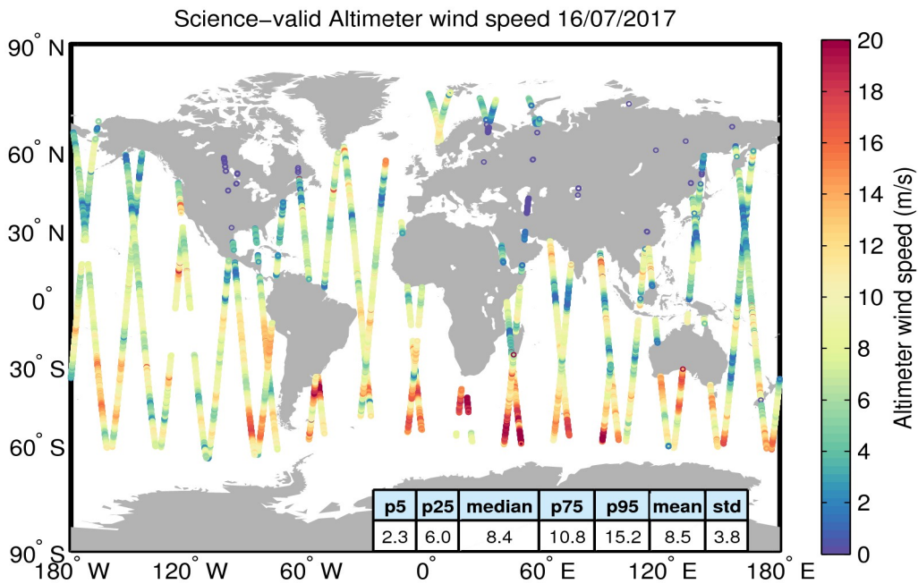
Figure 34. Geographical distribution of science-valid wind data over oceans and lakes for 16/07/2017. The statistical values shown in the table refer to the wind in m/s and are calculated over all measurements shown in the figure. Gray circles denote records that have been rejected based on the editing criteria described in Table 5.
