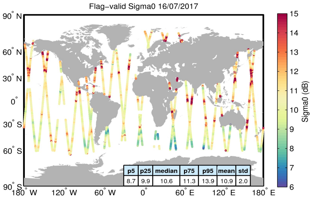
Figure 23. Geographical distribution of flag-valid sigma0 data over oceans and lakes for 16/07/2017. The statistical values shown in the table refer to the sigma0 in dB and are calculated over all measurements shown in the figure.
