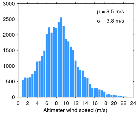
Figure 33. Histogram of flag-valid wind over oceans and lakes for 16/07/2017. The mean ( \mu ) and standard deviation ( \sigma ) are also shown. Note that values larger than 24 m/s are excluded from the histogram for the sake of readability but not from the computation of \mu and \sigma .
