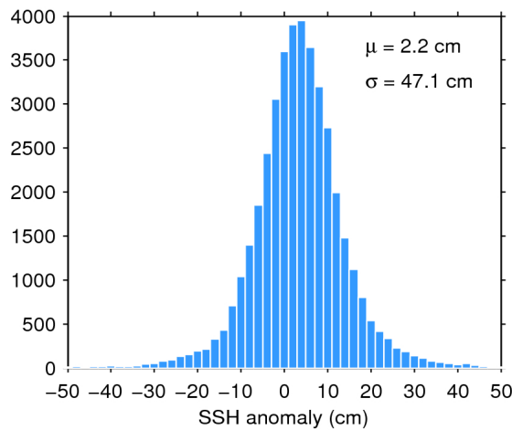
Figure 7. Histogram of flag-valid SSH anomaly over oceans and lakes for 16/07/2017. The mean ( \mu ) and standard deviation ( \sigma ) are also shown. Note that values outside [-50 50] cm are excluded from the histogram for the sake of readability but not from the computation of \mu and \sigma .
