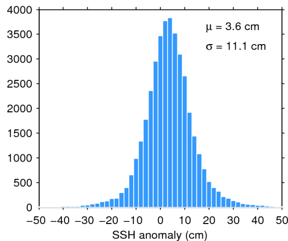
Figure 11. Histogram of science-valid SSH anomaly over oceans and lakes for 16/07/2017. The mean ( \mu ) and standard deviation ( \sigma ) are also shown. Note that values outside [-50 50] cm are excluded from the histogram for the sake of readability but not from the computation of \mu and \sigma .
