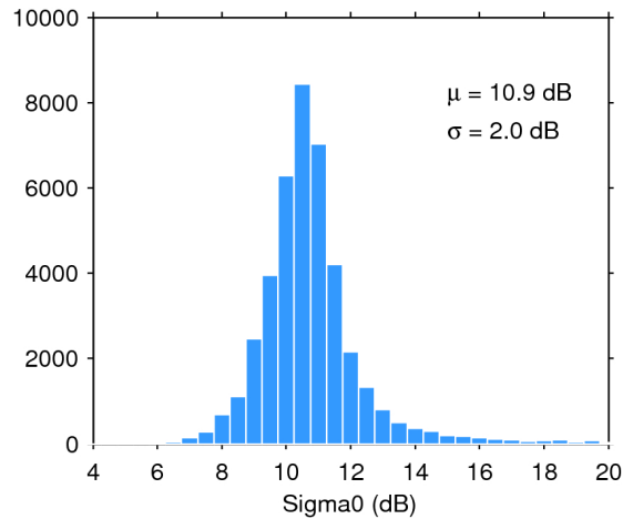
Figure 25. Histogram of flag-valid sigma0 over oceans and lakes for 16/07/2017. The mean ( \mu ) and standard deviation ( \sigma ) are also shown. Note that values outside [4 20] dB are excluded from the histogram for the sake of readability but not from the computation of \mu and \sigma .
