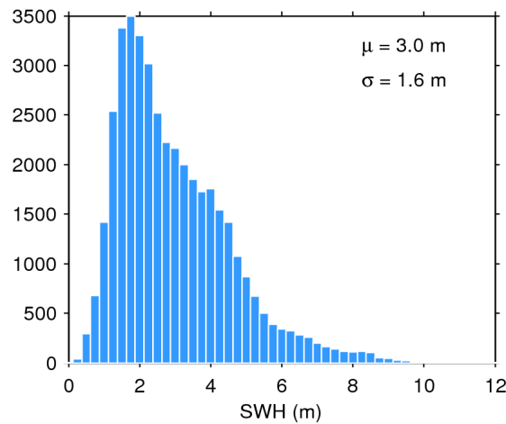
Figure 17. Histogram of flag-valid SWH over oceans and lakes for 16/07/2017. The mean ( \mu ) and standard deviation ( \sigma ) are also shown. Note that values larger than 12 m are excluded from the histogram for the sake of readability but not from the computation of \mu and \sigma .
