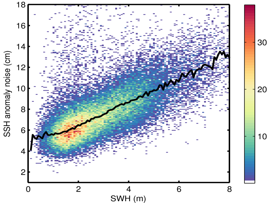
Figure 9. 2D histogram showing flag-valid SSH anomaly noise as a function of SWH for 16/07/2017. The black line denotes the median SSH anomaly noise as a function of SWH.
