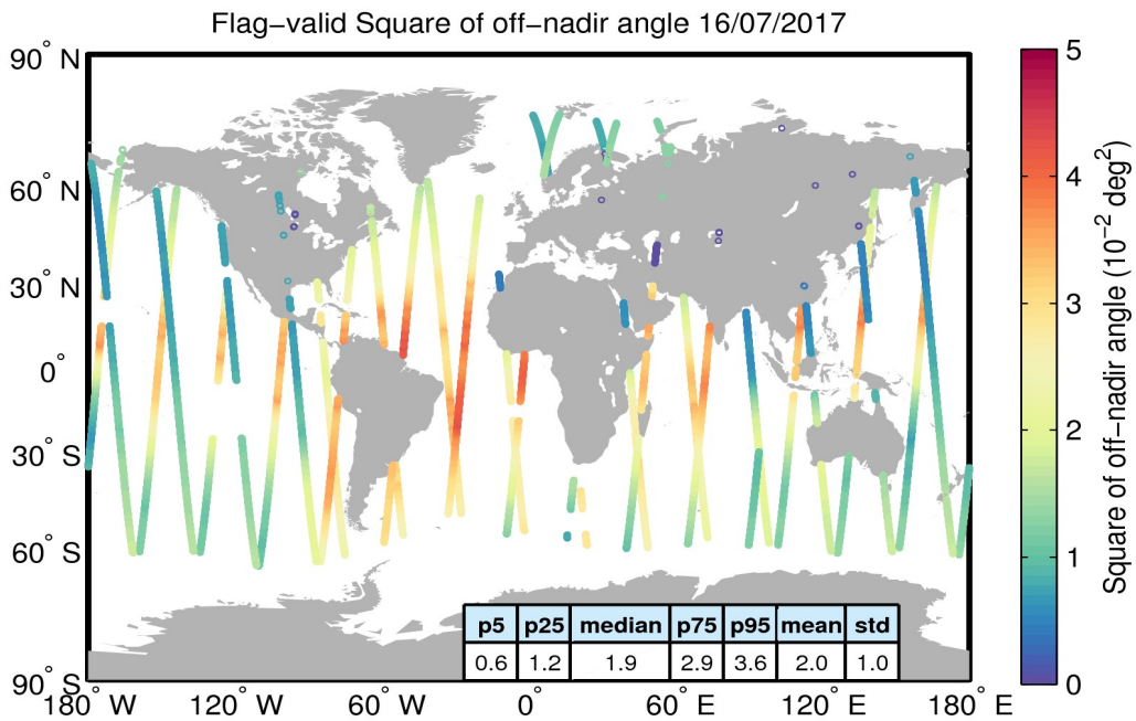
Figure 37. Geographical distribution of flag-valid mispointing data over oceans and lakes for 16/07/2017. The statistical values shown in the table refer to the mispointing in 10^{-2} deg 2 and are calculated over all measurements shown in the figure.
