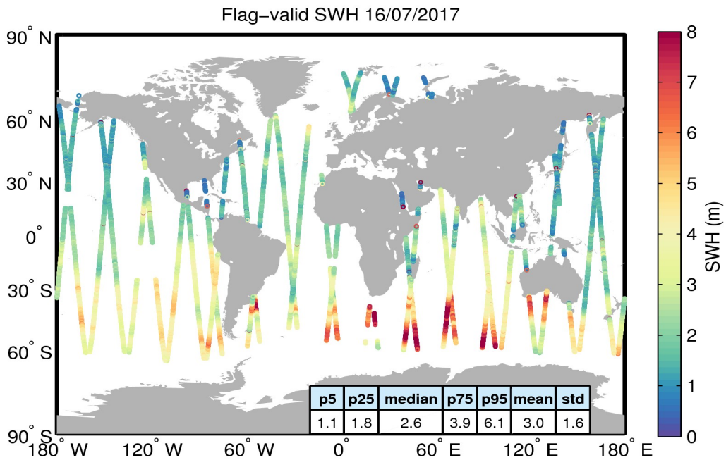
Figure 15. Geographical distribution of flag-valid SWH data over oceans and lakes for 16/07/2017. The statistical values shown in the table refer to the SWH in m and are calculated over all measurements shown in the figure.
