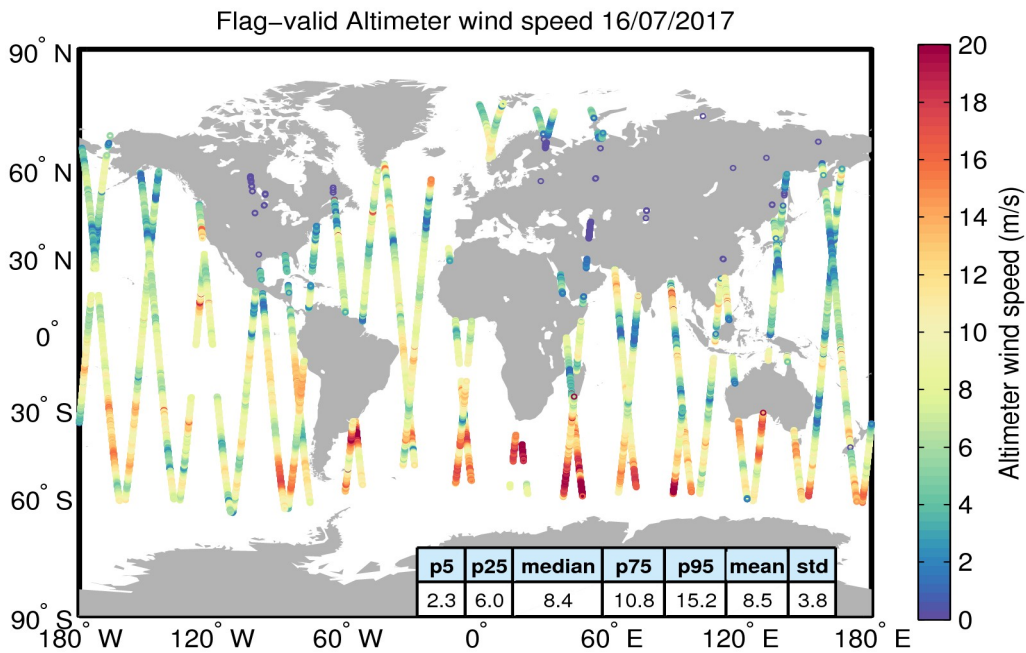
Figure 31. Geographical distribution of flag-valid wind data over oceans and lakes for 16/07/2017. The statistical values shown in the table refer to the wind in m/s and are calculated over all measurements shown in the figure.
