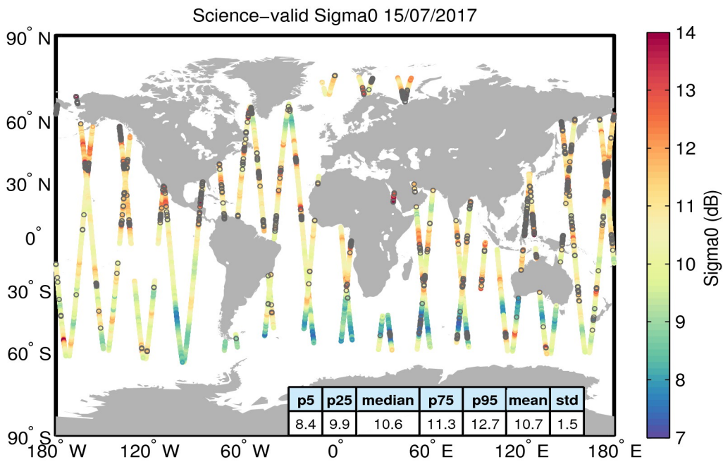
Figure 27. Geographical distribution of science-valid sigma0 data over oceans and lakes for 15/07/2017. The statistical values shown in the table refer to the sigma0 in dB and are calculated over all measurements shown in the figure. Gray circles denote records that have been rejected based on the editing criteria described in Table 4.
