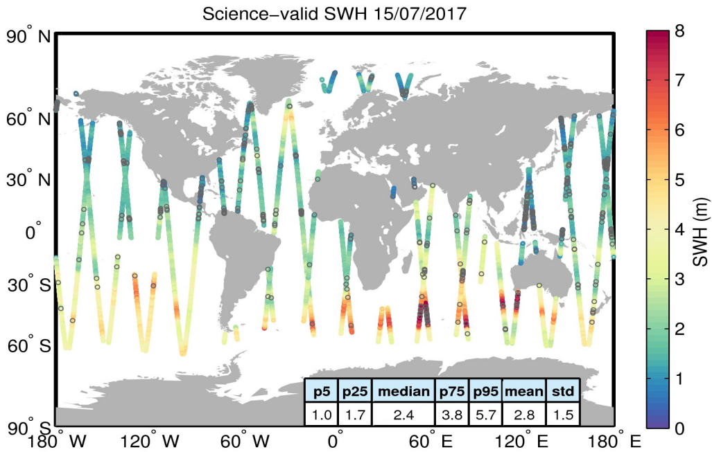
Figure 19. Geographical distribution of science-valid SWH data over oceans and lakes for 15/07/2017. The statistical values shown in the table refer to the SWH in m and are calculated over all measurements shown in the figure. Gray circles denote records that have been rejected based on the editing criteria described in Table 3.
