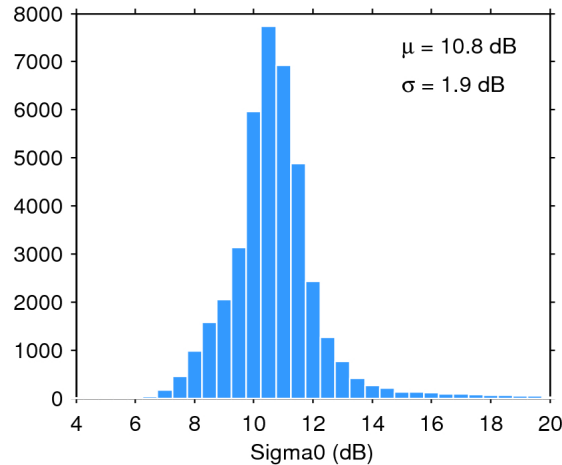
Figure 25. Histogram of flag-valid sigma0 over oceans and lakes for 15/07/2017. The mean ( \mu ) and standard deviation ( \sigma ) are also shown. Note that values outside [4 20] dB are excluded from the histogram for the sake of readability but not from the computation of \mu and \sigma .
