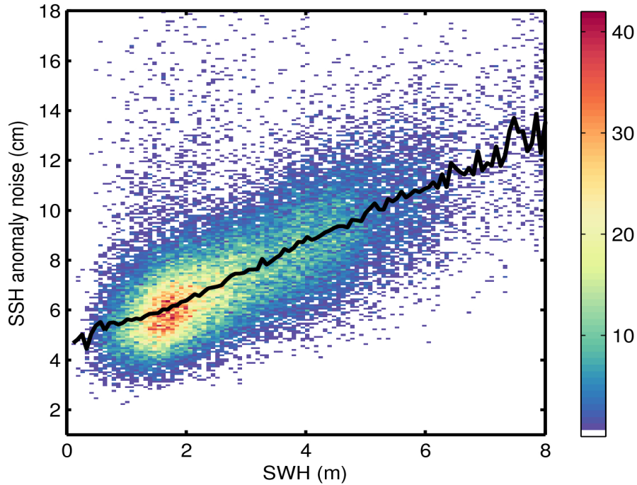
Figure 9. 2D histogram showing flag-valid SSH anomaly noise as a function of SWH for 15/07/2017. The black line denotes the median SSH anomaly noise as a function of SWH.
