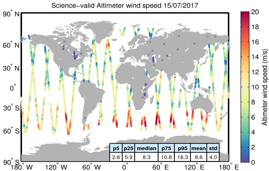
Figure 34. Geographical distribution of science-valid wind data over oceans and lakes for 15/07/2017. The statistical values shown in the table refer to the wind in m/s and are calculated over all measurements shown in the figure. Gray circles denote records that have been rejected based on the editing criteria described in Table 5.
