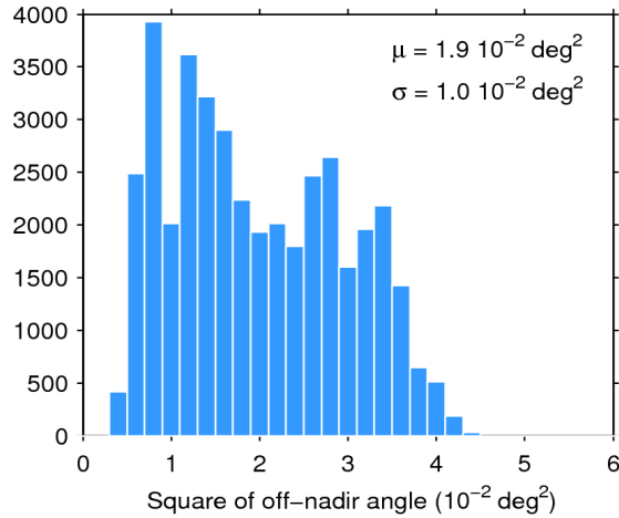
Figure 39. Histogram of flag-valid mispointing over oceans and lakes for 15/07/2017. The mean ( \mu ) and standard deviation ( \sigma ) are also shown. Note that values larger than 6 \cdot 10^{-2} \text{ deg}^2 are excluded from the histogram for the sake of readability but not from the computation of \mu and \sigma .
