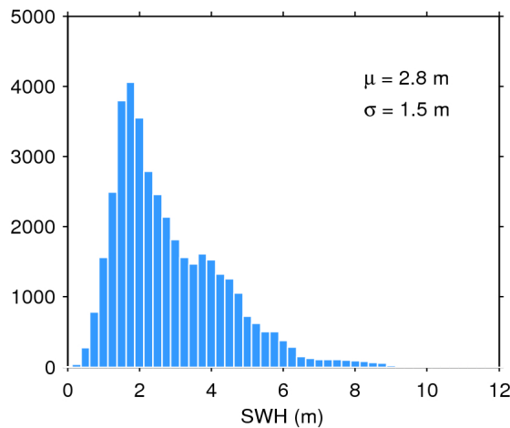
Figure 20. Histogram of science-valid SWH over oceans and lakes for 15/07/2017. The mean ( \mu ) and standard deviation ( \sigma ) are also shown. Note that values larger than 12 m are excluded from the histogram for the sake of readability but not from the computation of \mu and \sigma .
