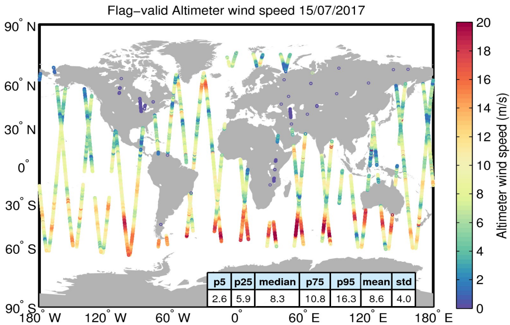
Figure 31. Geographical distribution of flag-valid wind data over oceans and lakes for 15/07/2017. The statistical values shown in the table refer to the wind in m/s and are calculated over all measurements shown in the figure.
