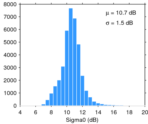
Figure 28. Histogram of science-valid sigma0 over oceans and lakes for 15/07/2017. The mean ( \mu ) and standard deviation ( \sigma ) are also shown. Note that values outside [4 20] dB are excluded from the histogram for the sake of readability but not from the computation of \mu and \sigma .
