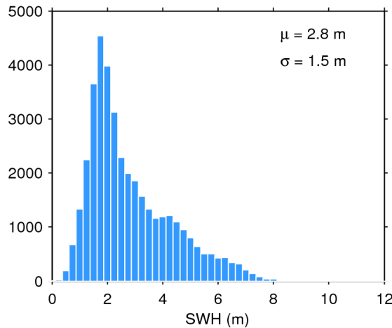
Figure 20. Histogram of science-valid SWH over oceans and lakes for 14/07/2017. The mean ( \mu ) and standard deviation ( \sigma ) are also shown. Note that values larger than 12 m are excluded from the histogram for the sake of readability but not from the computation of \mu and \sigma .
