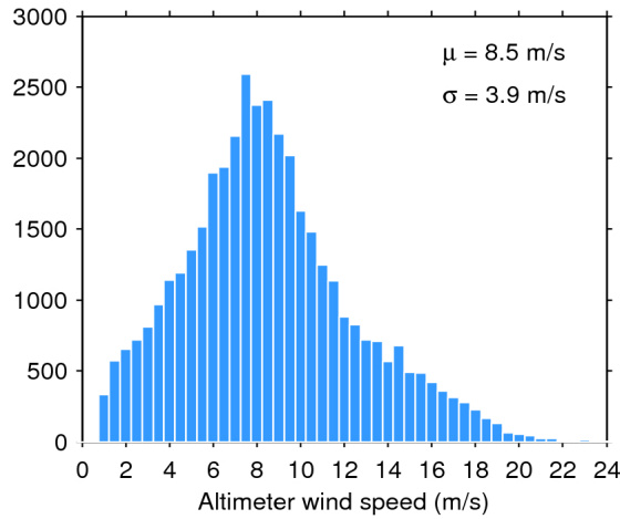
Figure 33. Histogram of flag-valid wind over oceans and lakes for 14/07/2017. The mean ( \mu ) and standard deviation ( \sigma ) are also shown. Note that values larger than 24 m/s are excluded from the histogram for the sake of readability but not from the computation of \mu and \sigma .
