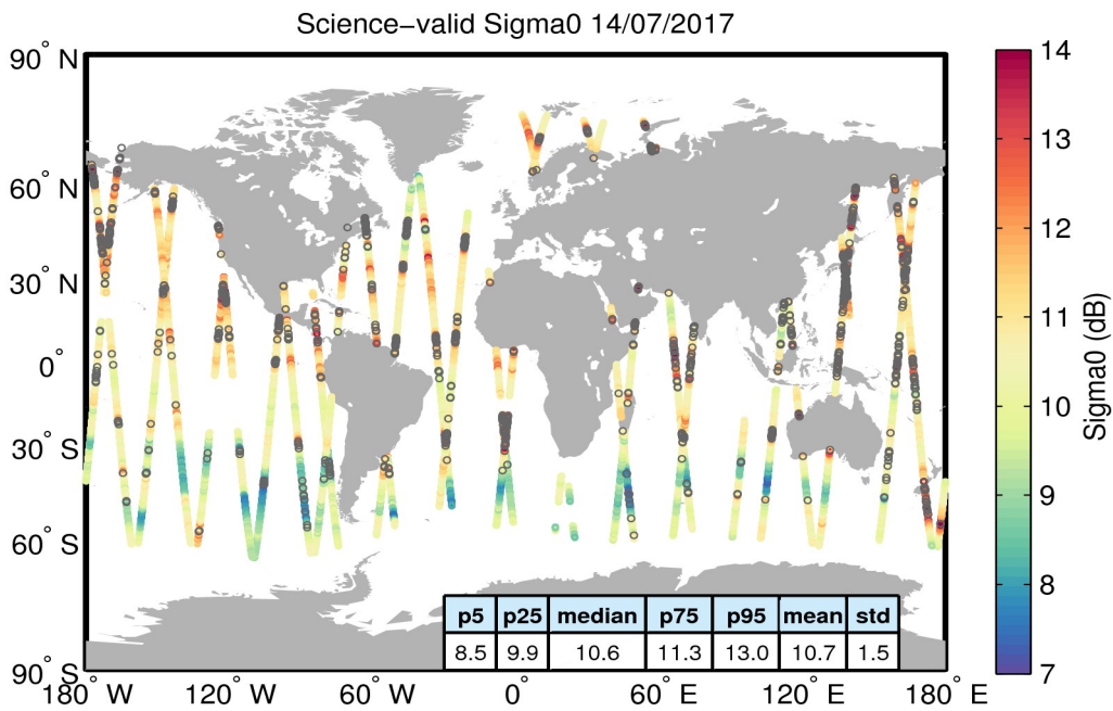
Figure 27. Geographical distribution of science-valid sigma0 data over oceans and lakes for 14/07/2017. The statistical values shown in the table refer to the sigma0 in dB and are calculated over all measurements shown in the figure. Gray circles denote records that have been rejected based on the editing criteria described in Table 4.
