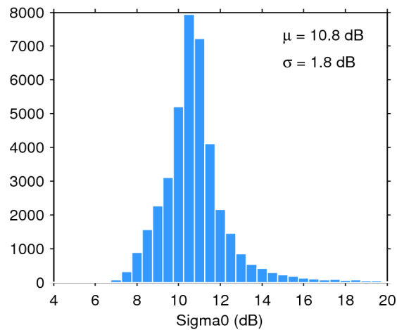
Figure 25. Histogram of flag-valid sigma0 over oceans and lakes for 14/07/2017. The mean ( \mu ) and standard deviation ( \sigma ) are also shown. Note that values outside [4 20] dB are excluded from the histogram for the sake of readability but not from the computation of \mu and \sigma .
