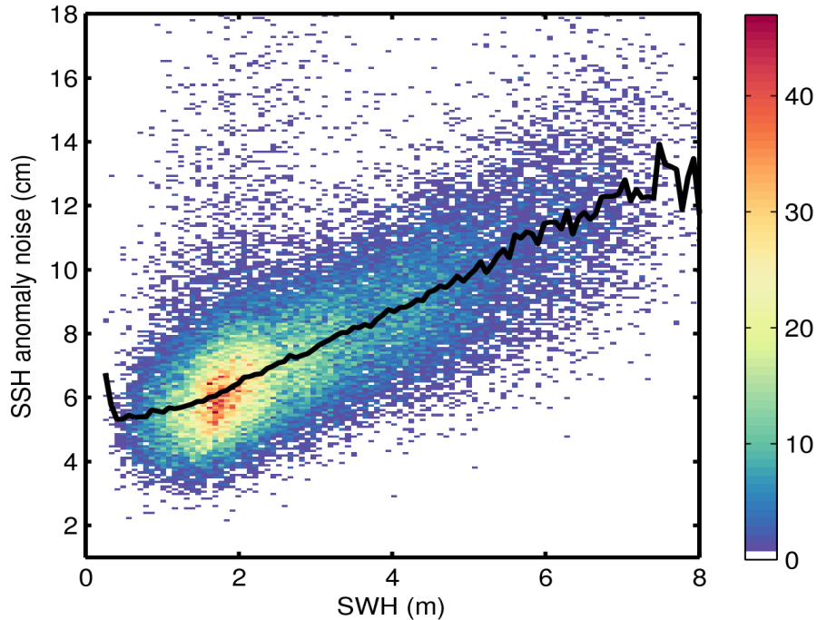
Figure 9. 2D histogram showing flag-valid SSH anomaly noise as a function of SWH for 14/07/2017. The black line denotes the median SSH anomaly noise as a function of SWH.
