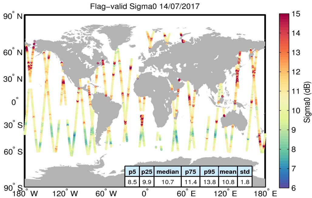
Figure 23. Geographical distribution of flag-valid sigma0 data over oceans and lakes for 14/07/2017. The statistical values shown in the table refer to the sigma0 in dB and are calculated over all measurements shown in the figure.
