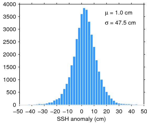
Figure 7. Histogram of flag-valid SSH anomaly over oceans and lakes for 14/07/2017. The mean ( \mu ) and standard deviation ( \sigma ) are also shown. Note that values outside [-50 50] cm are excluded from the histogram for the sake of readability but not from the computation of \mu and \sigma .
