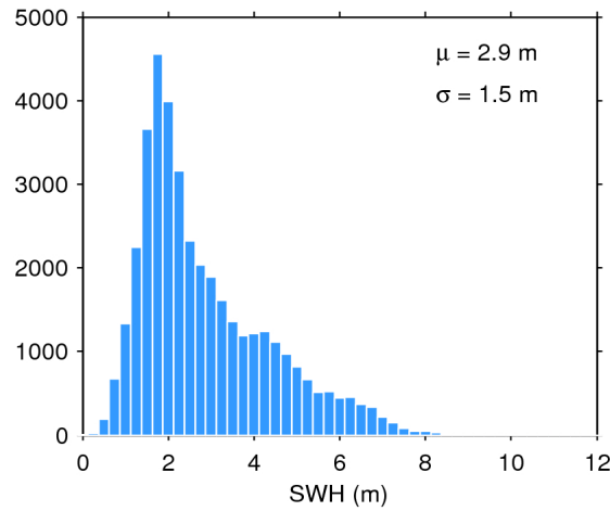
Figure 17. Histogram of flag-valid SWH over oceans and lakes for 14/07/2017. The mean ( \mu ) and standard deviation ( \sigma ) are also shown. Note that values larger than 12 m are excluded from the histogram for the sake of readability but not from the computation of \mu and \sigma .
