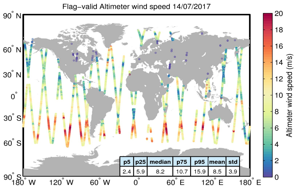
Figure 31. Geographical distribution of flag-valid wind data over oceans and lakes for 14/07/2017. The statistical values shown in the table refer to the wind in m/s and are calculated over all measurements shown in the figure.
