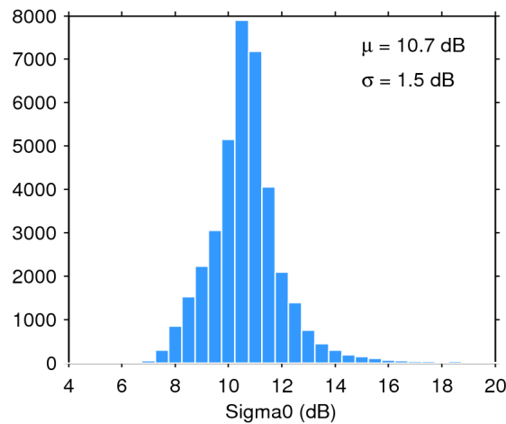
Figure 28. Histogram of science-valid sigma0 over oceans and lakes for 14/07/2017. The mean ( \mu ) and standard deviation ( \sigma ) are also shown. Note that values outside [4 20] dB are excluded from the histogram for the sake of readability but not from the computation of \mu and \sigma .
