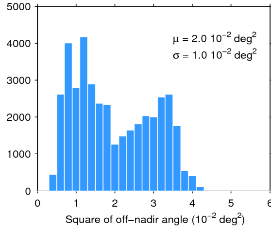
Figure 39. Histogram of flag-valid mispointing over oceans and lakes for 14/07/2017. The mean ( \mu ) and standard deviation ( \sigma ) are also shown. Note that values larger than 6 \cdot 10^{-2} \text{ deg}^2 are excluded from the histogram for the sake of readability but not from the computation of \mu and \sigma .
