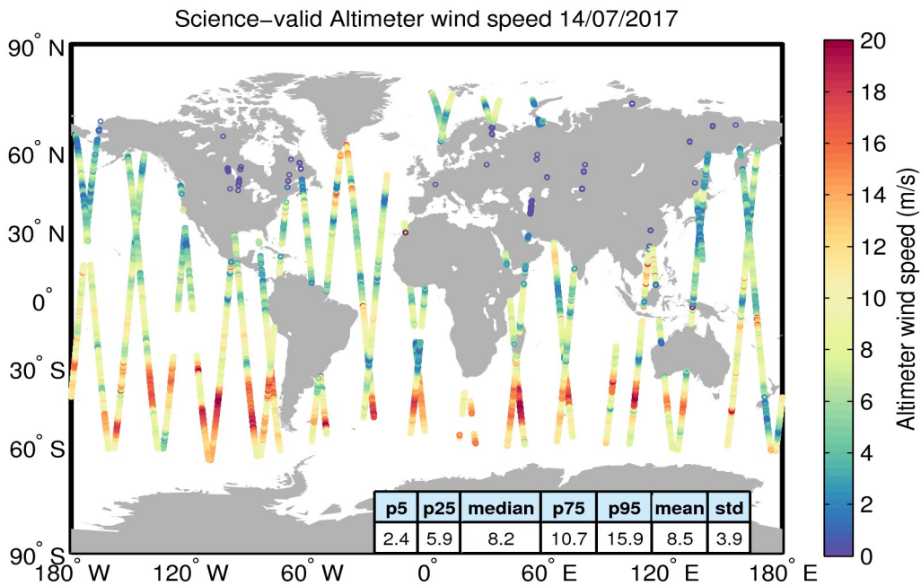
Figure 34. Geographical distribution of science-valid wind data over oceans and lakes for 14/07/2017. The statistical values shown in the table refer to the wind in m/s and are calculated over all measurements shown in the figure. Gray circles denote records that have been rejected based on the editing criteria described in Table 5.
