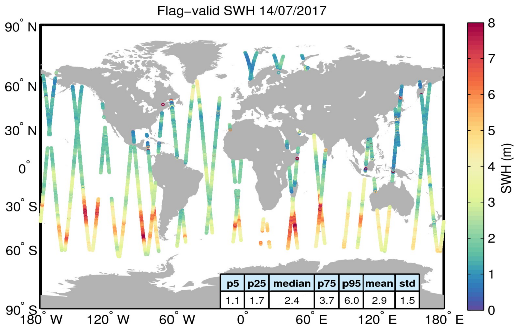
Figure 15. Geographical distribution of flag-valid SWH data over oceans and lakes for 14/07/2017. The statistical values shown in the table refer to the SWH in m and are calculated over all measurements shown in the figure.
