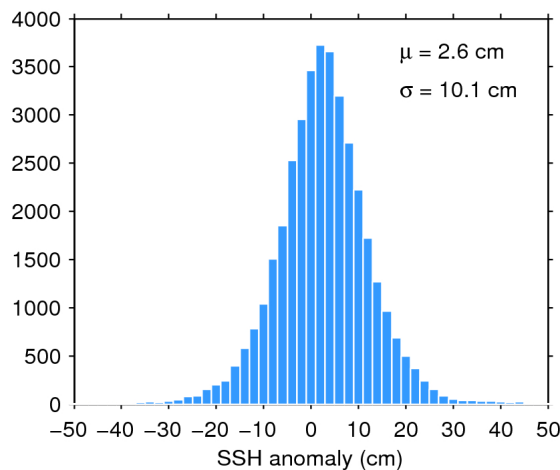
Figure 11. Histogram of science-valid SSH anomaly over oceans and lakes for 14/07/2017. The mean ( \mu ) and standard deviation ( \sigma ) are also shown. Note that values outside [-50 50] cm are excluded from the histogram for the sake of readability but not from the computation of \mu and \sigma .
