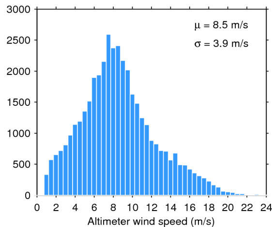
Figure 35. Histogram of science-valid wind over oceans and lakes for 14/07/2017. The mean ( \mu ) and standard deviation ( \sigma ) are also shown. Note that values larger than 24 m/s are excluded from the histogram for the sake of readability but not from the computation of \mu and \sigma .
