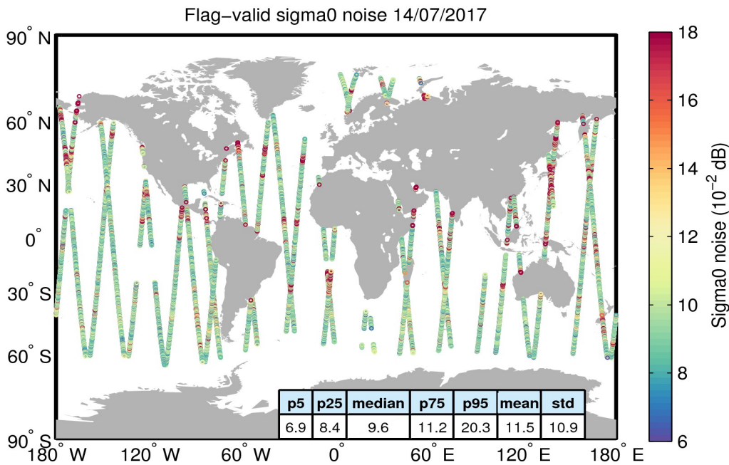
Figure 26. Geographical distribution of flag-valid 20-Hz sigma0 measurement noise over oceans and lakes for 14/07/2017. The statistical values shown in the table refer to the sigma0 noise and are calculated over all measurements shown in the figure.
