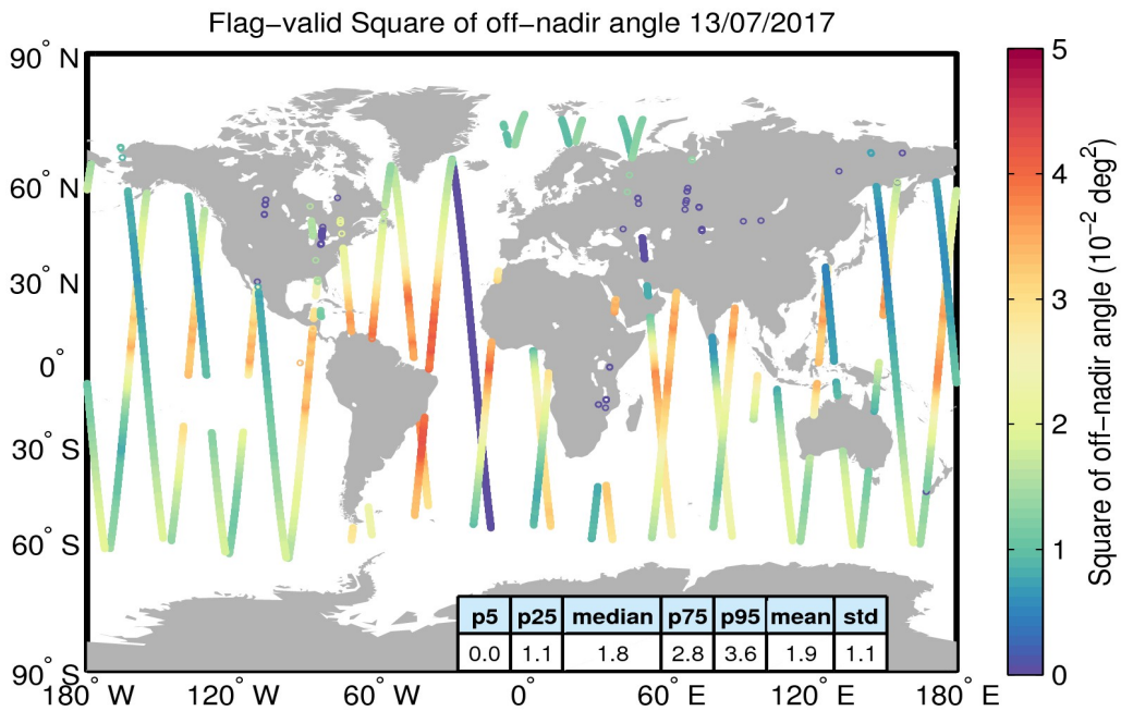
Figure 37. Geographical distribution of flag-valid mispointing data over oceans and lakes for 13/07/2017. The statistical values shown in the table refer to the mispointing in 10^{-2} deg 2 and are calculated over all measurements shown in the figure.
