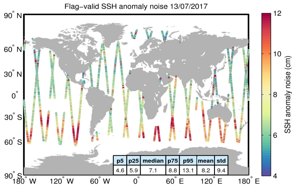
Figure 8. Geographical distribution of flag-valid 20-Hz SSH anomaly measurement noise over oceans and lakes for 13/07/2017. The statistical values shown in the table refer to the SSH anomaly noise and are calculated over all measurements shown in the figure.
