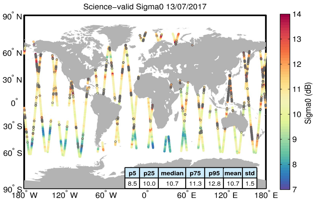
Figure 27. Geographical distribution of science-valid sigma0 data over oceans and lakes for 13/07/2017. The statistical values shown in the table refer to the sigma0 in dB and are calculated over all measurements shown in the figure. Gray circles denote records that have been rejected based on the editing criteria described in Table 4.
