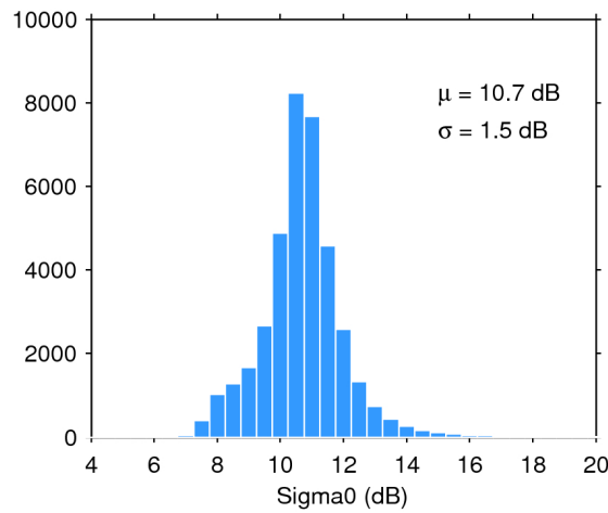
Figure 28. Histogram of science-valid sigma0 over oceans and lakes for 13/07/2017. The mean ( \mu ) and standard deviation ( \sigma ) are also shown. Note that values outside [4 20] dB are excluded from the histogram for the sake of readability but not from the computation of \mu and \sigma .
