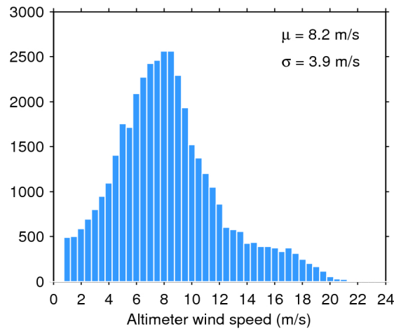
Figure 33. Histogram of flag-valid wind over oceans and lakes for 13/07/2017. The mean ( \mu ) and standard deviation ( \sigma ) are also shown. Note that values larger than 24 m/s are excluded from the histogram for the sake of readability but not from the computation of \mu and \sigma .
