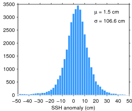
Figure 7. Histogram of flag-valid SSH anomaly over oceans and lakes for 13/07/2017. The mean ( \mu ) and standard deviation ( \sigma ) are also shown. Note that values outside [-50 50] cm are excluded from the histogram for the sake of readability but not from the computation of \mu and \sigma .
