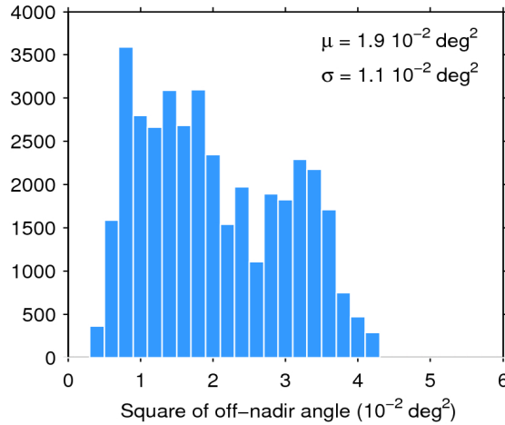
Figure 39. Histogram of flag-valid mispointing over oceans and lakes for 13/07/2017. The mean ( \mu ) and standard deviation ( \sigma ) are also shown. Note that values larger than 6 \cdot 10^{-2} \text{ deg}^2 are excluded from the histogram for the sake of readability but not from the computation of \mu and \sigma .
