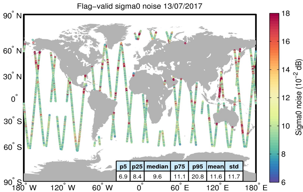
Figure 26. Geographical distribution of flag-valid 20-Hz sigma0 measurement noise over oceans and lakes for 13/07/2017. The statistical values shown in the table refer to the sigma0 noise and are calculated over all measurements shown in the figure.
