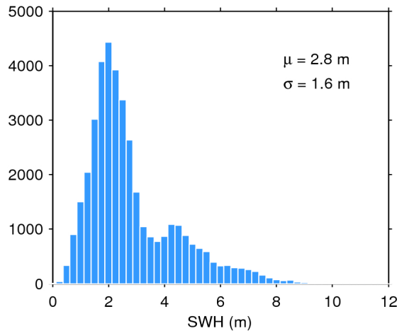
Figure 20. Histogram of science-valid SWH over oceans and lakes for 13/07/2017. The mean ( \mu ) and standard deviation ( \sigma ) are also shown. Note that values larger than 12 m are excluded from the histogram for the sake of readability but not from the computation of \mu and \sigma .
