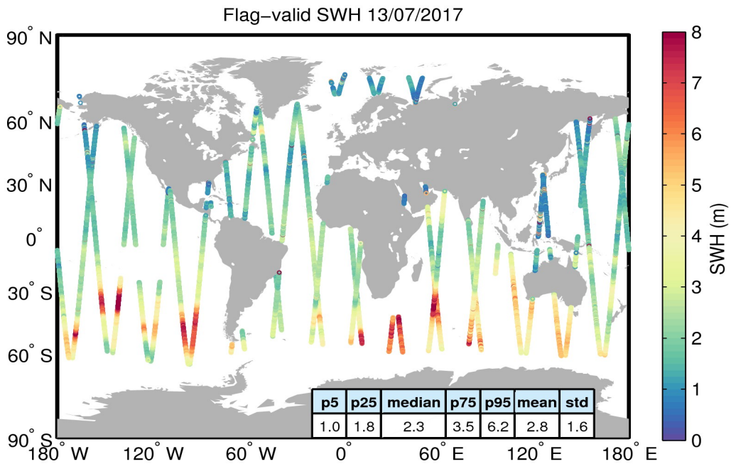
Figure 15. Geographical distribution of flag-valid SWH data over oceans and lakes for 13/07/2017. The statistical values shown in the table refer to the SWH in m and are calculated over all measurements shown in the figure.
