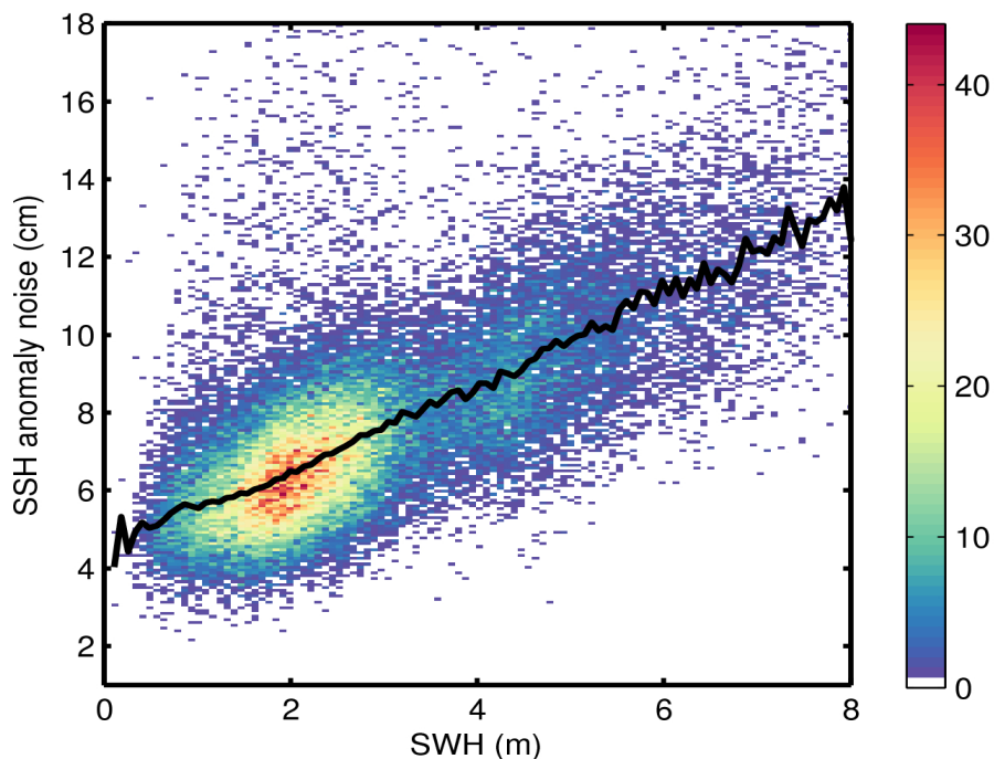
Figure 9. 2D histogram showing flag-valid SSH anomaly noise as a function of SWH for 13/07/2017. The black line denotes the median SSH anomaly noise as a function of SWH.
