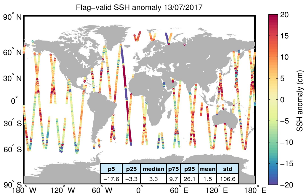
Figure 5. Geographical distribution of flag-valid 1-Hz SSH anomaly data over oceans and lakes for 13/07/2017. The statistical values shown in the table refer to the SSH anomaly in cm and are calculated over all measurements shown in the figure.
