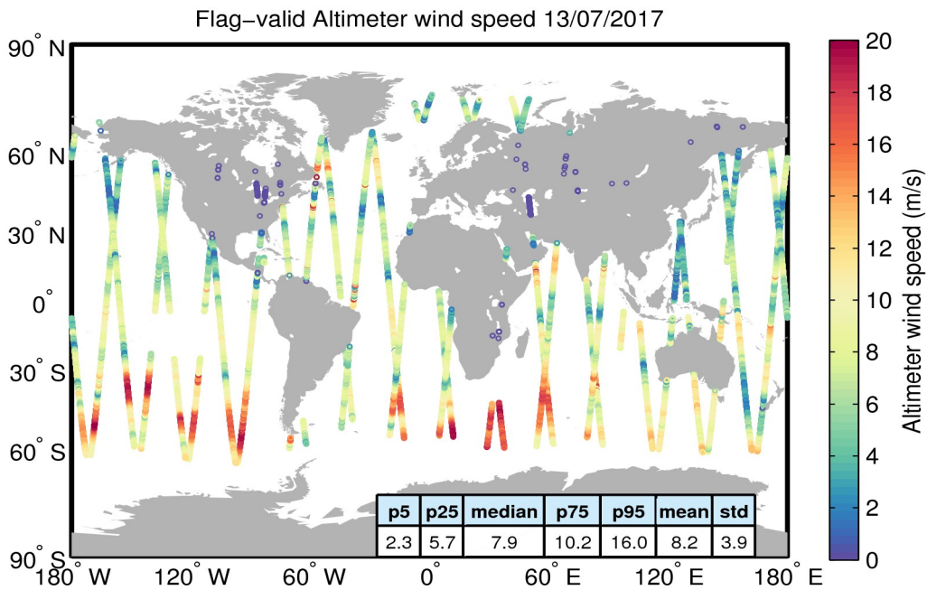
Figure 31. Geographical distribution of flag-valid wind data over oceans and lakes for 13/07/2017. The statistical values shown in the table refer to the wind in m/s and are calculated over all measurements shown in the figure.
