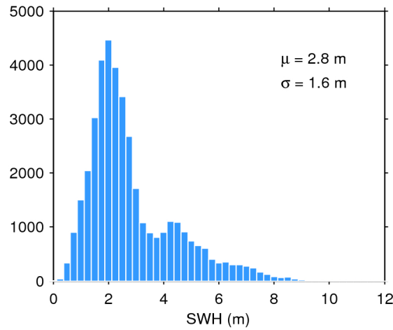
Figure 17. Histogram of flag-valid SWH over oceans and lakes for 13/07/2017. The mean ( \mu ) and standard deviation ( \sigma ) are also shown. Note that values larger than 12 m are excluded from the histogram for the sake of readability but not from the computation of \mu and \sigma .
