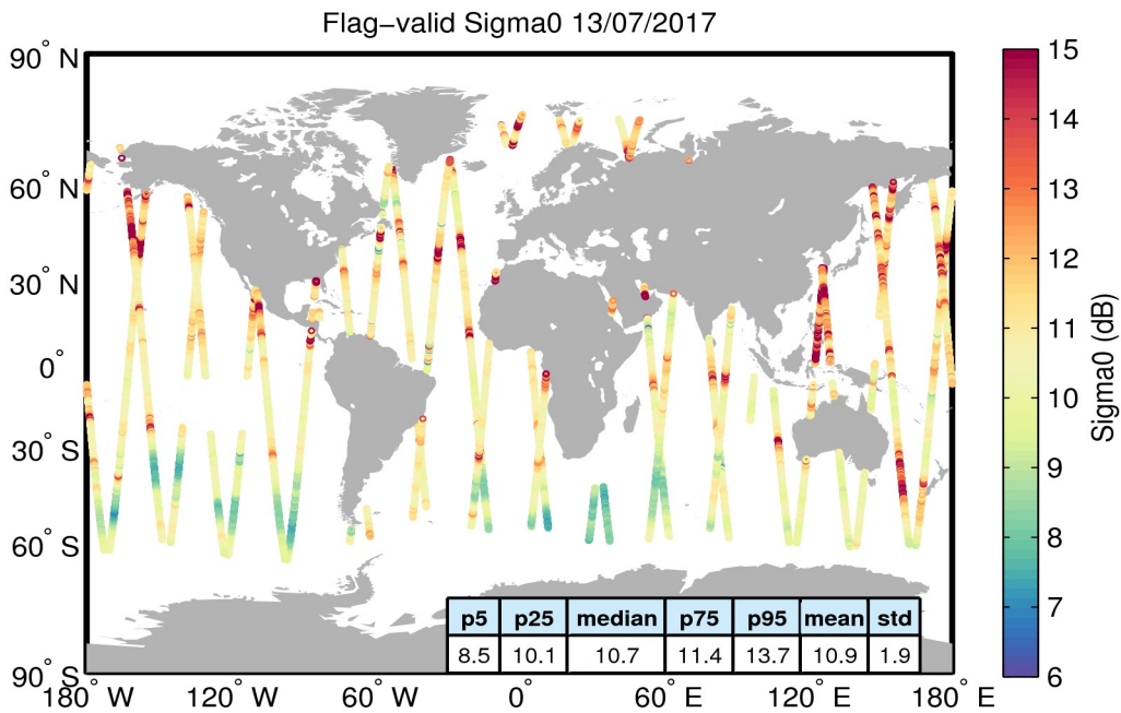
Figure 23. Geographical distribution of flag-valid sigma0 data over oceans and lakes for 13/07/2017. The statistical values shown in the table refer to the sigma0 in dB and are calculated over all measurements shown in the figure.
