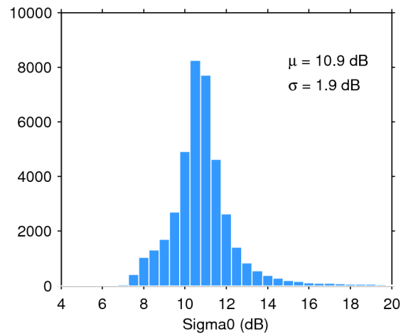
Figure 25. Histogram of flag-valid sigma0 over oceans and lakes for 13/07/2017. The mean ( \mu ) and standard deviation ( \sigma ) are also shown. Note that values outside [4 20] dB are excluded from the histogram for the sake of readability but not from the computation of \mu and \sigma .
