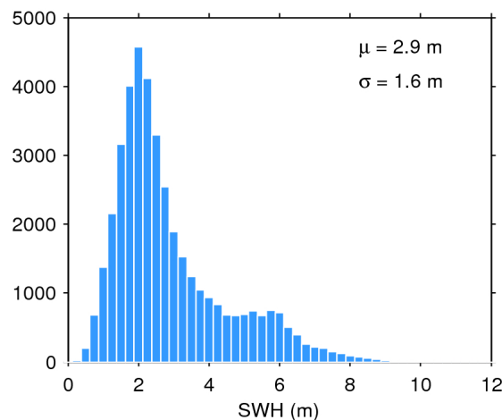
Figure 20. Histogram of science-valid SWH over oceans and lakes for 12/07/2017. The mean ( \mu ) and standard deviation ( \sigma ) are also shown. Note that values larger than 12 m are excluded from the histogram for the sake of readability but not from the computation of \mu and \sigma .
