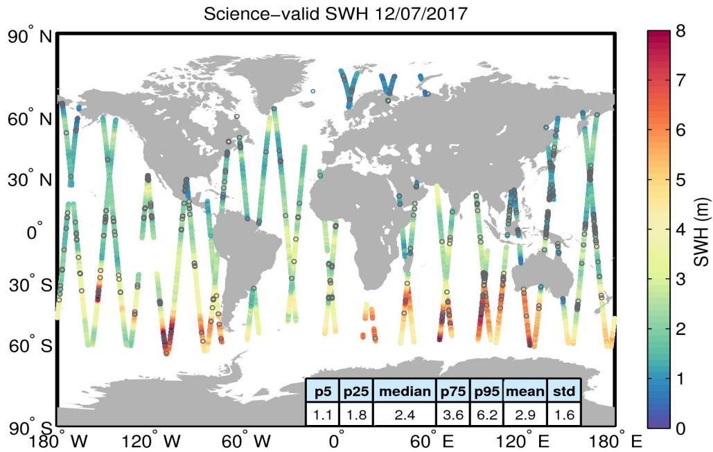
Figure 19. Geographical distribution of science-valid SWH data over oceans and lakes for 12/07/2017. The statistical values shown in the table refer to the SWH in m and are calculated over all measurements shown in the figure. Gray circles denote records that have been rejected based on the editing criteria described in Table 3.
