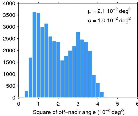
Figure 39. Histogram of flag-valid mispointing over oceans and lakes for 12/07/2017. The mean ( \mu ) and standard deviation ( \sigma ) are also shown. Note that values larger than 6 \cdot 10^{-2} \text{ deg}^2 are excluded from the histogram for the sake of readability but not from the computation of \mu and \sigma .
