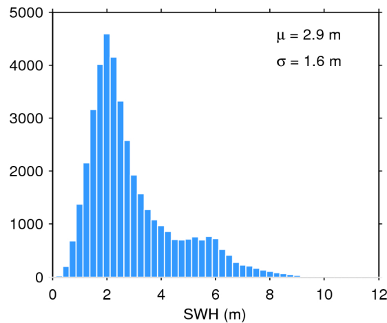
Figure 17. Histogram of flag-valid SWH over oceans and lakes for 12/07/2017. The mean ( \mu ) and standard deviation ( \sigma ) are also shown. Note that values larger than 12 m are excluded from the histogram for the sake of readability but not from the computation of \mu and \sigma .
