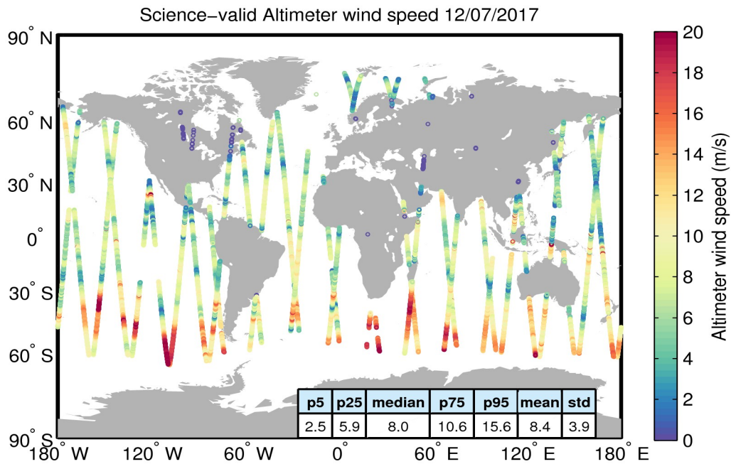
Figure 34. Geographical distribution of science-valid wind data over oceans and lakes for 12/07/2017. The statistical values shown in the table refer to the wind in m/s and are calculated over all measurements shown in the figure. Gray circles denote records that have been rejected based on the editing criteria described in Table 5.
