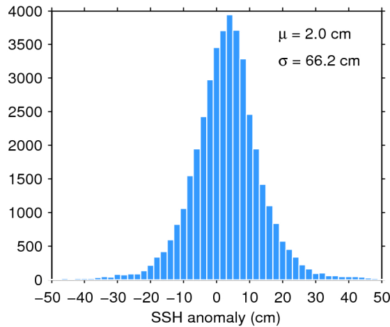
Figure 7. Histogram of flag-valid SSH anomaly over oceans and lakes for 12/07/2017. The mean ( \mu ) and standard deviation ( \sigma ) are also shown. Note that values outside [-50 50] cm are excluded from the histogram for the sake of readability but not from the computation of \mu and \sigma .
