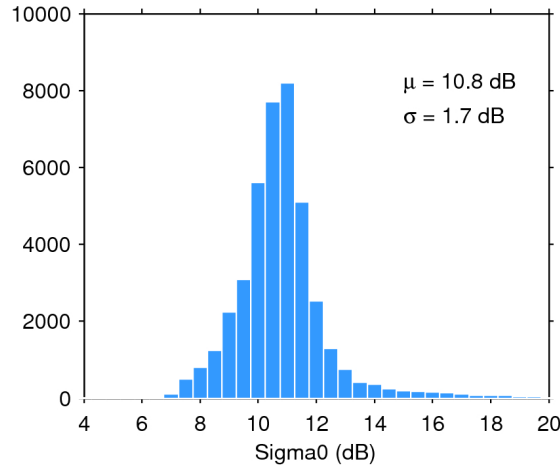
Figure 25. Histogram of flag-valid sigma0 over oceans and lakes for 12/07/2017. The mean ( \mu ) and standard deviation ( \sigma ) are also shown. Note that values outside [4 20] dB are excluded from the histogram for the sake of readability but not from the computation of \mu and \sigma .
