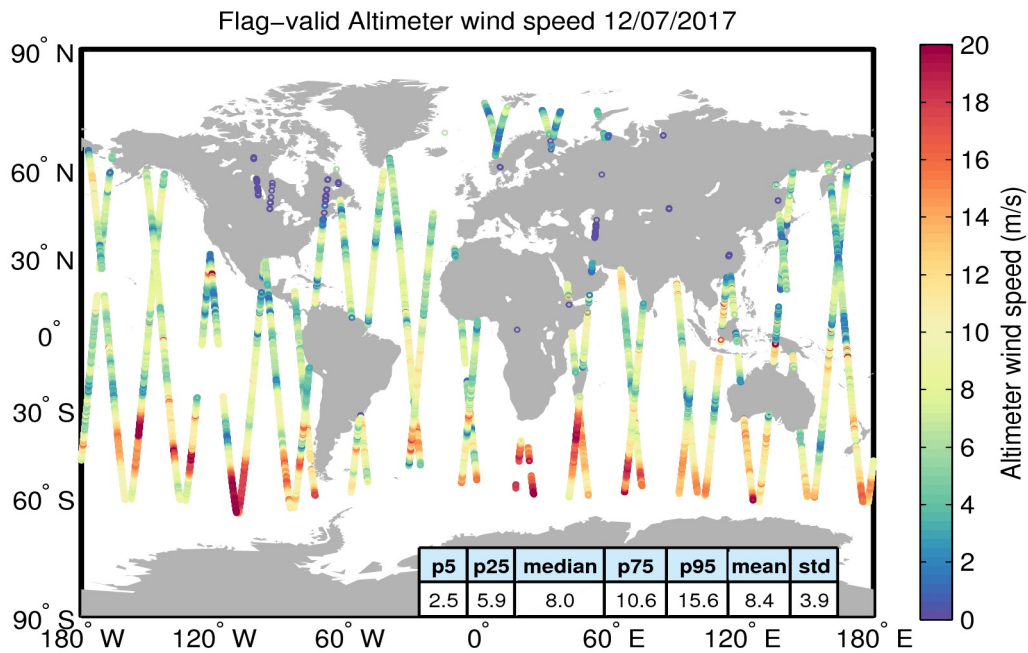
Figure 31. Geographical distribution of flag-valid wind data over oceans and lakes for 12/07/2017. The statistical values shown in the table refer to the wind in m/s and are calculated over all measurements shown in the figure.
