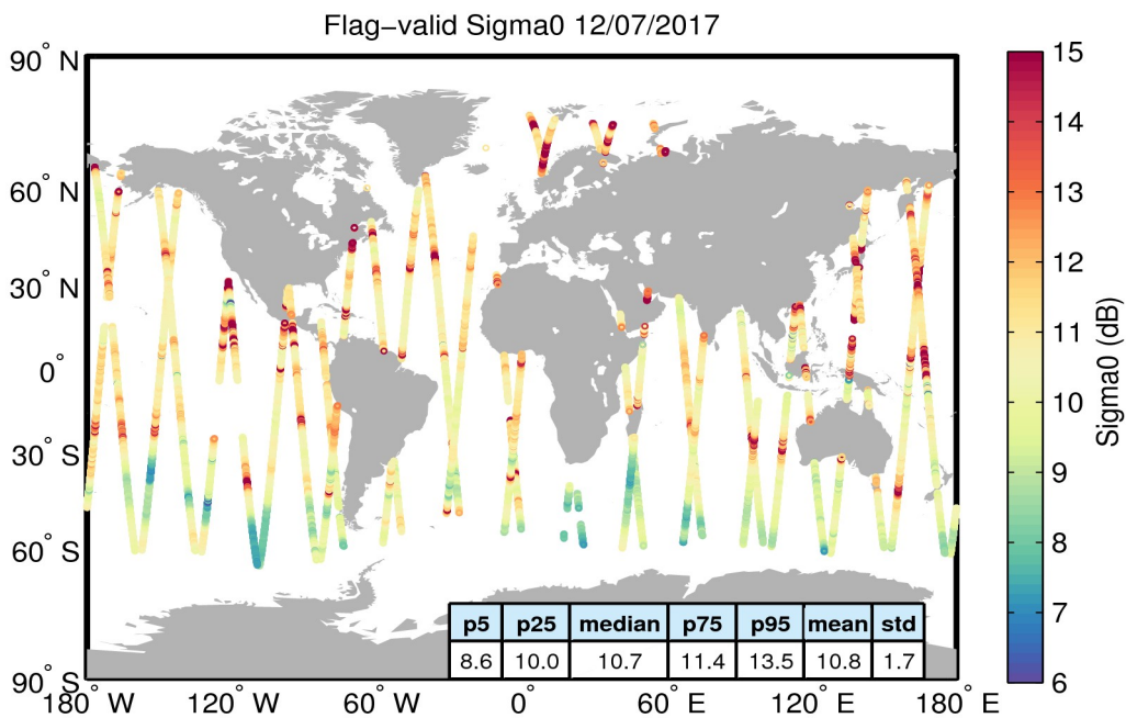
Figure 23. Geographical distribution of flag-valid sigma0 data over oceans and lakes for 12/07/2017. The statistical values shown in the table refer to the sigma0 in dB and are calculated over all measurements shown in the figure.
