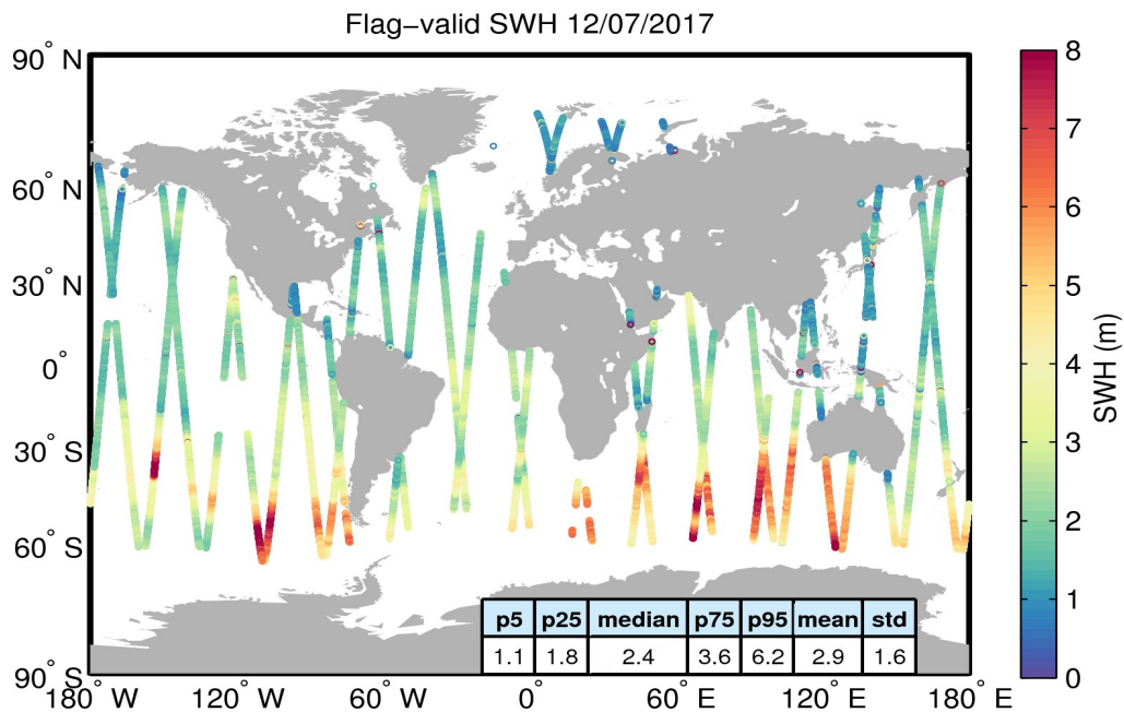
Figure 15. Geographical distribution of flag-valid SWH data over oceans and lakes for 12/07/2017. The statistical values shown in the table refer to the SWH in m and are calculated over all measurements shown in the figure.
