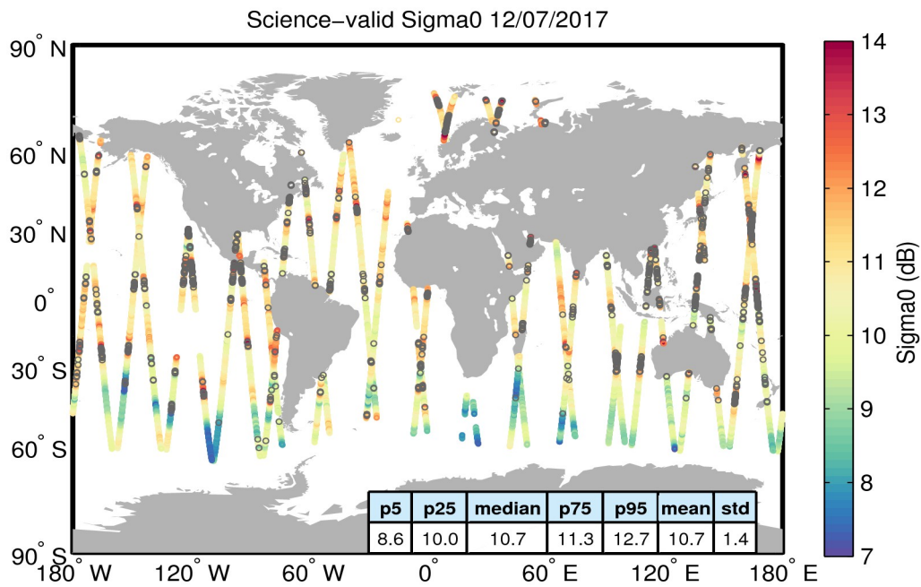
Figure 27. Geographical distribution of science-valid sigma0 data over oceans and lakes for 12/07/2017. The statistical values shown in the table refer to the sigma0 in dB and are calculated over all measurements shown in the figure. Gray circles denote records that have been rejected based on the editing criteria described in Table 4.
