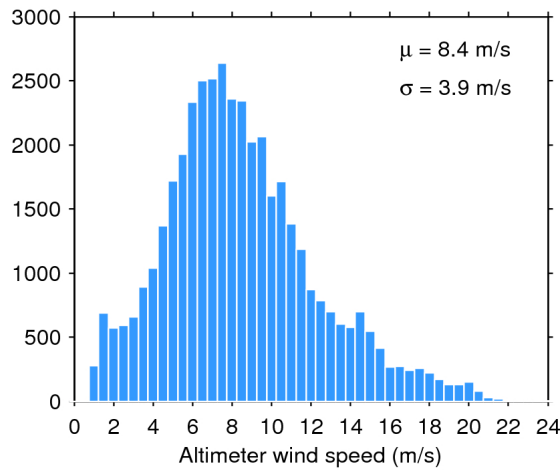
Figure 33. Histogram of flag-valid wind over oceans and lakes for 12/07/2017. The mean ( \mu ) and standard deviation ( \sigma ) are also shown. Note that values larger than 24 m/s are excluded from the histogram for the sake of readability but not from the computation of \mu and \sigma .
