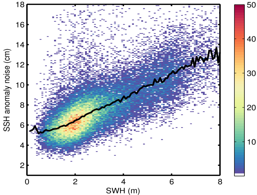
Figure 9. 2D histogram showing flag-valid SSH anomaly noise as a function of SWH for 12/07/2017. The black line denotes the median SSH anomaly noise as a function of SWH.
