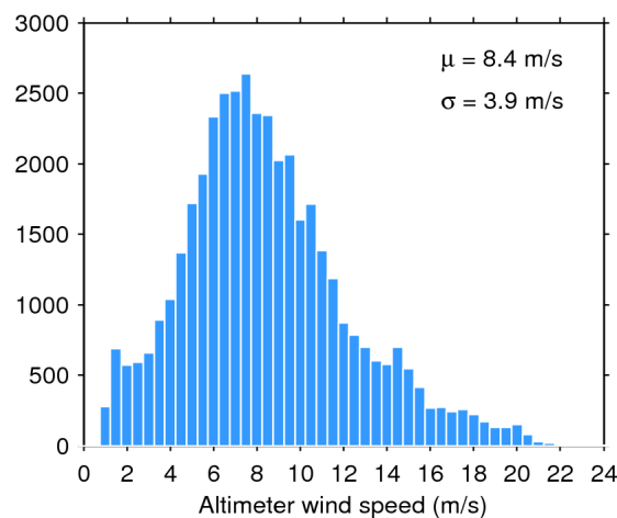
Figure 35. Histogram of science-valid wind over oceans and lakes for 12/07/2017. The mean ( \mu ) and standard deviation ( \sigma ) are also shown. Note that values larger than 24 m/s are excluded from the histogram for the sake of readability but not from the computation of \mu and \sigma .
