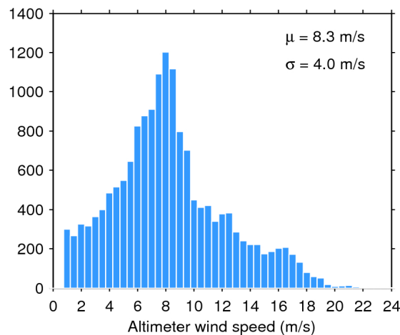
Figure 35. Histogram of science-valid wind over oceans and lakes for 11/07/2017. The mean ( \mu ) and standard deviation ( \sigma ) are also shown. Note that values larger than 24 m/s are excluded from the histogram for the sake of readability but not from the computation of \mu and \sigma .
