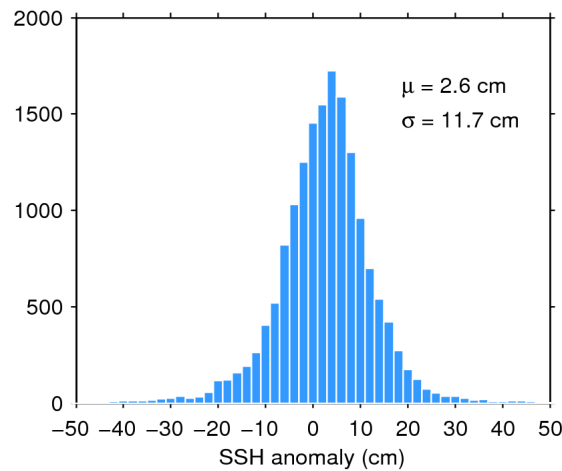
Figure 7. Histogram of flag-valid SSH anomaly over oceans and lakes for 11/07/2017. The mean ( \mu ) and standard deviation ( \sigma ) are also shown. Note that values outside [-50 50] cm are excluded from the histogram for the sake of readability but not from the computation of \mu and \sigma .
