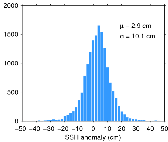
Figure 11. Histogram of science-valid SSH anomaly over oceans and lakes for 11/07/2017. The mean ( \mu ) and standard deviation ( \sigma ) are also shown. Note that values outside [-50 50] cm are excluded from the histogram for the sake of readability but not from the computation of \mu and \sigma .
