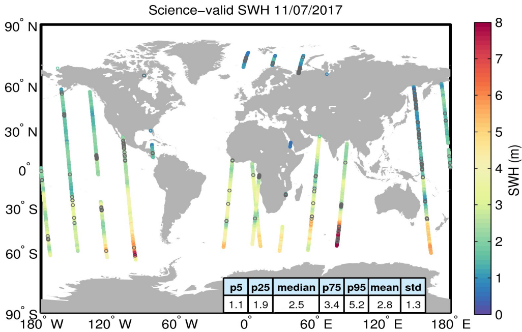
Figure 19. Geographical distribution of science-valid SWH data over oceans and lakes for 11/07/2017. The statistical values shown in the table refer to the SWH in m and are calculated over all measurements shown in the figure. Gray circles denote records that have been rejected based on the editing criteria described in Table 3.
