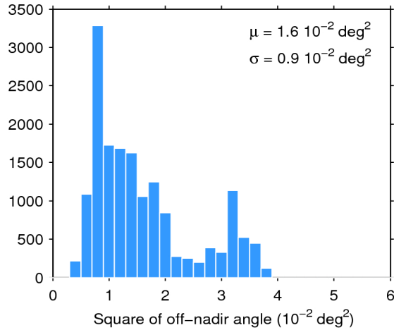
Figure 39. Histogram of flag-valid mispointing over oceans and lakes for 11/07/2017. The mean ( \mu ) and standard deviation ( \sigma ) are also shown. Note that values larger than 6 \cdot 10^{-2} \text{ deg}^2 are excluded from the histogram for the sake of readability but not from the computation of \mu and \sigma .
