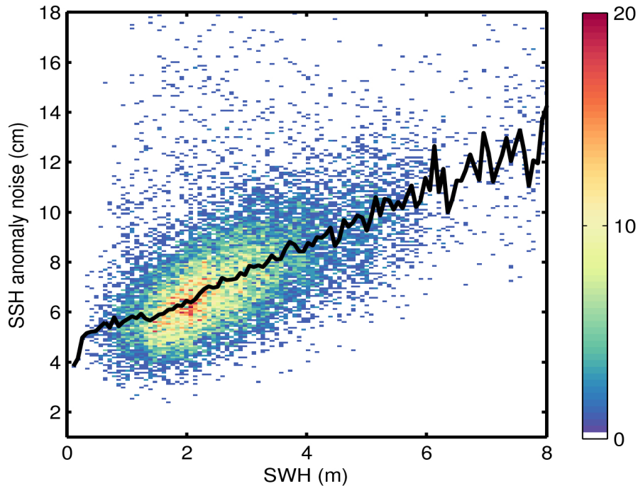
Figure 9. 2D histogram showing flag-valid SSH anomaly noise as a function of SWH for 11/07/2017. The black line denotes the median SSH anomaly noise as a function of SWH.
