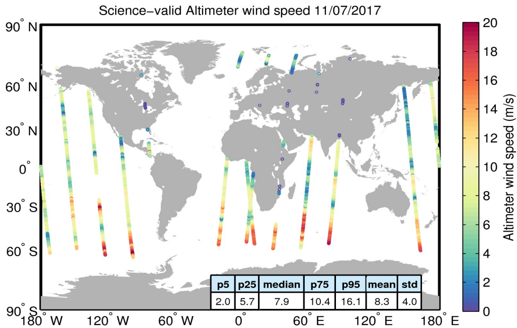
Figure 34. Geographical distribution of science-valid wind data over oceans and lakes for 11/07/2017. The statistical values shown in the table refer to the wind in m/s and are calculated over all measurements shown in the figure. Gray circles denote records that have been rejected based on the editing criteria described in Table 5.
