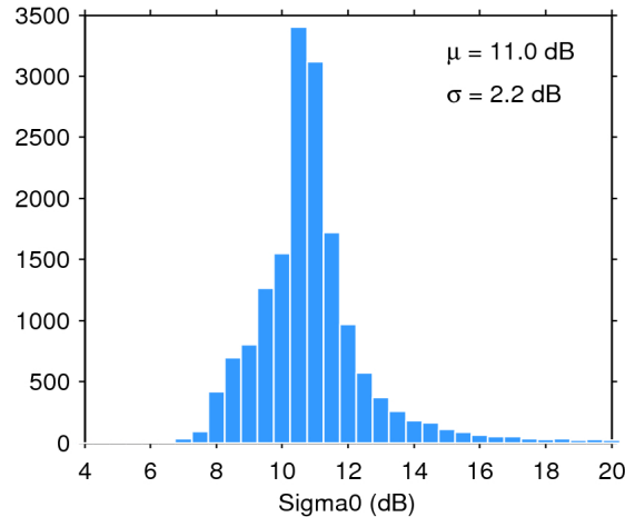
Figure 25. Histogram of flag-valid sigma0 over oceans and lakes for 11/07/2017. The mean ( \mu ) and standard deviation ( \sigma ) are also shown. Note that values outside [4 20] dB are excluded from the histogram for the sake of readability but not from the computation of \mu and \sigma .
