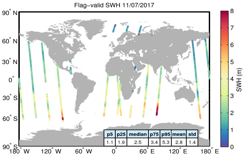
Figure 15. Geographical distribution of flag-valid SWH data over oceans and lakes for 11/07/2017. The statistical values shown in the table refer to the SWH in m and are calculated over all measurements shown in the figure.
