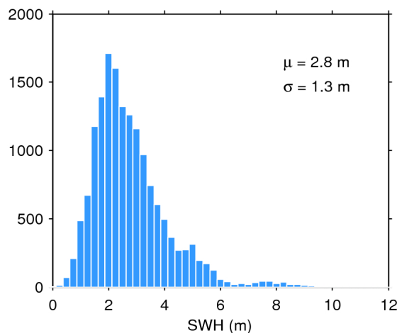
Figure 20. Histogram of science-valid SWH over oceans and lakes for 11/07/2017. The mean ( \mu ) and standard deviation ( \sigma ) are also shown. Note that values larger than 12 m are excluded from the histogram for the sake of readability but not from the computation of \mu and \sigma .
