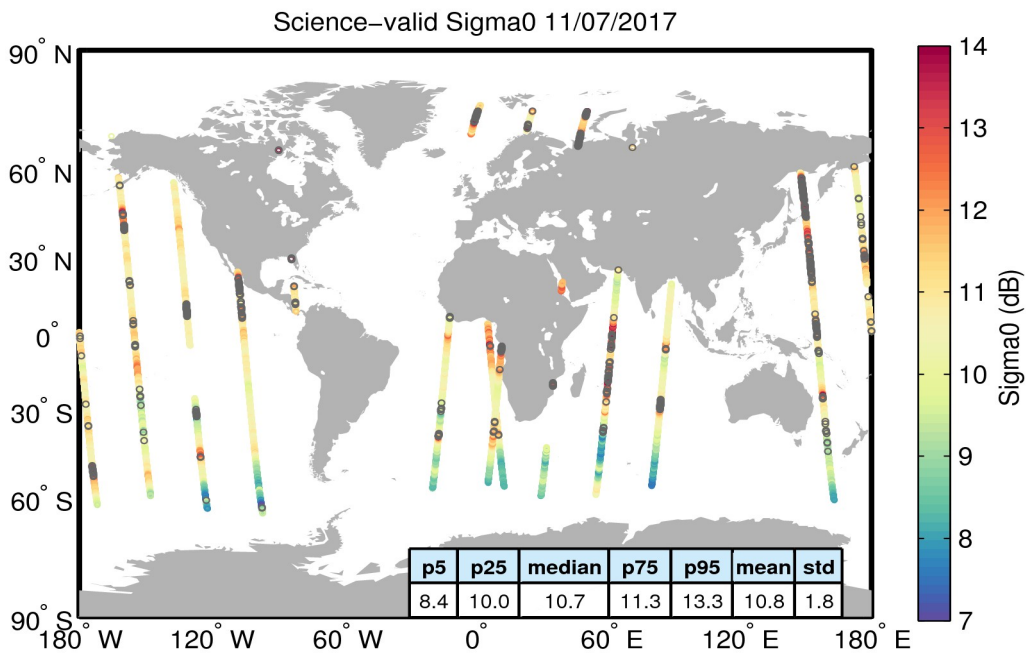
Figure 27. Geographical distribution of science-valid sigma0 data over oceans and lakes for 11/07/2017. The statistical values shown in the table refer to the sigma0 in dB and are calculated over all measurements shown in the figure. Gray circles denote records that have been rejected based on the editing criteria described in Table 4.
