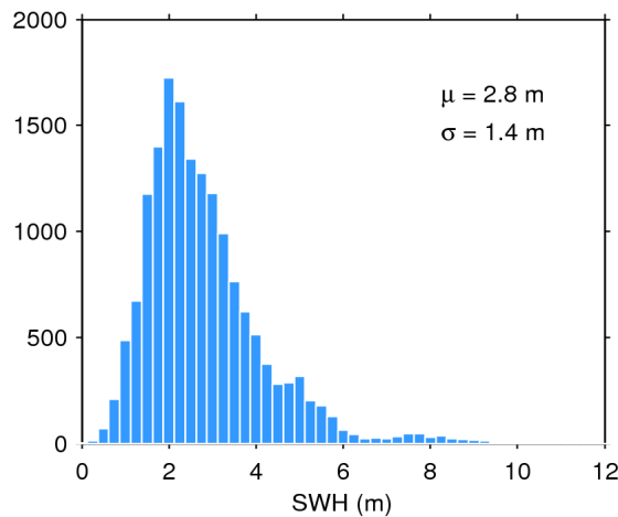
Figure 17. Histogram of flag-valid SWH over oceans and lakes for 11/07/2017. The mean ( \mu ) and standard deviation ( \sigma ) are also shown. Note that values larger than 12 m are excluded from the histogram for the sake of readability but not from the computation of \mu and \sigma .
