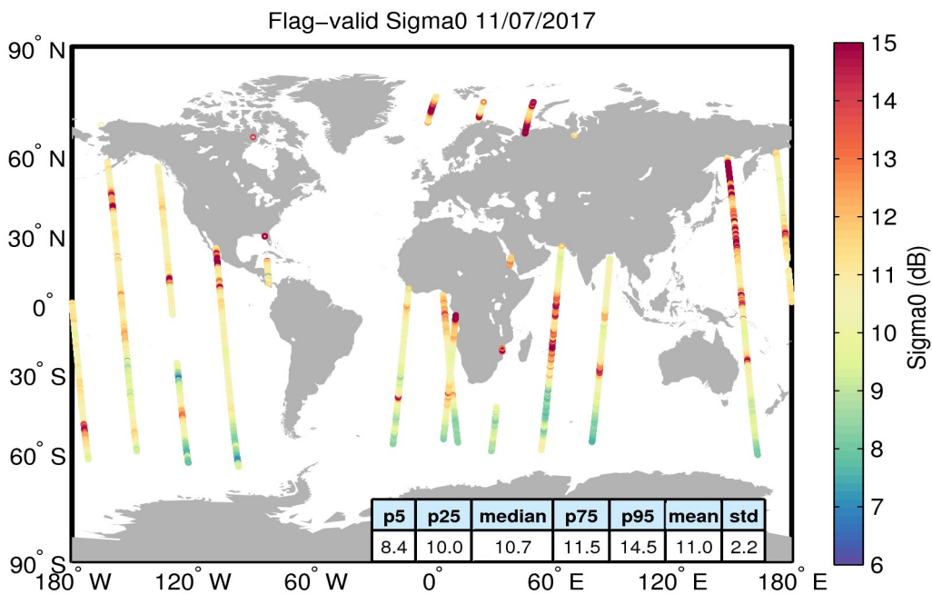
Figure 23. Geographical distribution of flag-valid sigma0 data over oceans and lakes for 11/07/2017. The statistical values shown in the table refer to the sigma0 in dB and are calculated over all measurements shown in the figure.
