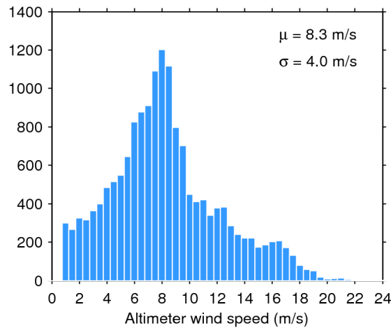
Figure 33. Histogram of flag-valid wind over oceans and lakes for 11/07/2017. The mean ( \mu ) and standard deviation ( \sigma ) are also shown. Note that values larger than 24 m/s are excluded from the histogram for the sake of readability but not from the computation of \mu and \sigma .
