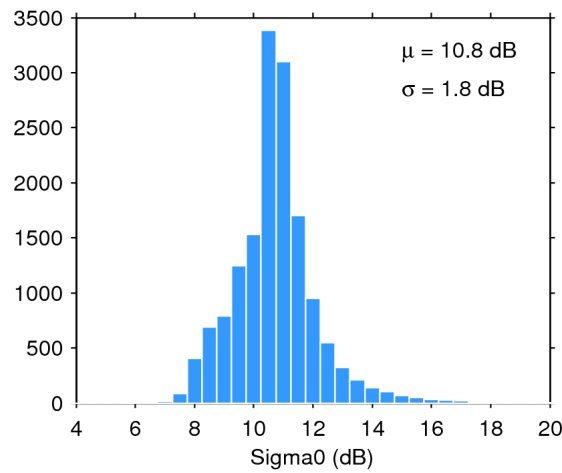
Figure 28. Histogram of science-valid sigma0 over oceans and lakes for 11/07/2017. The mean ( \mu ) and standard deviation ( \sigma ) are also shown. Note that values outside [4 20] dB are excluded from the histogram for the sake of readability but not from the computation of \mu and \sigma .
