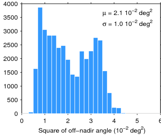
Figure 39. Histogram of flag-valid mispointing over oceans and lakes for 10/07/2017. The mean ( \mu ) and standard deviation ( \sigma ) are also shown. Note that values larger than 6 \cdot 10^{-2} \text{ deg}^2 are excluded from the histogram for the sake of readability but not from the computation of \mu and \sigma .
