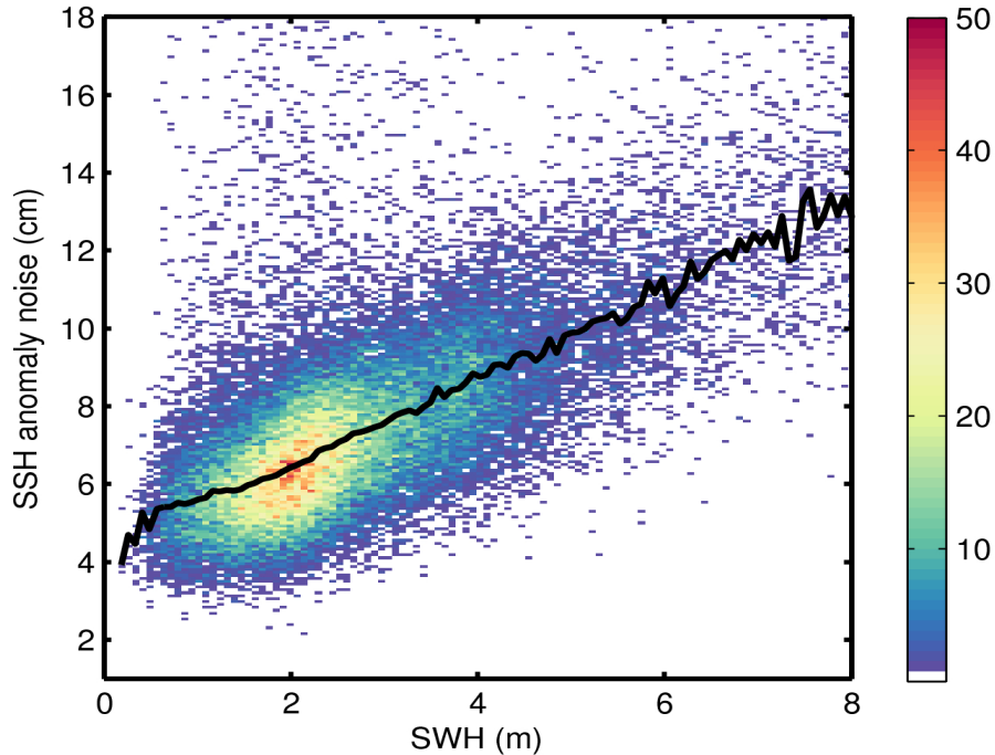
Figure 9. 2D histogram showing flag-valid SSH anomaly noise as a function of SWH for 10/07/2017. The black line denotes the median SSH anomaly noise as a function of SWH.
