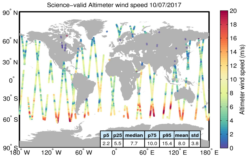
Figure 34. Geographical distribution of science-valid wind data over oceans and lakes for 10/07/2017. The statistical values shown in the table refer to the wind in m/s and are calculated over all measurements shown in the figure. Gray circles denote records that have been rejected based on the editing criteria described in Table 5.
