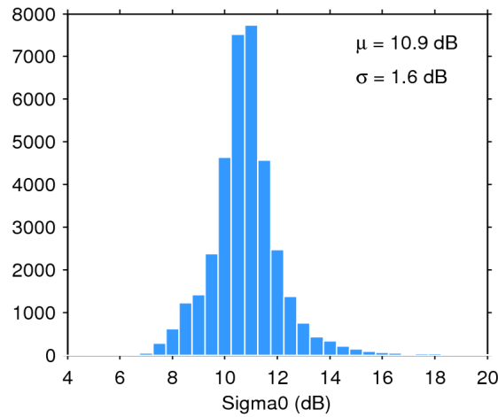
Figure 28. Histogram of science-valid sigma0 over oceans and lakes for 10/07/2017. The mean ( \mu ) and standard deviation ( \sigma ) are also shown. Note that values outside [4 20] dB are excluded from the histogram for the sake of readability but not from the computation of \mu and \sigma .
