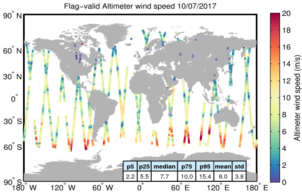
Figure 31. Geographical distribution of flag-valid wind data over oceans and lakes for 10/07/2017. The statistical values shown in the table refer to the wind in m/s and are calculated over all measurements shown in the figure.
