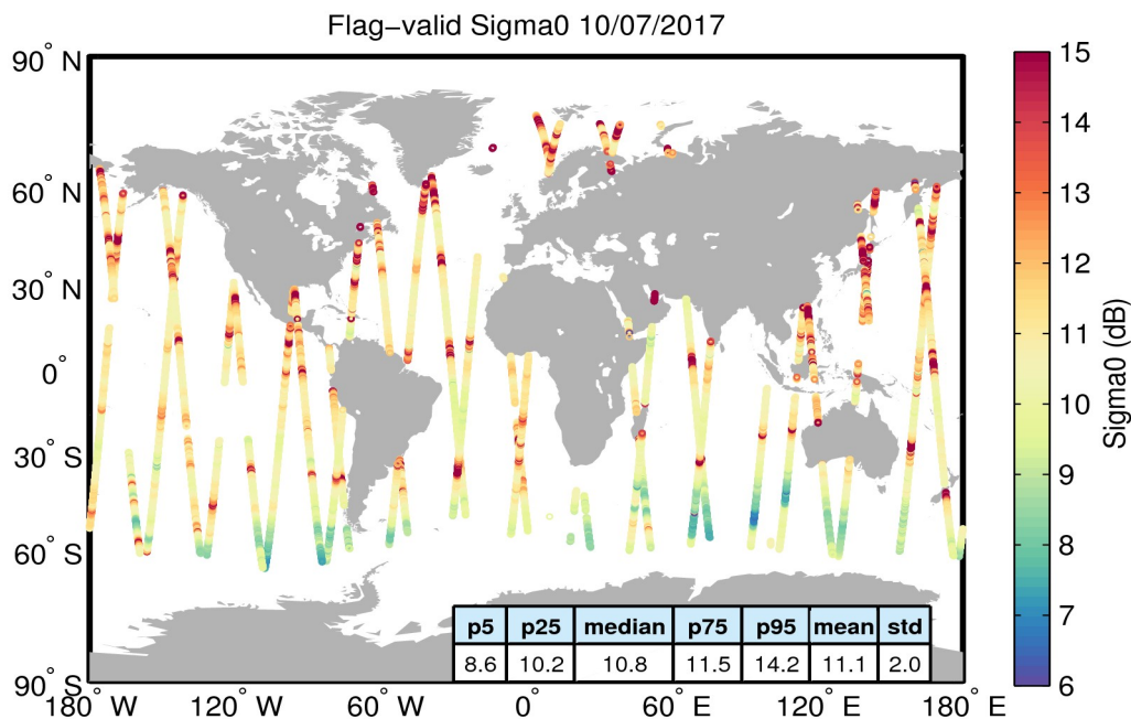
Figure 23. Geographical distribution of flag-valid sigma0 data over oceans and lakes for 10/07/2017. The statistical values shown in the table refer to the sigma0 in dB and are calculated over all measurements shown in the figure.
