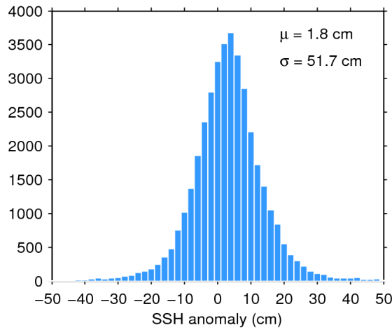
Figure 7. Histogram of flag-valid SSH anomaly over oceans and lakes for 10/07/2017. The mean ( \mu ) and standard deviation ( \sigma ) are also shown. Note that values outside [-50 50] cm are excluded from the histogram for the sake of readability but not from the computation of \mu and \sigma .
