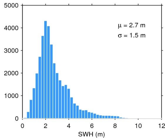
Figure 17. Histogram of flag-valid SWH over oceans and lakes for 10/07/2017. The mean ( \mu ) and standard deviation ( \sigma ) are also shown. Note that values larger than 12 m are excluded from the histogram for the sake of readability but not from the computation of \mu and \sigma .
