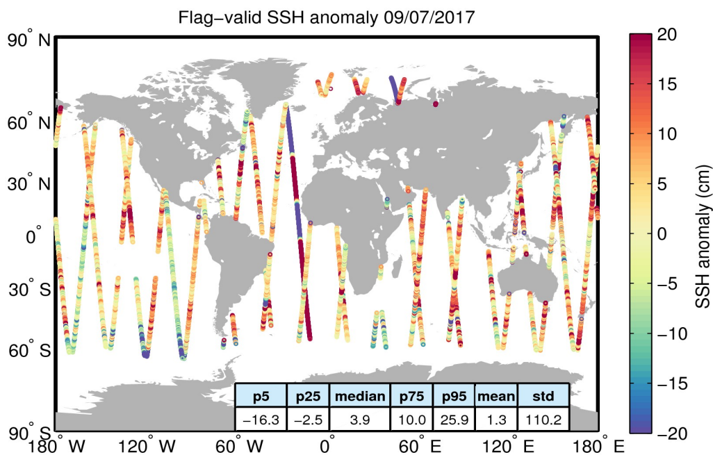
Figure 5. Geographical distribution of flag-valid 1-Hz SSH anomaly data over oceans and lakes for 09/07/2017. The statistical values shown in the table refer to the SSH anomaly in cm and are calculated over all measurements shown in the figure.
