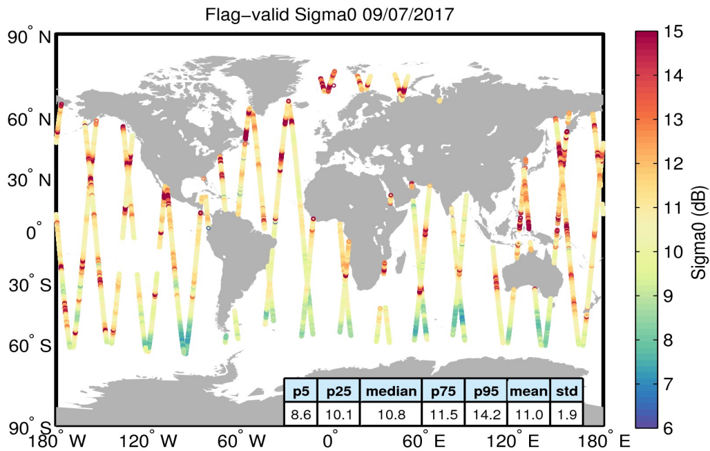
Figure 23. Geographical distribution of flag-valid sigma0 data over oceans and lakes for 09/07/2017. The statistical values shown in the table refer to the sigma0 in dB and are calculated over all measurements shown in the figure.
