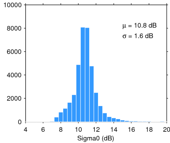
Figure 28. Histogram of science-valid sigma0 over oceans and lakes for 09/07/2017. The mean ( \mu ) and standard deviation ( \sigma ) are also shown. Note that values outside [4 20] dB are excluded from the histogram for the sake of readability but not from the computation of \mu and \sigma .
