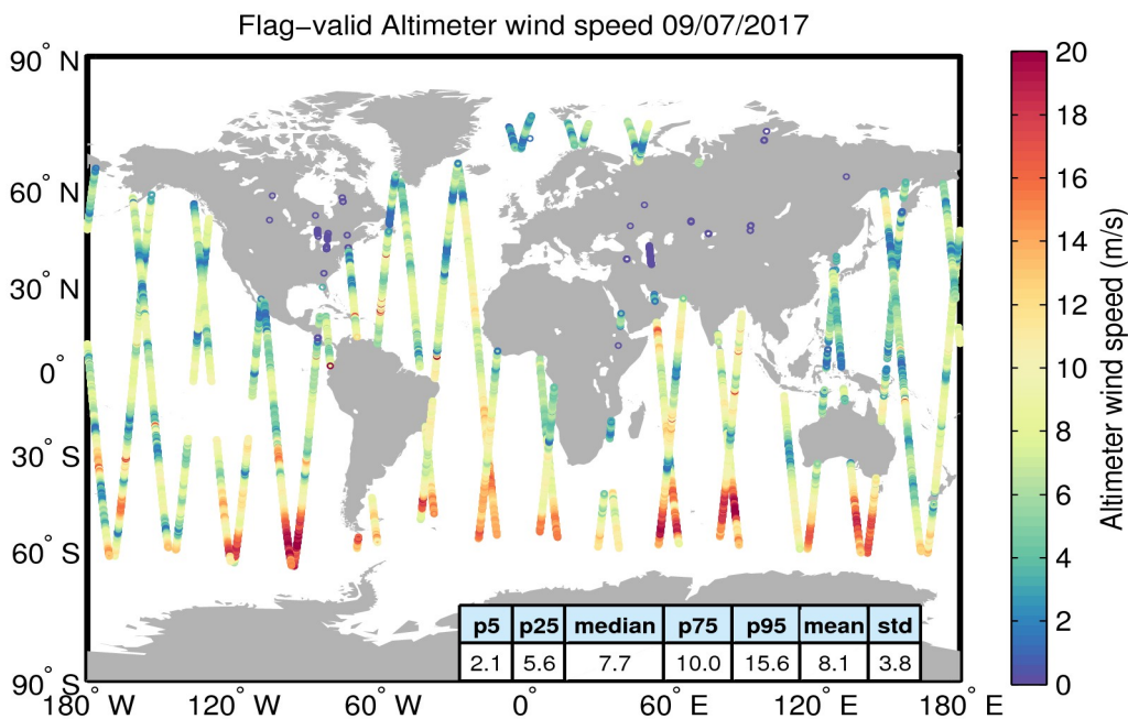
Figure 31. Geographical distribution of flag-valid wind data over oceans and lakes for 09/07/2017. The statistical values shown in the table refer to the wind in m/s and are calculated over all measurements shown in the figure.
