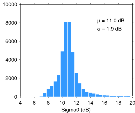
Figure 25. Histogram of flag-valid sigma0 over oceans and lakes for 09/07/2017. The mean ( \mu ) and standard deviation ( \sigma ) are also shown. Note that values outside [4 20] dB are excluded from the histogram for the sake of readability but not from the computation of \mu and \sigma .
