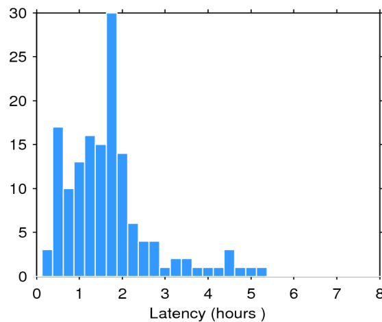
Figure 2. Histogram of the data latency for 09/07/2017. The y-axis denotes the number of files that are made available with a delay of x-hours with respect to the mean time of the records stored in the file.
