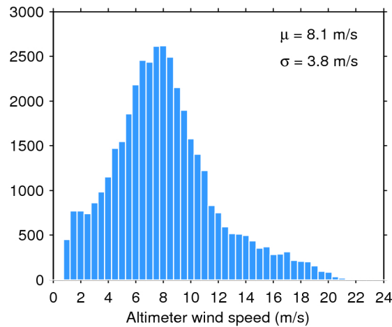
Figure 33. Histogram of flag-valid wind over oceans and lakes for 09/07/2017. The mean ( \mu ) and standard deviation ( \sigma ) are also shown. Note that values larger than 24 m/s are excluded from the histogram for the sake of readability but not from the computation of \mu and \sigma .
