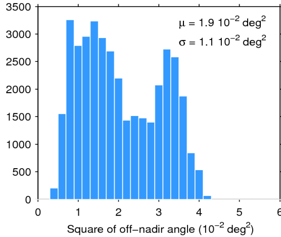
Figure 39. Histogram of flag-valid mispointing over oceans and lakes for 09/07/2017. The mean ( \mu ) and standard deviation ( \sigma ) are also shown. Note that values larger than 6 \cdot 10^{-2} \text{ deg}^2 are excluded from the histogram for the sake of readability but not from the computation of \mu and \sigma .
