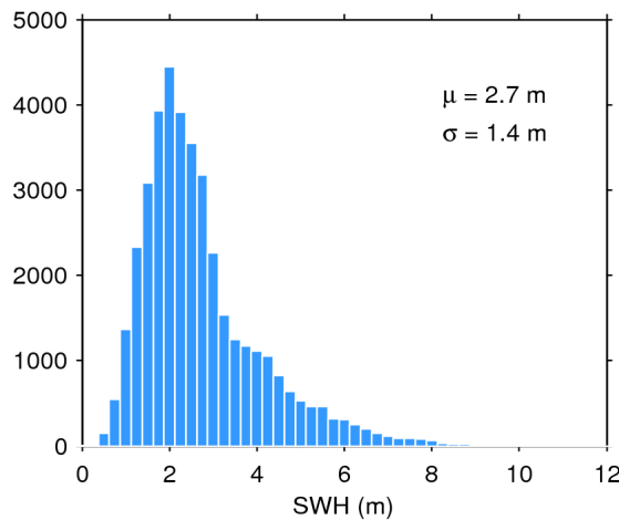
Figure 20. Histogram of science-valid SWH over oceans and lakes for 09/07/2017. The mean ( \mu ) and standard deviation ( \sigma ) are also shown. Note that values larger than 12 m are excluded from the histogram for the sake of readability but not from the computation of \mu and \sigma .
