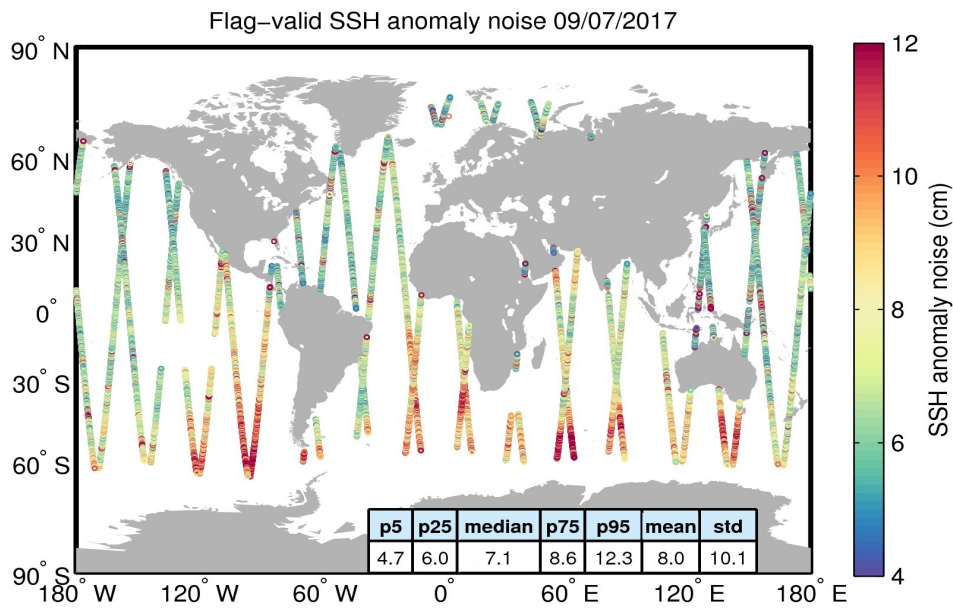
Figure 8. Geographical distribution of flag-valid 20-Hz SSH anomaly measurement noise over oceans and lakes for 09/07/2017. The statistical values shown in the table refer to the SSH anomaly noise and are calculated over all measurements shown in the figure.
