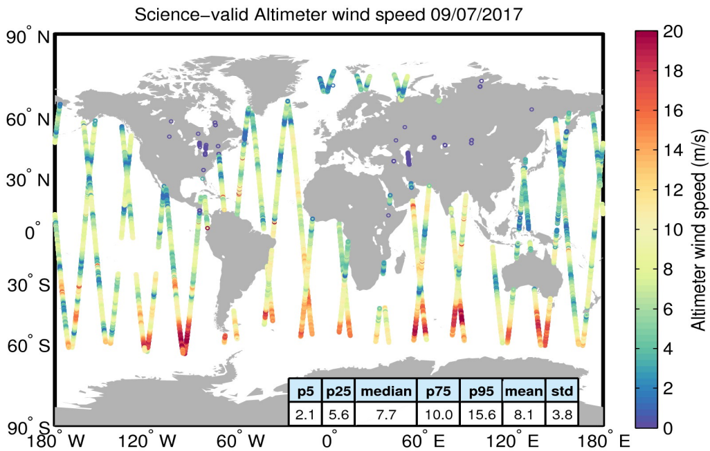
Figure 34. Geographical distribution of science-valid wind data over oceans and lakes for 09/07/2017. The statistical values shown in the table refer to the wind in m/s and are calculated over all measurements shown in the figure. Gray circles denote records that have been rejected based on the editing criteria described in Table 5.
