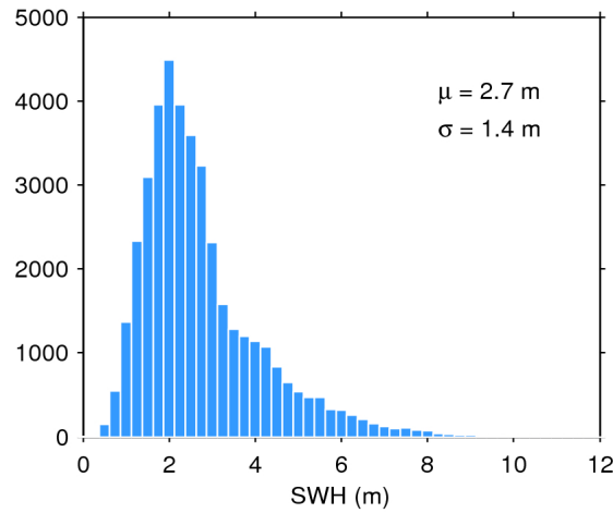
Figure 17. Histogram of flag-valid SWH over oceans and lakes for 09/07/2017. The mean ( \mu ) and standard deviation ( \sigma ) are also shown. Note that values larger than 12 m are excluded from the histogram for the sake of readability but not from the computation of \mu and \sigma .
