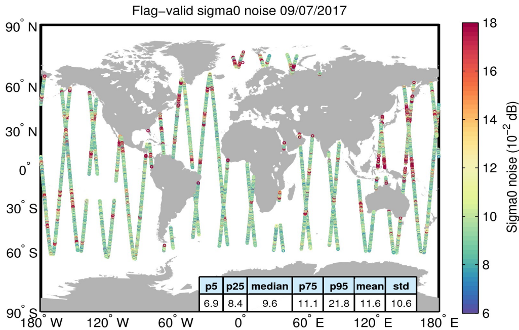
Figure 26. Geographical distribution of flag-valid 20-Hz sigma0 measurement noise over oceans and lakes for 09/07/2017. The statistical values shown in the table refer to the sigma0 noise and are calculated over all measurements shown in the figure.
