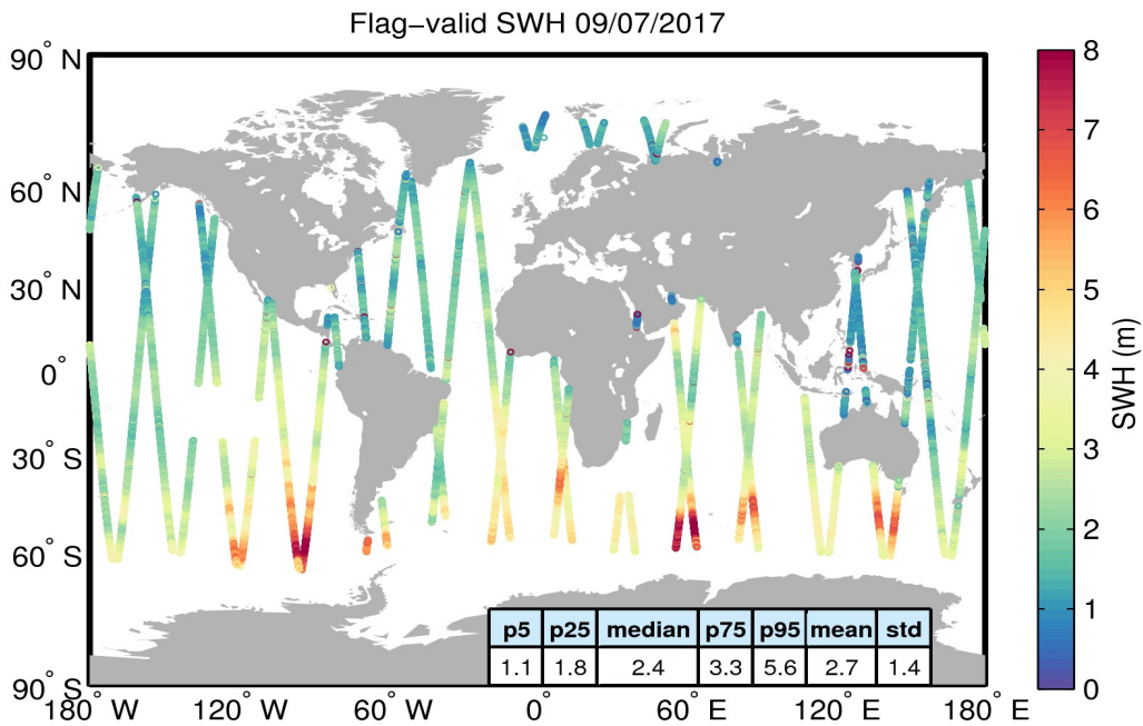
Figure 15. Geographical distribution of flag-valid SWH data over oceans and lakes for 09/07/2017. The statistical values shown in the table refer to the SWH in m and are calculated over all measurements shown in the figure.
