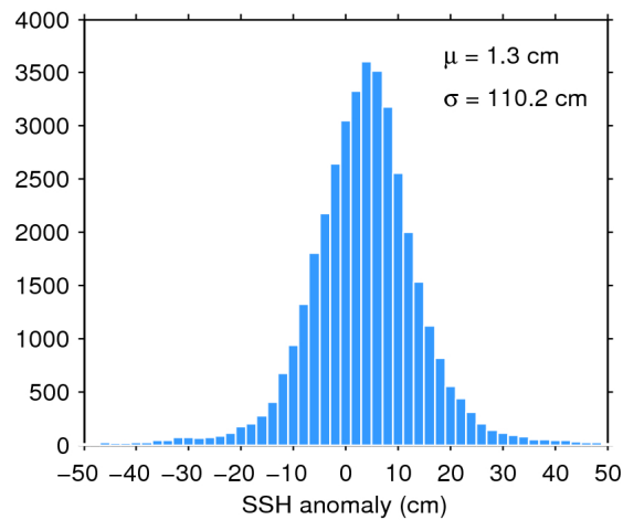
Figure 7. Histogram of flag-valid SSH anomaly over oceans and lakes for 09/07/2017. The mean ( \mu ) and standard deviation ( \sigma ) are also shown. Note that values outside [-50 50] cm are excluded from the histogram for the sake of readability but not from the computation of \mu and \sigma .
