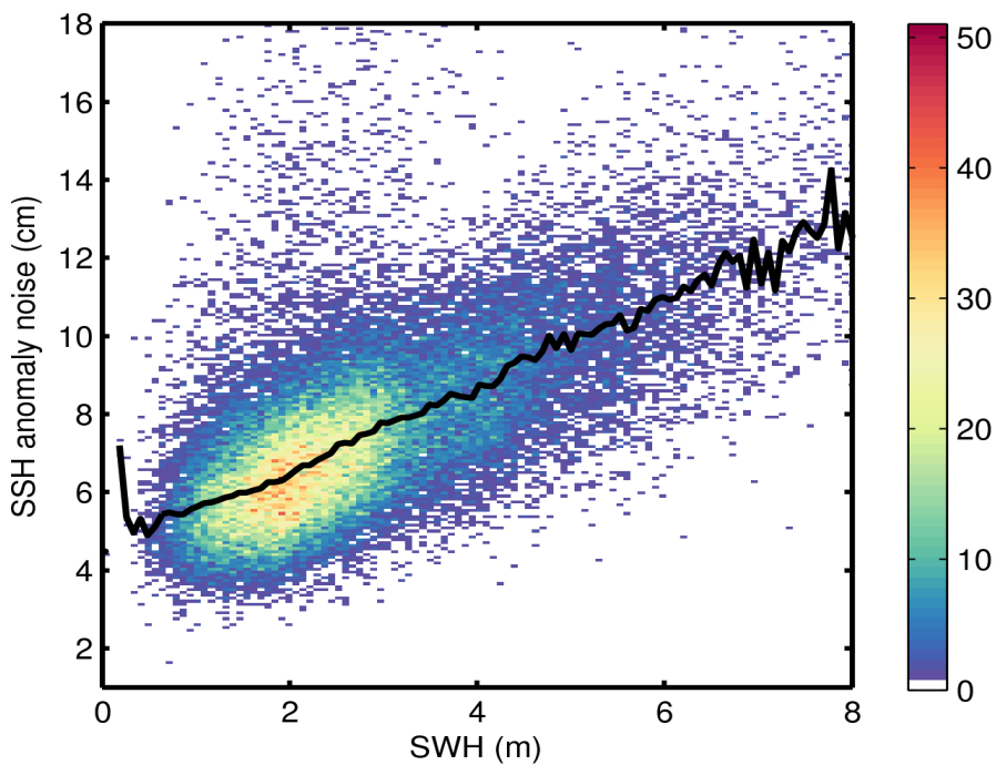
Figure 9. 2D histogram showing flag-valid SSH anomaly noise as a function of SWH for 09/07/2017. The black line denotes the median SSH anomaly noise as a function of SWH.
