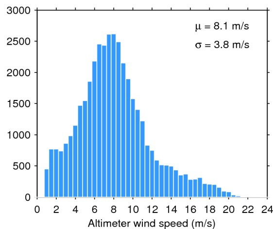
Figure 35. Histogram of science-valid wind over oceans and lakes for 09/07/2017. The mean ( \mu ) and standard deviation ( \sigma ) are also shown. Note that values larger than 24 m/s are excluded from the histogram for the sake of readability but not from the computation of \mu and \sigma .
