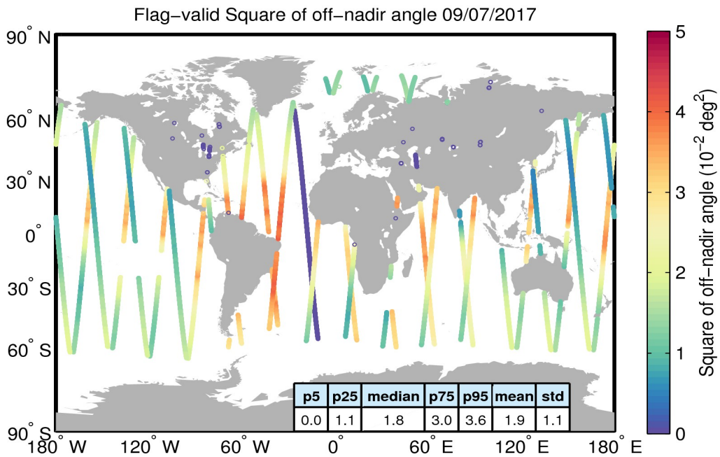
Figure 37. Geographical distribution of flag-valid mispointing data over oceans and lakes for 09/07/2017. The statistical values shown in the table refer to the mispointing in 10^{-2} deg 2 and are calculated over all measurements shown in the figure.
