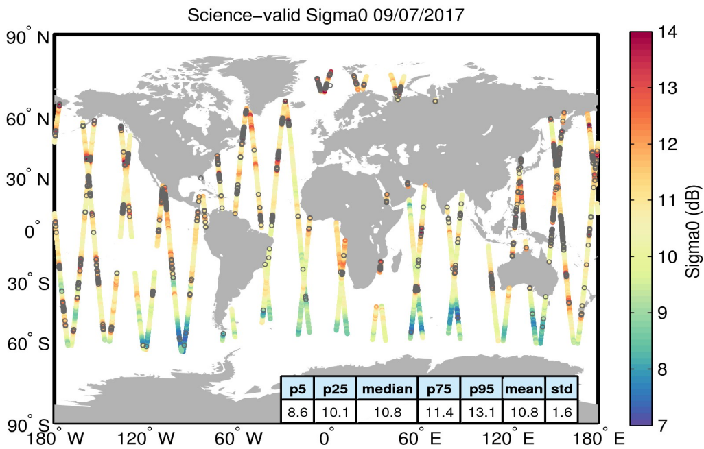
Figure 27. Geographical distribution of science-valid sigma0 data over oceans and lakes for 09/07/2017. The statistical values shown in the table refer to the sigma0 in dB and are calculated over all measurements shown in the figure. Gray circles denote records that have been rejected based on the editing criteria described in Table 4.
