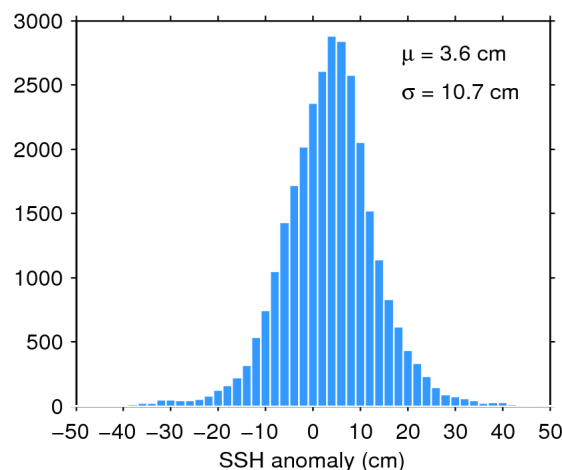
Figure 11. Histogram of science-valid SSH anomaly over oceans and lakes for 09/07/2017. The mean ( \mu ) and standard deviation ( \sigma ) are also shown. Note that values outside [-50 50] cm are excluded from the histogram for the sake of readability but not from the computation of \mu and \sigma .
