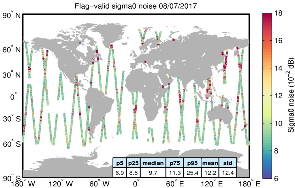
Figure 26. Geographical distribution of flag-valid 20-Hz sigma0 measurement noise over oceans and lakes for 08/07/2017. The statistical values shown in the table refer to the sigma0 noise and are calculated over all measurements shown in the figure.
