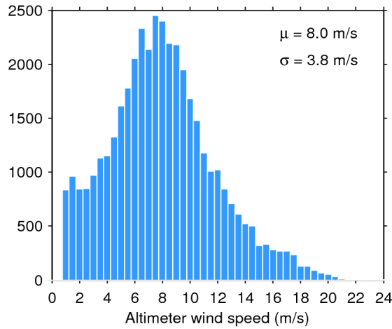
Figure 33. Histogram of flag-valid wind over oceans and lakes for 08/07/2017. The mean ( \mu ) and standard deviation ( \sigma ) are also shown. Note that values larger than 24 m/s are excluded from the histogram for the sake of readability but not from the computation of \mu and \sigma .
