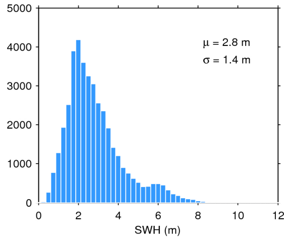
Figure 17. Histogram of flag-valid SWH over oceans and lakes for 08/07/2017. The mean ( \mu ) and standard deviation ( \sigma ) are also shown. Note that values larger than 12 m are excluded from the histogram for the sake of readability but not from the computation of \mu and \sigma .
