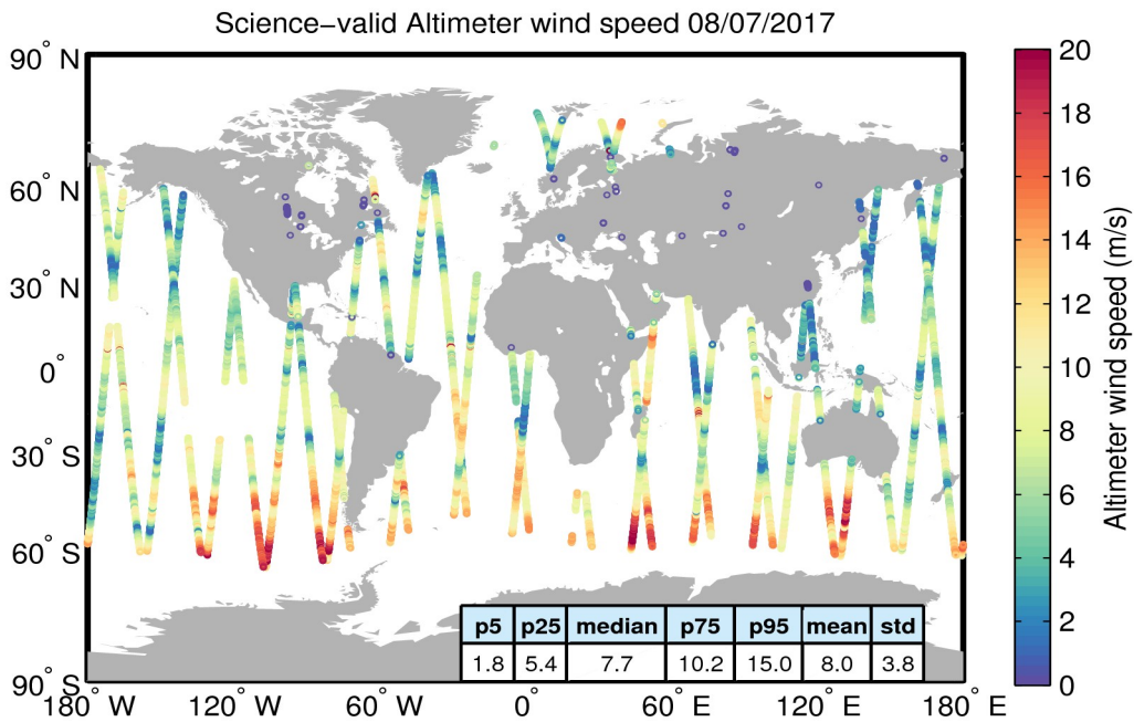
Figure 34. Geographical distribution of science-valid wind data over oceans and lakes for 08/07/2017. The statistical values shown in the table refer to the wind in m/s and are calculated over all measurements shown in the figure. Gray circles denote records that have been rejected based on the editing criteria described in Table 5.
