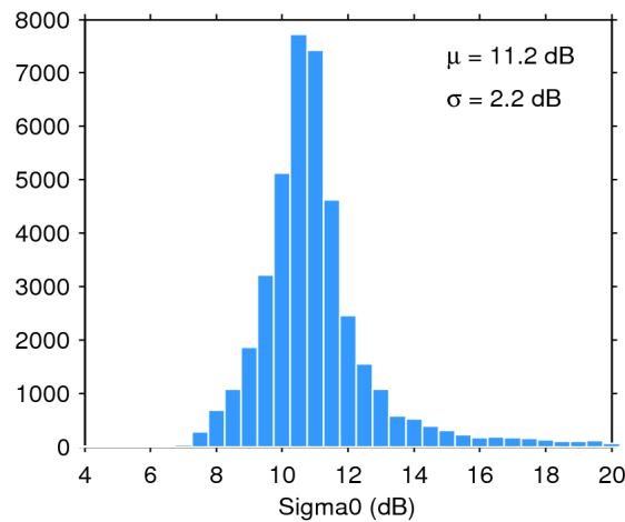
Figure 25. Histogram of flag-valid sigma0 over oceans and lakes for 08/07/2017. The mean ( \mu ) and standard deviation ( \sigma ) are also shown. Note that values outside [4 20] dB are excluded from the histogram for the sake of readability but not from the computation of \mu and \sigma .
