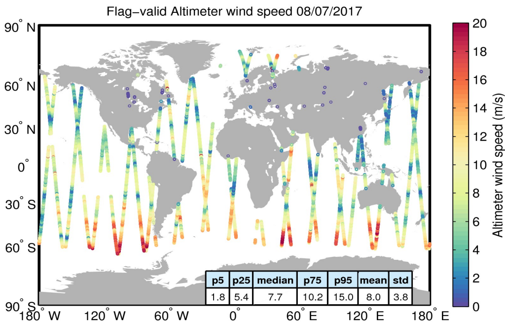
Figure 31. Geographical distribution of flag-valid wind data over oceans and lakes for 08/07/2017. The statistical values shown in the table refer to the wind in m/s and are calculated over all measurements shown in the figure.
