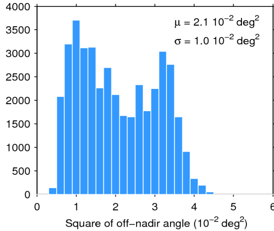
Figure 39. Histogram of flag-valid mispointing over oceans and lakes for 08/07/2017. The mean ( \mu ) and standard deviation ( \sigma ) are also shown. Note that values larger than 6 \cdot 10^{-2} \text{ deg}^2 are excluded from the histogram for the sake of readability but not from the computation of \mu and \sigma .
