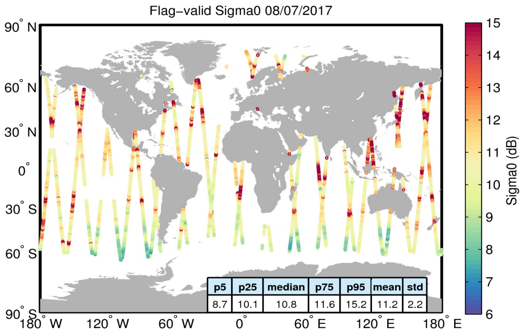
Figure 23. Geographical distribution of flag-valid sigma0 data over oceans and lakes for 08/07/2017. The statistical values shown in the table refer to the sigma0 in dB and are calculated over all measurements shown in the figure.
