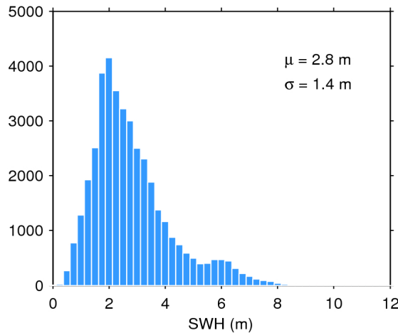
Figure 20. Histogram of science-valid SWH over oceans and lakes for 08/07/2017. The mean ( \mu ) and standard deviation ( \sigma ) are also shown. Note that values larger than 12 m are excluded from the histogram for the sake of readability but not from the computation of \mu and \sigma .
