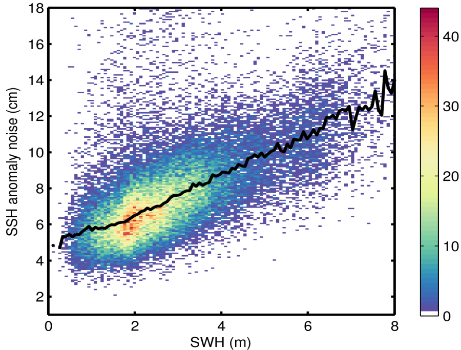
Figure 9. 2D histogram showing flag-valid SSH anomaly noise as a function of SWH for 08/07/2017. The black line denotes the median SSH anomaly noise as a function of SWH.
