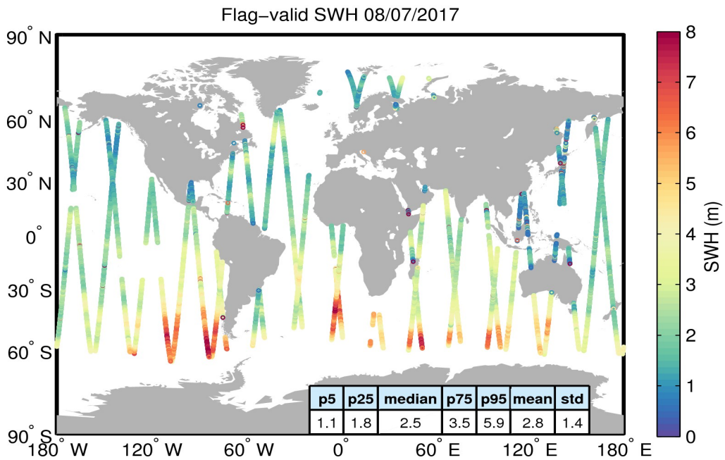
Figure 15. Geographical distribution of flag-valid SWH data over oceans and lakes for 08/07/2017. The statistical values shown in the table refer to the SWH in m and are calculated over all measurements shown in the figure.
