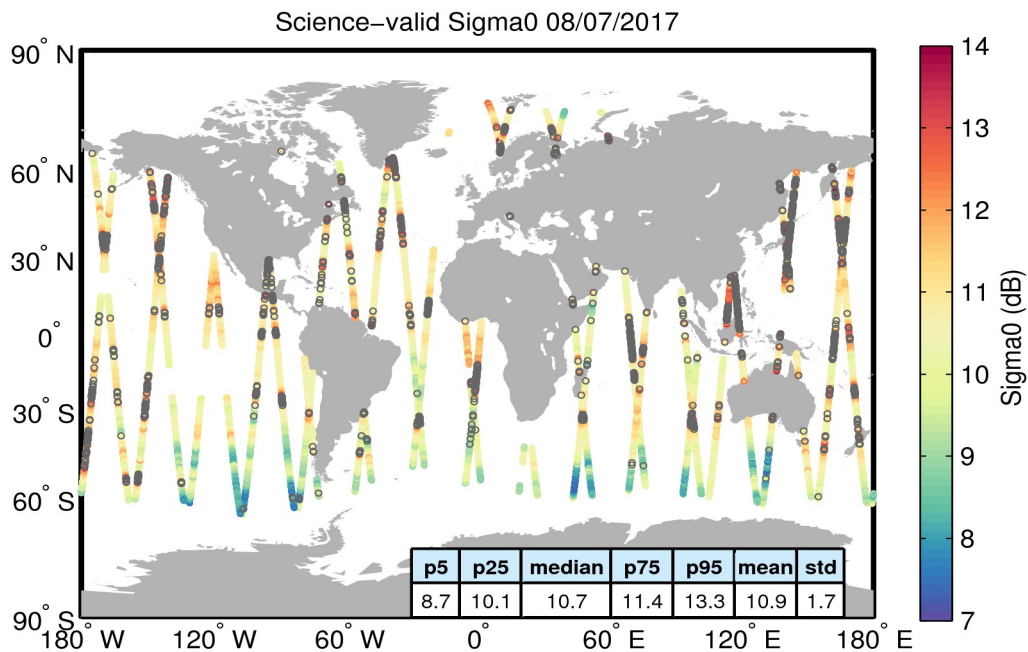
Figure 27. Geographical distribution of science-valid sigma0 data over oceans and lakes for 08/07/2017. The statistical values shown in the table refer to the sigma0 in dB and are calculated over all measurements shown in the figure. Gray circles denote records that have been rejected based on the editing criteria described in Table 4.
