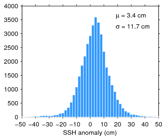
Figure 11. Histogram of science-valid SSH anomaly over oceans and lakes for 08/07/2017. The mean ( \mu ) and standard deviation ( \sigma ) are also shown. Note that values outside [-50 50] cm are excluded from the histogram for the sake of readability but not from the computation of \mu and \sigma .
