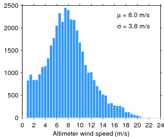
Figure 35. Histogram of science-valid wind over oceans and lakes for 08/07/2017. The mean ( \mu ) and standard deviation ( \sigma ) are also shown. Note that values larger than 24 m/s are excluded from the histogram for the sake of readability but not from the computation of \mu and \sigma .
