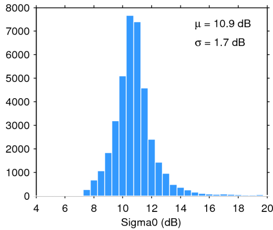
Figure 28. Histogram of science-valid sigma0 over oceans and lakes for 08/07/2017. The mean ( \mu ) and standard deviation ( \sigma ) are also shown. Note that values outside [4 20] dB are excluded from the histogram for the sake of readability but not from the computation of \mu and \sigma .
