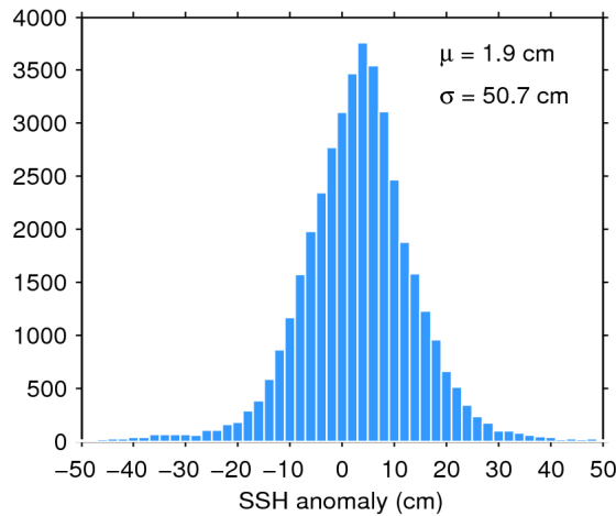
Figure 7. Histogram of flag-valid SSH anomaly over oceans and lakes for 08/07/2017. The mean ( \mu ) and standard deviation ( \sigma ) are also shown. Note that values outside [-50 50] cm are excluded from the histogram for the sake of readability but not from the computation of \mu and \sigma .
