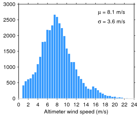
Figure 33. Histogram of flag-valid wind over oceans and lakes for 07/07/2017. The mean ( \mu ) and standard deviation ( \sigma ) are also shown. Note that values larger than 24 m/s are excluded from the histogram for the sake of readability but not from the computation of \mu and \sigma .
