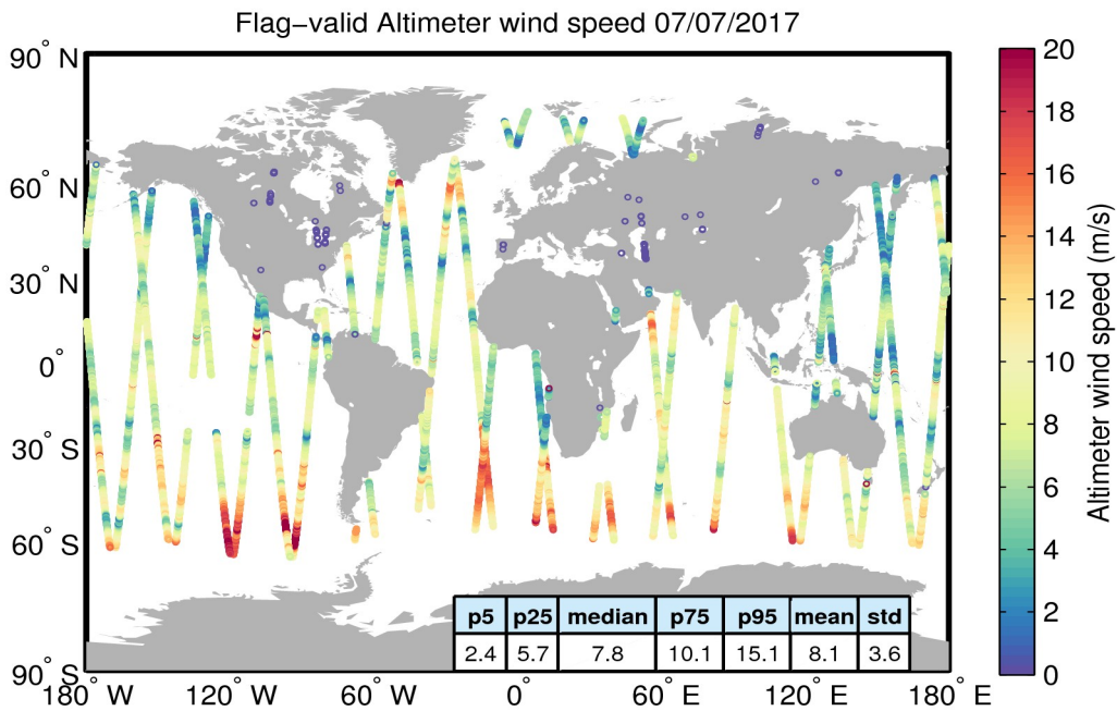
Figure 31. Geographical distribution of flag-valid wind data over oceans and lakes for 07/07/2017. The statistical values shown in the table refer to the wind in m/s and are calculated over all measurements shown in the figure.
