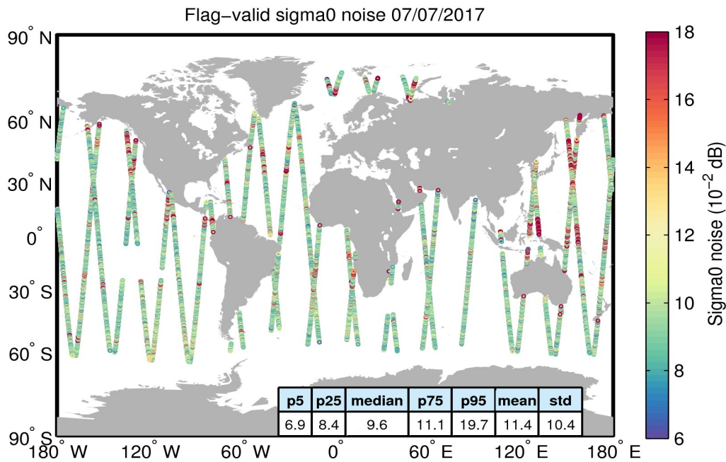
Figure 26. Geographical distribution of flag-valid 20-Hz sigma0 measurement noise over oceans and lakes for 07/07/2017. The statistical values shown in the table refer to the sigma0 noise and are calculated over all measurements shown in the figure.
