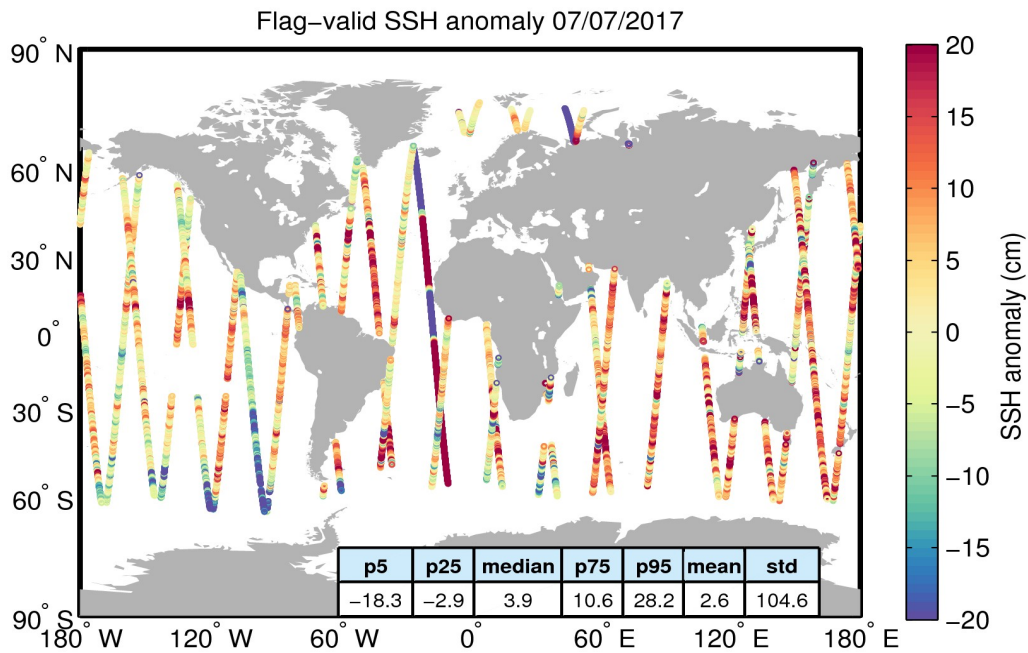
Figure 5. Geographical distribution of flag-valid 1-Hz SSH anomaly data over oceans and lakes for 07/07/2017. The statistical values shown in the table refer to the SSH anomaly in cm and are calculated over all measurements shown in the figure.
