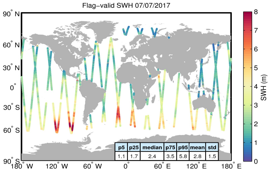
Figure 15. Geographical distribution of flag-valid SWH data over oceans and lakes for 07/07/2017. The statistical values shown in the table refer to the SWH in m and are calculated over all measurements shown in the figure.
