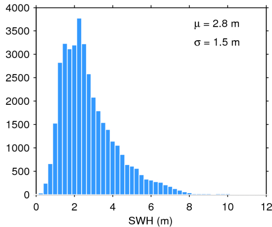
Figure 20. Histogram of science-valid SWH over oceans and lakes for 07/07/2017. The mean ( \mu ) and standard deviation ( \sigma ) are also shown. Note that values larger than 12 m are excluded from the histogram for the sake of readability but not from the computation of \mu and \sigma .
