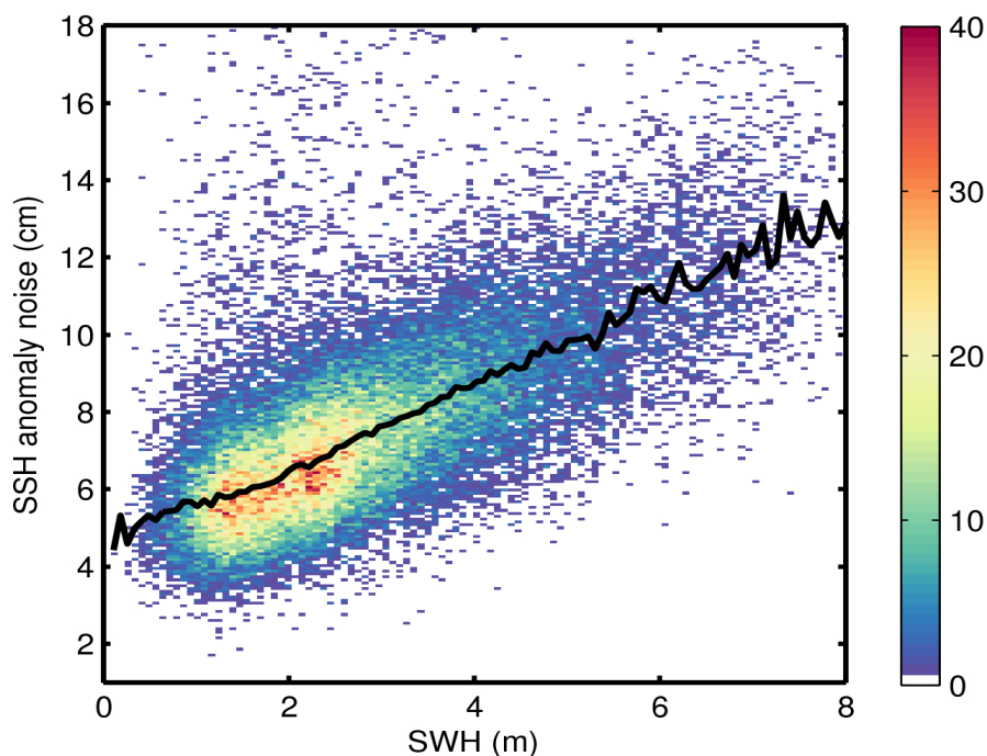
Figure 9. 2D histogram showing flag-valid SSH anomaly noise as a function of SWH for 07/07/2017. The black line denotes the median SSH anomaly noise as a function of SWH.
