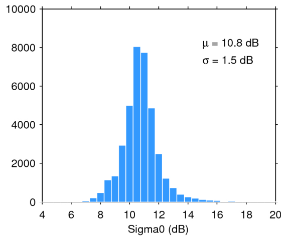
Figure 28. Histogram of science-valid sigma0 over oceans and lakes for 07/07/2017. The mean ( \mu ) and standard deviation ( \sigma ) are also shown. Note that values outside [4 20] dB are excluded from the histogram for the sake of readability but not from the computation of \mu and \sigma .
