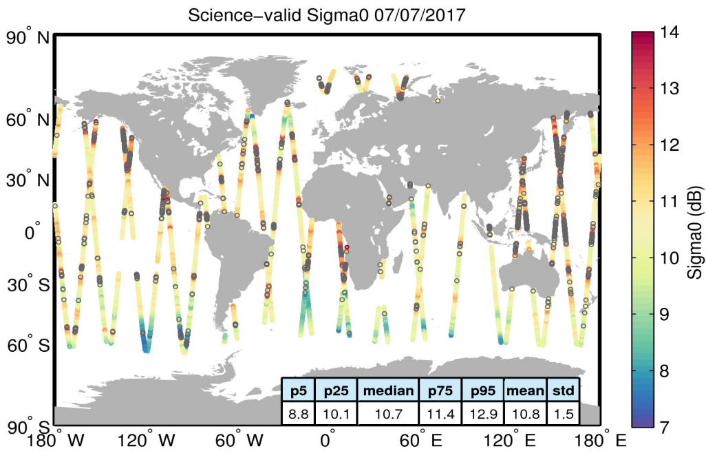
Figure 27. Geographical distribution of science-valid sigma0 data over oceans and lakes for 07/07/2017. The statistical values shown in the table refer to the sigma0 in dB and are calculated over all measurements shown in the figure. Gray circles denote records that have been rejected based on the editing criteria described in Table 4.
