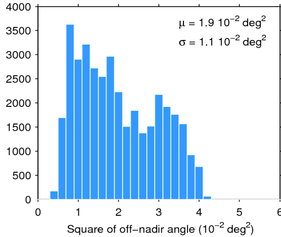
Figure 39. Histogram of flag-valid mispointing over oceans and lakes for 07/07/2017. The mean ( \mu ) and standard deviation ( \sigma ) are also shown. Note that values larger than 6 \cdot 10^{-2} \text{ deg}^2 are excluded from the histogram for the sake of readability but not from the computation of \mu and \sigma .
