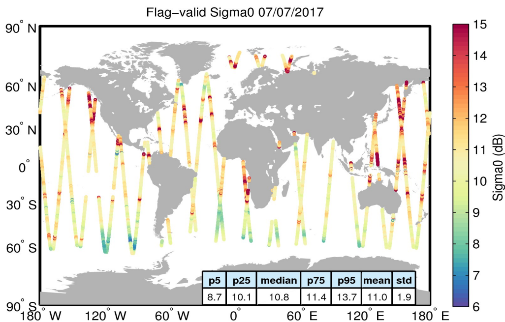
Figure 23. Geographical distribution of flag-valid sigma0 data over oceans and lakes for 07/07/2017. The statistical values shown in the table refer to the sigma0 in dB and are calculated over all measurements shown in the figure.
