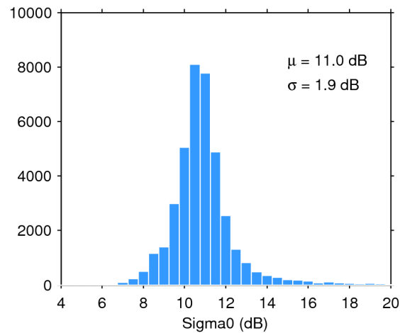
Figure 25. Histogram of flag-valid sigma0 over oceans and lakes for 07/07/2017. The mean ( \mu ) and standard deviation ( \sigma ) are also shown. Note that values outside [4 20] dB are excluded from the histogram for the sake of readability but not from the computation of \mu and \sigma .
