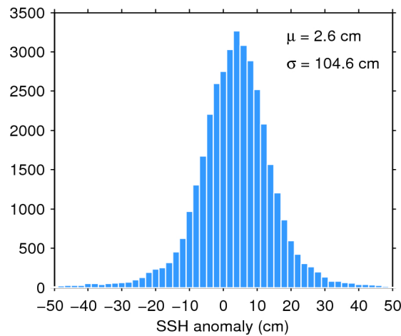
Figure 7. Histogram of flag-valid SSH anomaly over oceans and lakes for 07/07/2017. The mean ( \mu ) and standard deviation ( \sigma ) are also shown. Note that values outside [-50 50] cm are excluded from the histogram for the sake of readability but not from the computation of \mu and \sigma .
