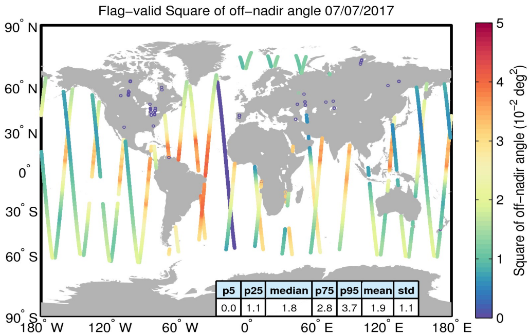
Figure 37. Geographical distribution of flag-valid mispointing data over oceans and lakes for 07/07/2017. The statistical values shown in the table refer to the mispointing in 10^{-2} deg 2 and are calculated over all measurements shown in the figure.
