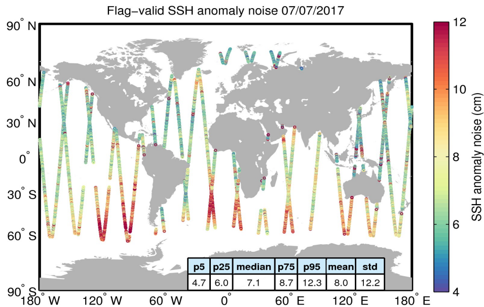
Figure 8. Geographical distribution of flag-valid 20-Hz SSH anomaly measurement noise over oceans and lakes for 07/07/2017. The statistical values shown in the table refer to the SSH anomaly noise and are calculated over all measurements shown in the figure.
