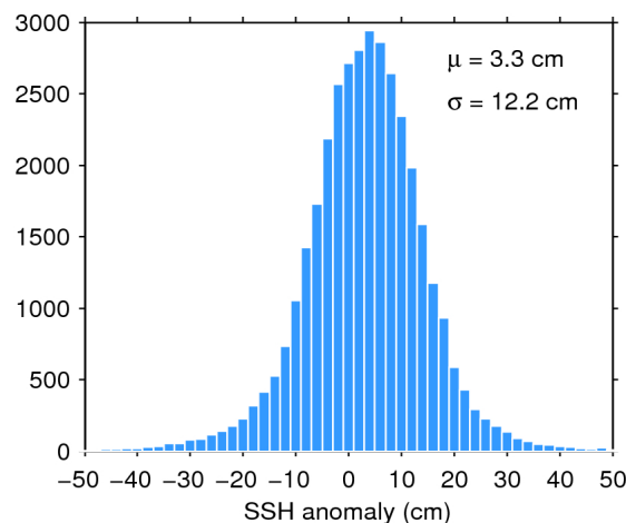
Figure 11. Histogram of science-valid SSH anomaly over oceans and lakes for 06/07/2017. The mean ( \mu ) and standard deviation ( \sigma ) are also shown. Note that values outside [-50 50] cm are excluded from the histogram for the sake of readability but not from the computation of \mu and \sigma .
