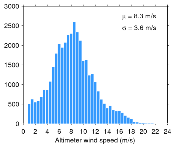
Figure 35. Histogram of science-valid wind over oceans and lakes for 06/07/2017. The mean ( \mu ) and standard deviation ( \sigma ) are also shown. Note that values larger than 24 m/s are excluded from the histogram for the sake of readability but not from the computation of \mu and \sigma .
