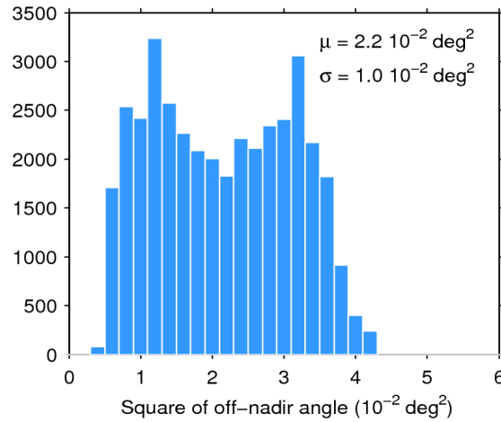
Figure 39. Histogram of flag-valid mispointing over oceans and lakes for 06/07/2017. The mean ( \mu ) and standard deviation ( \sigma ) are also shown. Note that values larger than 6 \cdot 10^{-2} \text{ deg}^2 are excluded from the histogram for the sake of readability but not from the computation of \mu and \sigma .
