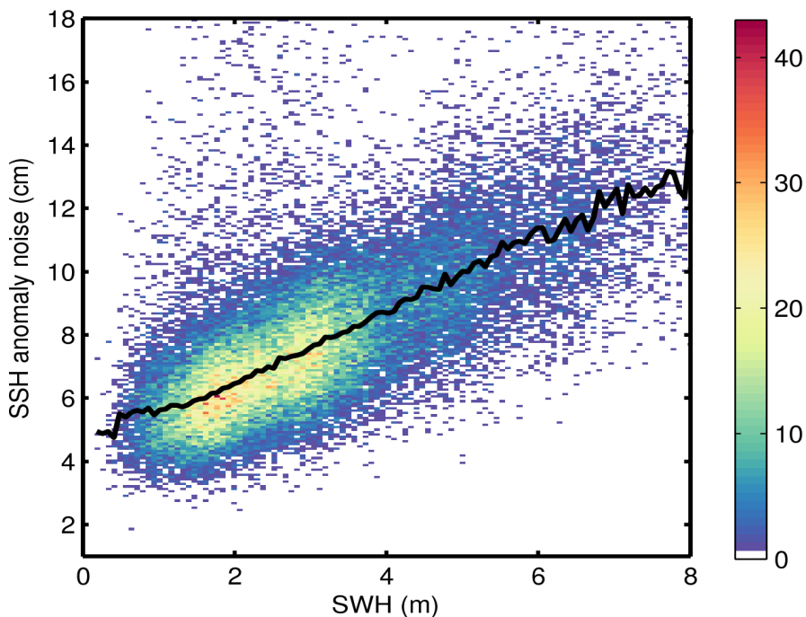
Figure 9. 2D histogram showing flag-valid SSH anomaly noise as a function of SWH for 06/07/2017. The black line denotes the median SSH anomaly noise as a function of SWH.
