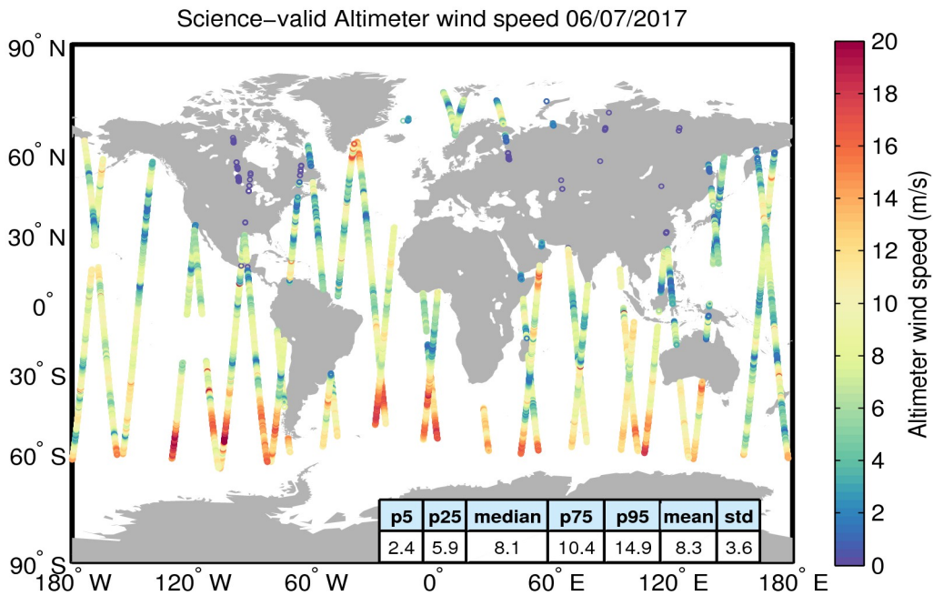
Figure 34. Geographical distribution of science-valid wind data over oceans and lakes for 06/07/2017. The statistical values shown in the table refer to the wind in m/s and are calculated over all measurements shown in the figure. Gray circles denote records that have been rejected based on the editing criteria described in Table 5.
