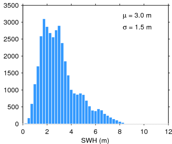
Figure 20. Histogram of science-valid SWH over oceans and lakes for 06/07/2017. The mean ( \mu ) and standard deviation ( \sigma ) are also shown. Note that values larger than 12 m are excluded from the histogram for the sake of readability but not from the computation of \mu and \sigma .
