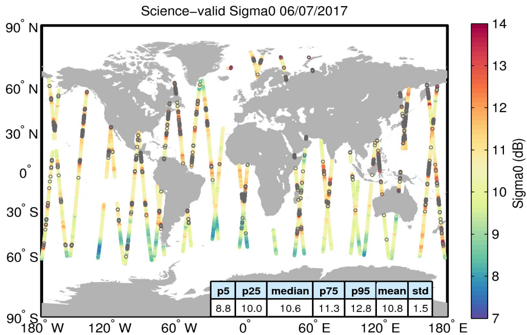
Figure 27. Geographical distribution of science-valid sigma0 data over oceans and lakes for 06/07/2017. The statistical values shown in the table refer to the sigma0 in dB and are calculated over all measurements shown in the figure. Gray circles denote records that have been rejected based on the editing criteria described in Table 4.
