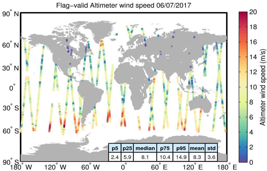
Figure 31. Geographical distribution of flag-valid wind data over oceans and lakes for 06/07/2017. The statistical values shown in the table refer to the wind in m/s and are calculated over all measurements shown in the figure.
