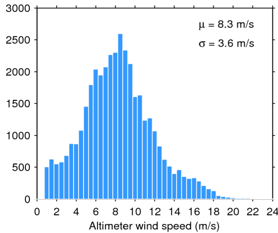
Figure 33. Histogram of flag-valid wind over oceans and lakes for 06/07/2017. The mean ( \mu ) and standard deviation ( \sigma ) are also shown. Note that values larger than 24 m/s are excluded from the histogram for the sake of readability but not from the computation of \mu and \sigma .
