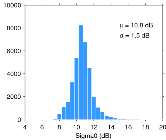
Figure 28. Histogram of science-valid sigma0 over oceans and lakes for 06/07/2017. The mean ( \mu ) and standard deviation ( \sigma ) are also shown. Note that values outside [4 20] dB are excluded from the histogram for the sake of readability but not from the computation of \mu and \sigma .
