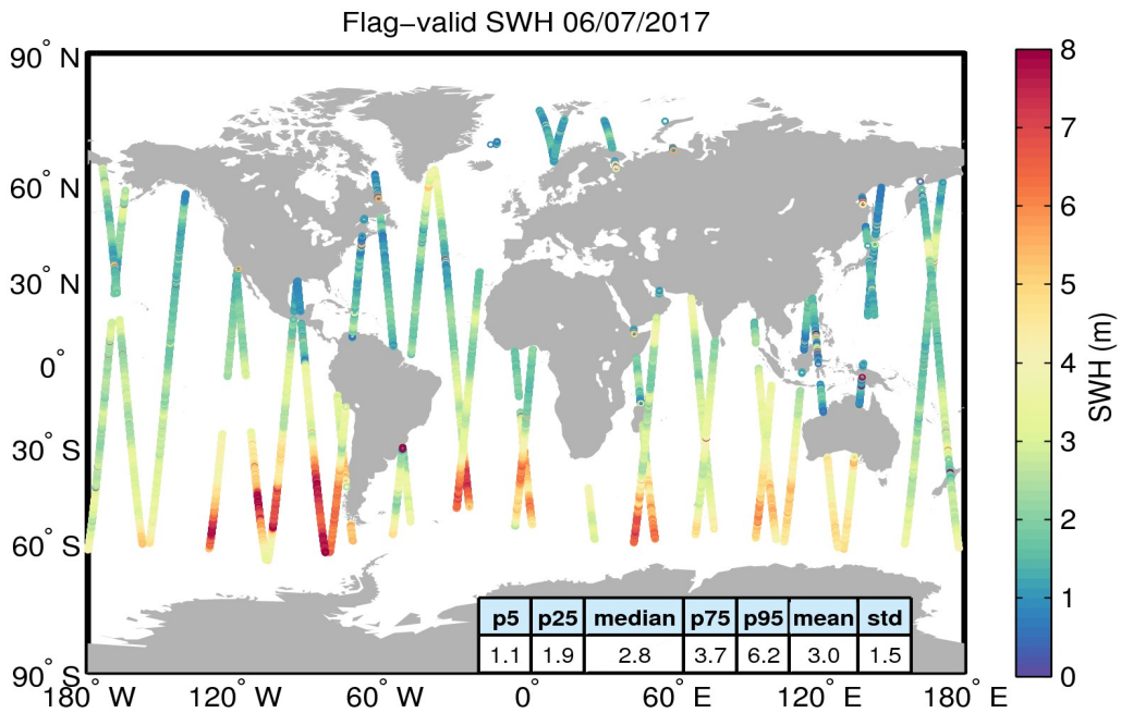
Figure 15. Geographical distribution of flag-valid SWH data over oceans and lakes for 06/07/2017. The statistical values shown in the table refer to the SWH in m and are calculated over all measurements shown in the figure.
