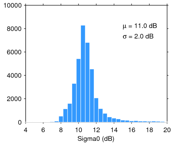
Figure 25. Histogram of flag-valid sigma0 over oceans and lakes for 06/07/2017. The mean ( \mu ) and standard deviation ( \sigma ) are also shown. Note that values outside [4 20] dB are excluded from the histogram for the sake of readability but not from the computation of \mu and \sigma .
